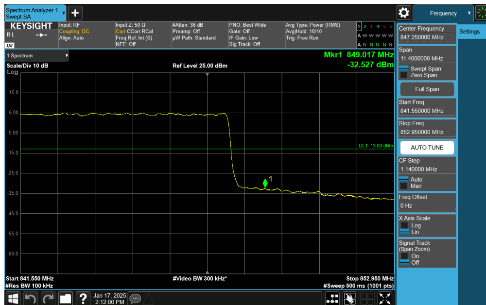
Plot 7-66. Upper BE Plot (NR Band n26 DFT-s-OFDM \pi/2 BPSK – 15.0MHz - Full RB)
