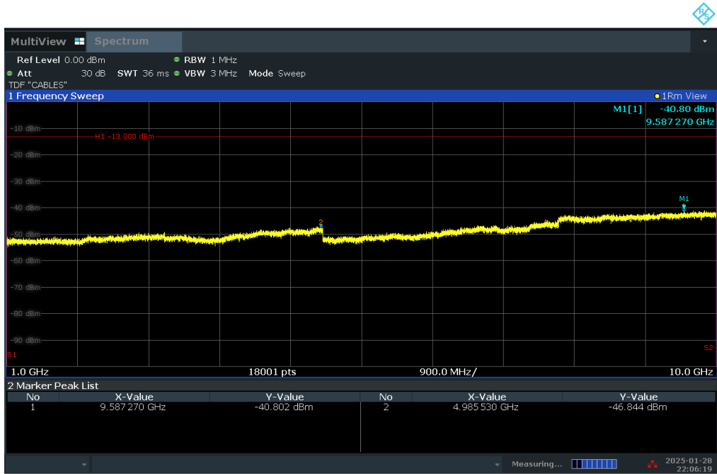
Plot 7-33. Conducted Spurious Plot (LTE Band 26/5 - 10MHz QPSK - RB Size 1, RB Offset 25 - High Channel)
