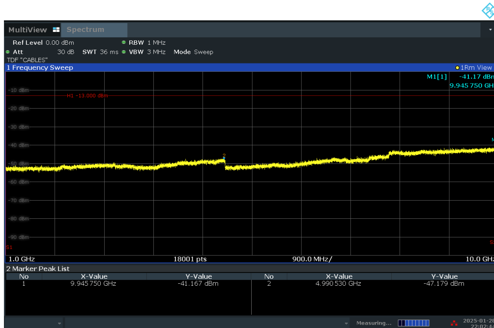
Plot 7-27. Conducted Spurious Plot (LTE Band 26/5 - 10MHz QPSK - RB Size 1, RB Offset 25 - Low Channel)
