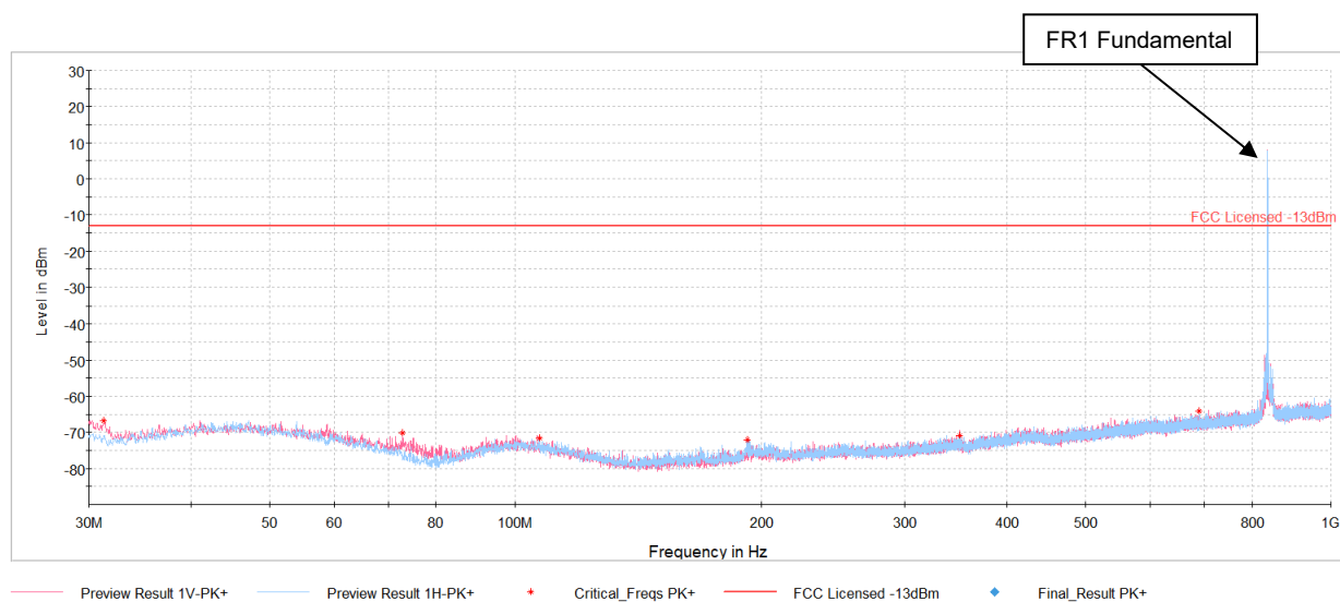
Plot 7-79. Antenna BCM Radiated Spurious Plot below 1GHz (NR Band n26/n5)
