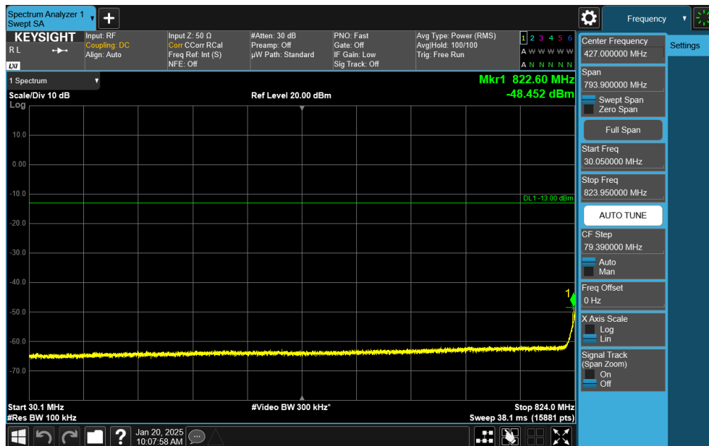
Plot 7-37. Conducted Spurious Plot (NR Band n26/n5 - 20.0MHz DFT-s-OFDM QPSK - RB Size 1, RB Offset 50 - Mid Channel)
