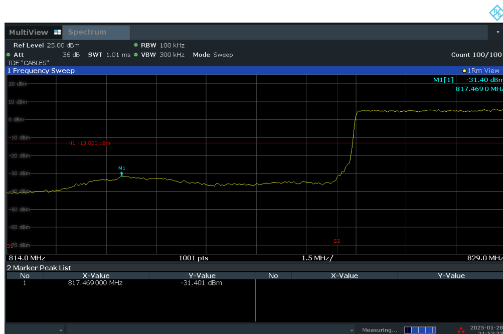
Plot 7-59. Lower BE Plot (LTE Band 5 - 10MHz QPSK – Full RB Configuration)
