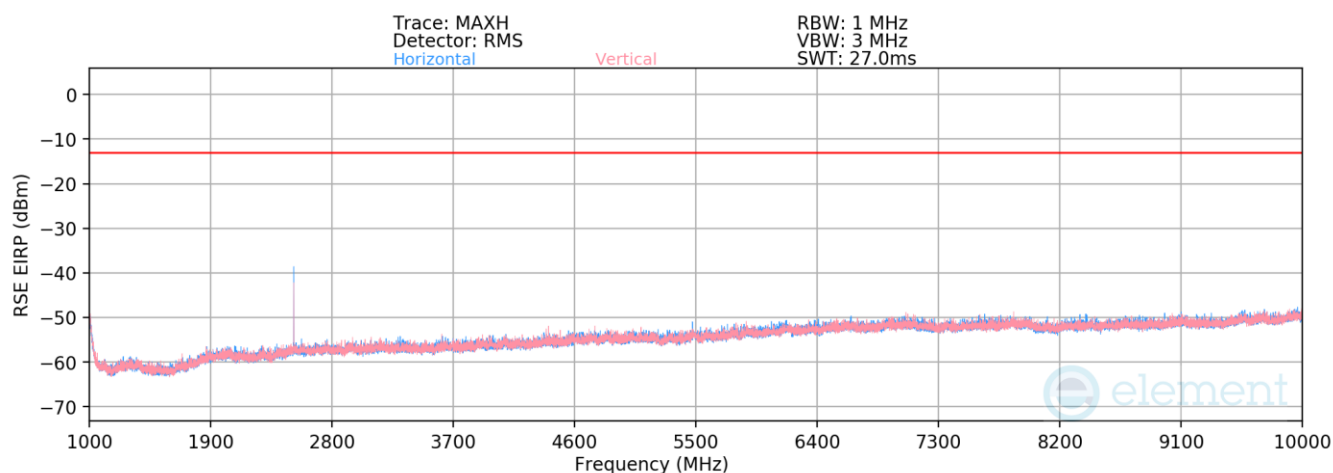
Plot 7-80. Antenna BCM Radiated Spurious Plot above 1GHz (NR Band n26/n5)
