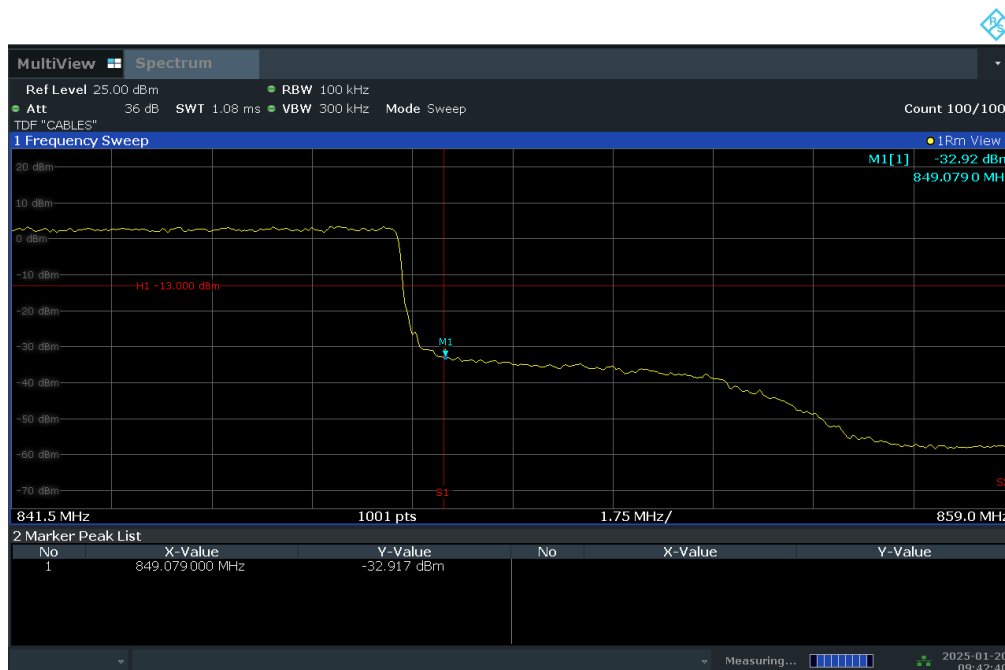
Plot 7-52. Upper BE Plot (LTE Band 26 - 15MHz QPSK – Full RB Configuration)
