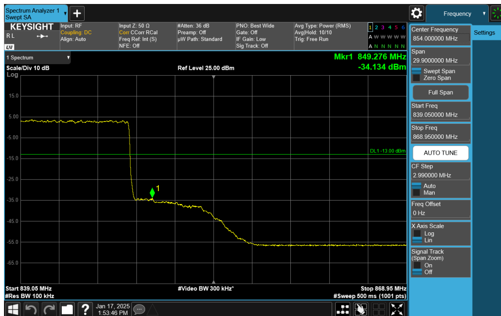
Plot 7-76. Upper BE Plot (NR Band n5 DFT-s-OFDM \pi/2 BPSK – 20.0MHz - Full RB)
