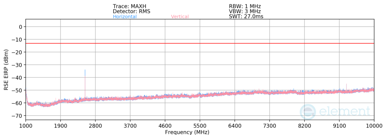
Plot 7-78. Antenna BCM Radiated Spurious Plot above 1GHz (LTE Band 26/5)
