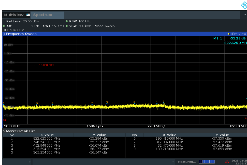
Plot 7-28. Conducted Spurious Plot (LTE Band 26/5 - 10MHz QPSK - RB Size 1, RB Offset 25 - Mid Channel)
