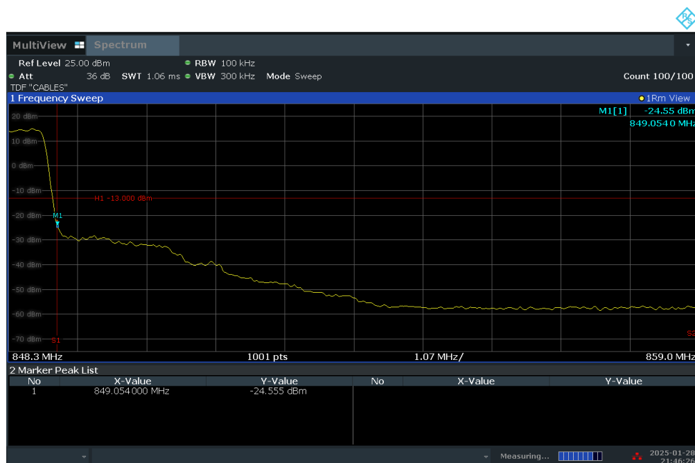
Plot 7-54. Upper BE Plot (LTE Band 5 – 1.4MHz QPSK – Full RB Configuration)
