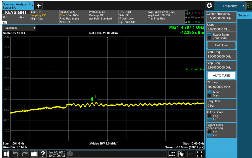
Plot 7-36. Conducted Spurious Plot (NR Band n26/n5 - 20.0MHz DFT-s-OFDM QPSK - RB Size 1, RB Offset 50 - Low Channel)
