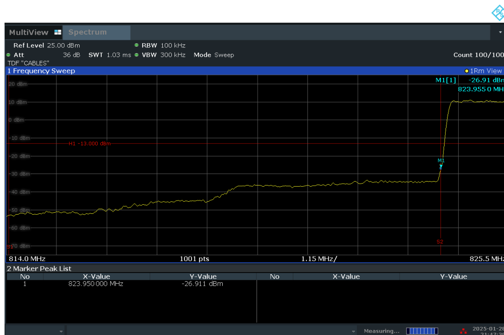
Plot 7-55. Lower BE Plot (LTE Band 5 - 3MHz QPSK – Full RB Configuration)
