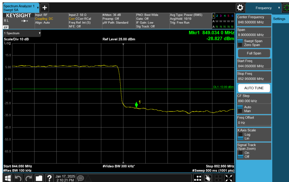
Plot 7-64. Upper BE Plot (NR Band n26 DFT-s-OFDM \pi/2 BPSK – 10.0MHz - Full RB)
