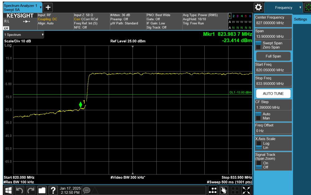
Plot 7-67. Lower BE Plot (NR Band n26 DFT-s-OFDM \pi/2 BPSK – 20.0MHz - Full RB)
