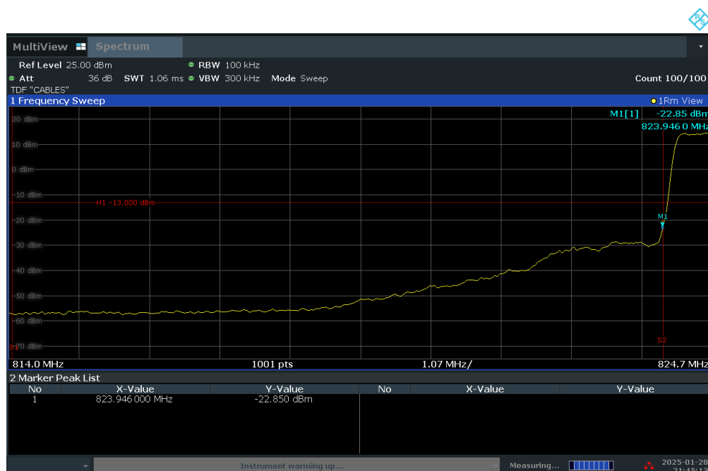
Plot 7-53. Lower BE Plot (LTE Band 5 – 1.4MHz QPSK – Full RB Configuration)
