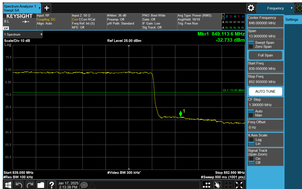
Plot 7-68. Upper BE Plot (NR Band n26 DFT-s-OFDM \pi/2 BPSK – 20.0MHz - Full RB)
