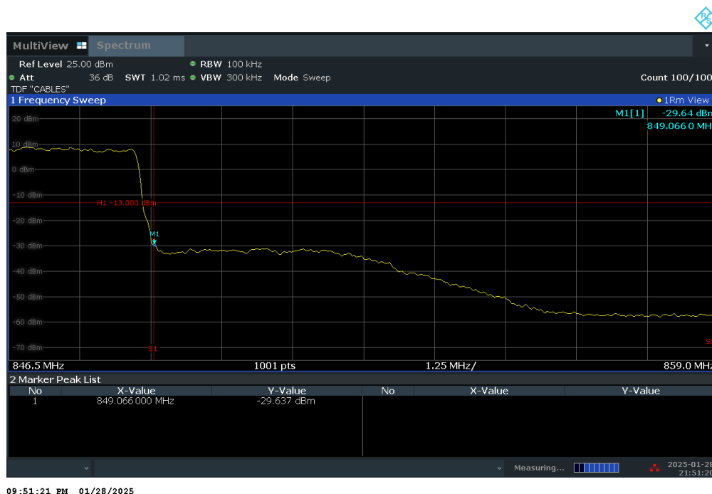
Plot 7-58. Upper BE Plot (LTE Band 5 - 5MHz QPSK – Full RB Configuration)
