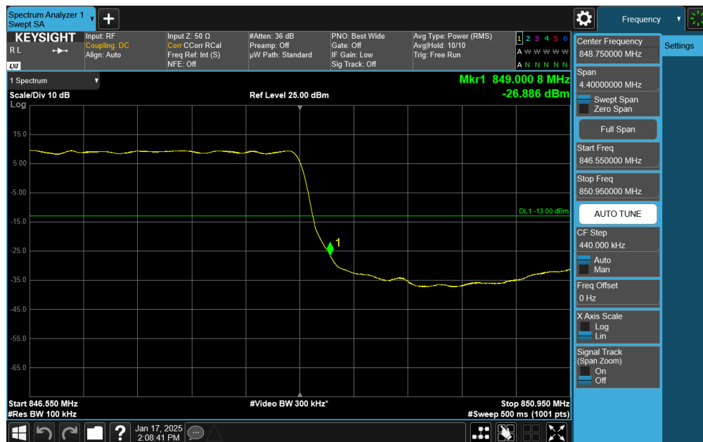
Plot 7-62. Upper BE Plot (NR Band n26 CP-OFDM \pi/2 BPSK – 5.0MHz - Full RB)
