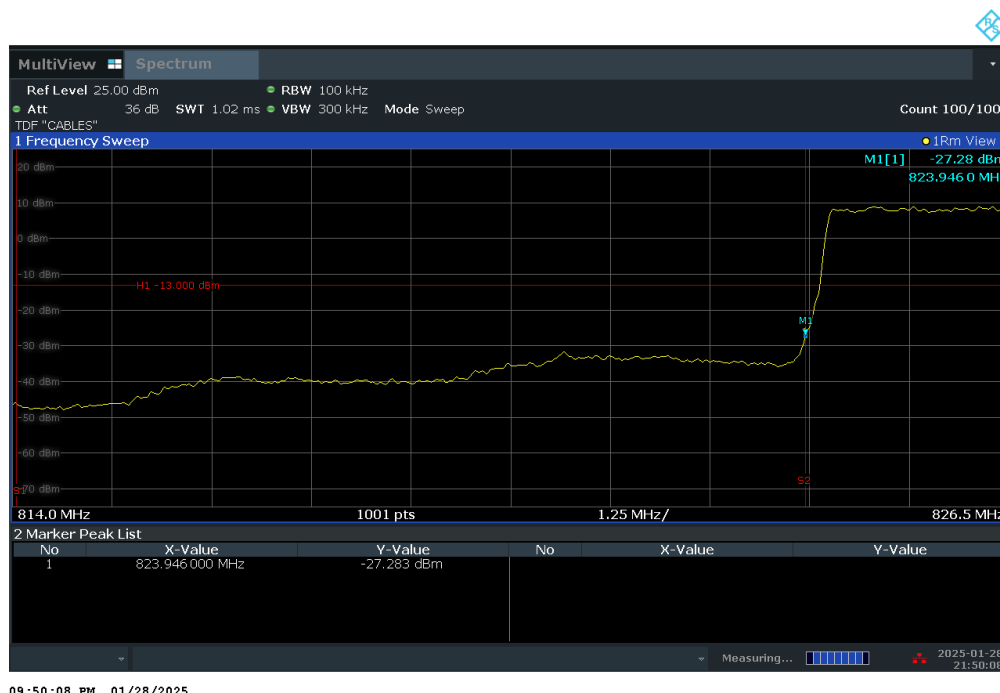
Plot 7-57. Lower BE Plot (LTE Band 5 - 5MHz QPSK – Full RB Configuration)
