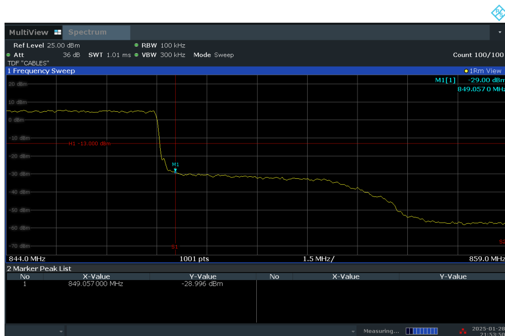
Plot 7-60. Upper BE Plot (LTE Band 5 - 10MHz QPSK – Full RB Configuration)
