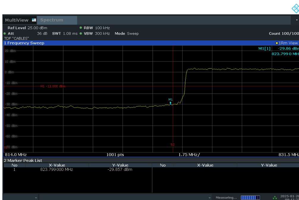
Plot 7-51. Lower BE Plot (LTE Band 26 - 15MHz QPSK – Full RB Configuration)
