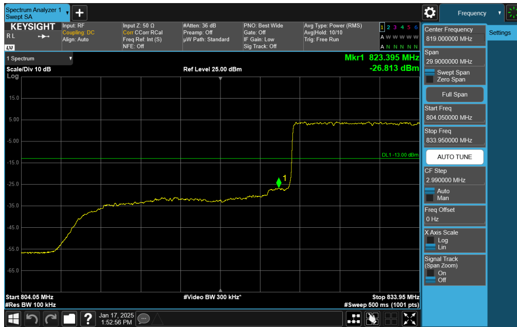
Plot 7-75. Lower BE Plot (NR Band n5 DFT-s-OFDM \pi/2 BPSK – 20.0MHz - Full RB)
