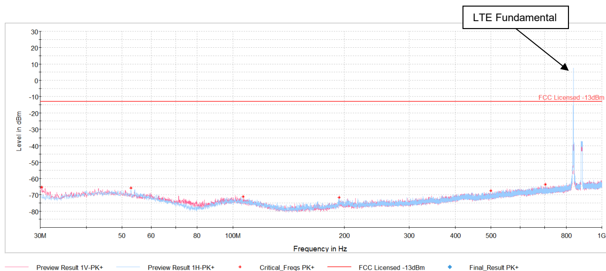
Plot 7-77. Antenna BCM Radiated Spurious Plot below 1GHz (LTE Band 26/5)
