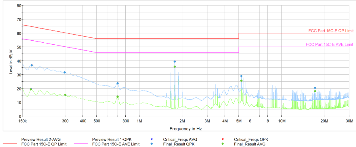
Plot 7-60. AC Line Conducted Plot with 802.11n Ch.157 (N), with AC/DC adapter & magnetic charger
