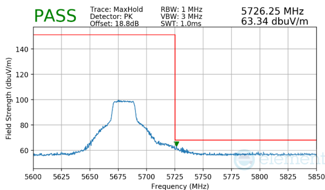
Plot 7-50. (Pk & Avg, Ch.136, 802.11n, MCS7)
