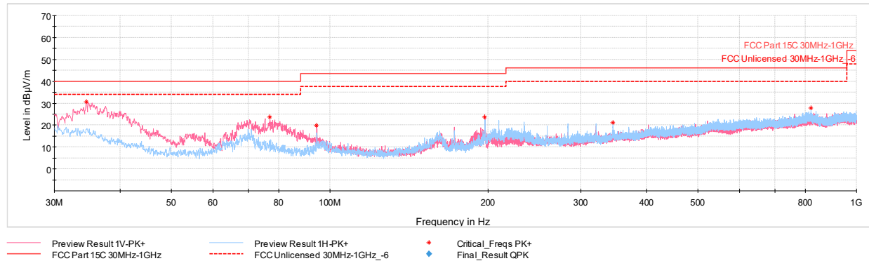
Plot 7-58. Radiated Spurious Emissions Below 1GHz – Simultaneous Transmission
