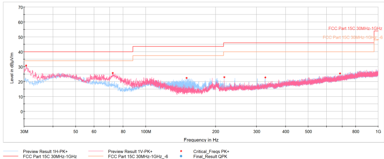
Plot 7-57. Radiated Spurious Emissions below 1GHz, 802.11n, Ch. 157 with AC/DC Adapter & magnetic charger
