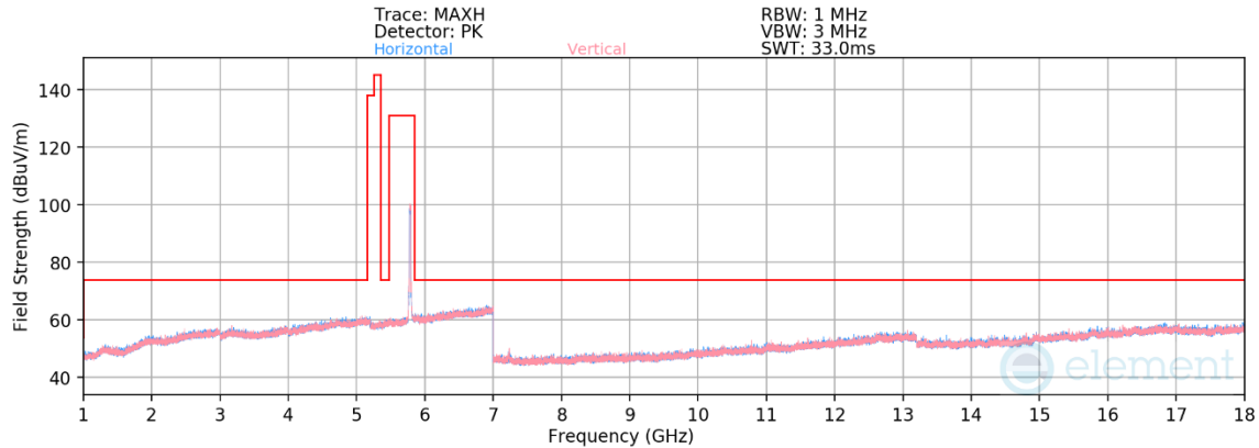
Plot 7-38. Radiated Spurious Emissions above 1GHz(802.11n – Ch. 157)
