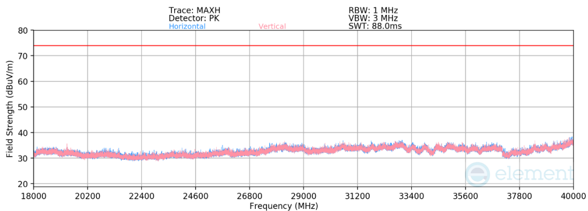
Plot 7-39. Radiated Emissions 18GHz-40GHz (802.11n – Ch. 157)
