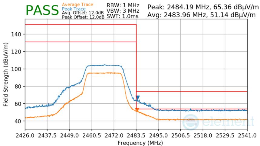
Plot 7-74. Radiated Restricted Upper Band Edge Measurement
