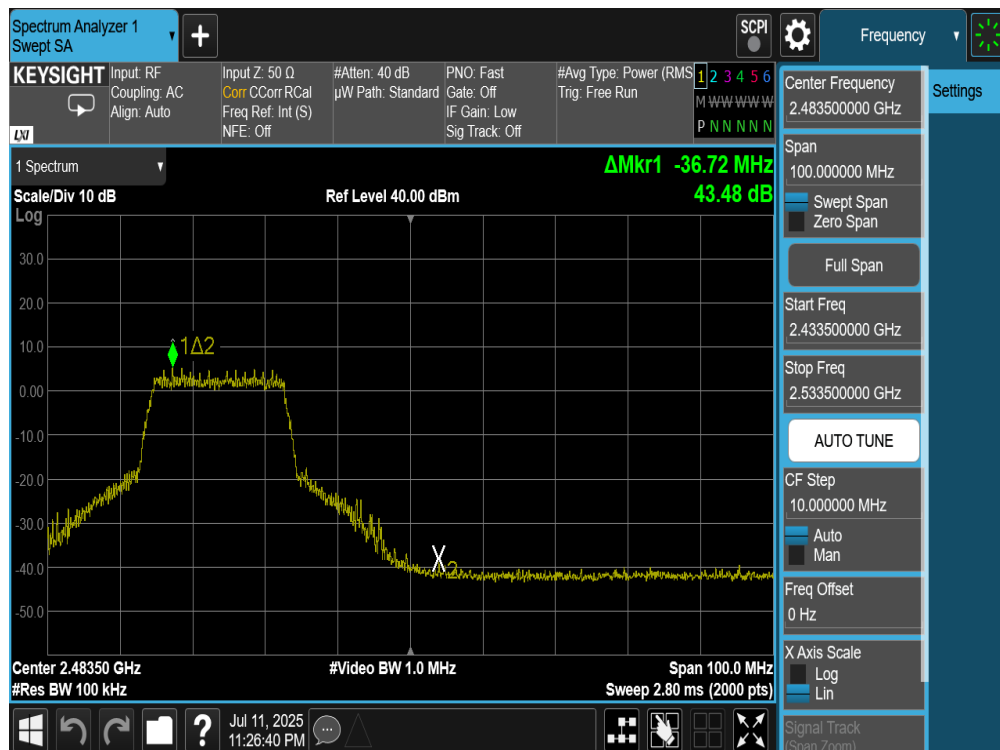
Plot 7-49. Band Edge Plot (802.11n (2.4GHz) – Ch. 10) – MCS7
