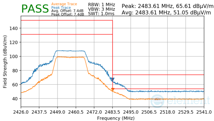
Plot 7-78. Radiated Restricted Upper Band Edge Measurement
