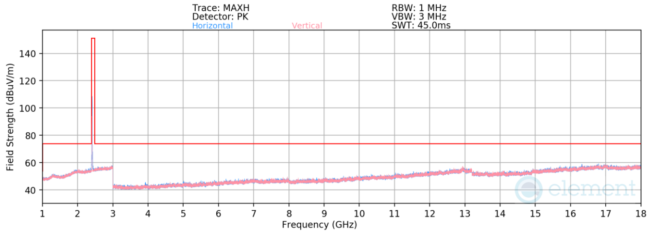
Plot 7-59. Radiated Spurious Emissions above 1GHz (802.11b – Ch. 1)
