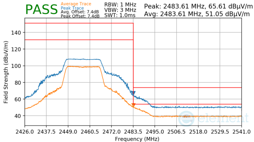
Plot 7-72. Radiated Restricted Upper Band Edge Measurement
