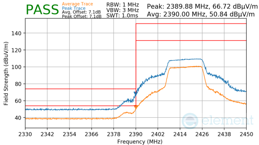
Plot 7-68. Radiated Restricted Lower Band Edge Measurement
