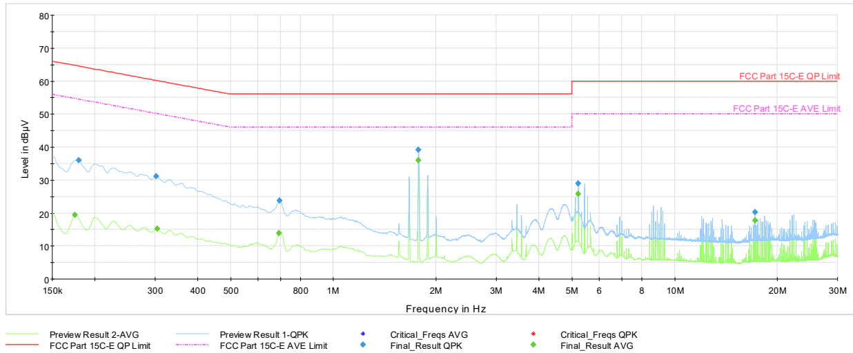
Plot 7-83. AC Line Conducted Plot 802.11b - Ch.6 (L1, with AC/DC adaptor via USB-C cable with magnetic charger)
