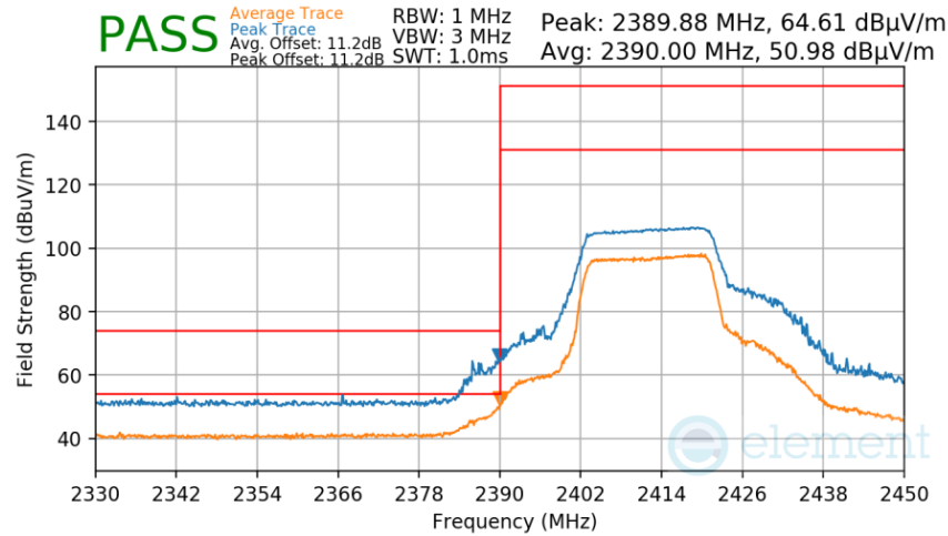
Plot 7-76. Radiated Restricted Lower Band Edge Measurement
