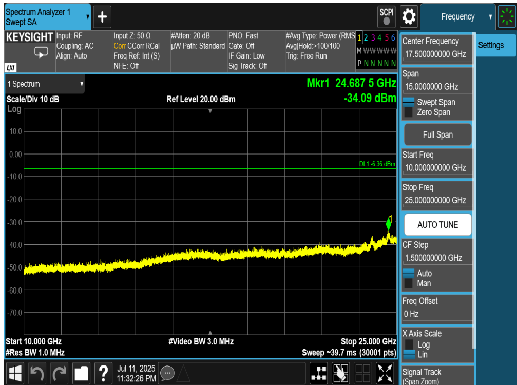
Plot 7-58. Conducted Spurious Plot (802.11b – Ch. 11)
