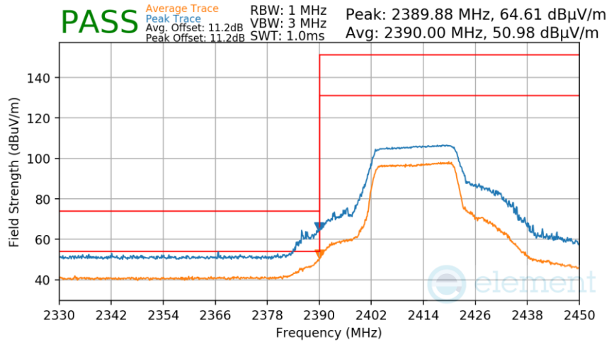
Plot 7-67. Radiated Restricted Lower Band Edge Measurement
