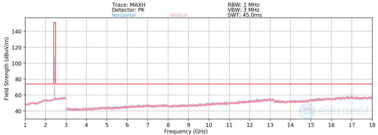
Plot 7-60. Radiated Spurious Emissions above 1GHz (802.11b – Ch. 6)
