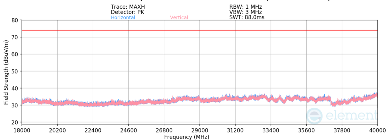
Plot 7-61. Radiated Spurious Emissions Above 18GHz (802.11b – Ch. 6)
