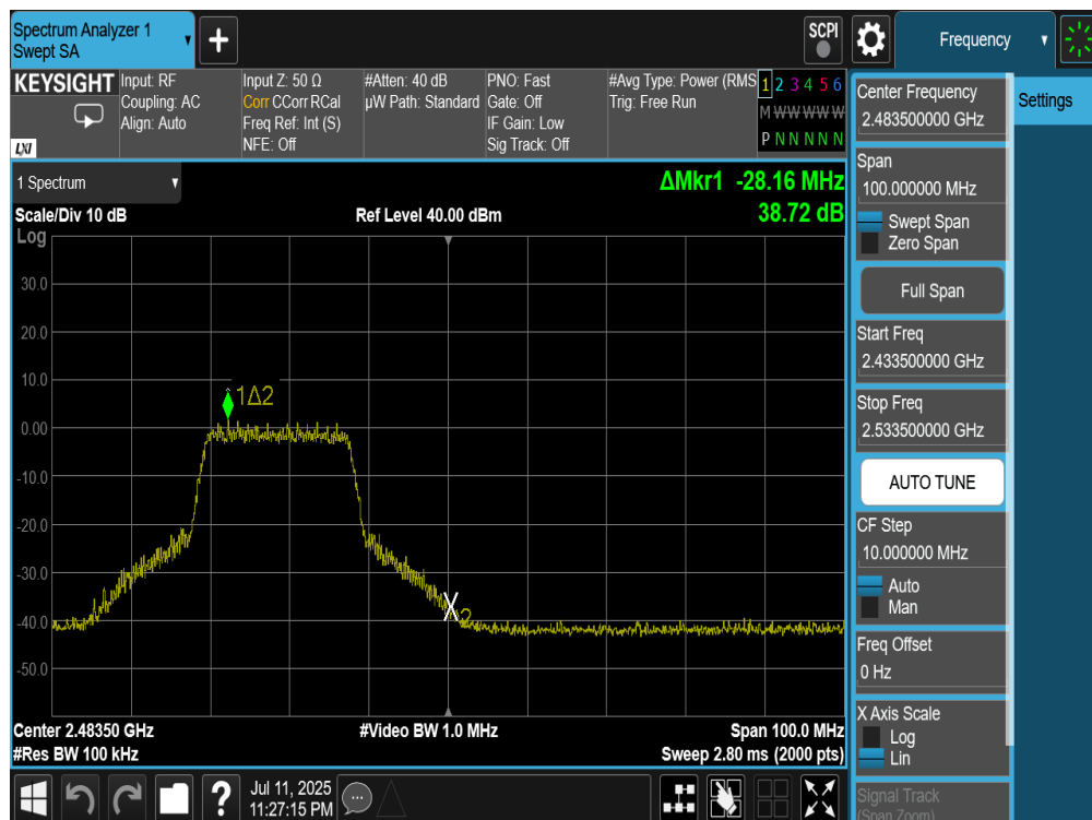
Plot 7-50. Band Edge Plot (802.11n (2.4GHz) – Ch. 11) – MCS7
