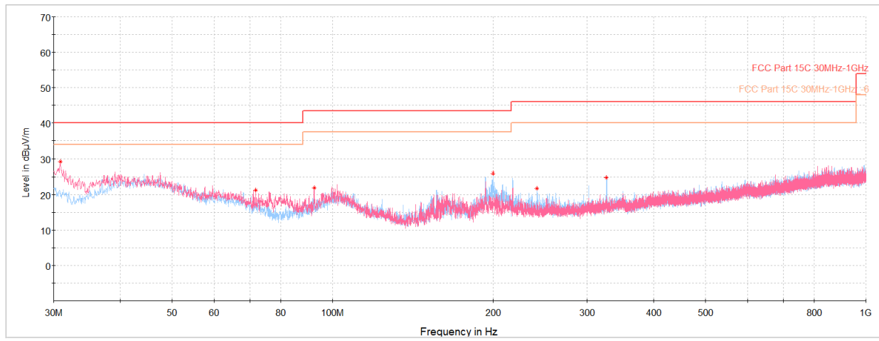
Plot 7-82. Radiated Spurious Emissions below 1GHz 11b Ch.6, with AC/DC Adapter via USB-C cable with magnetic charger
