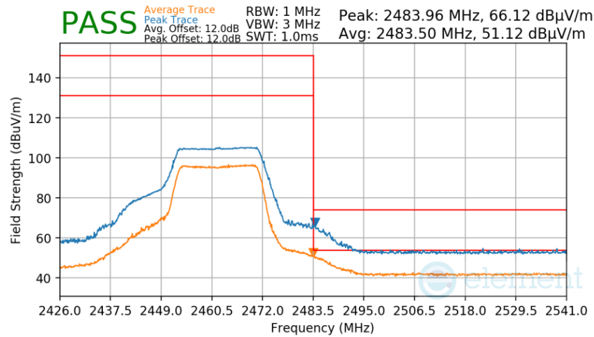
Plot 7-73. Radiated Restricted Upper Band Edge Measurement
