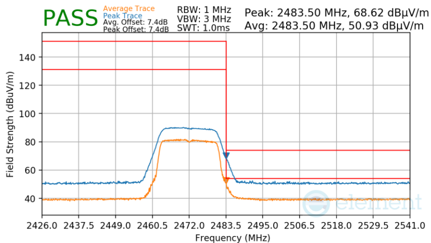
Plot 7-75. Radiated Restricted Upper Band Edge Measurement
