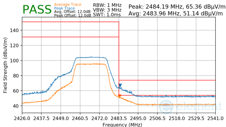
Plot 7-80. Radiated Restricted Upper Band Edge Measurement
