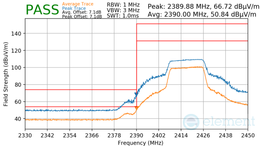
Plot 7-77. Radiated Restricted Lower Band Edge Measurement
