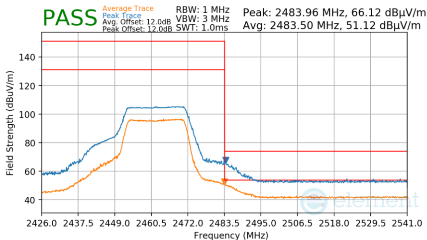
Plot 7-79. Radiated Restricted Upper Band Edge Measurement
