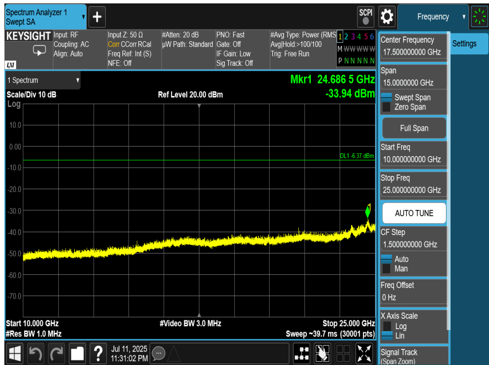
Plot 7-56. Conducted Spurious Plot (802.11b – Ch. 6)
