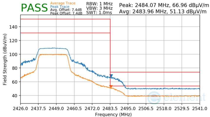
Plot 7-70. Radiated Restricted Upper Band Edge Measurement
