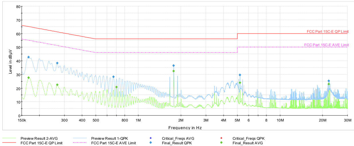
Plot 7-84. AC Line Conducted Plot 802.11b - Ch.6 (N, with AC/DC adaptor via USB-C cable with magnetic charger)
