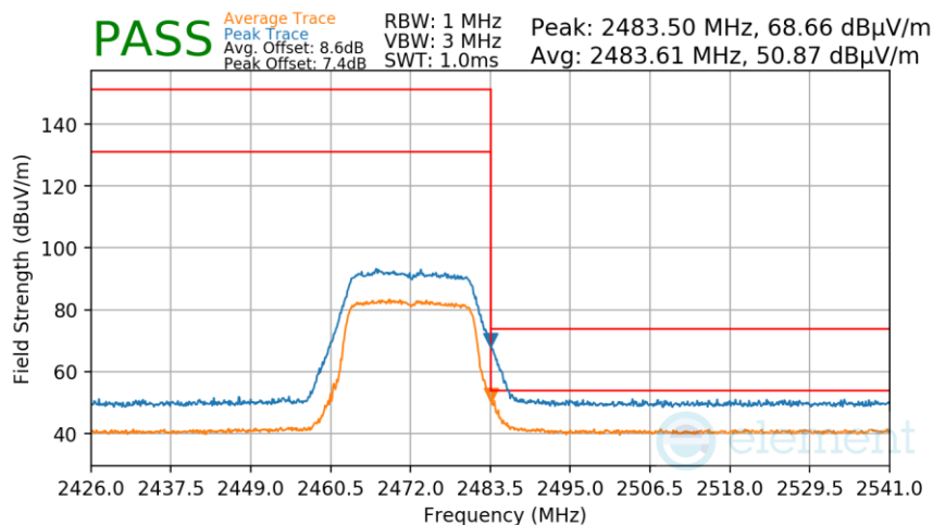
Plot 7-81. Radiated Restricted Upper Band Edge Measurement
