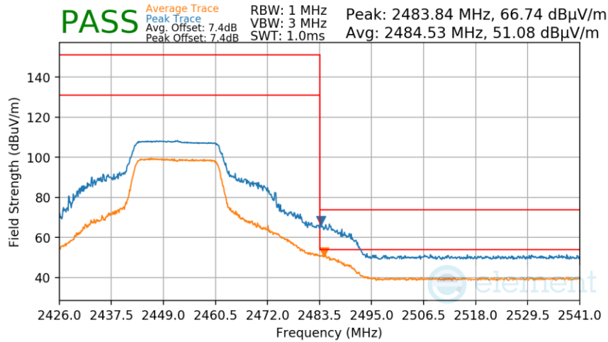
Plot 7-71. Radiated Restricted Upper Band Edge Measurement
