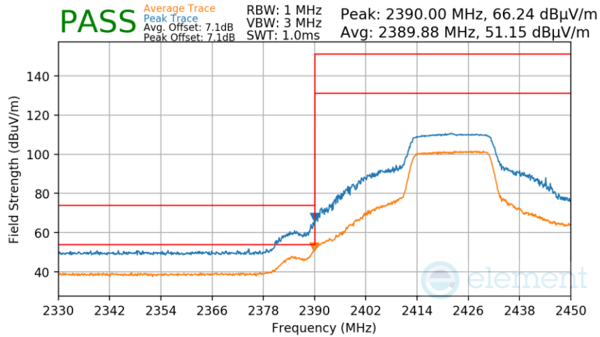
Plot 7-69. Radiated Restricted Lower Band Edge Measurement
