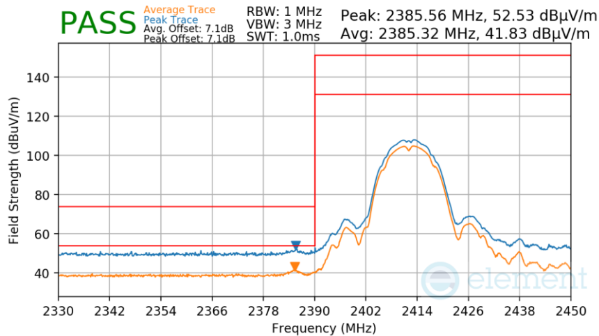
Plot 7-63. Radiated Restricted Lower Band Edge Measurement
