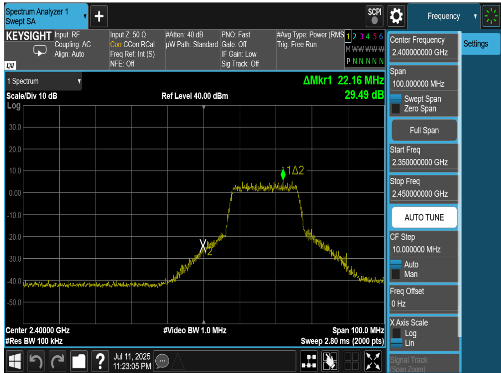
Plot 7-48. Band Edge Plot (802.11n (2.4GHz) – Ch. 2) – MCS7
