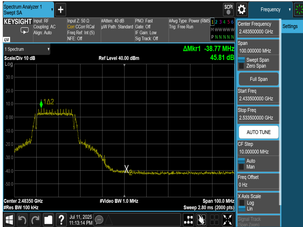
Plot 7-33. Band Edge Plot (802.11g – Ch. 9) – 6Mbps
