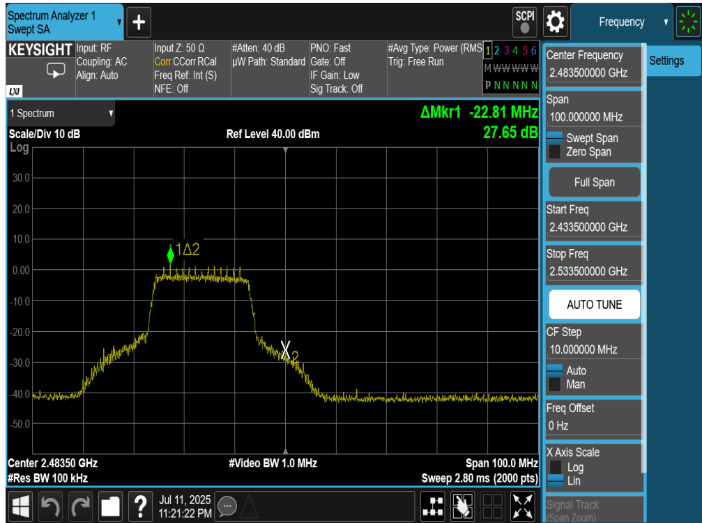
Plot 7-45. Band Edge Plot (802.11n (2.4GHz) – Ch. 12) – MCS0
