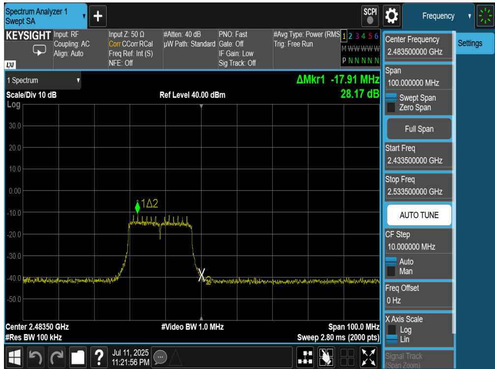
Plot 7-46. Band Edge Plot (802.11n (2.4GHz) – Ch. 13) – MCS0
