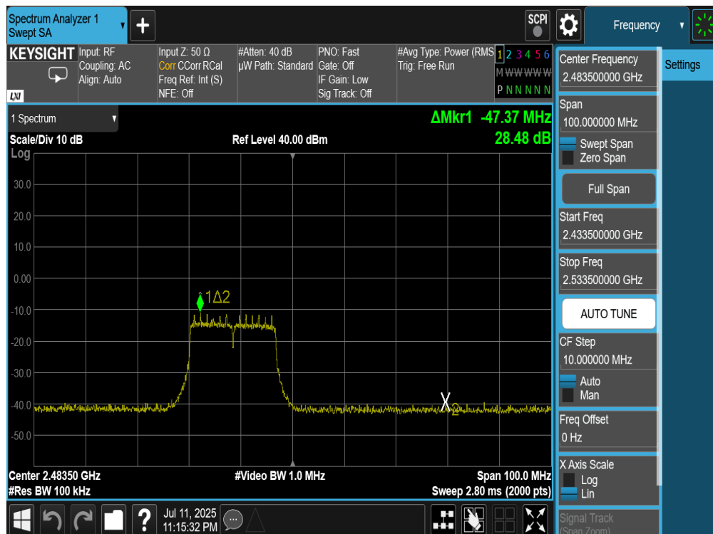
Plot 7-37. Band Edge Plot (802.11g – Ch. 13) – 6Mbps
