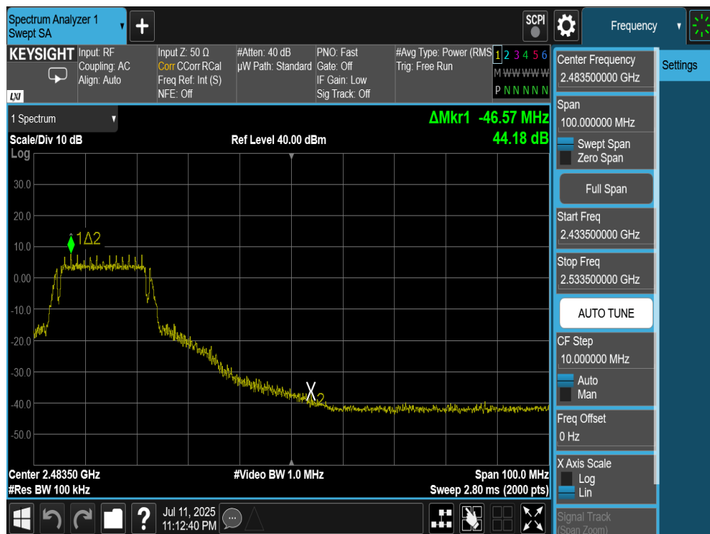
Plot 7-32. Band Edge Plot (802.11g – Ch. 8) – 6Mbps
