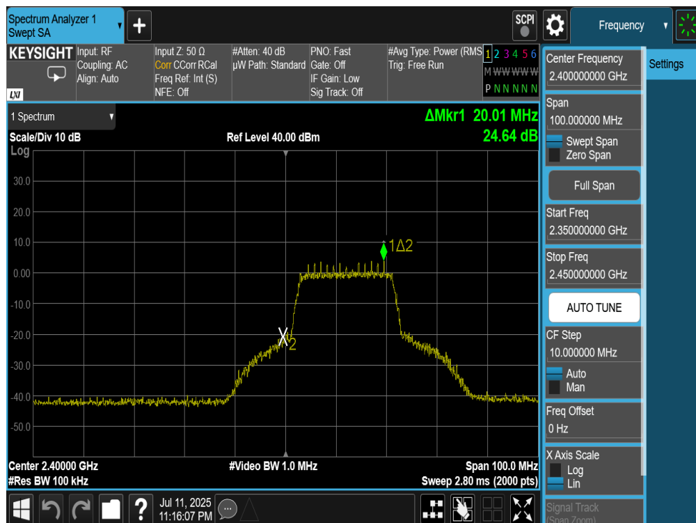
Plot 7-38. Band Edge Plot (802.11n (2.4GHz) – Ch. 1) – MCS0
