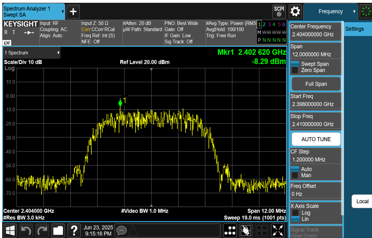
Plot 7-16. Power Spectral Density Plot (Bluetooth (HDR8), 8Mbps, iPA – Ch. 1)
