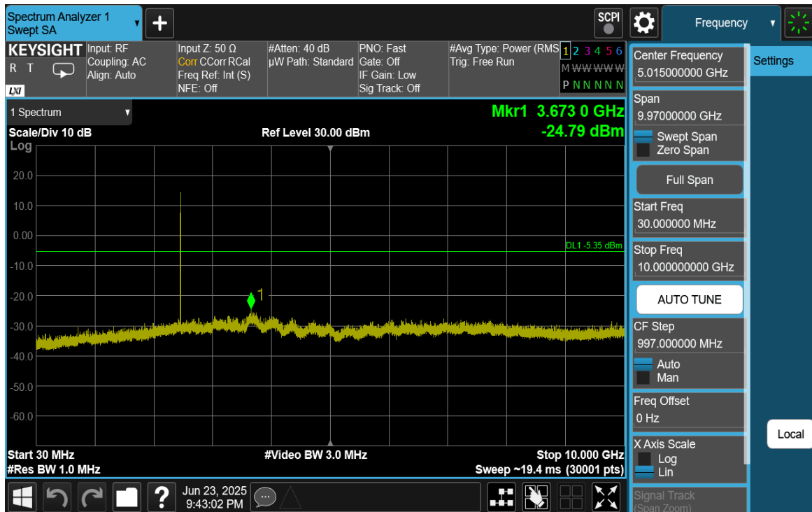
Plot 7-27. Conducted Spurious Plot (Bluetooth (HDR4), 4 Mbps, ePA – Ch. 73)
