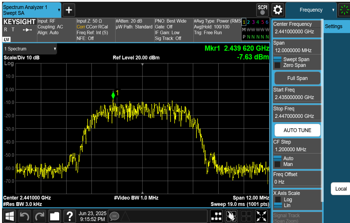
Plot 7-17. Power Spectral Density Plot (Bluetooth (HDR8), 8Mbps, iPA – Ch. 38)
