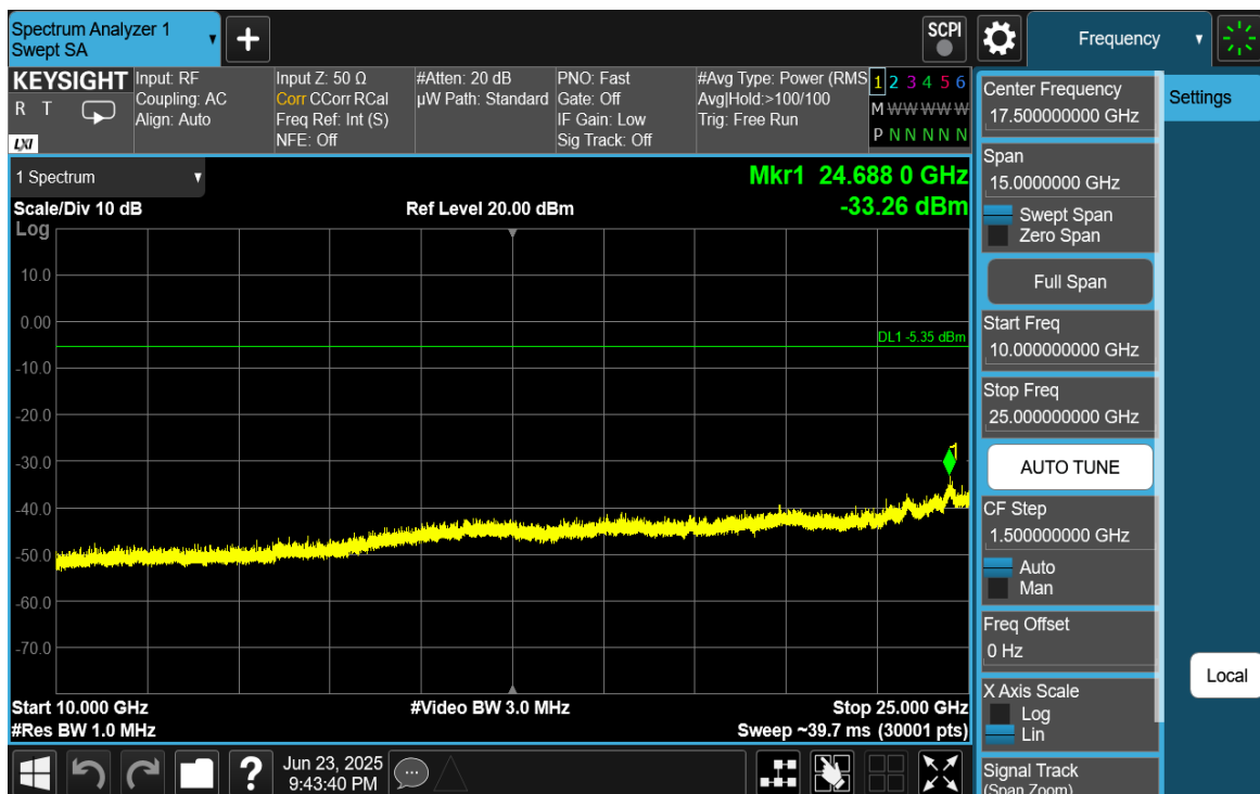
Plot 7-28. Conducted Spurious Plot (Bluetooth (HDR4), 4 Mbps, ePA – Ch. 73)
