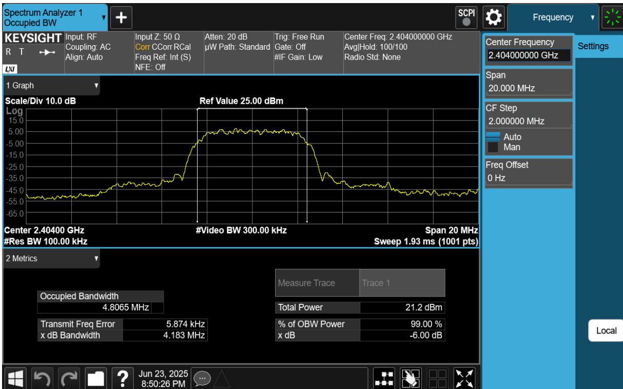
Plot 7-4. 6dB BW & 99% OBW Plot (Bluetooth (HDR8), 8Mbps, ePA – Ch. 1)
