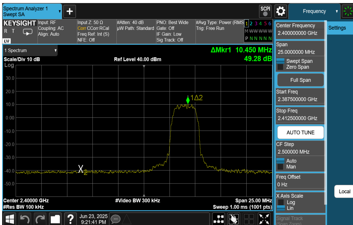
Plot 7-19. Band Edge Plot (Bluetooth (HDR4), ePA – Ch. 1)
