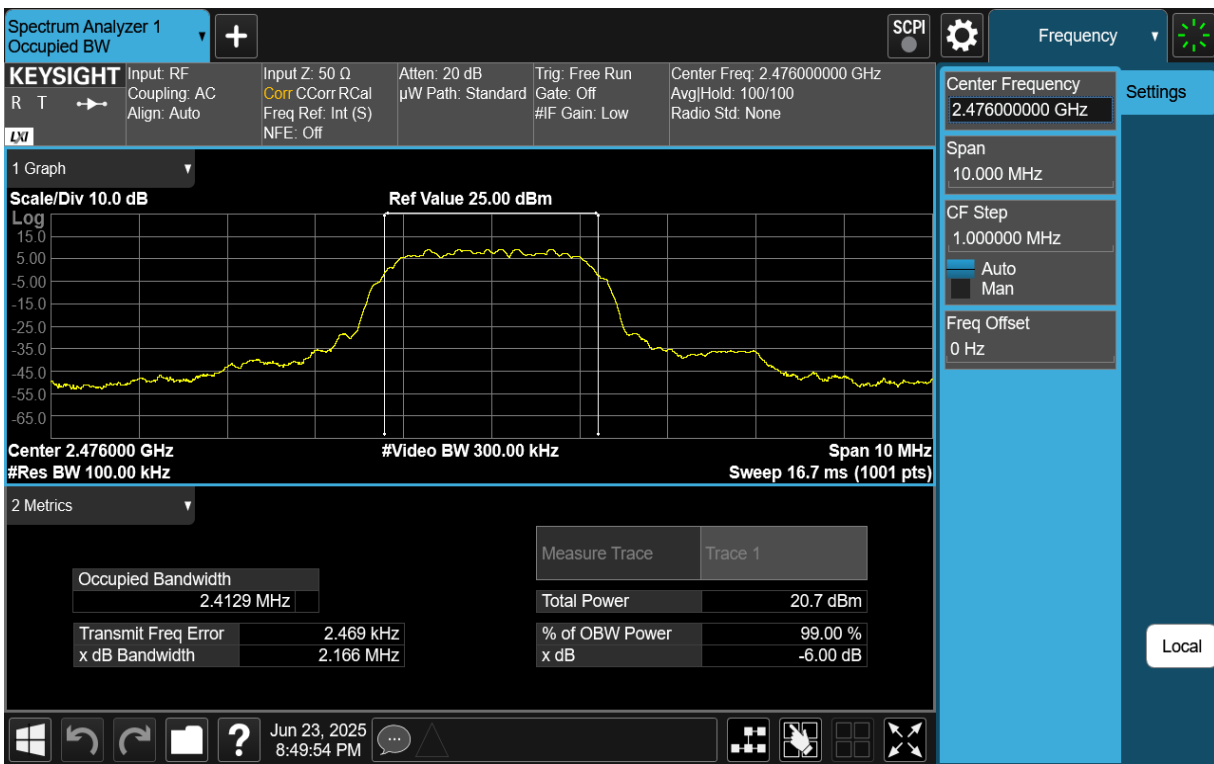
Plot 7-3. 6dB BW & 99% OBW Plot (Bluetooth (HDR4), 4Mbps, ePA – Ch. 73)
