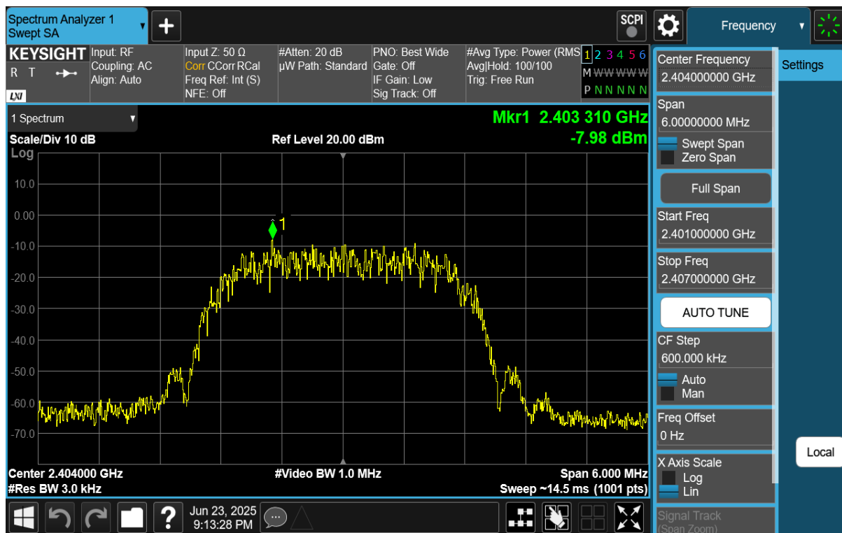
Plot 7-10. Power Spectral Density Plot (Bluetooth (HDR4), 4Mbps, iPA – Ch. 1)
