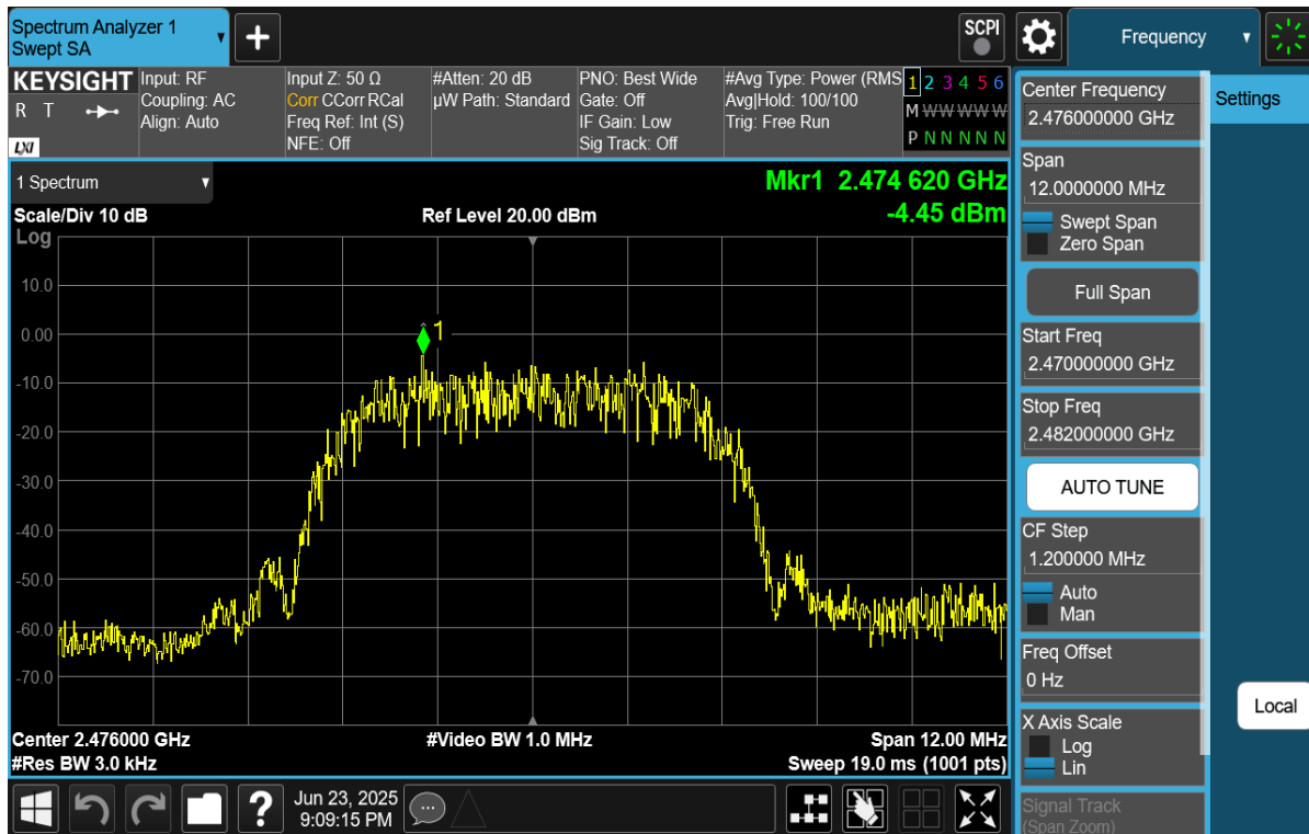
Plot 7-15. Power Spectral Density Plot (Bluetooth (HDR8), 8Mbps, ePA – Ch. 73)
