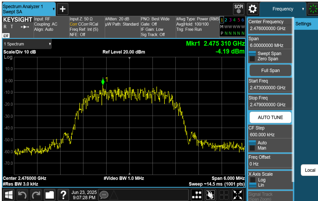
Plot 7-9. Power Spectral Density Plot (Bluetooth (HDR4), 4Mbps, ePA – Ch. 73)
