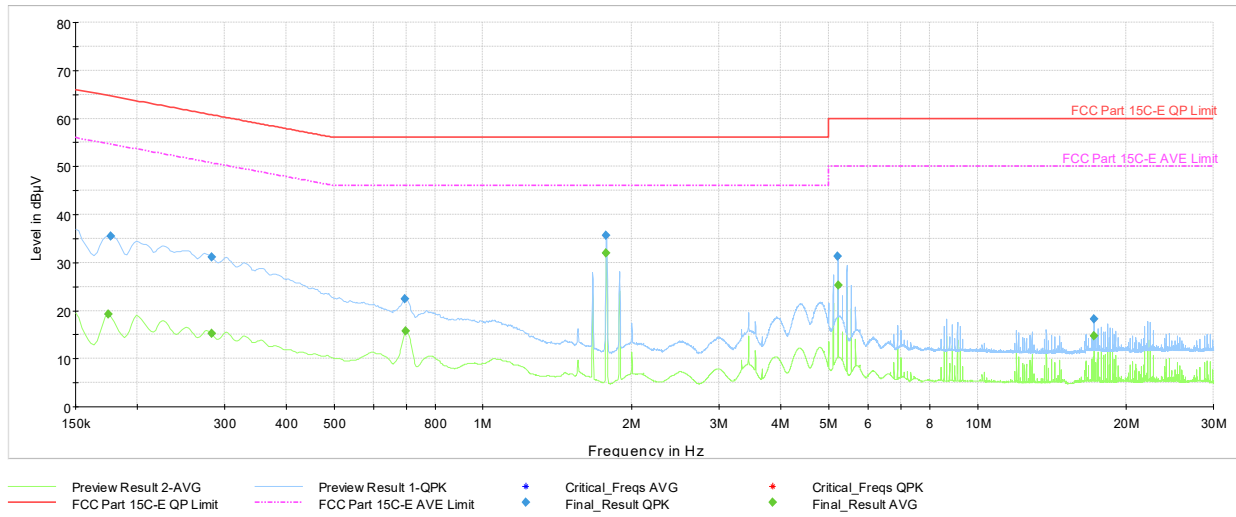
Plot 7-38. AC Line Conducted Plot with Bluetooth HDR (L1, 4Mbps ePA - Ch.38 with AC/DC adaptor via USB-C cable with magnetic charger)
