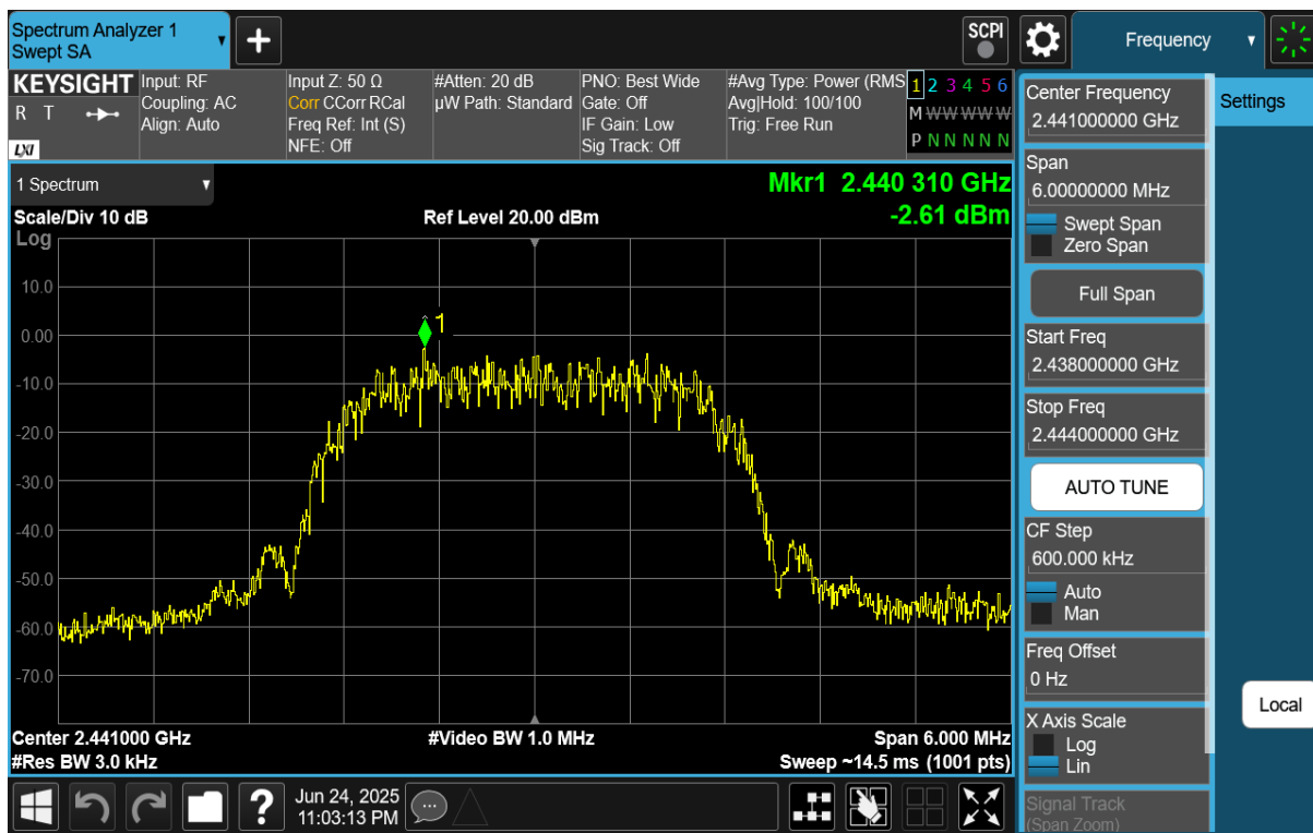
Plot 7-8. Power Spectral Density Plot (Bluetooth (HDR4), 4Mbps, ePA – Ch. 38)
