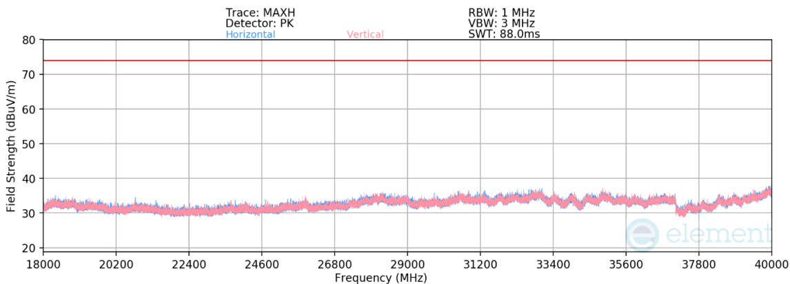
Plot 7-31. Radiated Spurious Emissions above 18GHz (4Mbps, HDR4, ePA – Ch. 38)
