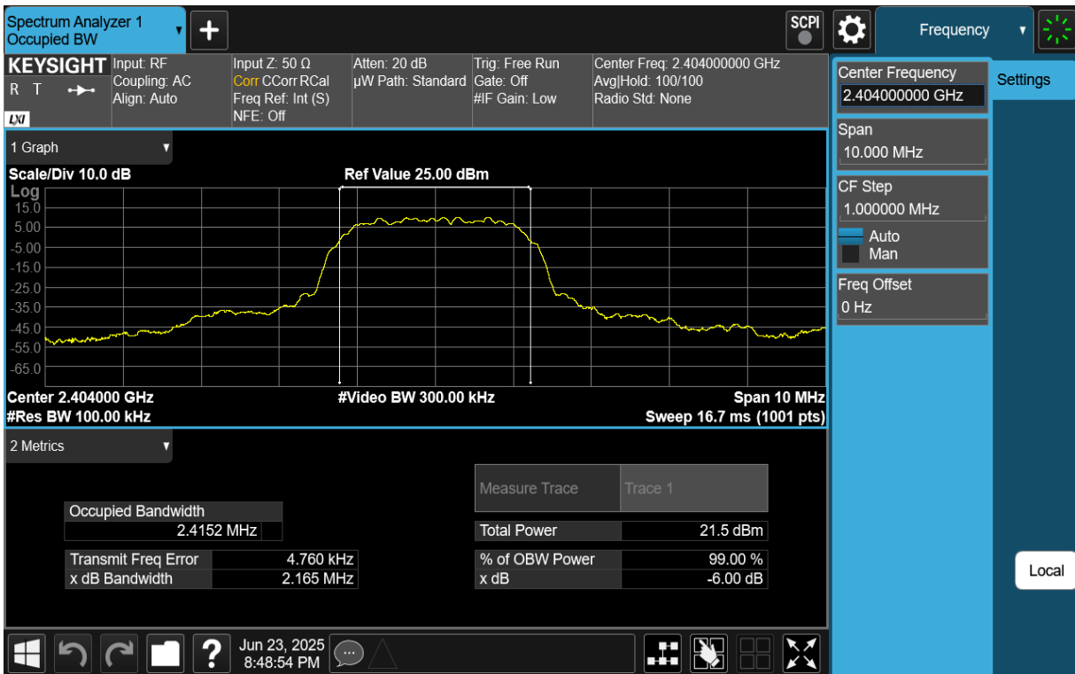
Plot 7-1. 6dB BW & 99% OBW Plot (Bluetooth (HDR4), 4Mbps, ePA – Ch. 1)
