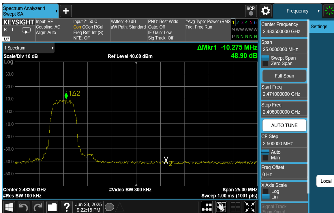
Plot 7-20. Band Edge Plot (Bluetooth (HDR4), ePA – Ch. 73)
