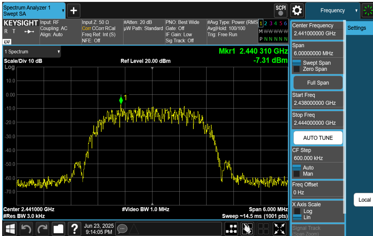
Plot 7-11. Power Spectral Density Plot (Bluetooth (HDR4), 4Mbps, iPA – Ch. 38)
