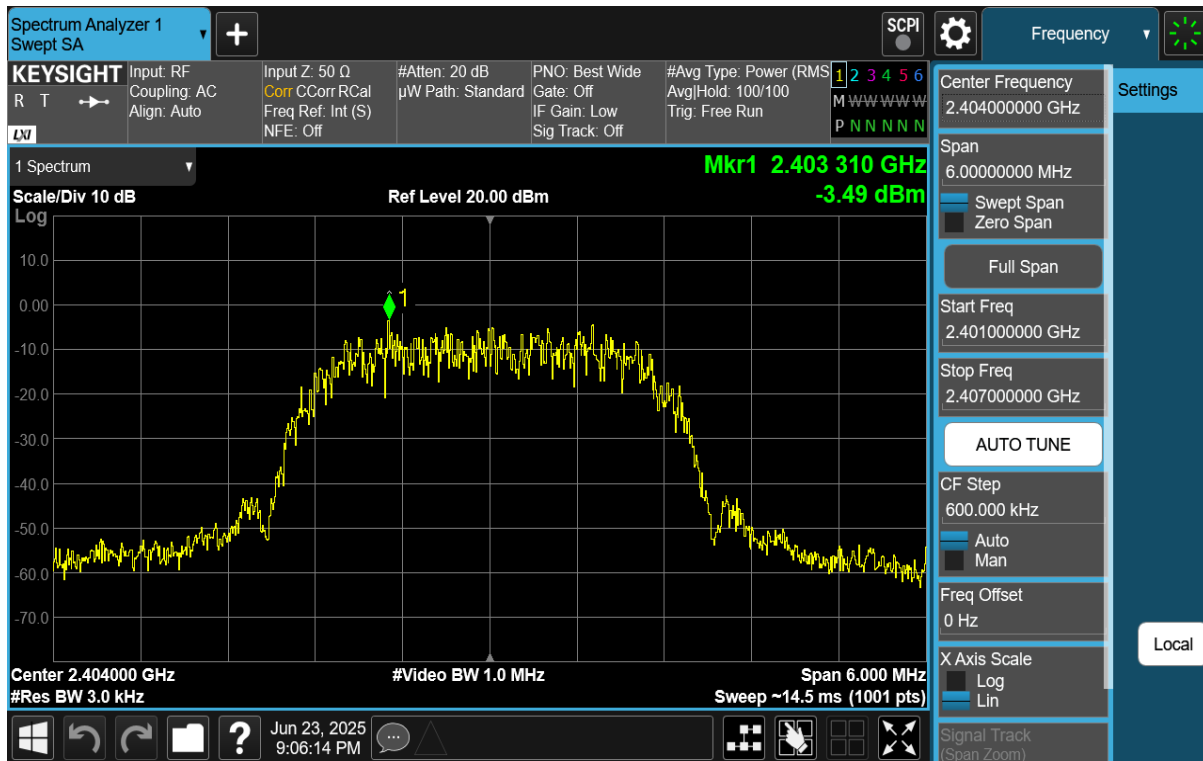
Plot 7-7. Power Spectral Density Plot (Bluetooth (HDR4), 4Mbps, ePA – Ch. 1)
