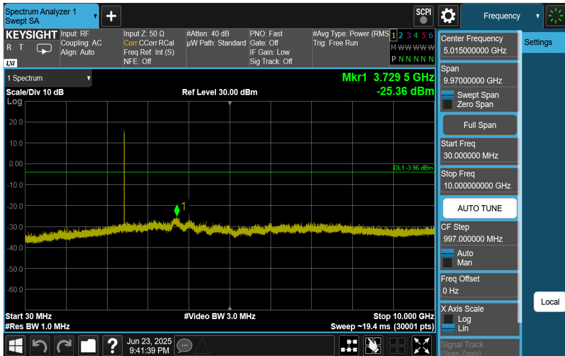
Plot 7-25. Conducted Spurious Plot (Bluetooth (HDR4), 4 Mbps, ePA – Ch. 38)
