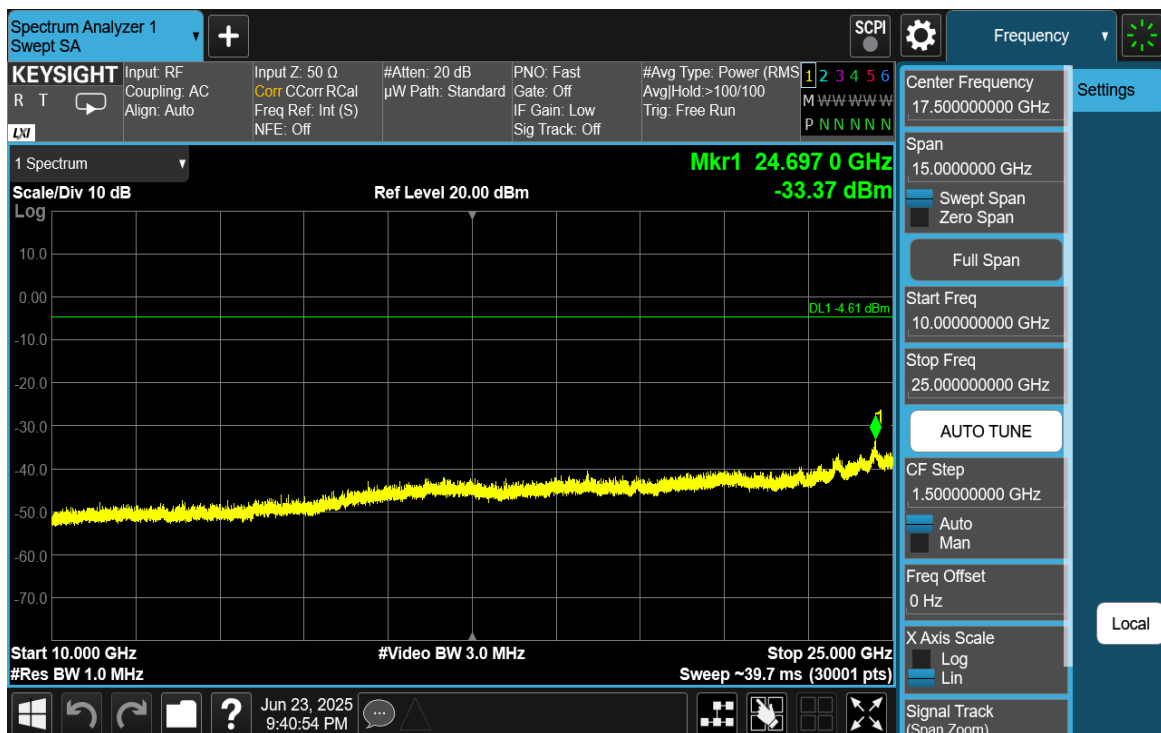
Plot 7-24. Conducted Spurious Plot (Bluetooth (HDR4), 4 Mbps, ePA – Ch. 1)
