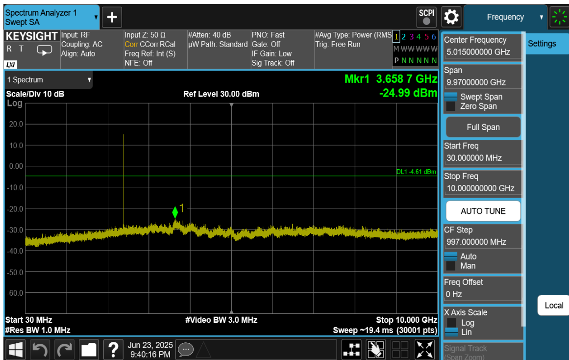
Plot 7-23. Conducted Spurious Plot (Bluetooth (HDR4), 4 Mbps, ePA – Ch. 1)
