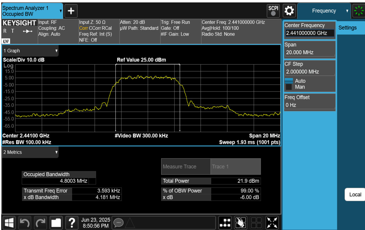
Plot 7-5. 6dB BW & 99% OBW Plot (Bluetooth (HDR8), 8Mbps, ePA – Ch. 38)
