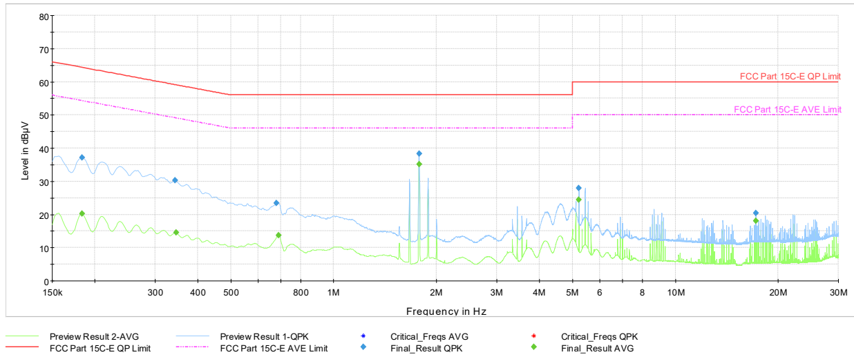
Plot 7-39. AC Line Conducted Plot with Bluetooth HDR (N, 4Mbps ePA - Ch.38 with AC/DC adaptor via USB-C cable with magnetic charger)
