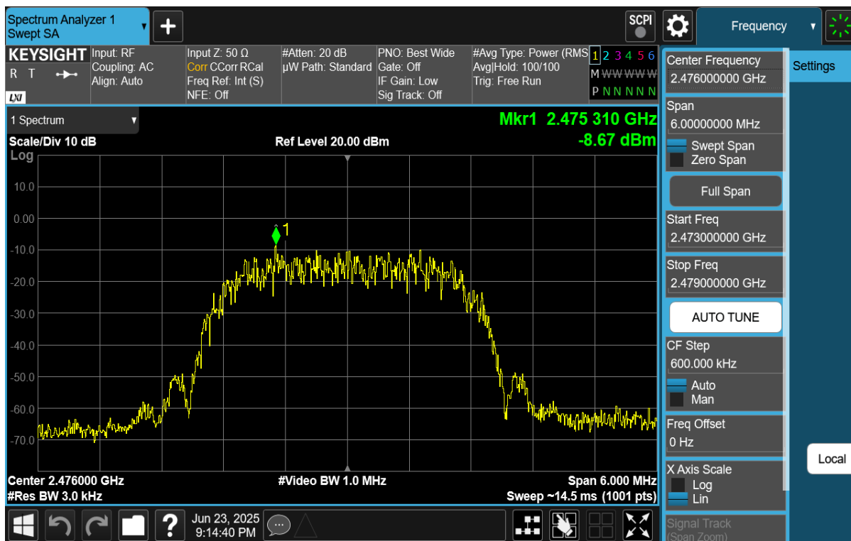
Plot 7-12. Power Spectral Density Plot (Bluetooth (HDR4), 4Mbps, iPA – Ch. 73)
