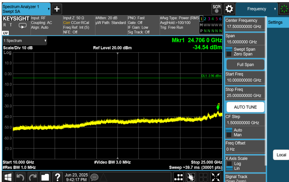
Plot 7-26. Conducted Spurious Plot (Bluetooth (HDR4), 4 Mbps, ePA – Ch. 38)
