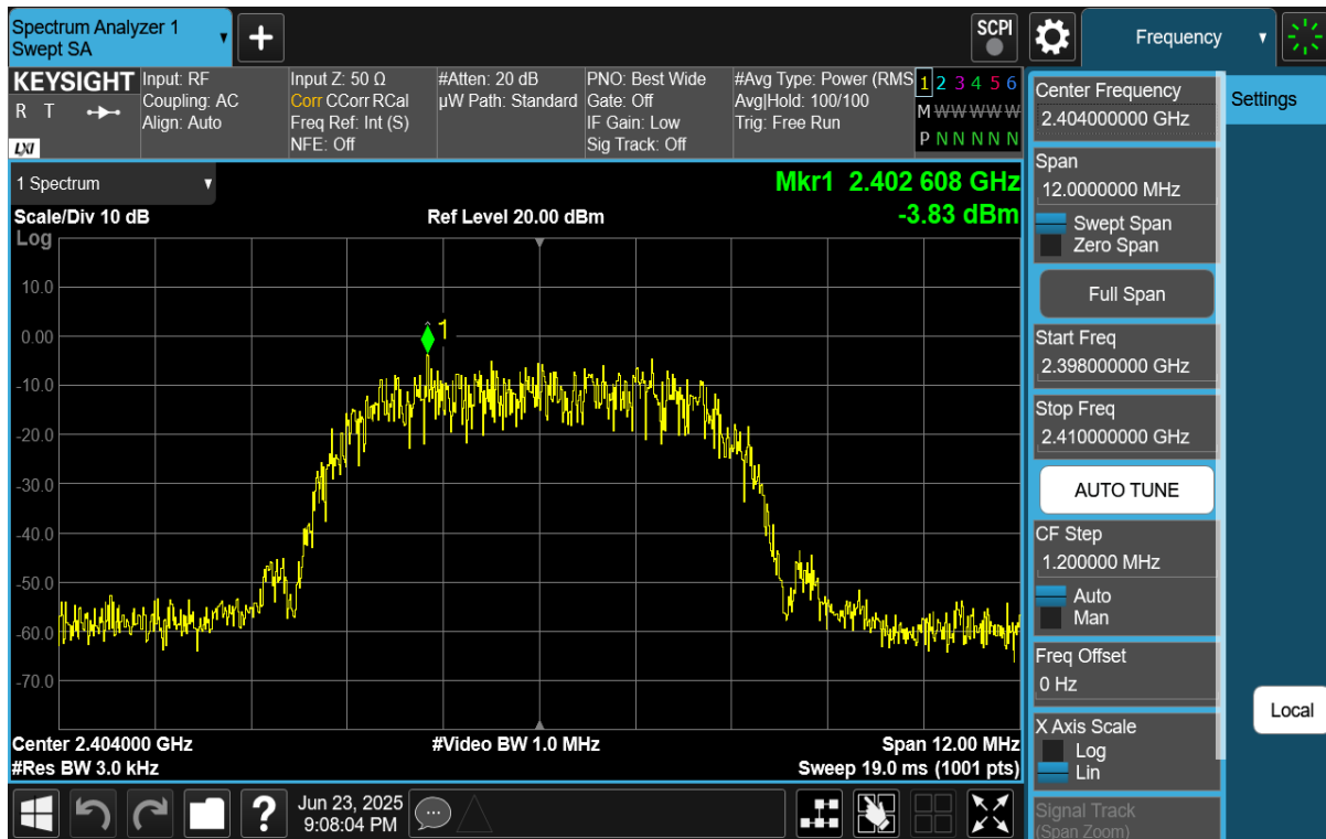
Plot 7-13. Power Spectral Density Plot (Bluetooth (HDR8), 8Mbps, ePA – Ch. 1)
