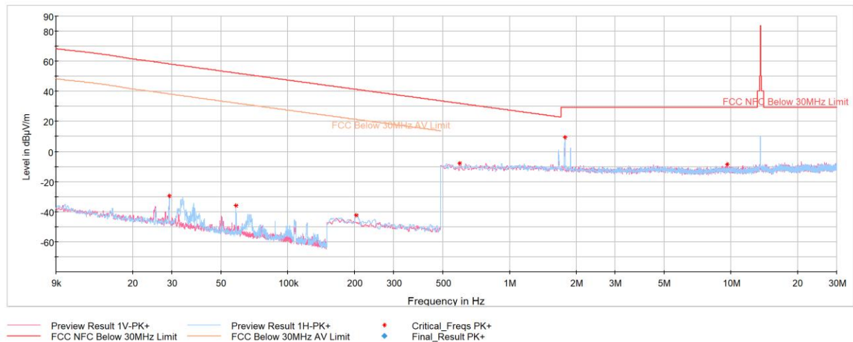
Plot 7-9. Radiated Spurious Emissions 9kHz – 30MHz (Reader 10% Ask 1 out of 4, with AC/DC Adapter and Magnetic Charger)
