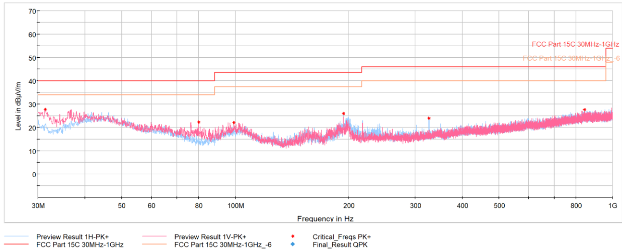
Plot 7-11. Radiated Spurious Emissions 30MHz – 1GHz (Reader 10% Ask 1 out of 4, with AC/DC Adapter and Magnetic Charger)
