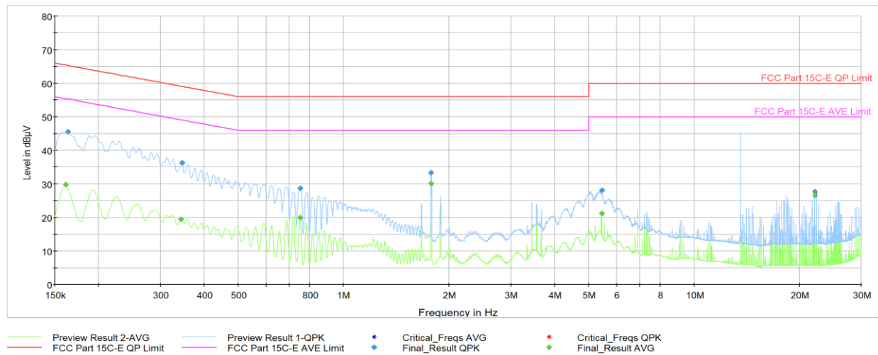
Plot 7-13. AC Line-Conducted Plot (N, CE F 212kbps, with AC/DC Adapter and Magnetic Charger)
