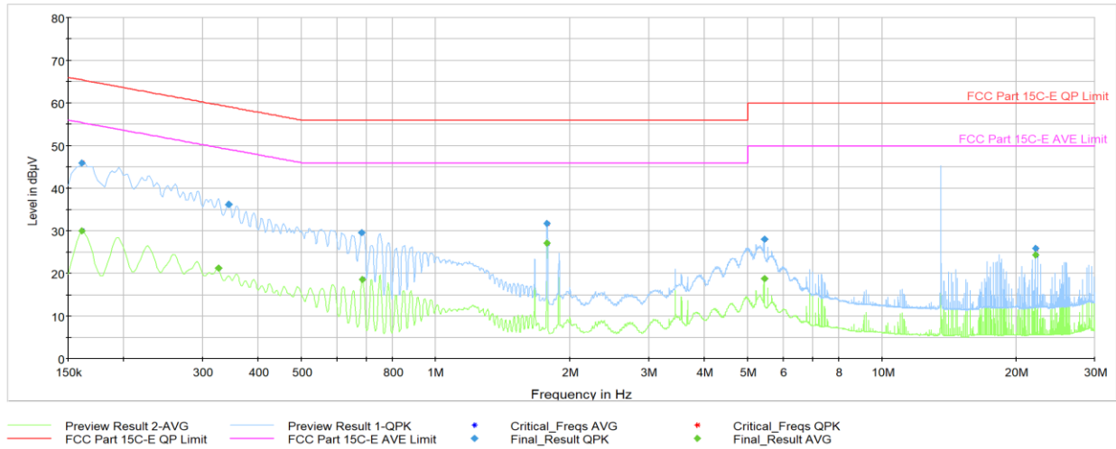
Plot 7-14. AC Line-Conducted Plot (L1, Reader 10% Ask 1 out of 4, with AC/DC Adapter and Magnetic Charger)
