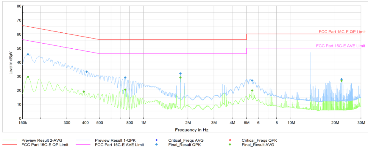
Plot 7-15. AC Line-Conducted Plot (N, Reader 10% Ask 1 out of 4, with AC/DC Adapter and Magnetic Charger)
