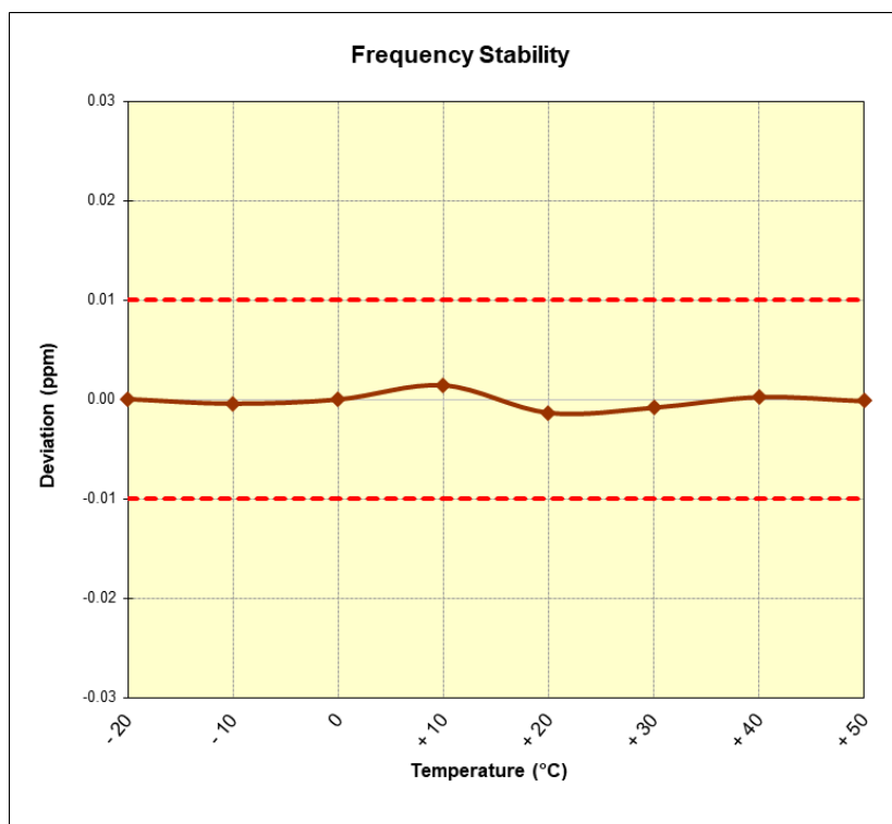
Figure 7-3. Frequency Stability Plot (CE F 212kbps)
