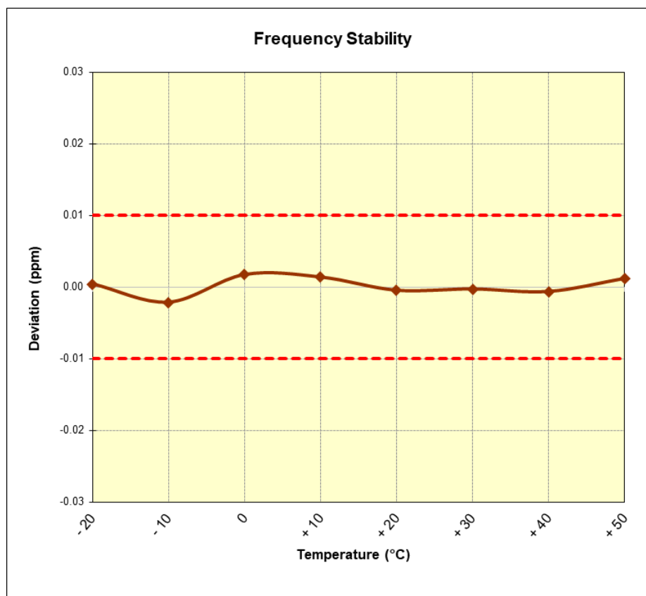
Figure 7-4. Frequency Stability Plot (Reader 10% ASK 1 out of 4)
