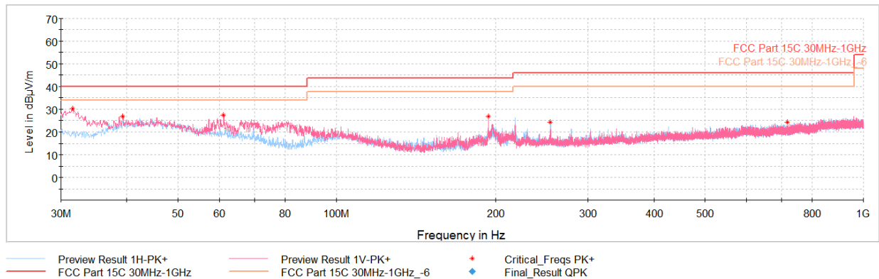
Plot 6-12. Radiated Spurious Emissions 30MHz – 1GHz (Mode 1, with Host Laptop via USB-C Cable)
