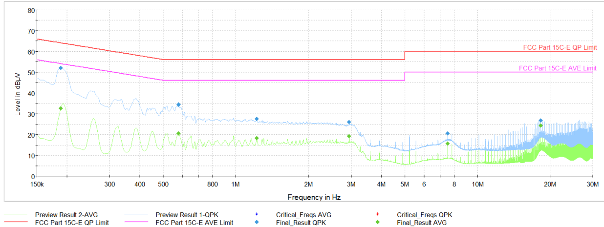
Plot 6-14. AC Line Conducted Plot (N - Mode 1, with Host Laptop via USB-C Cable)
