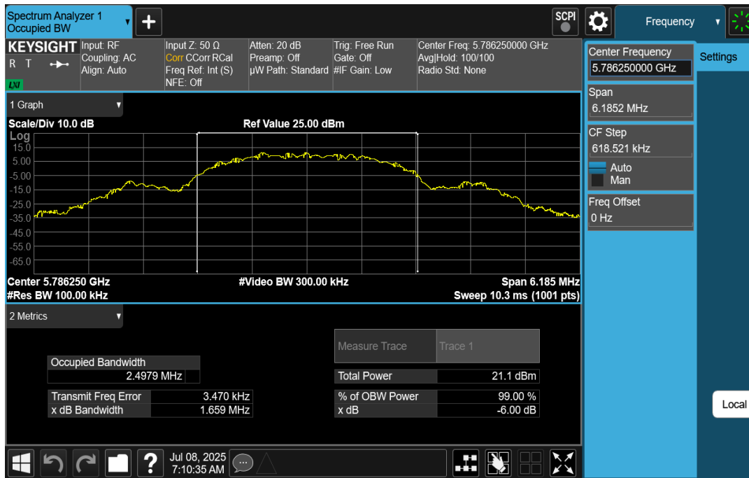
Plot 7-5. 6dB BW & 99% OBW (O-QPSK – 5786.25MHz, 500kbps)
