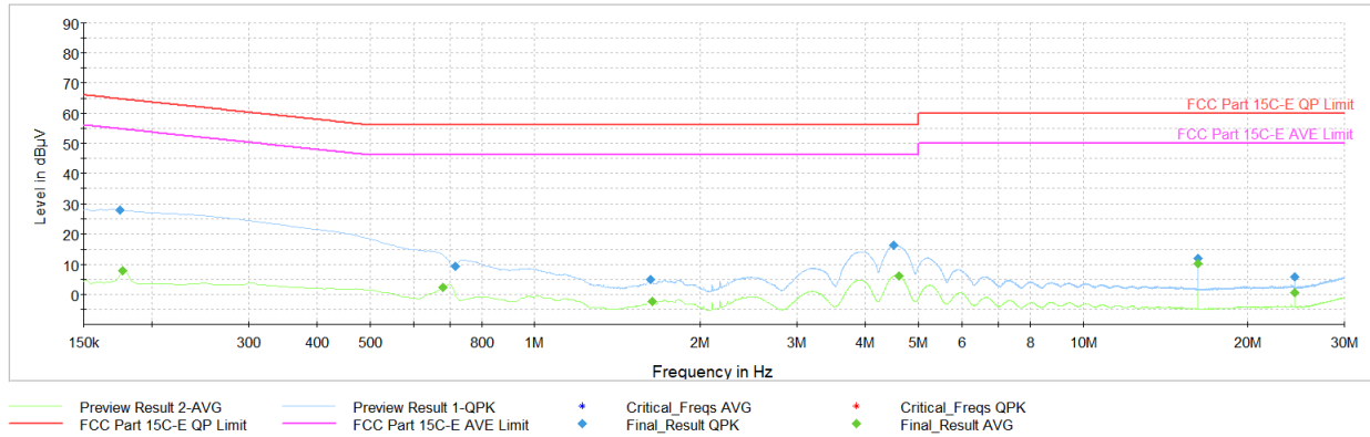
Plot 7-30. AC Line Conducted Plot WF1 (O-QPSK – 5786.25MHz) (L1) with AC/DC adaptor to USB-C cable with wire charger
