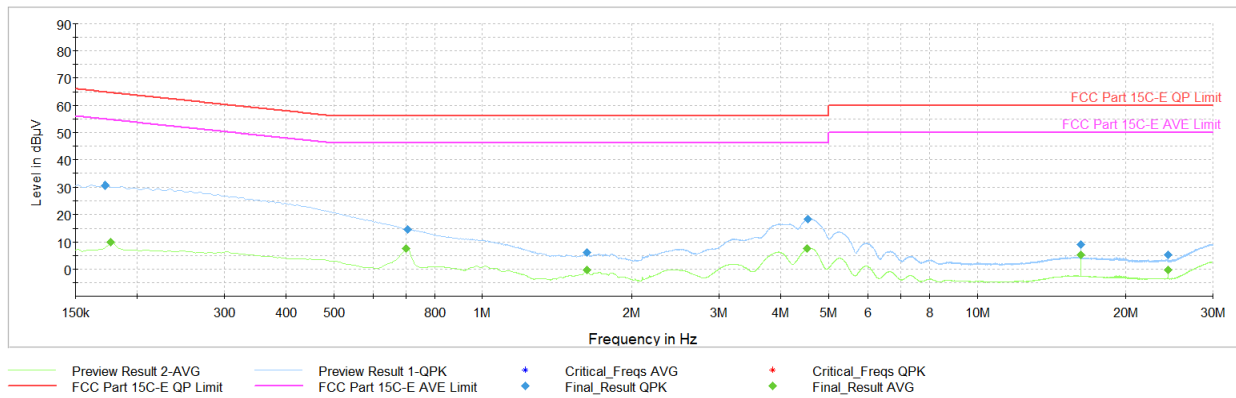
Plot 7-31. AC Line Conducted Plot WF1 (O-QPSK – 5786.25MHz) (N) with AC/DC adaptor to USB-C cable with wire charger
