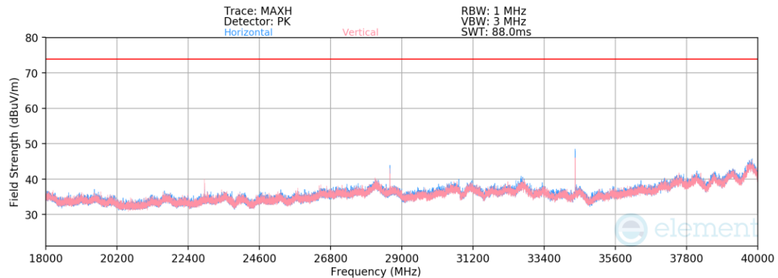
Plot 7-20. Radiated Spurious Emissions Above 18GHz (O-QPSK – 5726.25MHz)
