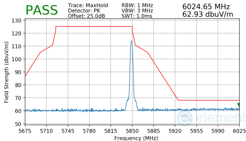
Plot 7-28. Radiated Upper Band Edge Measurement (Pk, 5848.75MHz, O-QPSK, 1000Kbps)
