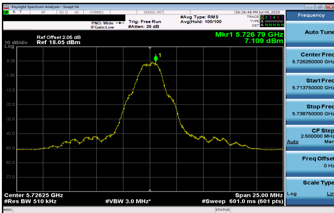
Plot 7-10. PSD (BDR 5726.25MHz, 250kbps)
