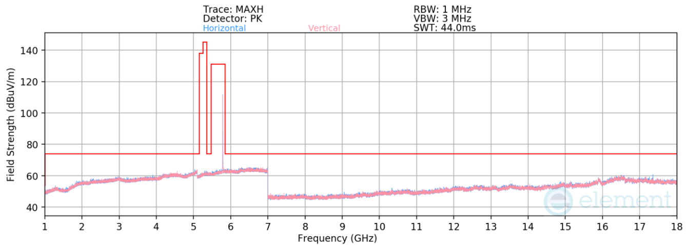
Plot 7-21. Radiated Spurious Emissions 1-18GHz (O-QPSK – 5786.25MHz)
