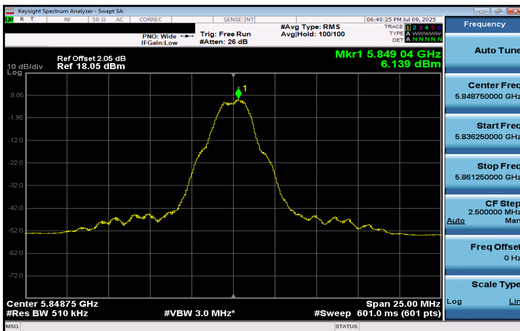
Plot 7-12. PSD (BDR 5848.75MHz, 250kbps)
