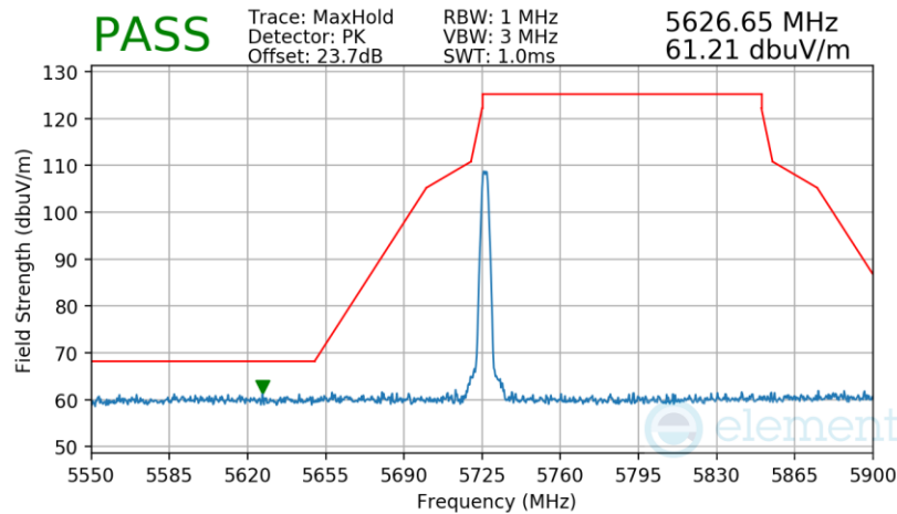
Plot 7-27. Radiated Lower Band Edge Measurement (Pk, 5726.25MHz, O-QPSK, 1000Kbps)
