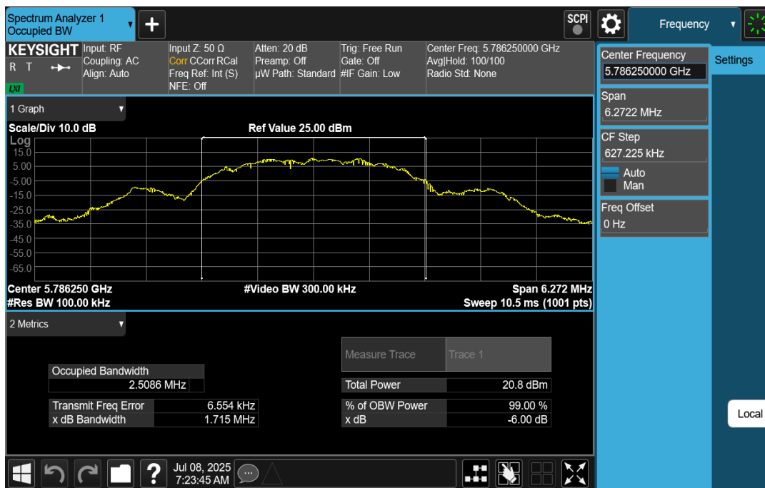
Plot 7-8. 6dB BW & 99% OBW (O-QPSK – 5786.25MHz, 1000kbps )
