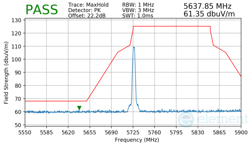
Plot 7-23. Radiated Lower Band Edge Measurement (Pk, 5726.25MHz, O-QPSK, 250Kbps)
