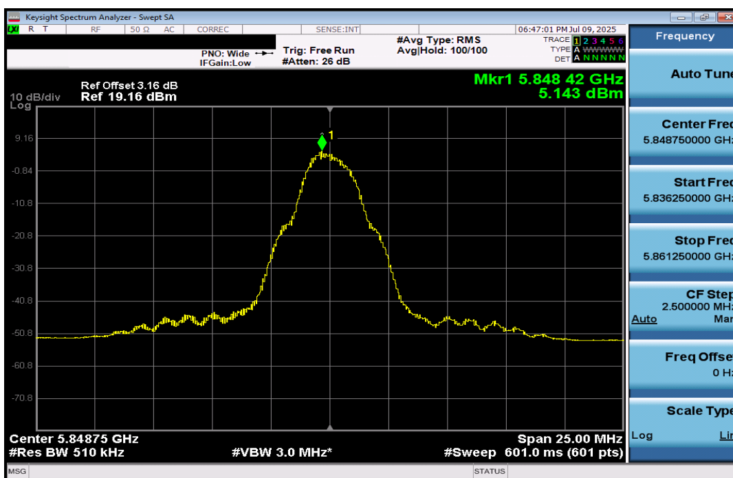
Plot 7-15. PSD (BDR 5848.75MHz, 500kbps)
