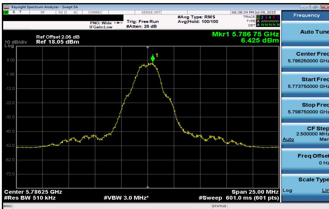
Plot 7-11. PSD (BDR 5786.25MHz, 250kbps)
