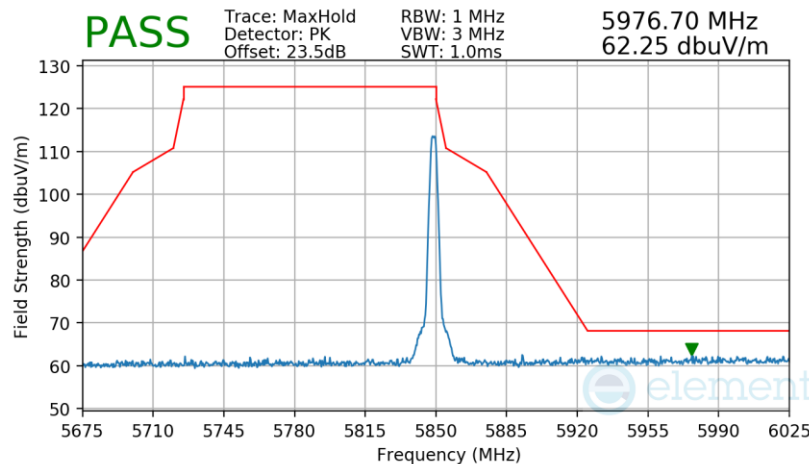
Plot 7-24. Radiated Upper Band Edge Measurement (Pk, 5848.75MHz, O-QPSK, 250Kbps)
