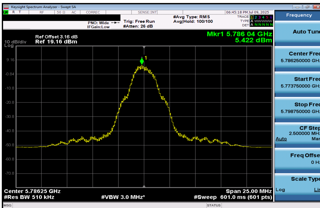
Plot 7-14. PSD (BDR 5786.25MHz, 500kbps)
