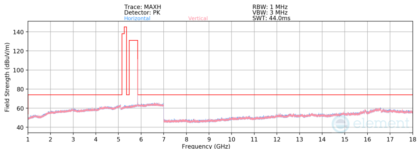
Plot 7-22. Radiated Spurious Emissions 1-18GHz (O-QPSK – 5848.75MHz)
