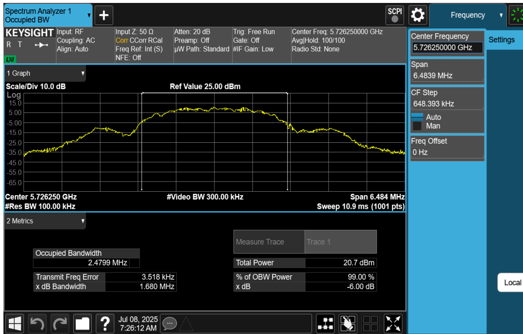
Plot 7-7. 6dB BW & 99% OBW (O-QPSK – 5726.25MHz, 1000kbps )
