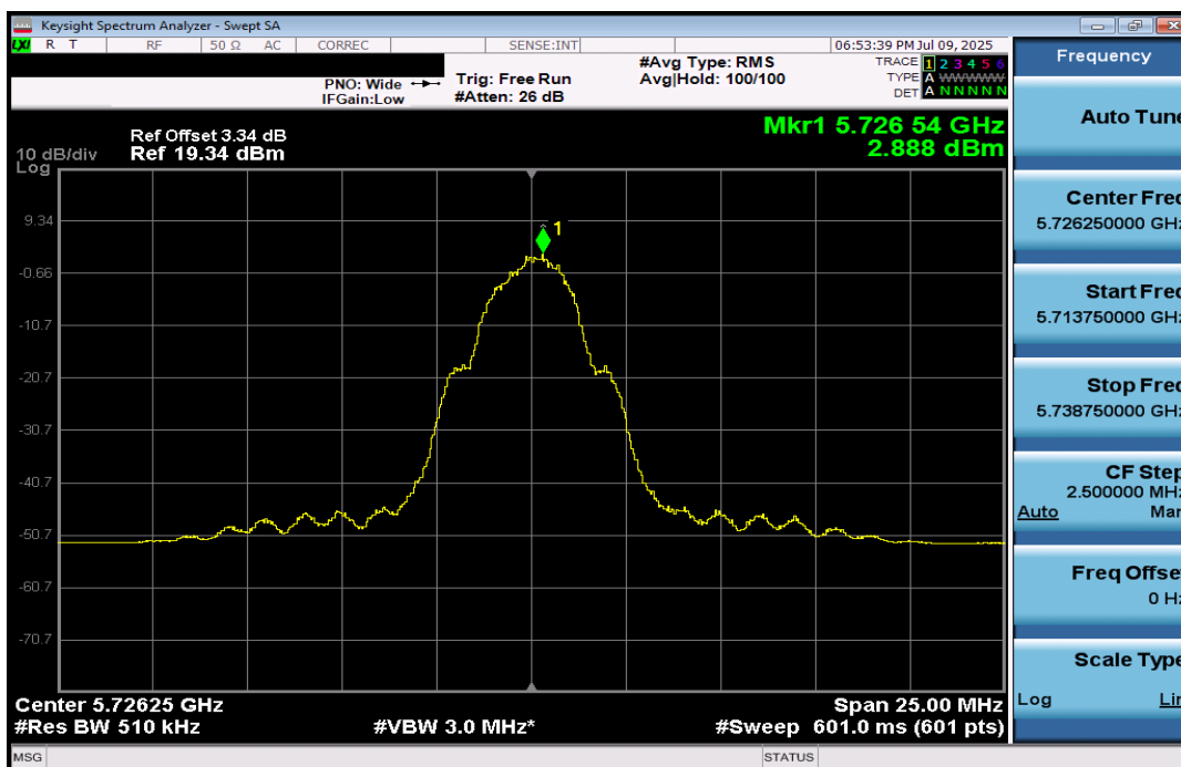
Plot 7-16. PSD (BDR 5726.25MHz, 1000kbps)
