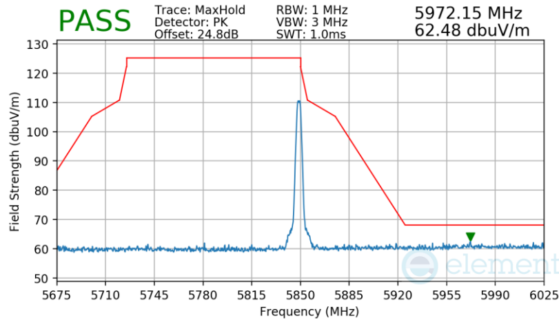
Plot 7-26. Radiated Upper Band Edge Measurement (Pk, 5848.75MHz, O-QPSK, 500Kbps)
