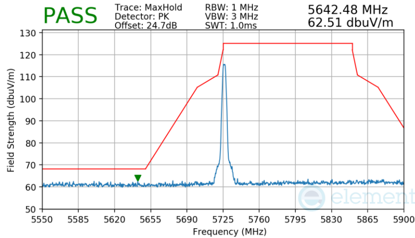
Plot 7-25. Radiated Lower Band Edge Measurement (Pk, 5726.25MHz, O-QPSK, 500Kbps)
