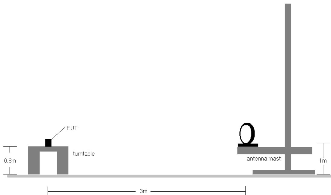
Figure 7-5. Radiated Test Setup < 30MHz
