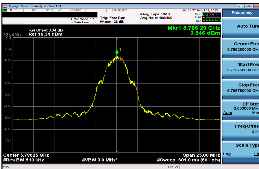
Plot 7-17. PSD (BDR 5786.25MHz, 1000kbps)
