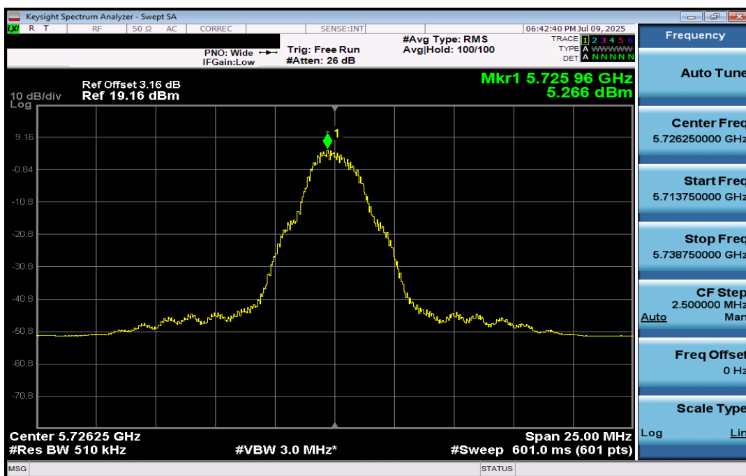
Plot 7-13. PSD (BDR 5726.25MHz, 500kbps)
