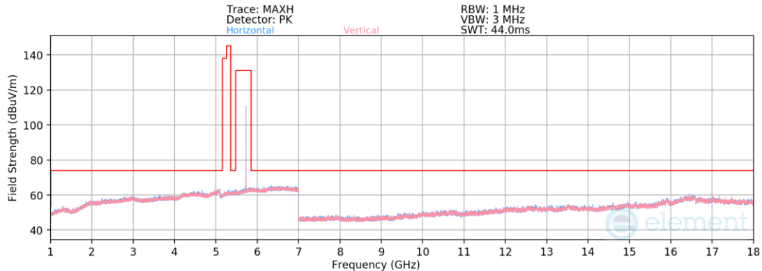
Plot 7-19. Radiated Spurious Emissions 1-18GHz (O-QPSK – 5726.25MHz)
