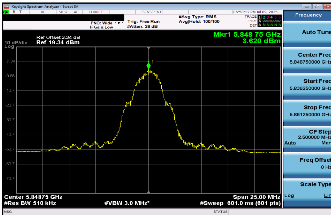
Plot 7-18. PSD (BDR 5848.75MHz, 1000kbps)
