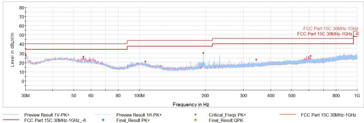
Plot 7-29. Radiated Spurious Emissions Below 1GHz WF1 (O-QPSK – 5786.25MHz), with AC/DC adaptor to USB-C cable with wire charger
