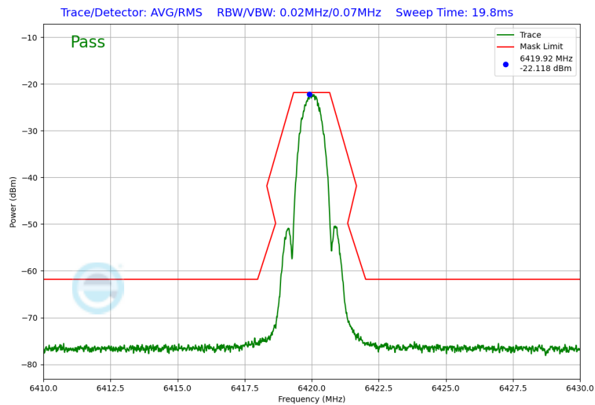
Plot 7-48. In Band Emission Plot (NB UNII LE, 1Mbps – 6420MHz)
