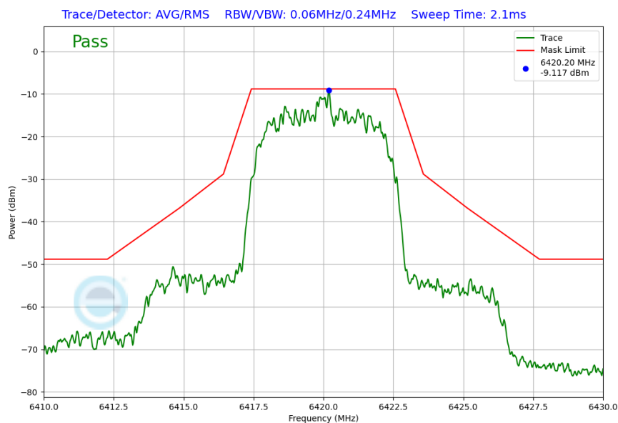
Plot 7-57. In Band Emission Plot (NB UNII HDR8 – 6420MHz)
