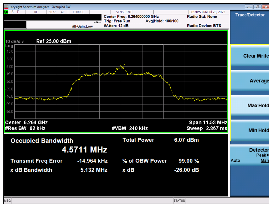
Plot 7-14. 26dB BW & 99% OBW (NB UNII HDR8 – 6264MHz)
