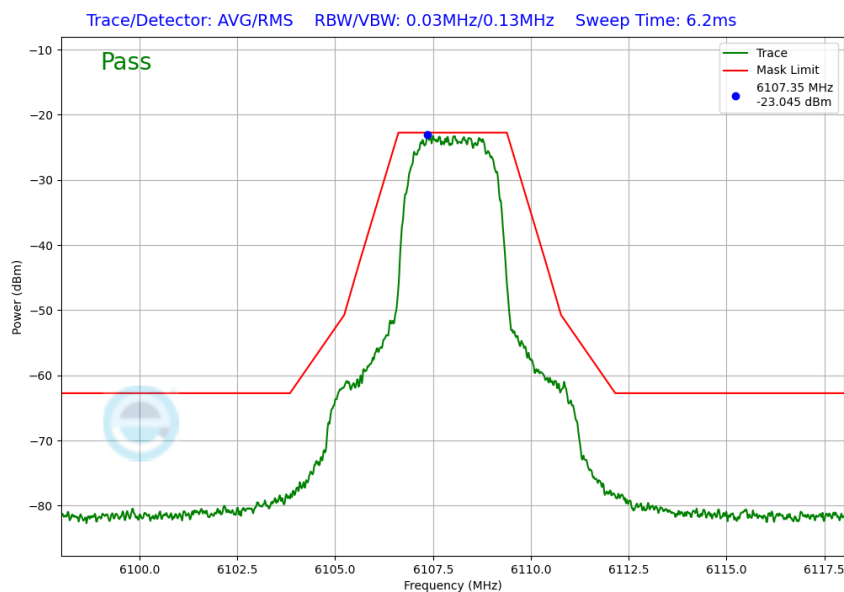
Plot 7-58. In Band Emission Plot (NB UNII HDRp4 – 6108MHz)
