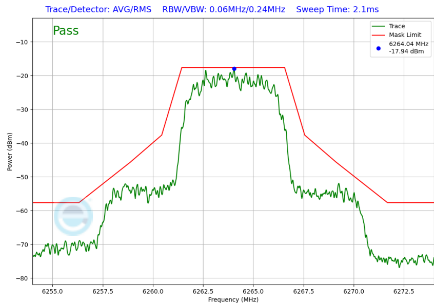
Plot 7-56. In Band Emission Plot (NB UNII HDR8 – 6264MHz)
