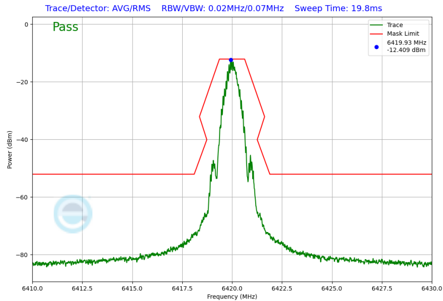
Plot 7-45. In Band Emission Plot (NB UNII BDR – 6420MHz)
