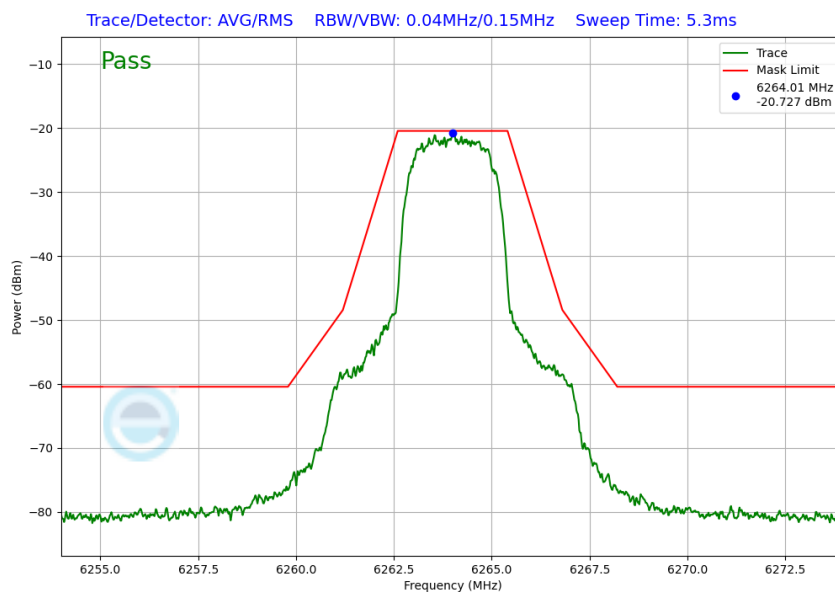
Plot 7-59. In Band Emission Plot (NB UNII HDRp4 – 6264MHz)
