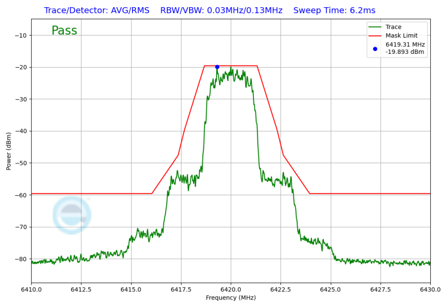
Plot 7-54. In Band Emission Plot (NB UNII HDR4 – 6420MHz)
