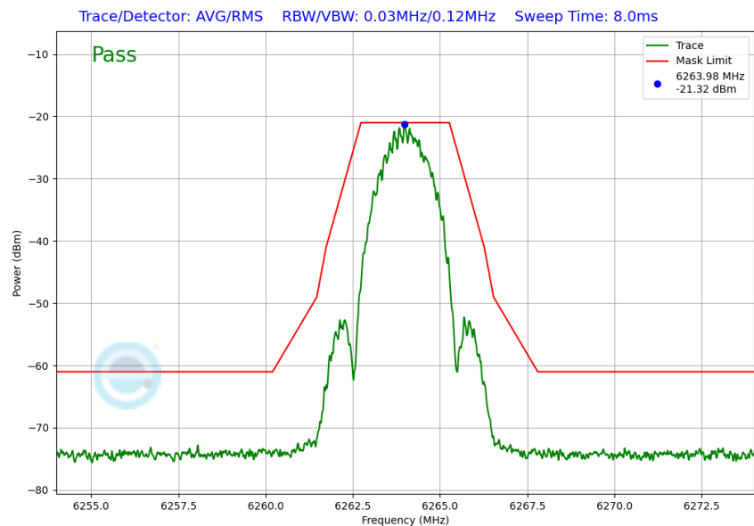
Plot 7-50. In Band Emission Plot (NB UNII LE, 2Mbps – 6264MHz)
