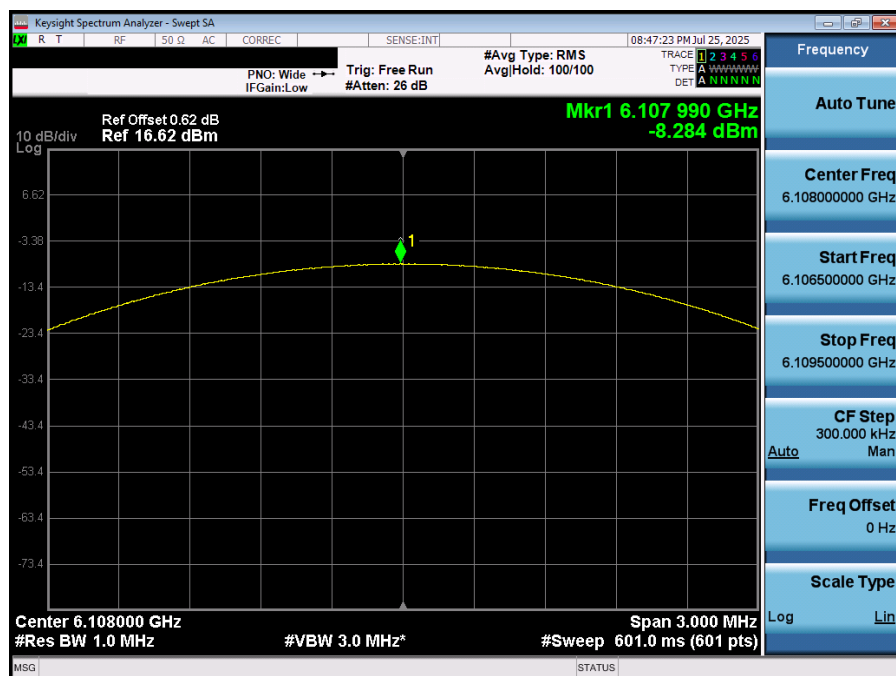
Plot 7-28. PSD (NB UNII LE, 2Mbps – 6108MHz)
