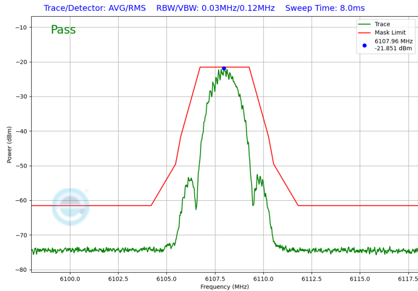
Plot 7-49. In Band Emission Plot (NB UNII LE, 2Mbps – 6108MHz)
