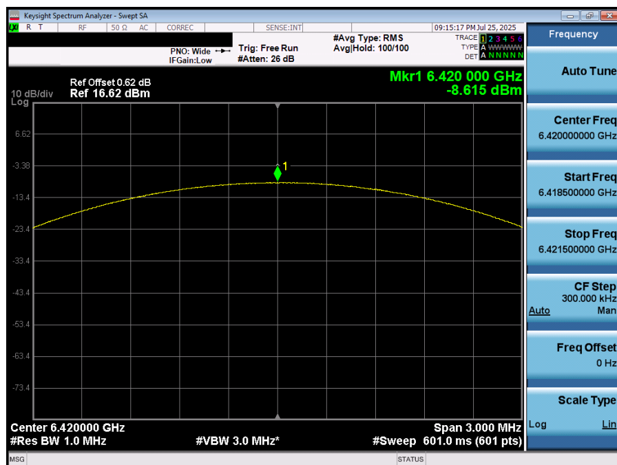
Plot 7-30. PSD (NB UNII LE, 2Mbps – 6420MHz)
