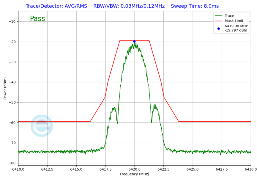
Plot 7-51. In Band Emission Plot (NB UNII LE, 2Mbps – 6420MHz)
