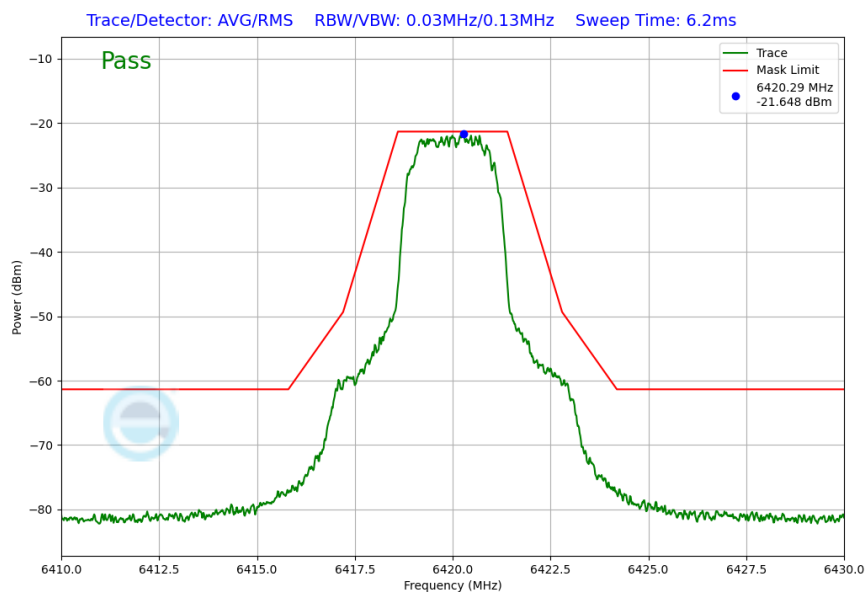
Plot 7-60. In Band Emission Plot (NB UNII HDRp4 – 6420MHz)
