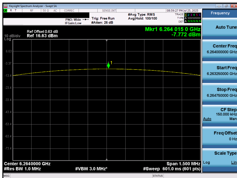
Plot 7-26. PSD (NB UNII LE, 1Mbps – 6264MHz)
