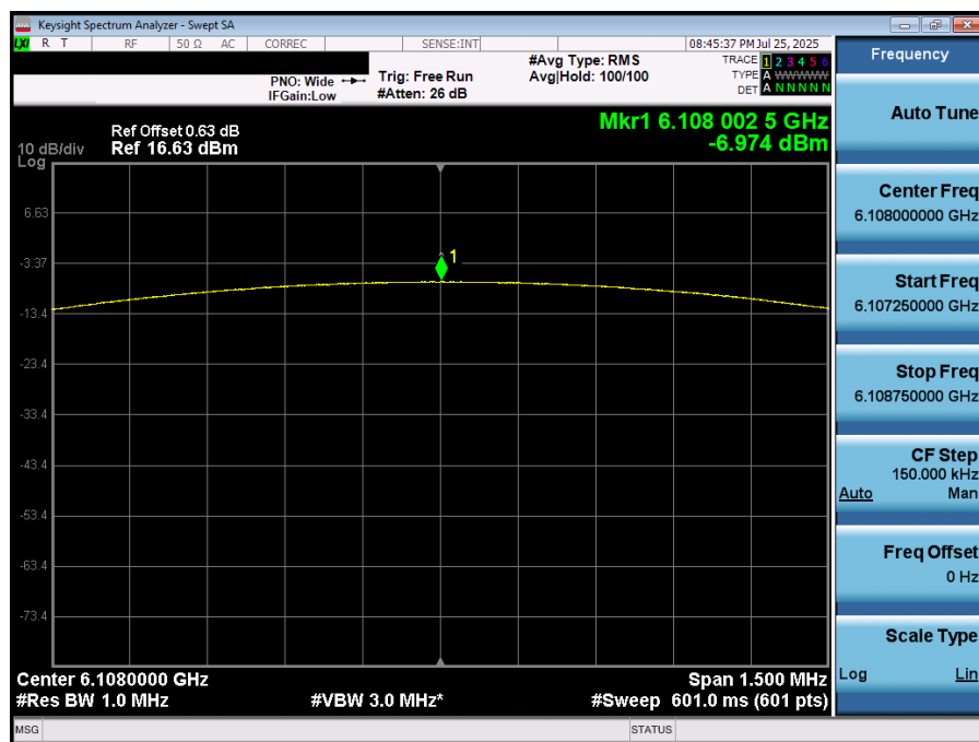
Plot 7-25. PSD (NB UNII LE, 1Mbps – 6108MHz)
