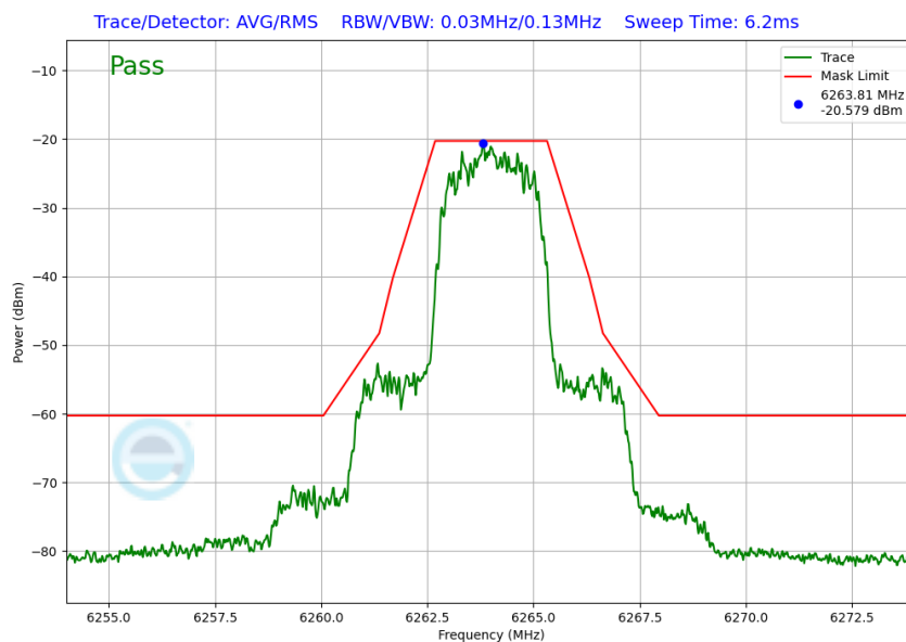
Plot 7-53. In Band Emission Plot (NB UNII HDR4 – 6264MHz)
