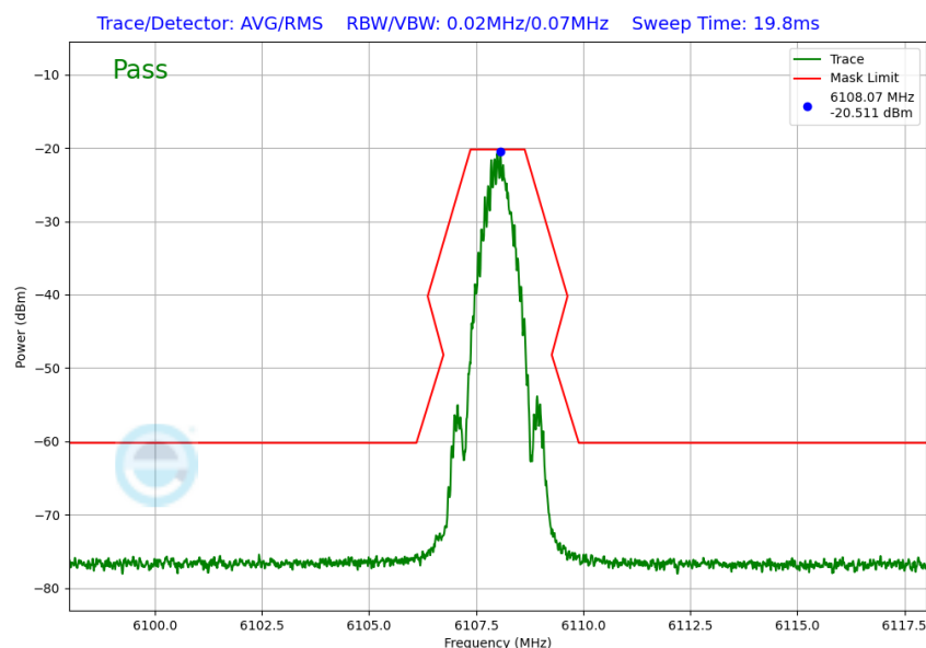
Plot 7-43. In Band Emission Plot (NB UNII BDR – 6108MHz)
