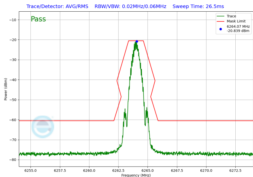
Plot 7-44. In Band Emission Plot (NB UNII BDR – 6264MHz)
