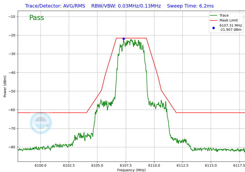
Plot 7-52. In Band Emission Plot (NB UNII HDR4 – 6108MHz)
