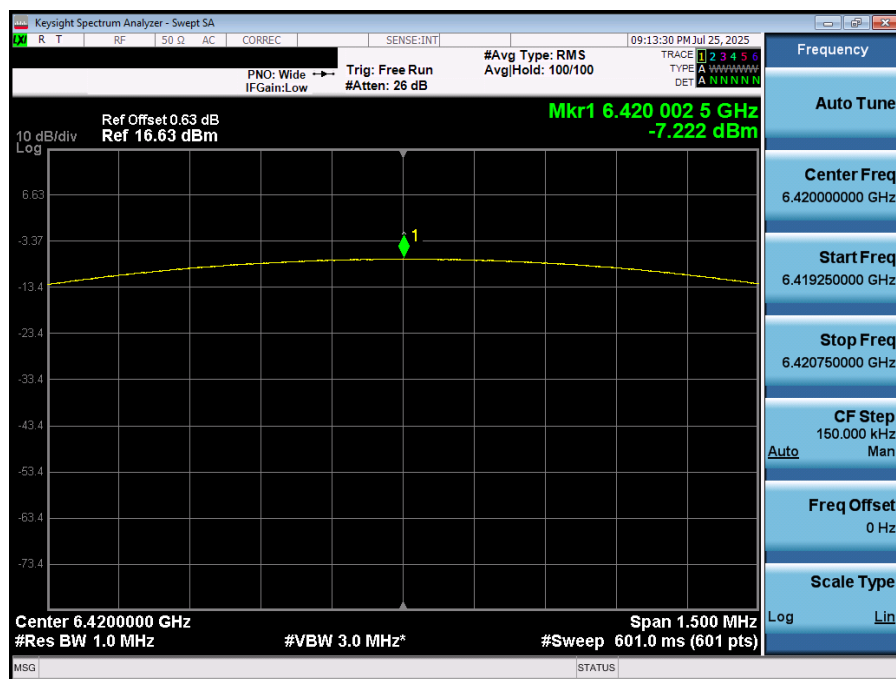
Plot 7-27. PSD (NB UNII LE, 1Mbps – 6420MHz)
