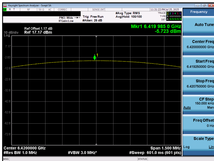
Plot 7-24. PSD (NB UNII BDR – 6420MHz)
