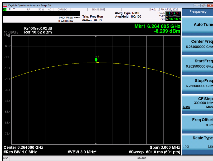
Plot 7-29. PSD (NB UNII LE, 2Mbps – 6264MHz)
