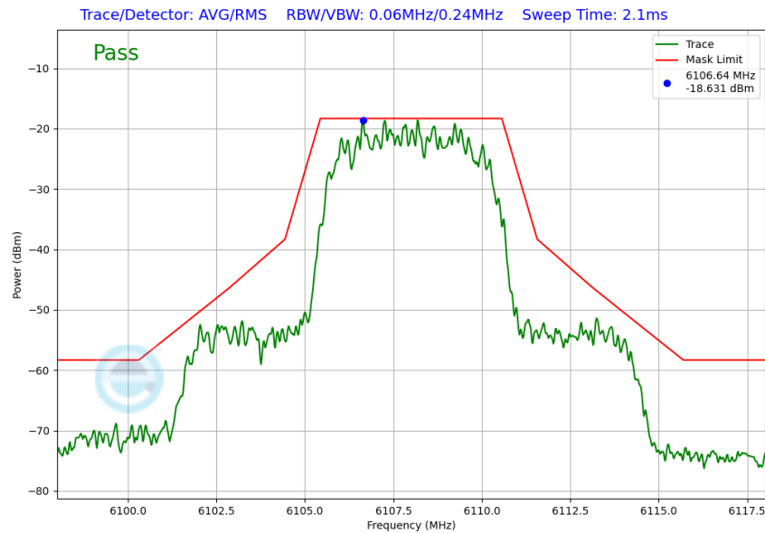
Plot 7-55. In Band Emission Plot (NB UNII HDR8 – 6108MHz)
