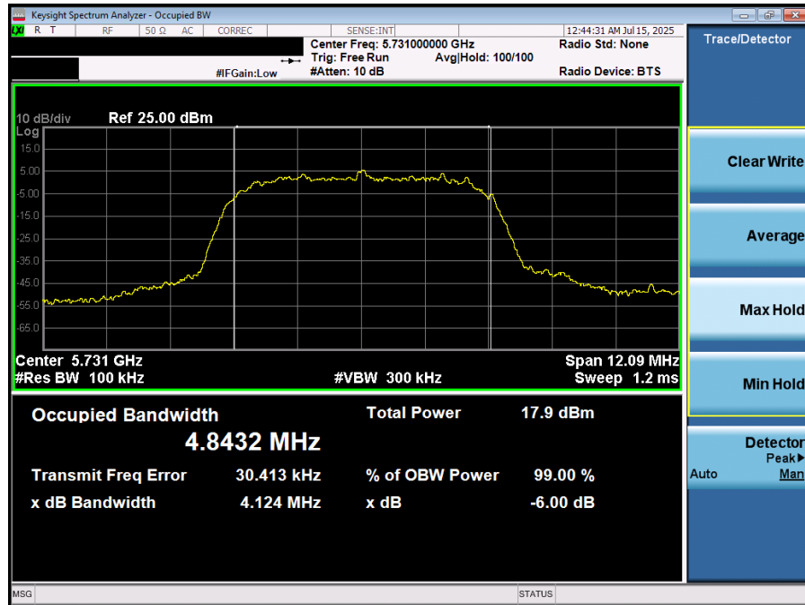
Plot 7-40. 6dB BW & 99% OBW (NB UNII HDRp8 – 5731MHz)
