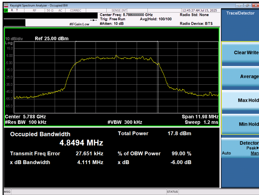
Plot 7-41. 6dB BW & 99% OBW (NB UNII HDRp8 – 5788MHz)
