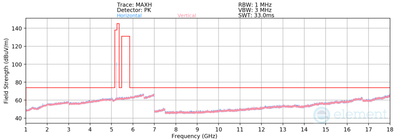
Plot 7-88. Radiated Spurious Emissions 1-18GHz (BDR GFSK – 5245MHz)
