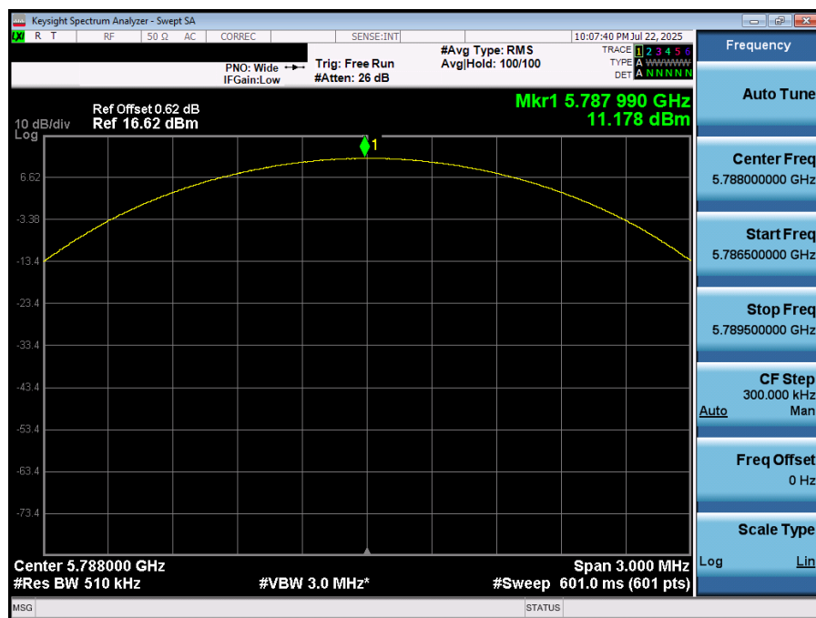
Plot 7-71. PSD (NB UNII LE2M - 5788MHz)
