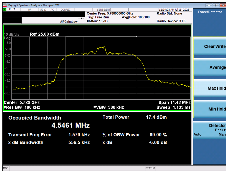
Plot 7-35. 6dB BW & 99% OBW (NB UNII HDR8 – 5788MHz)
