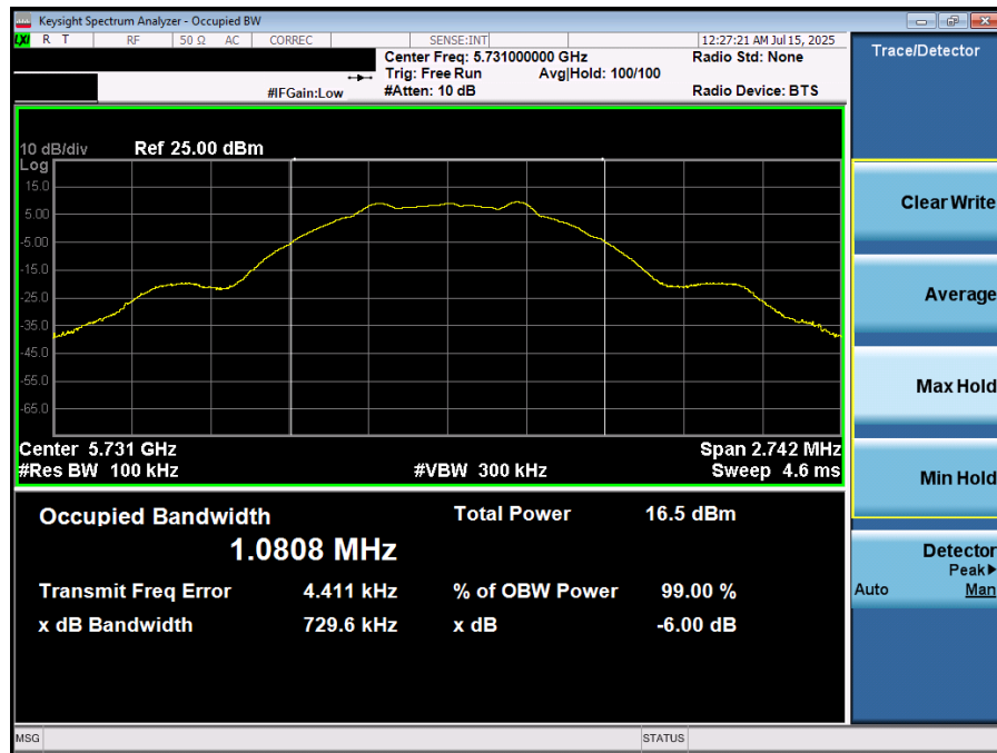
Plot 7-25. 6dB BW & 99% OBW (NB UNII LE1M – 5731MHz)
