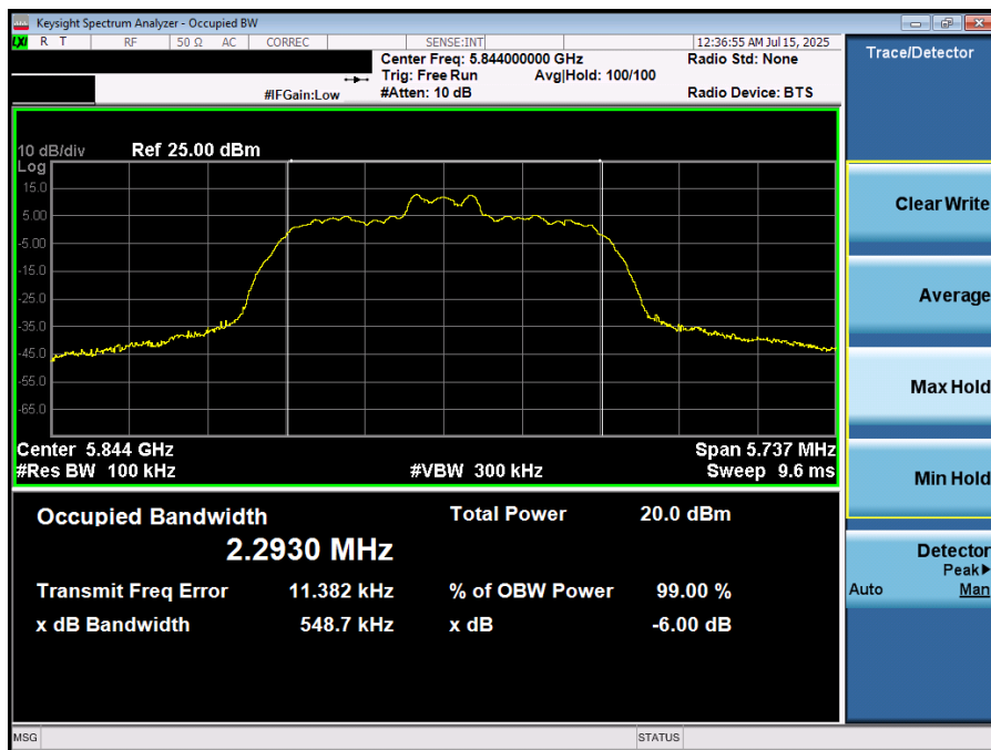
Plot 7-33. 6dB BW & 99% OBW (NB UNII HDR4 – 5844MHz)
