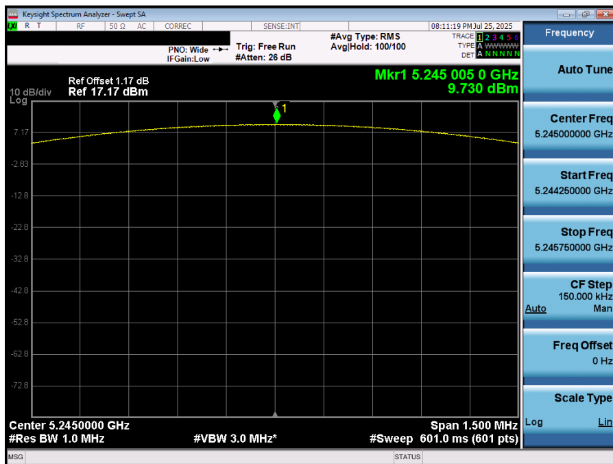
Plot 7-45. PSD (NB UNII BDR - 5245MHz)
