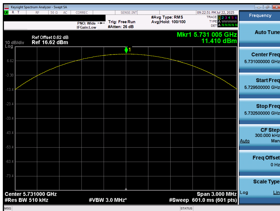
Plot 7-70. PSD (NB UNII LE2M - 5731MHz)
