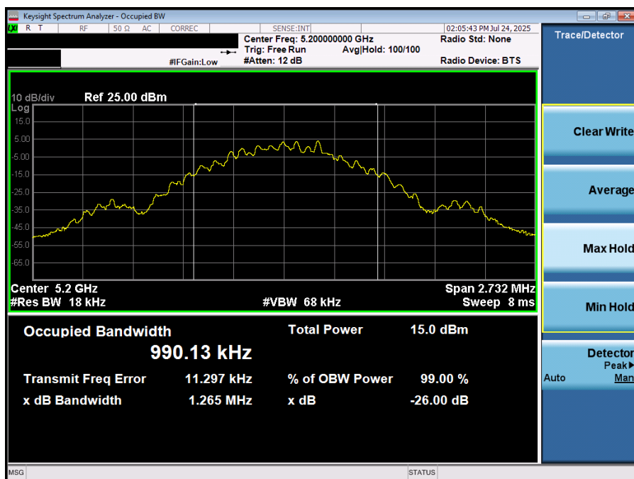
Plot 7-2. 26dB BW & 99% OBW (NB UNII BDR– 5200MHz)
