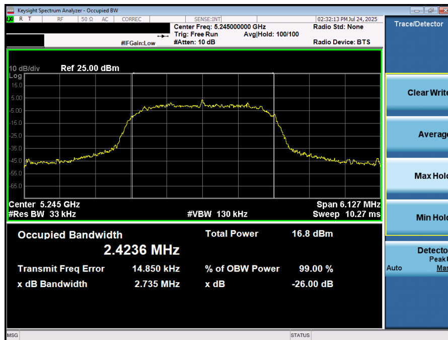
Plot 7-18. 26dB BW & 99% OBW (NB UNII HDRp4- 5245MHz)
