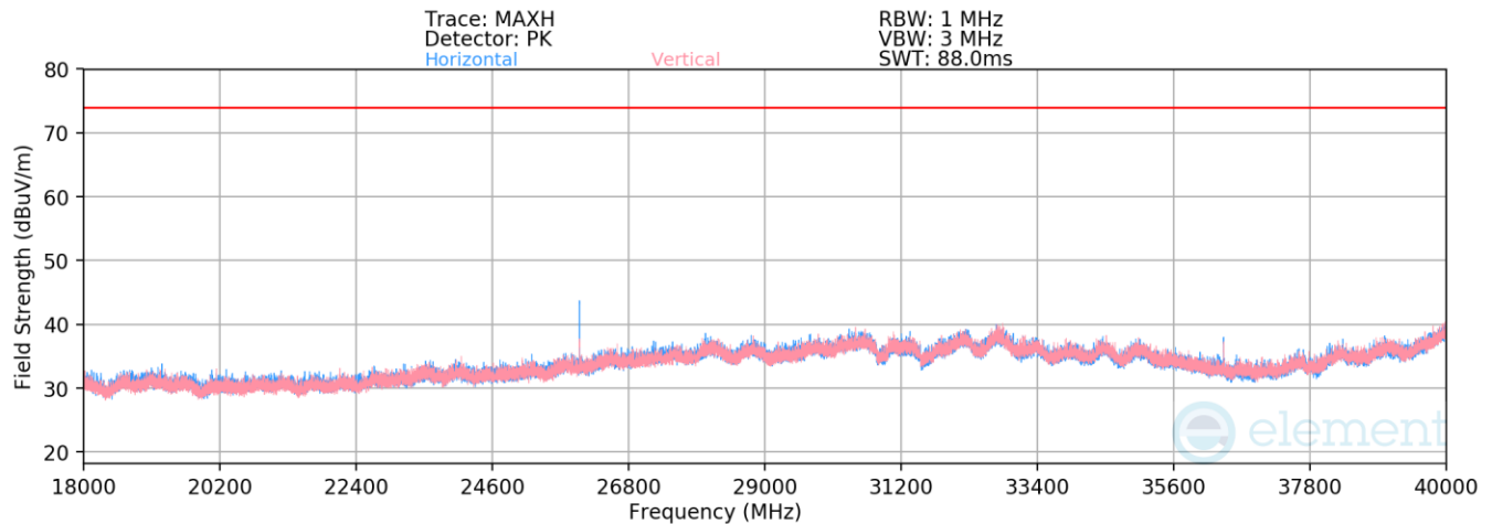
Plot 7-87. Radiated Spurious Emissions Above 18GHz (BDR GFSK – 5200MHz)
