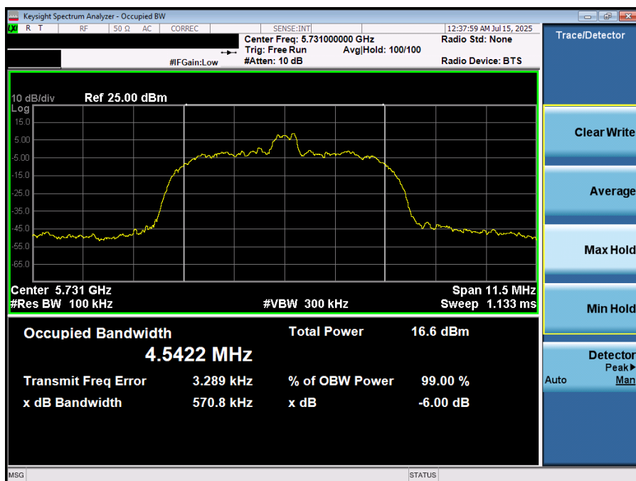
Plot 7-34. 6dB BW & 99% OBW (NB UNII HDR8 – 5731MHz)
