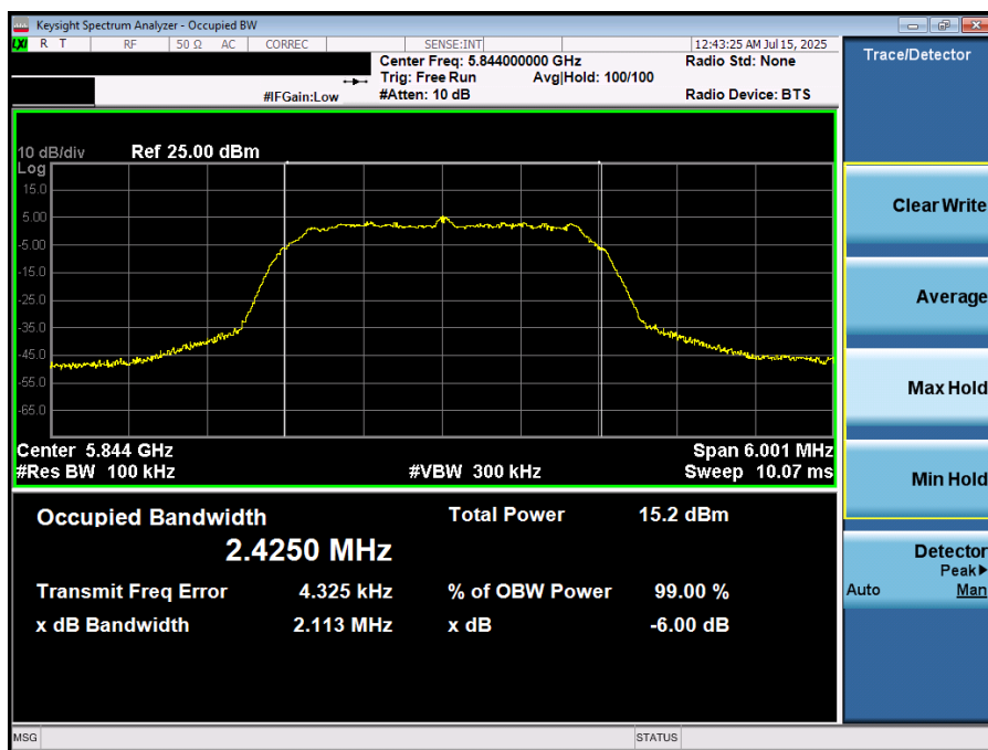
Plot 7-39. 6dB BW & 99% OBW (NB UNII HDRp4 – 5844MHz)
