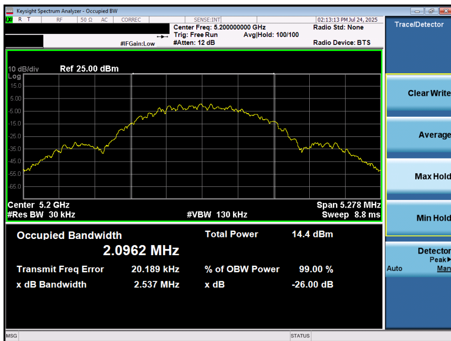
Plot 7-8. 26dB BW & 99% OBW (NB UNII LE2M – 5200MHz)
