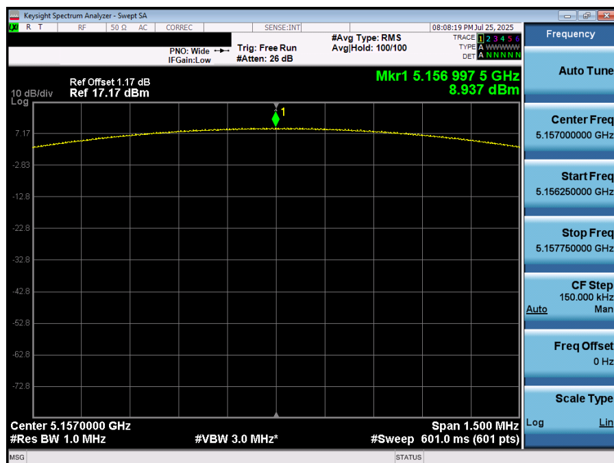
Plot 7-43. PSD (NB UNII BDR – 5157MHz)
