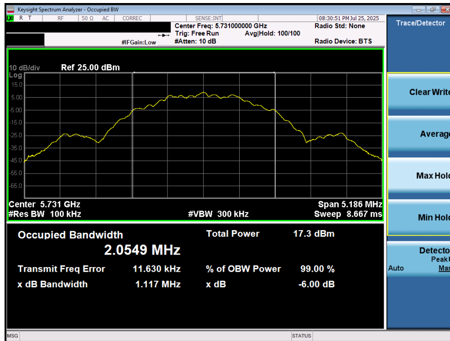
Plot 7-28. 6dB BW & 99% OBW (NB UNII LE2M – 5731MHz)
