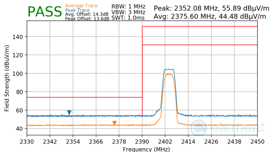
Plot 7-52. Radiated Restricted Lower Band Edge Measurement
