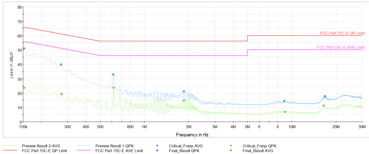
Plot 7-58. AC Line Conducted Plot with Bluetooth (N, HDR4 – Ch.38 with AC/DC adaptor via USB-C cable)
