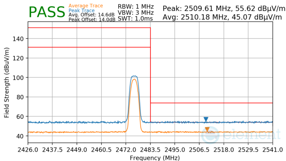
Plot 7-53. Radiated Restricted Upper Band Edge Measurement
