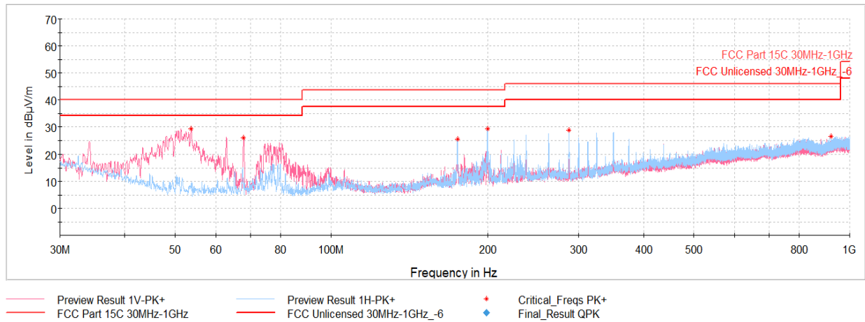
Plot 7-55. Radiated Spurious Emissions Below 1GHz (HDR4 – Ch.1 with AC/DC adaptor via USB-C cable)
