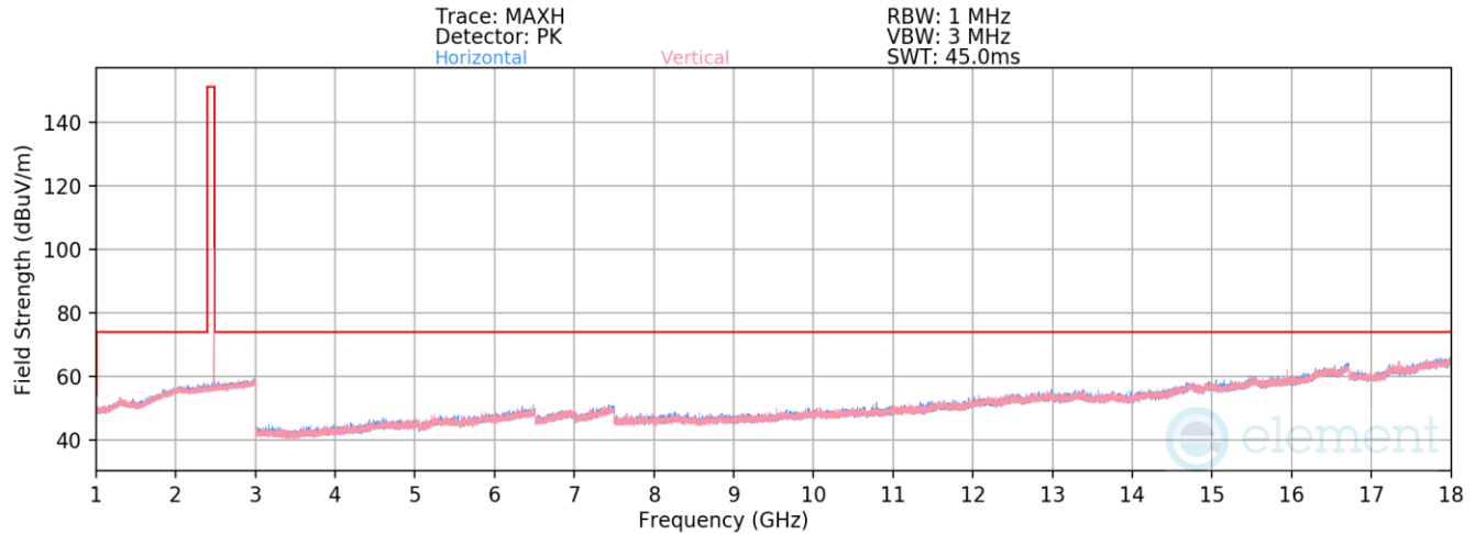
Plot 7-42. Radiated Spurious Emissions 1-18GHz (4Mbps, HDR4 – Ch. 73)
