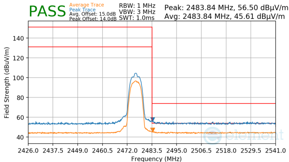
Plot 7-50. Radiated Restricted Upper Band Edge Measurement
