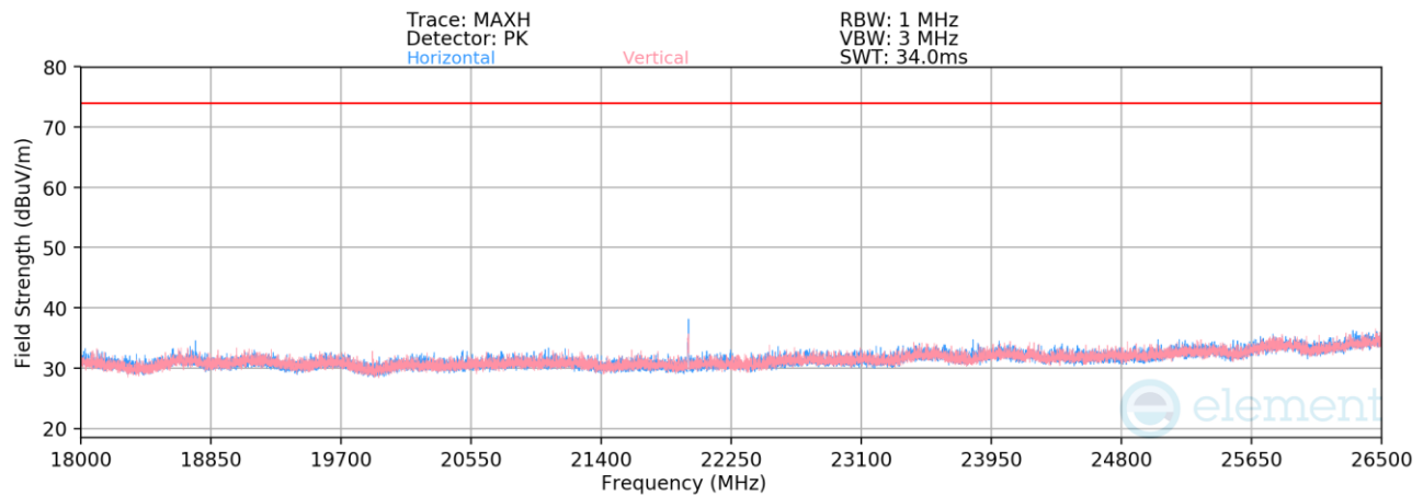
Plot 7-41. Radiated Spurious Emissions 18-26.5GHz (4Mbps, HDR4 – Ch. 38)
