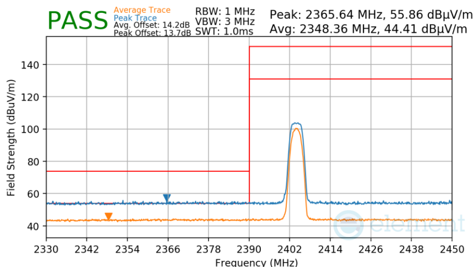
Plot 7-51. Radiated Restricted Lower Band Edge Measurement
