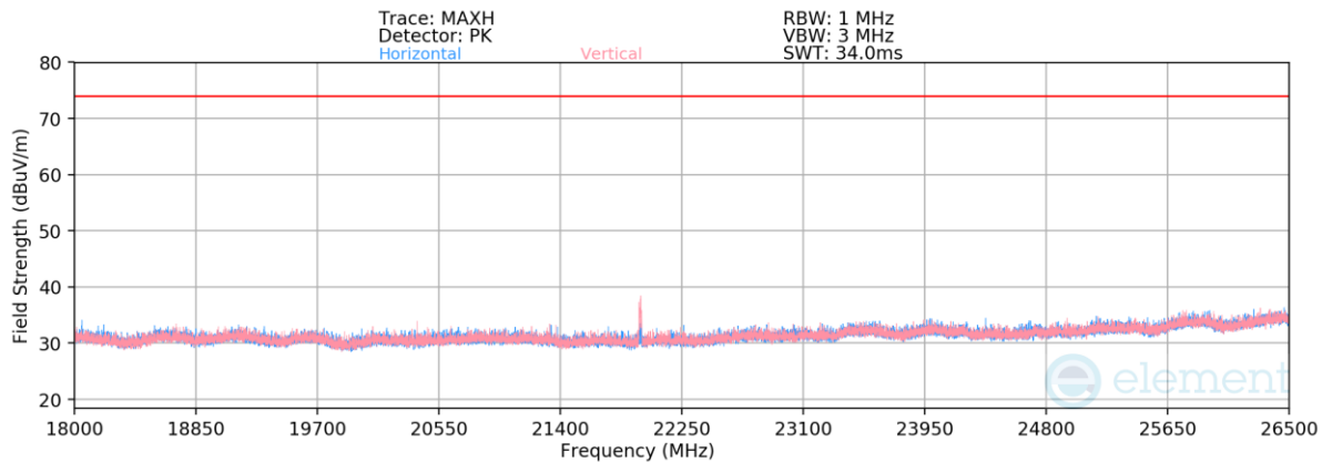
Plot 7-45. Radiated Spurious Emissions 18-26.5GHz (4Mbps, HDRp4 – Ch. 38)
