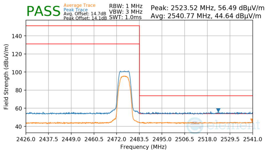
Plot 7-54. Radiated Restricted Upper Band Edge Measurement
