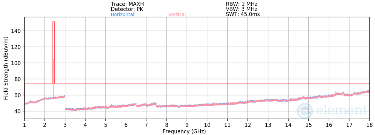
Plot 7-44. Radiated Spurious Emissions 1-18GHz (4Mbps, HDRp4 – Ch. 38)
