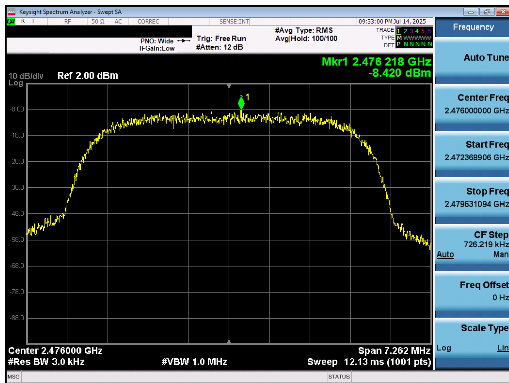
Plot 7-24. Power Spectral Density Plot (Bluetooth (HDR8), 8Mbps – Ch. 73)
