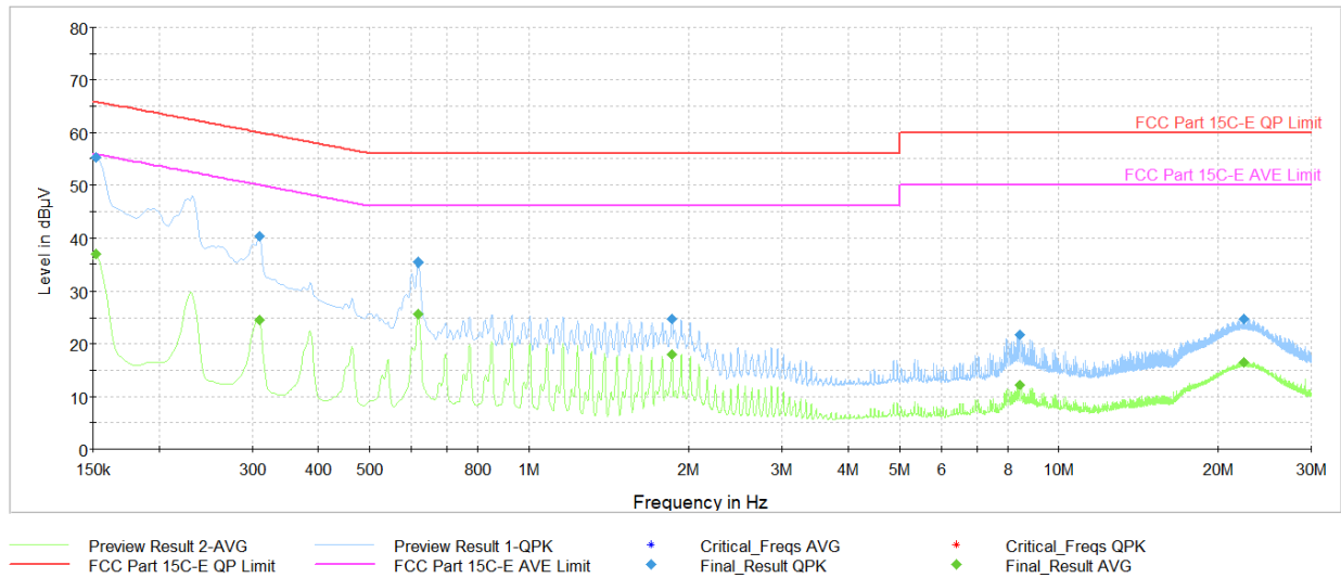
Plot 7-59. AC Line Conducted Plot with Bluetooth (L1, HDRp4 – Ch.38 with AC/DC adaptor via USB-C cable)
