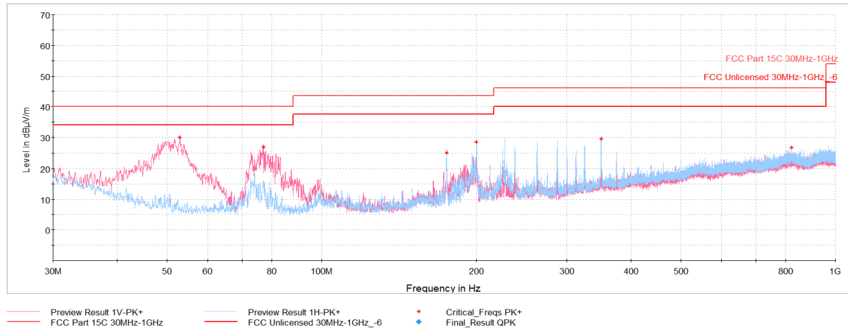
Plot 7-56. Radiated Spurious Emissions Below 1GHz (HDRp4 – Ch.1 with AC/DC adaptor via USB-C cable)
