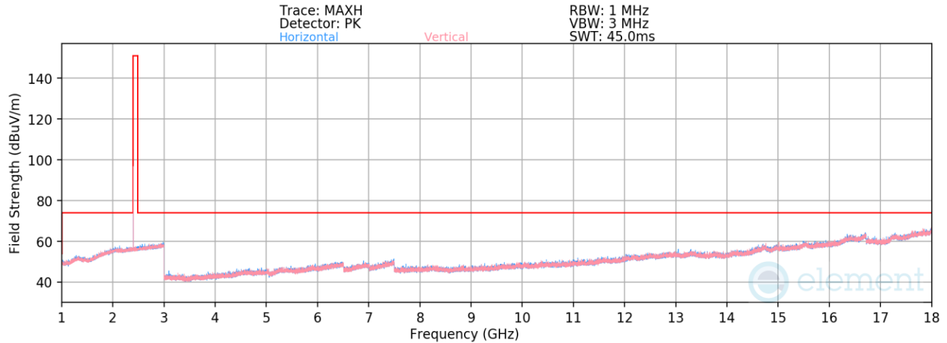
Plot 7-43. Radiated Spurious Emissions 1-18GHz (4Mbps, HDRp4 – Ch. 1)
