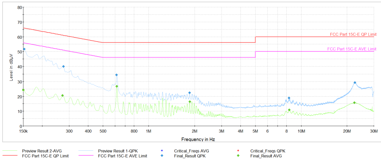
Plot 7-57. AC Line Conducted Plot with Bluetooth (L1, HDR4 – Ch.38 with host PC via USB-C cable)
