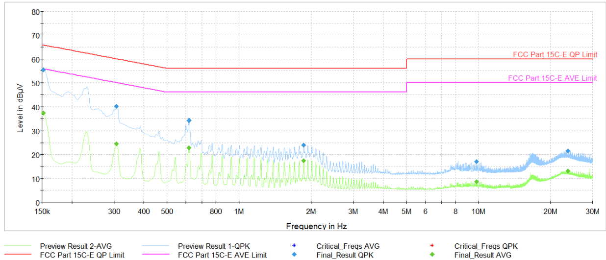
Plot 7-60. AC Line Conducted Plot with Bluetooth (N, HDRp4 – Ch.38 with AC/DC adaptor via USB-C cable)
