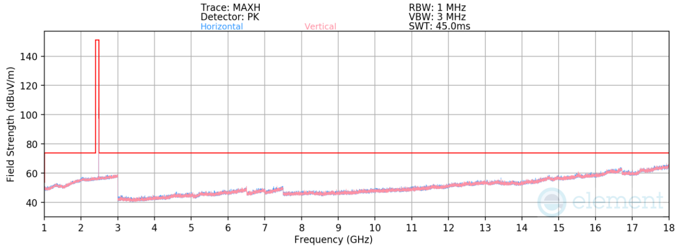
Plot 7-46. Radiated Spurious Emissions 1-18GHz (4Mbps, HDRp4 – Ch. 73)
