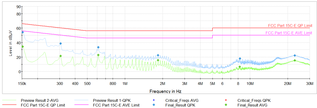
Plot 7-39. AC Line-Conducted Test Plot (N, GFSK – Ch.39, with host PC via USB-C cable)
