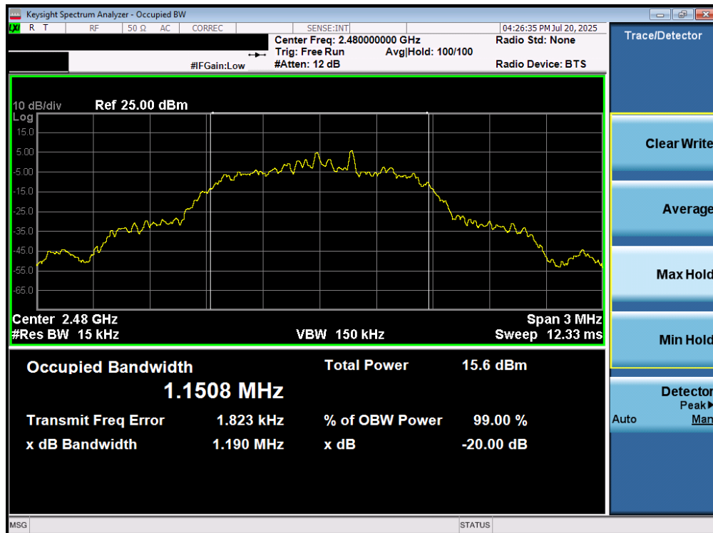
Plot 7-6. 20dB BW and 99% OBW Plot (Bluetooth, 8DPS – Ch. 78)
