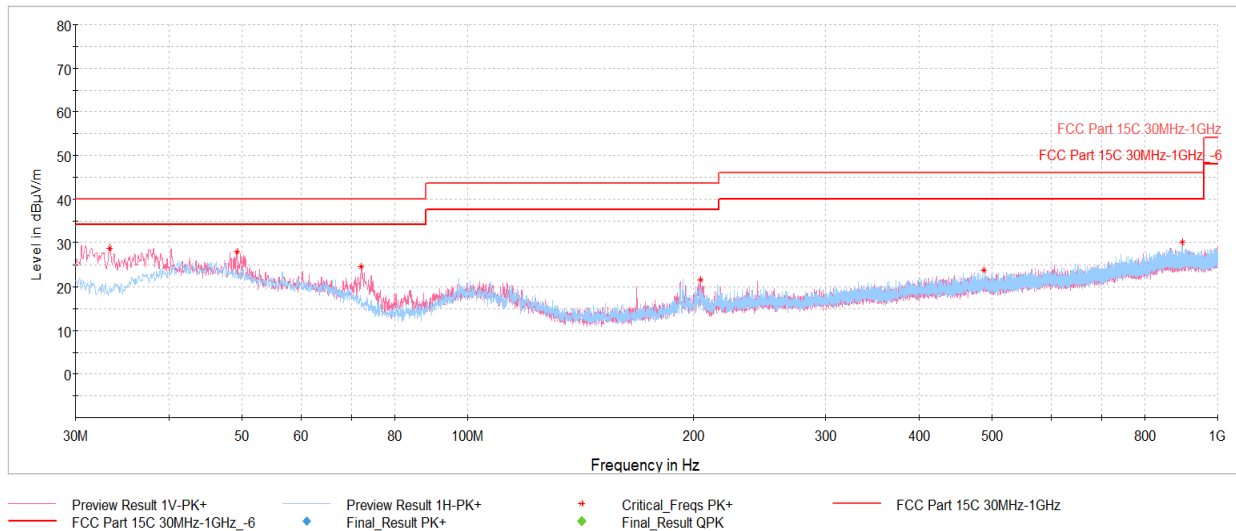
Plot 7-37. Radiated Spurious Emissions Below 1GHz (GFSK – Ch.39, with AC/DC adaptor via USB-C cable)
