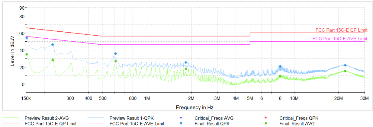
Plot 7-38. AC Line-Conducted Test Plot (L1, GFSK – Ch.39, with host PC via USB-C cable)
