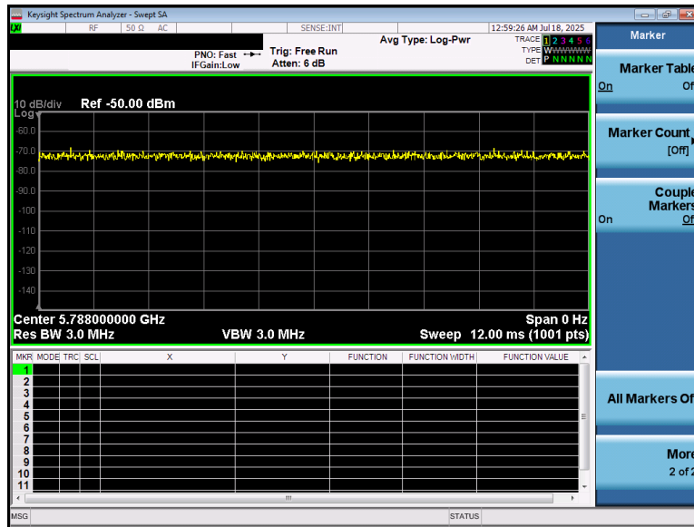
Equation 7-3 NB UNII-3 Duty Cycle Calculation
