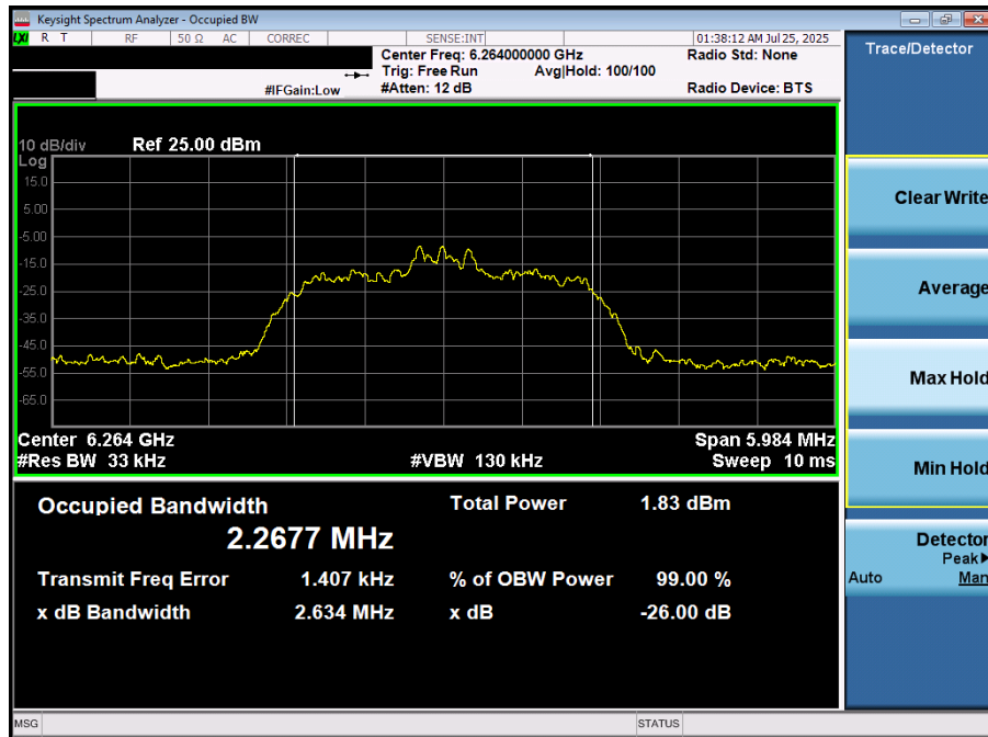
Plot 7-11. 26dB BW & 99% OBW (NB UNII HDR4 – 6264MHz)
