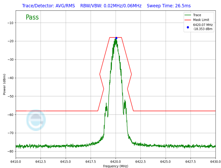
Plot 7-45. In Band Emission Plot (NB UNII BDR – 6420MHz)
