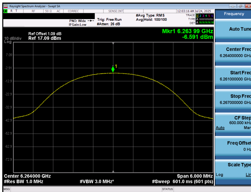
Plot 7-32. PSD (NB UNII HDR4 – 6264MHz)
