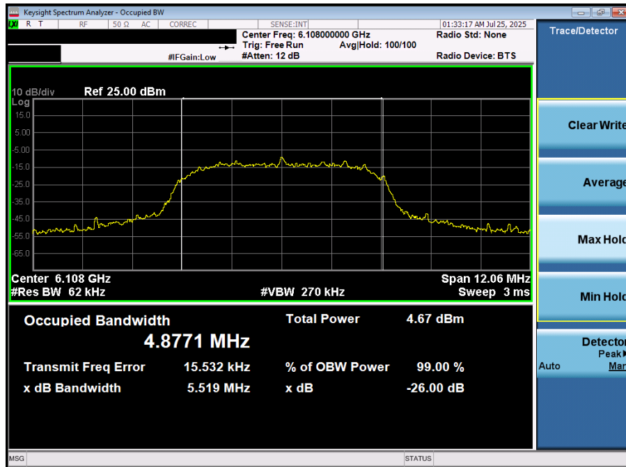
Plot 7-19. 26dB BW & 99% OBW (NB UNII HDRp8 – 6108MHz)
