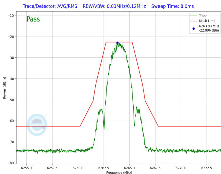
Plot 7-50. In Band Emission Plot (NB UNII LE2M – 6264MHz)
