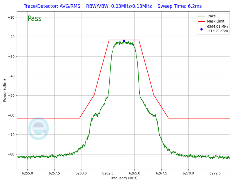
Plot 7-59. In Band Emission Plot (NB UNII HDRp4 – 6264MHz)
