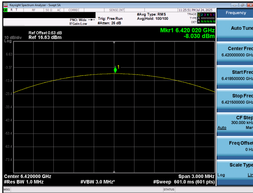
Plot 7-30. PSD (NB UNII LE2M – 6420MHz)
