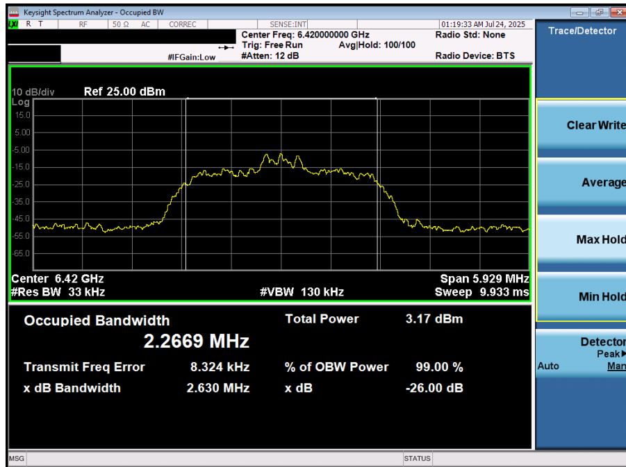
Plot 7-12. 26dB BW & 99% OBW (NB UNII HDR4 – 6420MHz)
