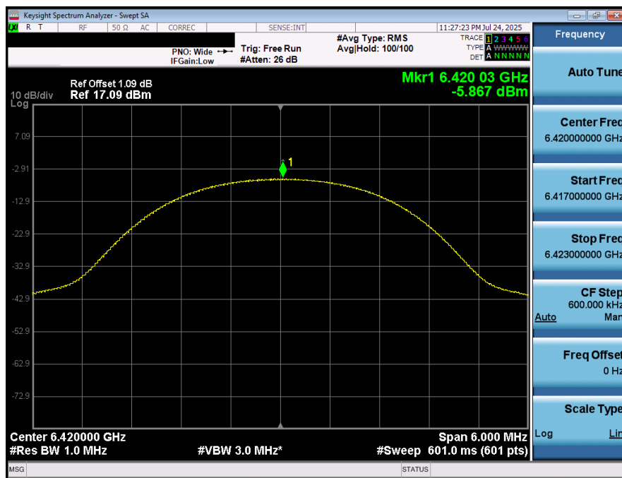
Plot 7-33. PSD (NB UNII HDR4 – 6420MHz)
