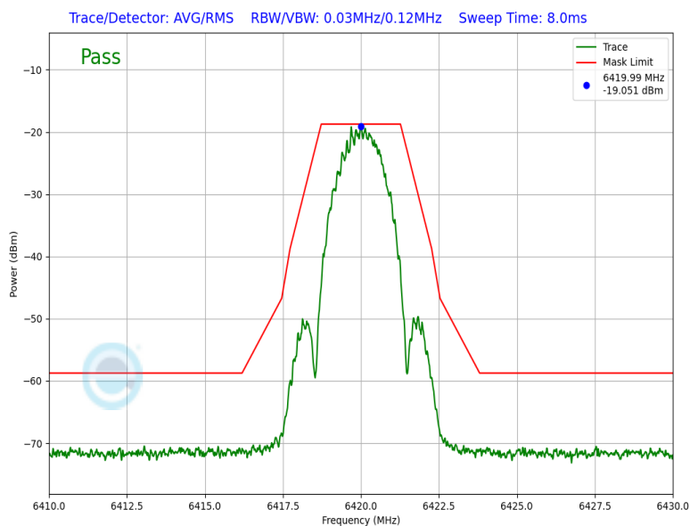
Plot 7-51. In Band Emission Plot (NB UNII LE2M – 6420MHz)
