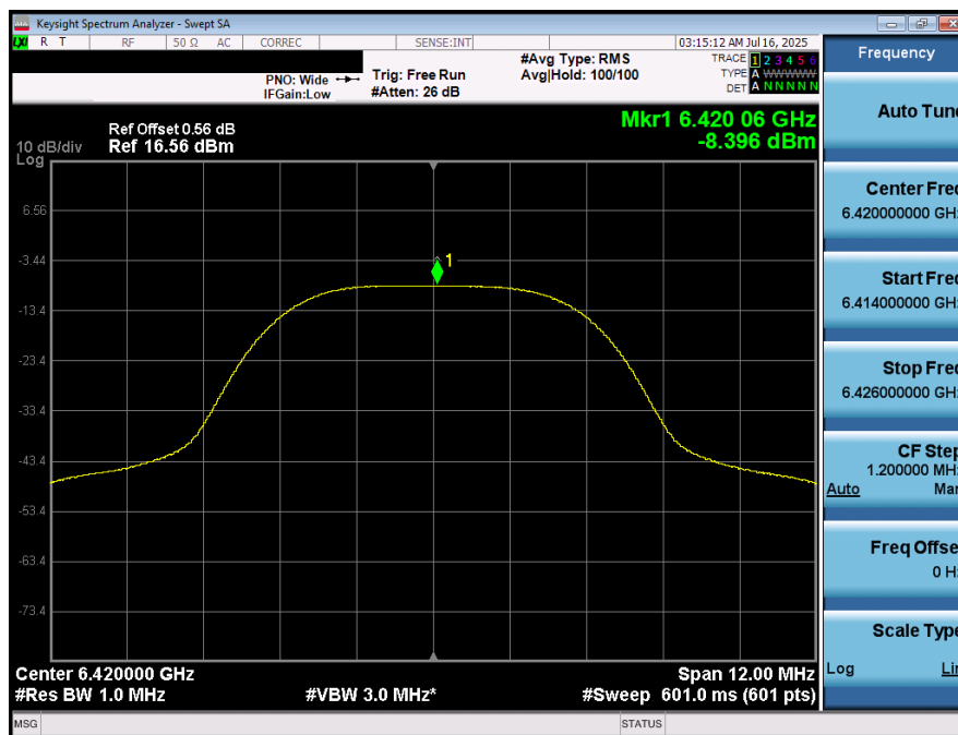
Plot 7-42. PSD (NB UNII HDRp8 – 6420MHz)
