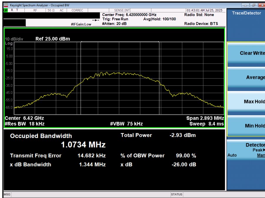
Plot 7-6. 26dB BW & 99% OBW (NB UNII LE1M – 6420MHz)
