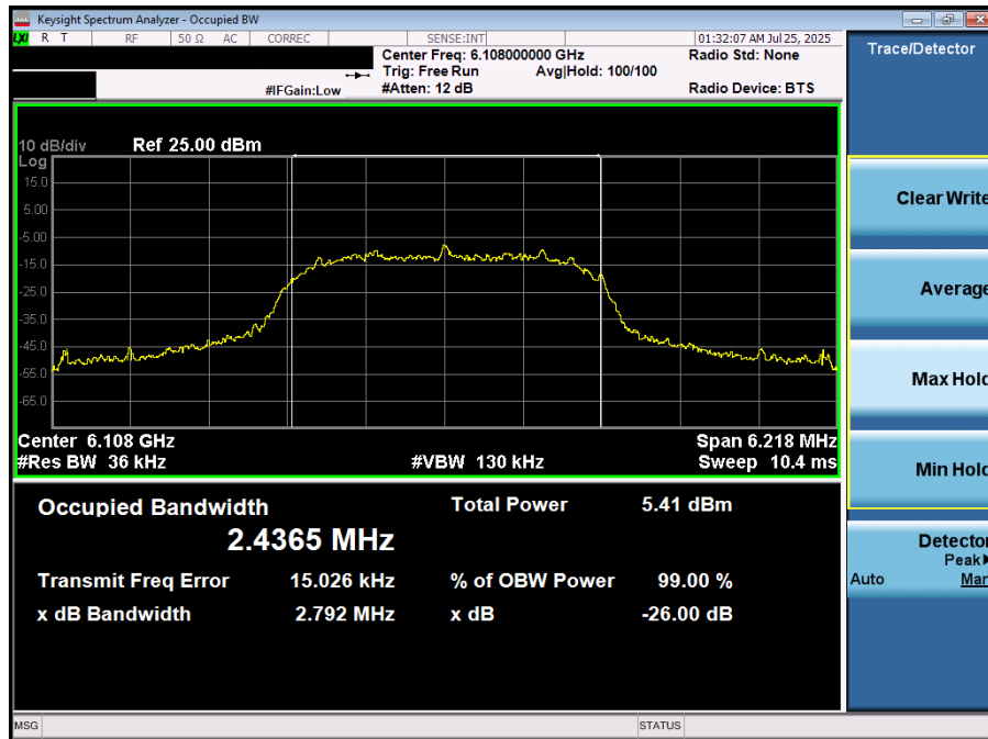
Plot 7-16. 26dB BW & 99% OBW (NB UNII HDRp4 – 6108MHz)
