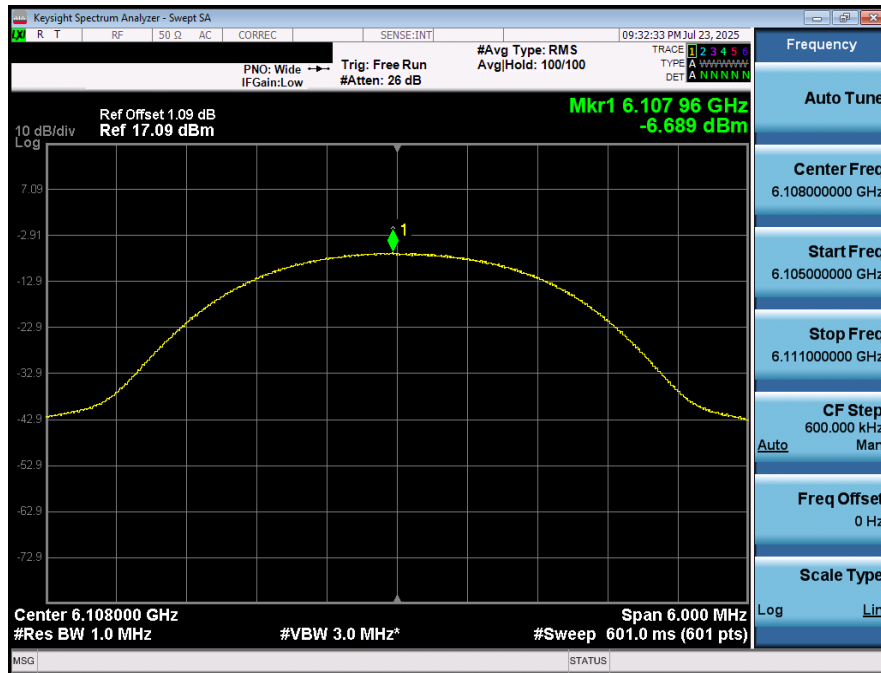
Plot 7-31. PSD (NB UNII HDR4 – 6108MHz)
