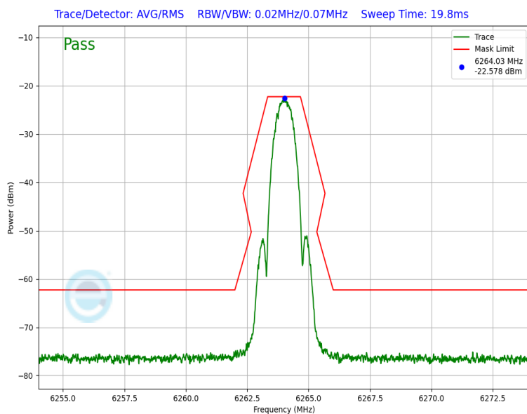
Plot 7-47. In Band Emission Plot (NB UNII LE1M – 6264MHz)
