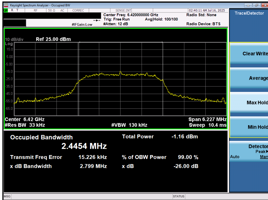
Plot 7-18. 26dB BW & 99% OBW (NB UNII HDRp4 – 6420MHz)
