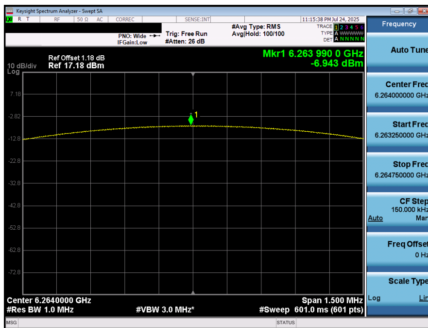
Plot 7-23. PSD (NB UNII BDR – 6264MHz)
