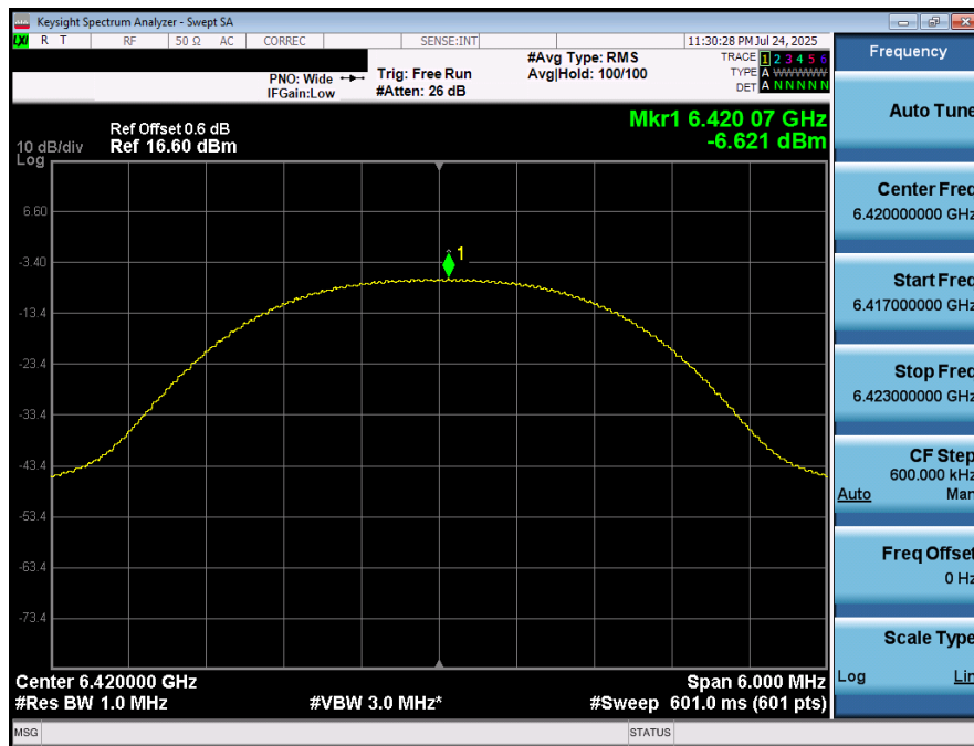
Plot 7-39. PSD (NB UNII HDRp4 - 6420MHz)
