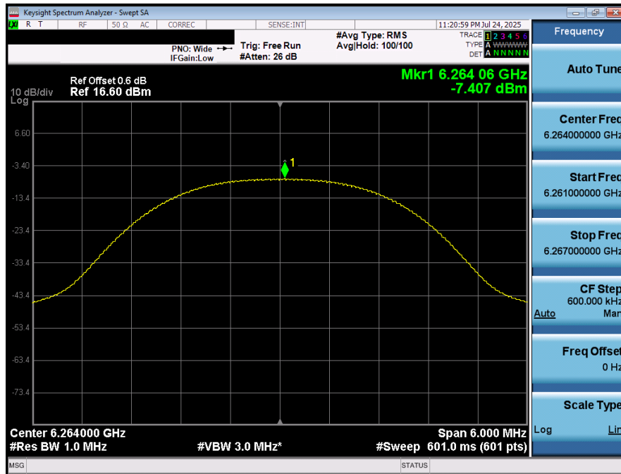
Plot 7-38. PSD (NB UNII HDRp4 - 6264MHz)
