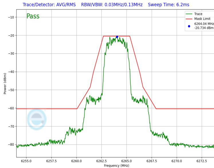
Plot 7-53. In Band Emission Plot (NB UNII HDR4 – 6264MHz)
