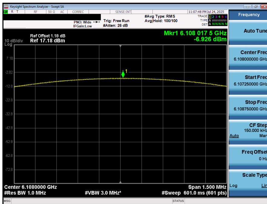
Plot 7-22. PSD (NB UNII BDR – 6108MHz)
