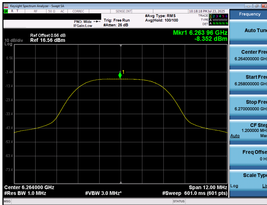
Plot 7-41. PSD (NB UNII HDRp8 – 6264MHz)
