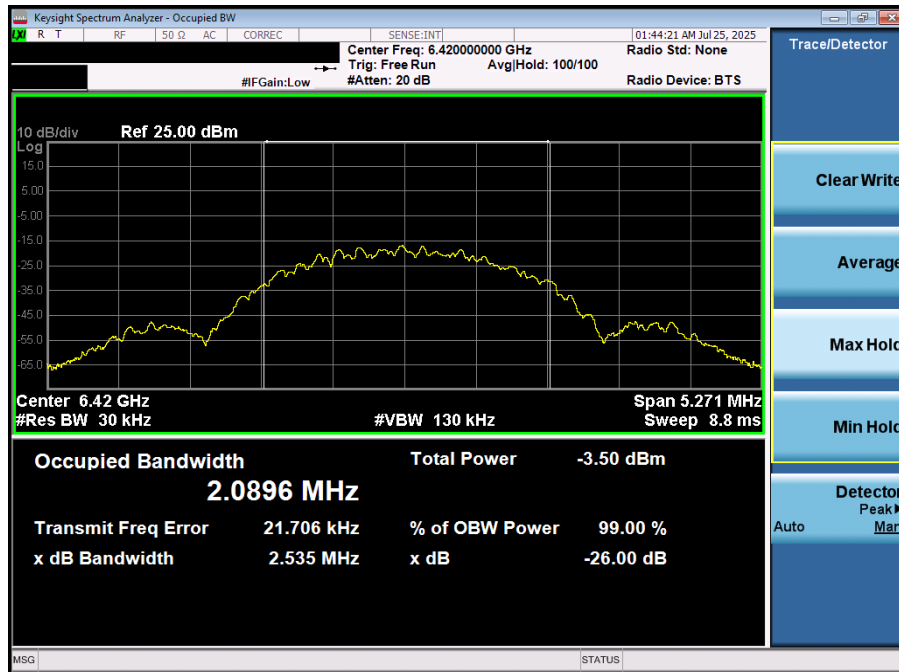
Plot 7-9. 26dB BW & 99% OBW (NB UNII LE2M – 6420MHz)
