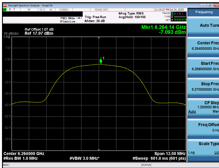
Plot 7-35. PSD (NB UNII HDR8 – 6264MHz)
