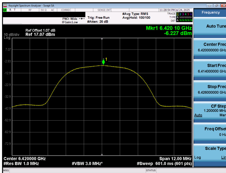
Plot 7-36. PSD (NB UNII HDR8 - 6420MHz)
