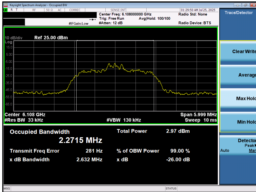
Plot 7-10. 26dB BW & 99% OBW (NB UNII HDR4 – 6108MHz)
