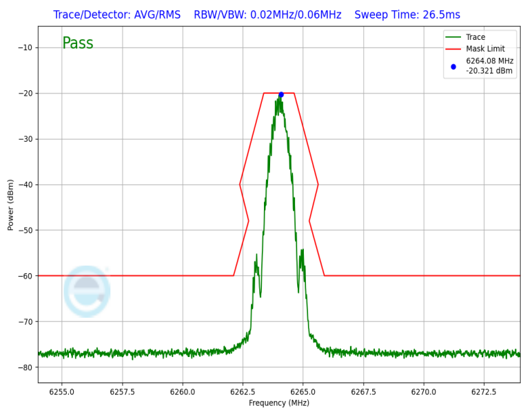
Plot 7-44. In Band Emission Plot (NB UNII BDR – 6264MHz)
