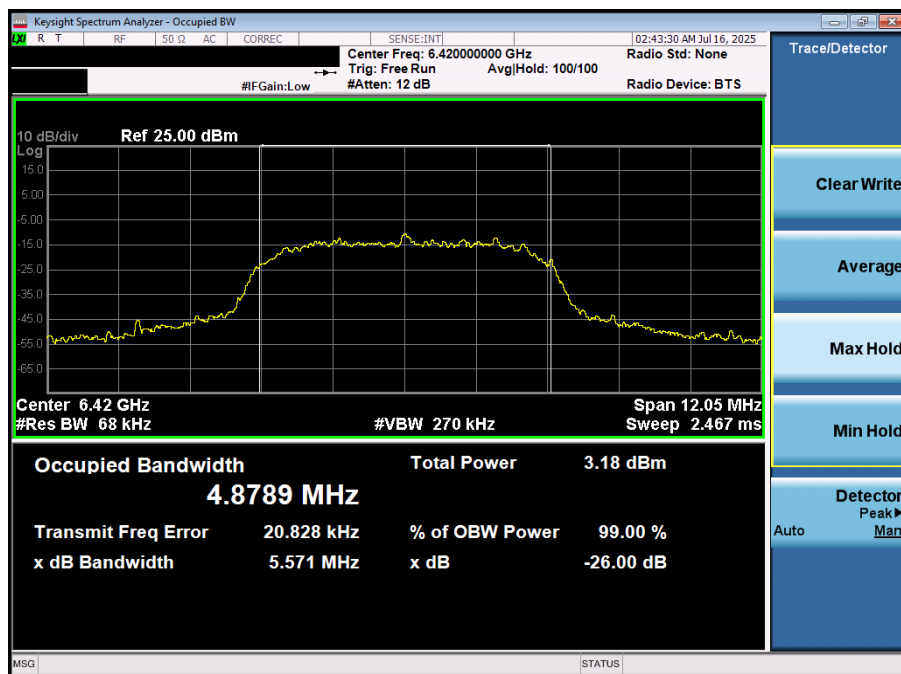
Plot 7-21. 26dB BW & 99% OBW (NB UNII HDRp8 – 6420MHz)
