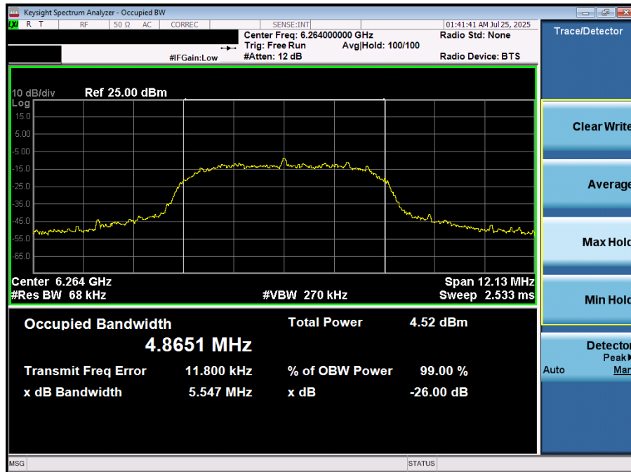
Plot 7-20. 26dB BW & 99% OBW (NB UNII HDRp8 – 6264MHz)
