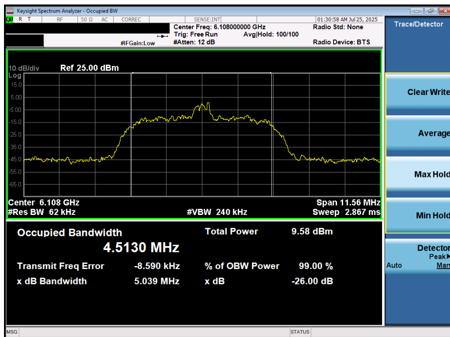
Plot 7-13. 26dB BW & 99% OBW (NB UNII HDR8 – 6108MHz)
