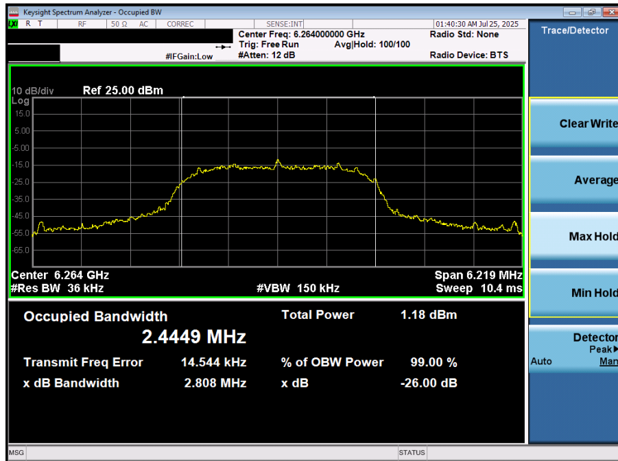
Plot 7-17. 26dB BW & 99% OBW (NB UNII HDRp4 – 6264MHz)
