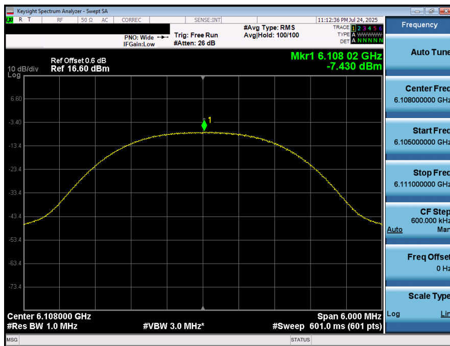
Plot 7-37. PSD (NB UNII HDRp4 - 6108MHz)
