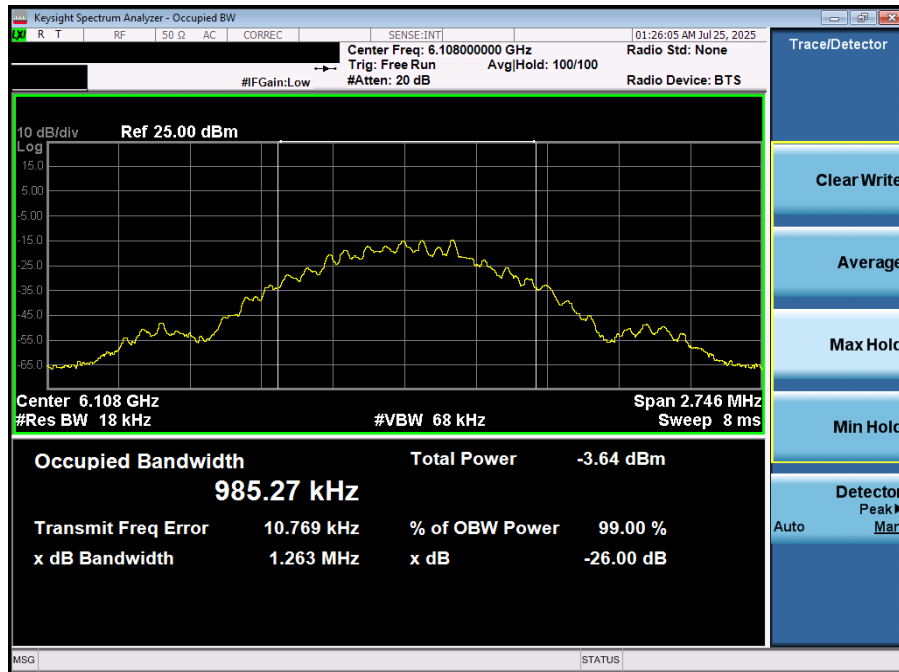
Plot 7-1. 26dB BW & 99% OBW (NB UNII BDR – 6108MHz)
