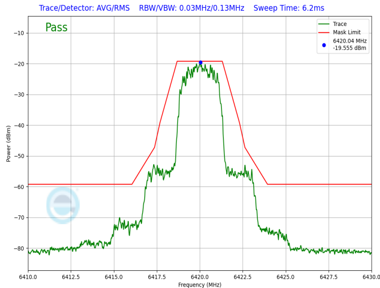
Plot 7-54. In Band Emission Plot (NB UNII HDR4 – 6420MHz)
