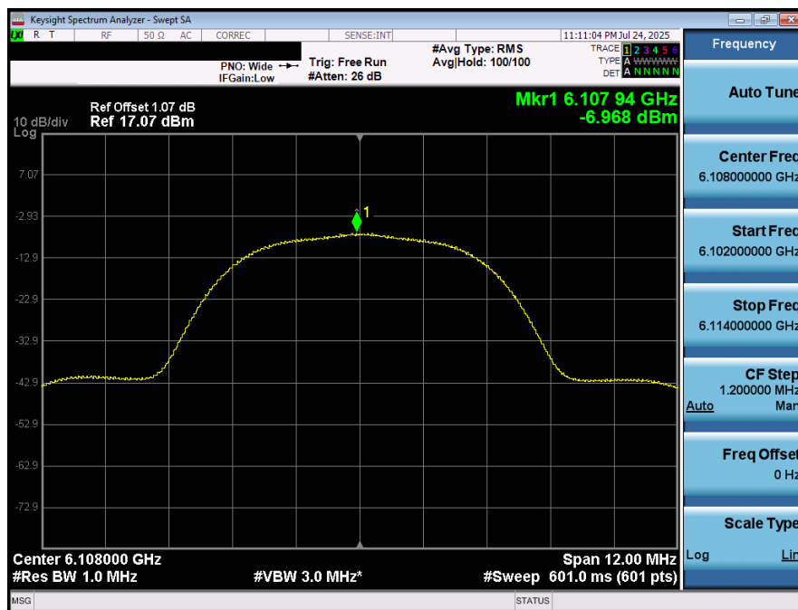
Plot 7-34. PSD (NB UNII HDR8 – 6108MHz)
