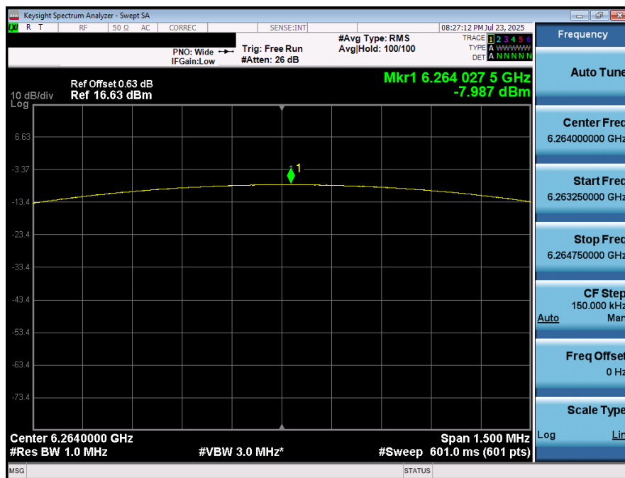
Plot 7-26. PSD (NB UNII LE1M – 6264MHz)
