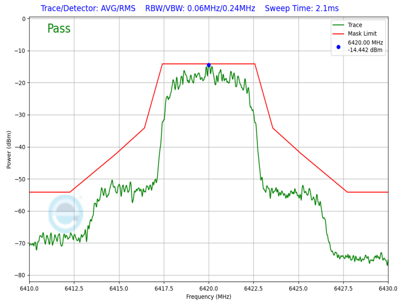
Plot 7-57. In Band Emission Plot (NB UNII HDR8 – 6420MHz)
