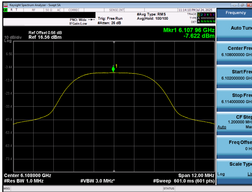
Plot 7-40. PSD (NB UNII HDRp8 – 6108MHz)
