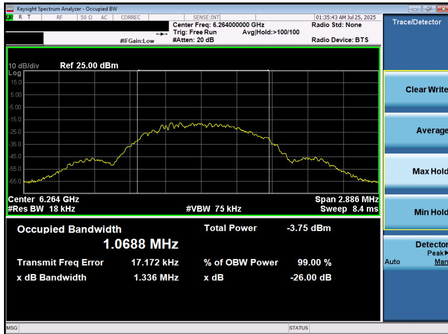
Plot 7-5. 26dB BW & 99% OBW (NB UNII LE1M – 6264MHz)
