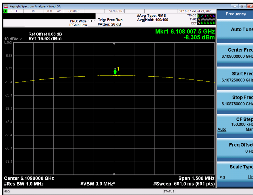
Plot 7-25. PSD (NB UNII LE1M – 6108MHz)
