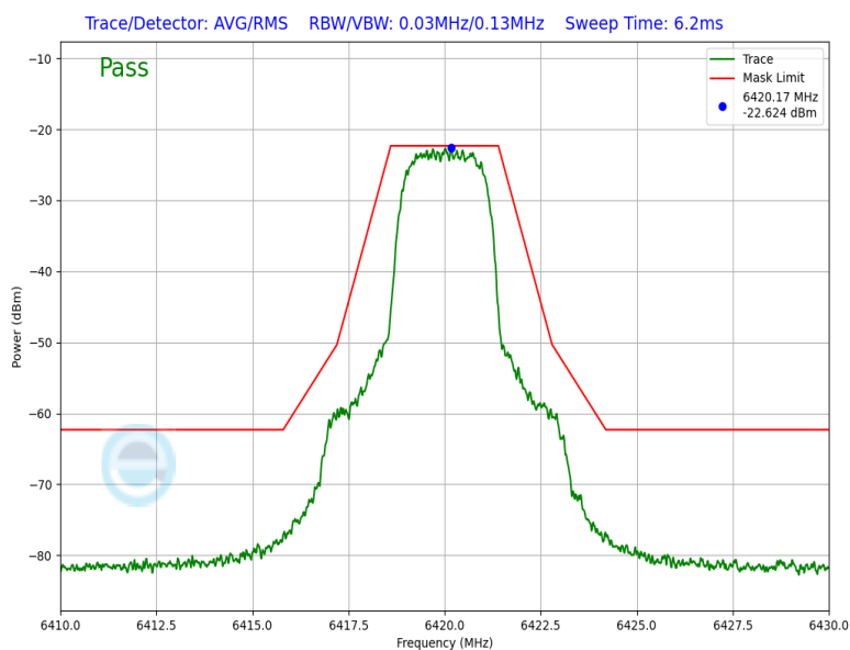
Plot 7-60. In Band Emission Plot (NB UNII HDRp4 – 6420MHz)
