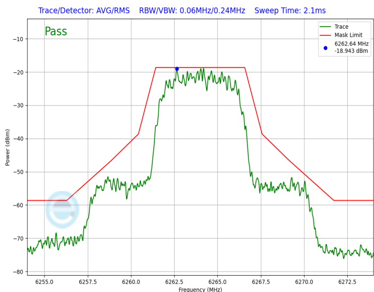
Plot 7-56. In Band Emission Plot (NB UNII HDR8 – 6264MHz)
