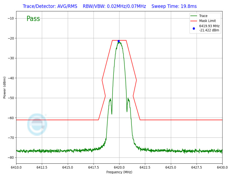
Plot 7-48. In Band Emission Plot (NB UNII LE1M – 6420MHz)
