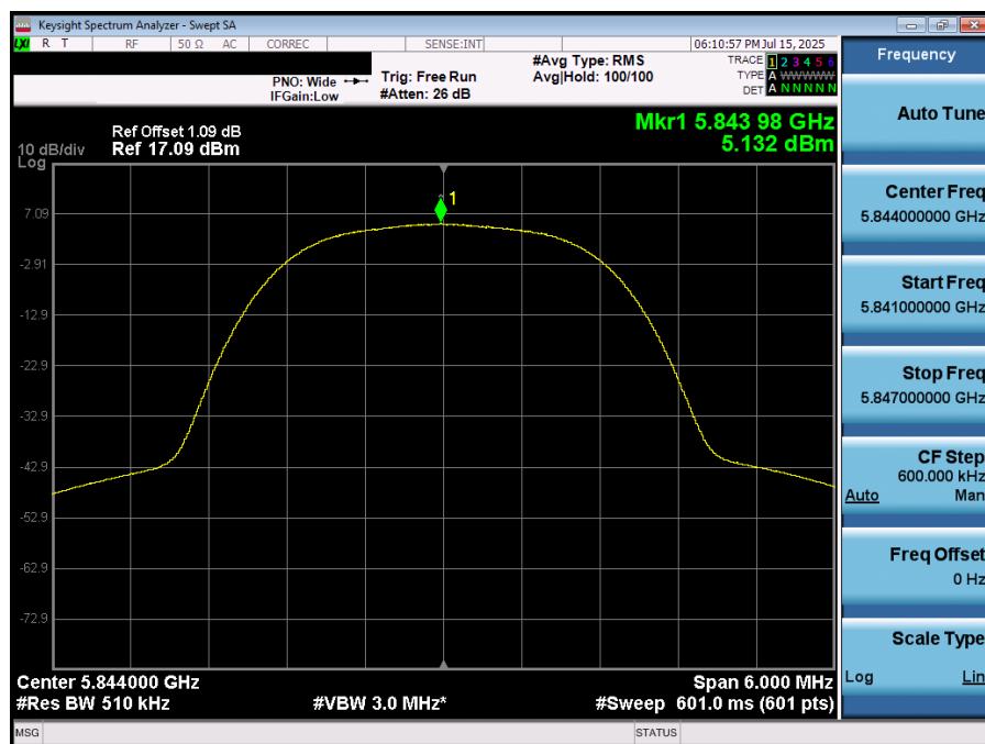
Plot 7-75. PSD (NB UNII HDR4 – 5844MHz)
