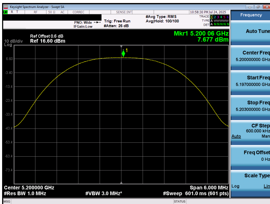
Plot 7-59. PSD (NB UNII HDRp4 – 5200MHz)
