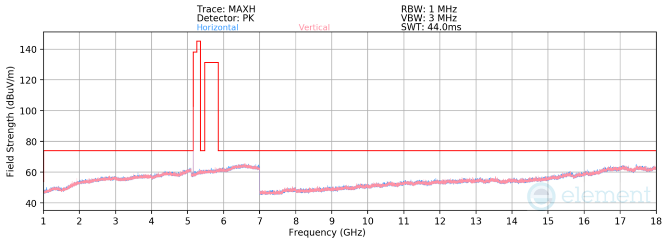
Plot 7-93. Radiated Spurious Emissions 1-18GHz (NB UNII LE1M – 5157MHz)
