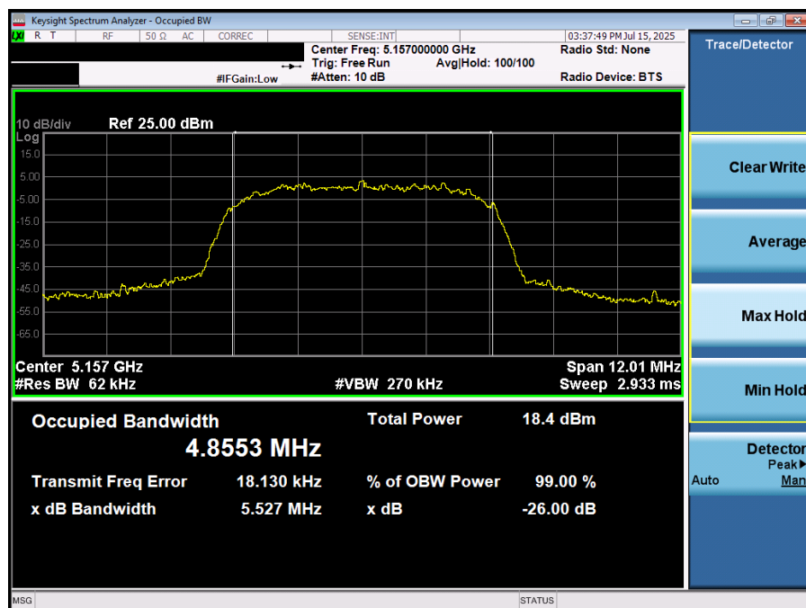
Plot 7-19. 26dB BW & 99% OBW (NB UNII HDRp8– 5157MHz)
