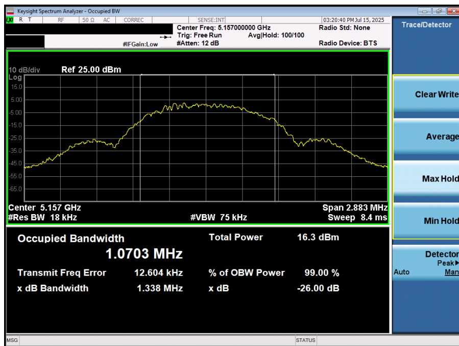
Plot 7-4. 26dB BW & 99% OBW (NB UNII LE1M - 5157MHz)
