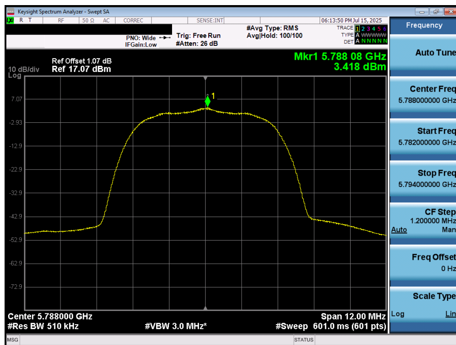
Plot 7-77. PSD (NB UNII HDR8 – 5788MHz)
