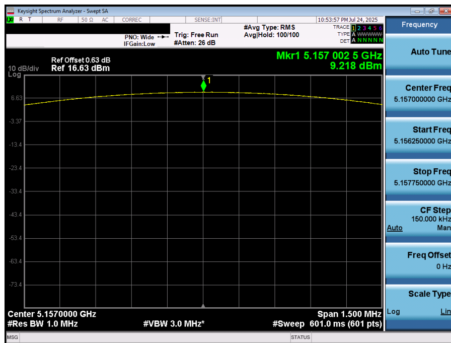
Plot 7-46. PSD (NB UNII LE1M – 5157MHz)
