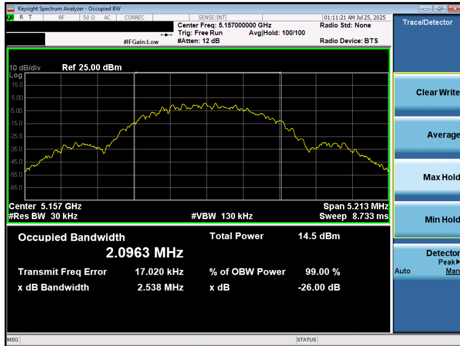
Plot 7-7. 26dB BW & 99% OBW (NB UNII LE2M – 5157MHz)
