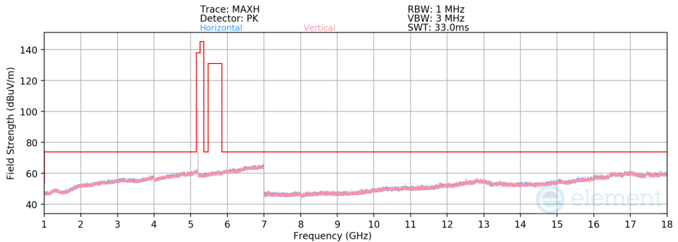
Plot 7-86. Radiated Spurious Emissions 1-18GHz (BDR GFSK – 5200MHz)
