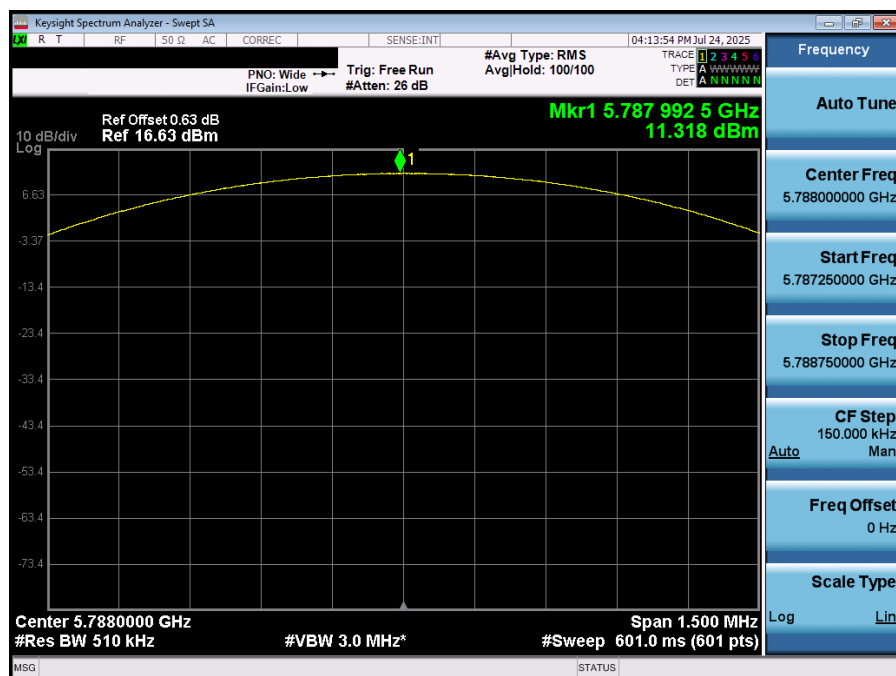
Plot 7-68. PSD (NB UNII LE1M – 5788MHz)
