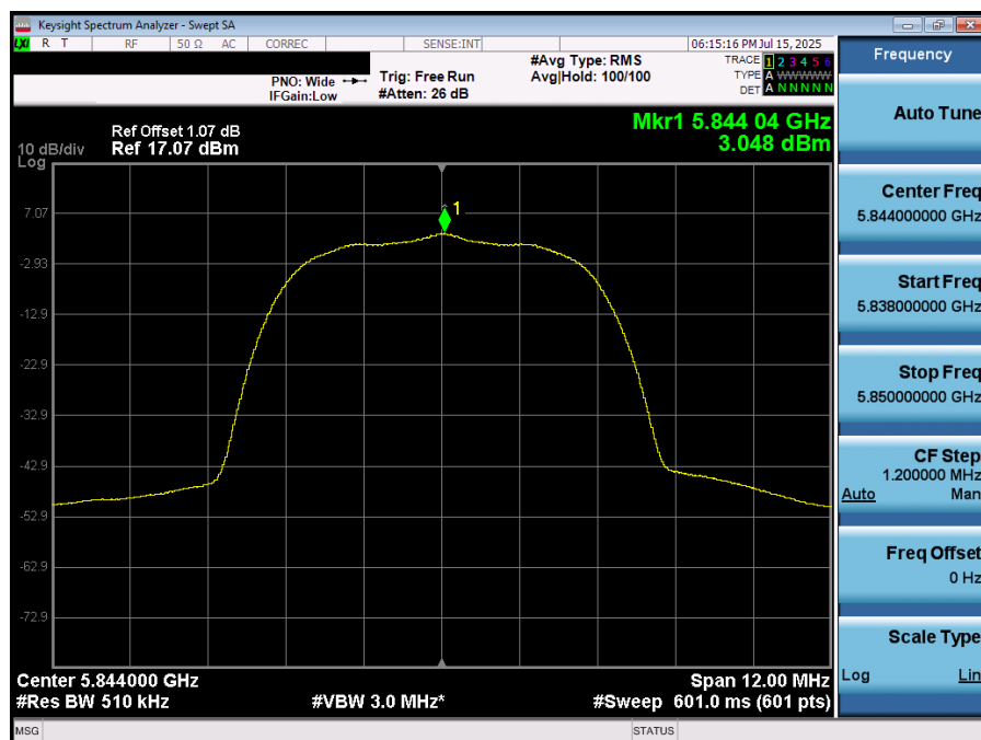
Plot 7-78. PSD (NB UNII HDR8 – 5844MHz)
