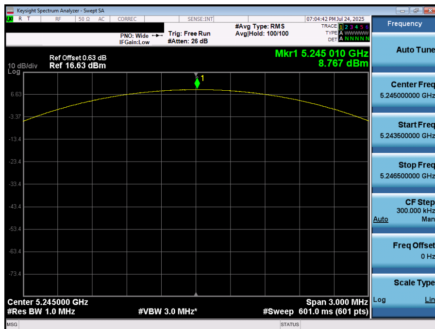
Plot 7-51. PSD (NB UNII LE2M – 5245MHz)
