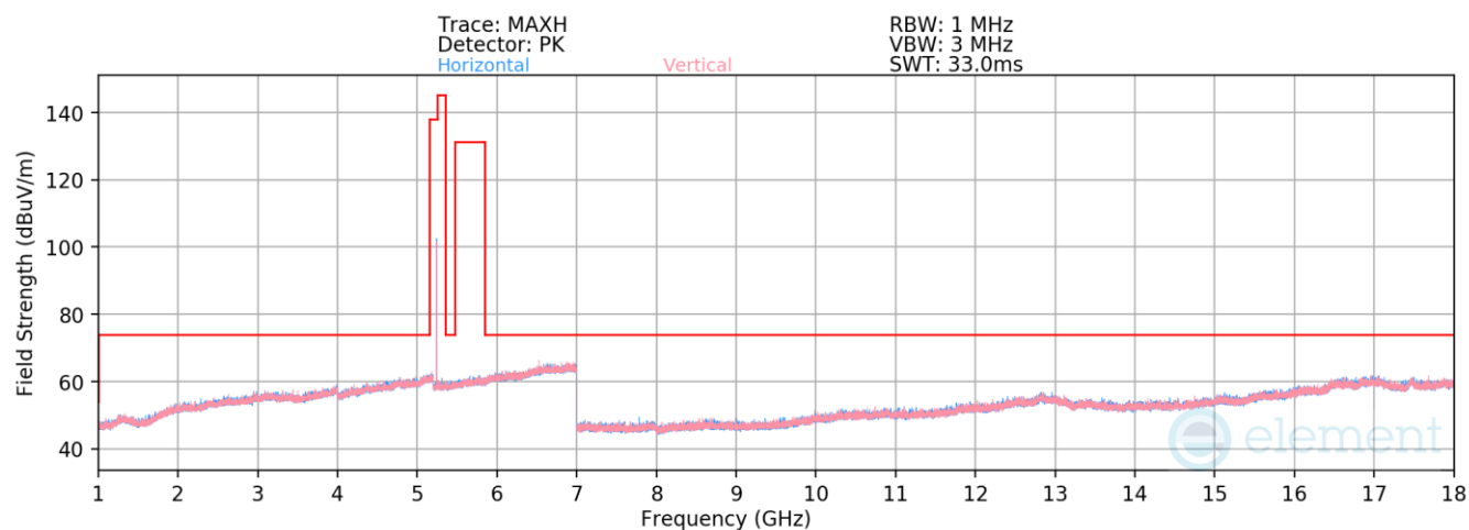
Plot 7-87. Radiated Spurious Emissions 1-18GHz (BDR GFSK – 5245MHz)
