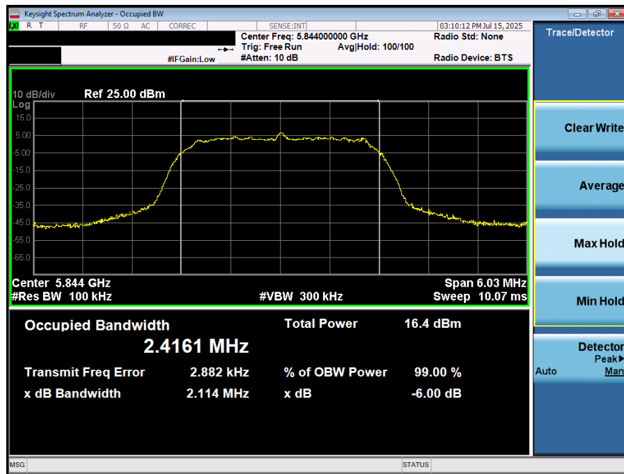
Plot 7-39. 6dB BW & 99% OBW (NB UNII HDRp4 – 5844MHz)
