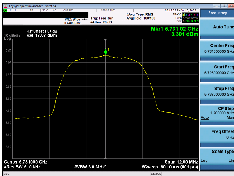
Plot 7-76. PSD (NB UNII HDR8 – 5731MHz)
