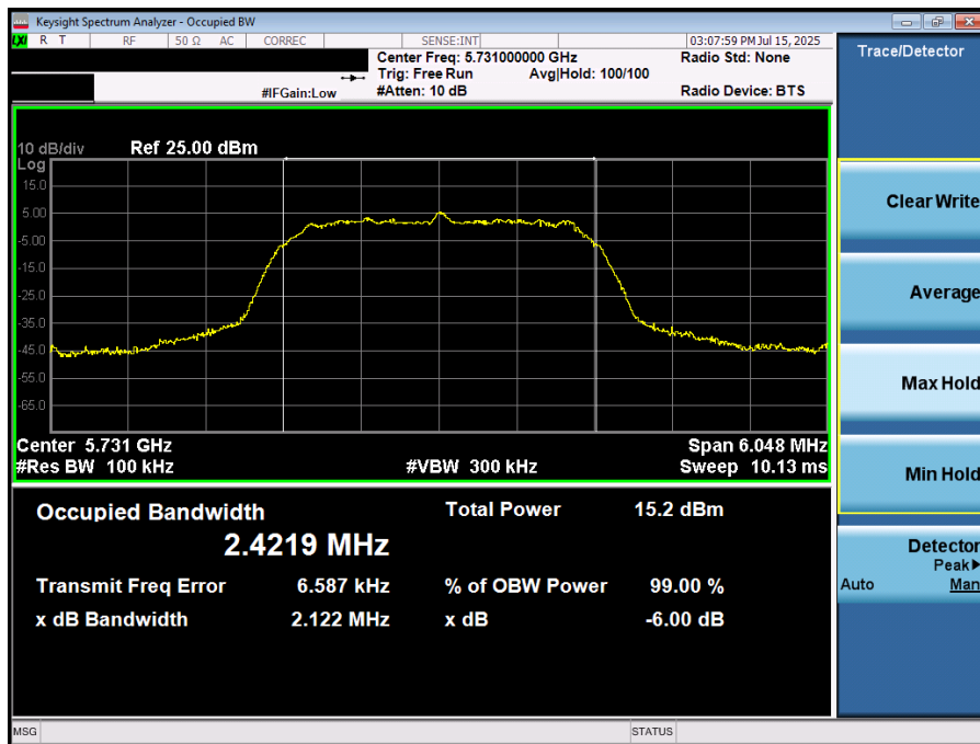
Plot 7-37. 6dB BW & 99% OBW (NB UNII HDRp4 – 5731MHz)
