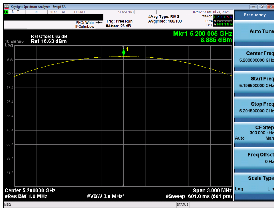
Plot 7-50. PSD (NB UNII LE2M - 5200MHz)
