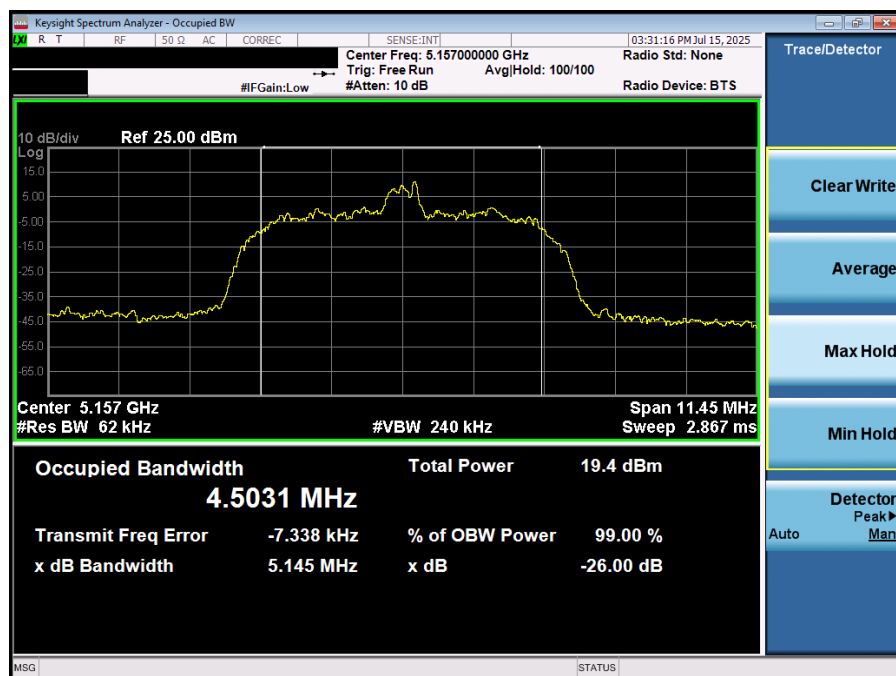
Plot 7-13. 26dB BW & 99% OBW (NB UNII HDR8- 5157MHz)
