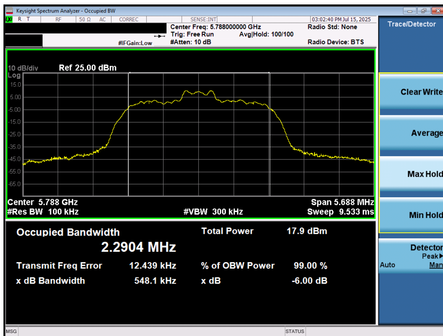
Plot 7-32. 6dB BW & 99% OBW (NB UNII HDR4 – 5788MHz)
