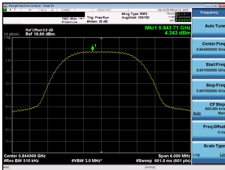
Plot 7-81. PSD (NB UNII HDRp4 – 5844MHz)
