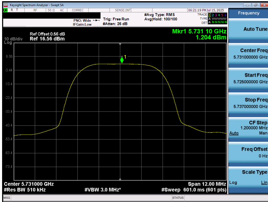
Plot 7-82. PSD (NB UNII HDRp8 – 5731MHz)
