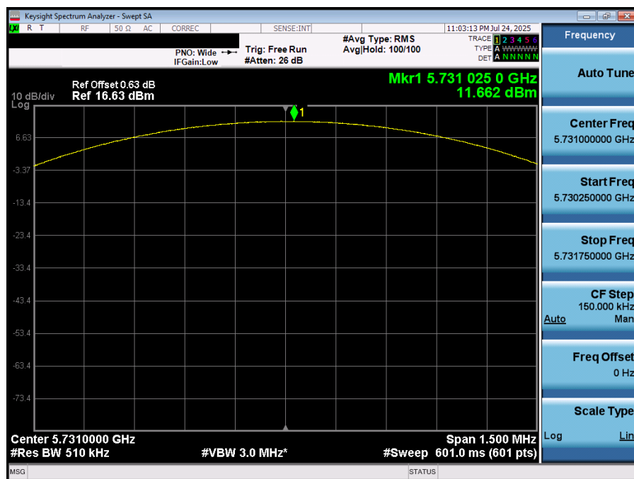
Plot 7-67. PSD (NB UNII LE1M – 5731MHz)
