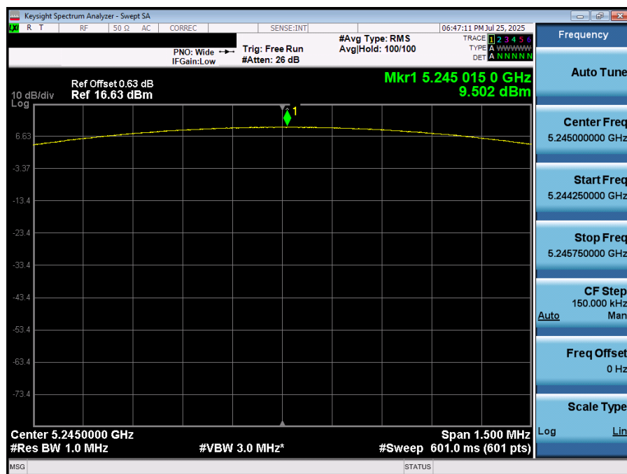
Plot 7-48. PSD (NB UNII LE1M – 5245MHz)
