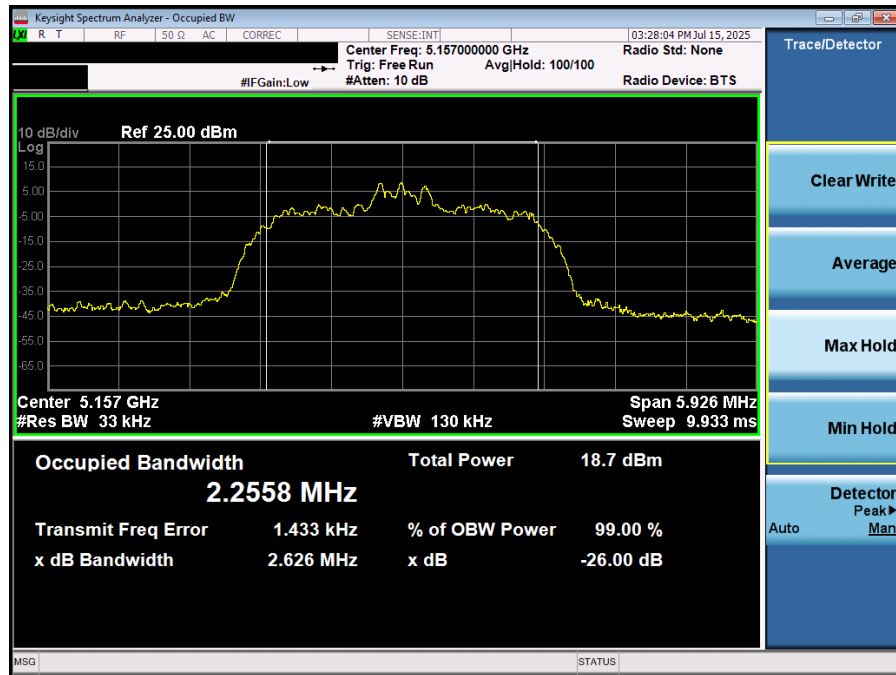
Plot 7-10. 26dB BW & 99% OBW (NB UNII HDR4– 5157MHz)
