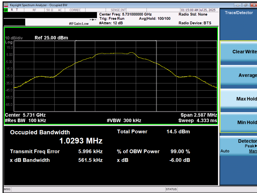
Plot 7-22. 6dB BW & 99% OBW (NB UNII BDR – 5731MHz)
