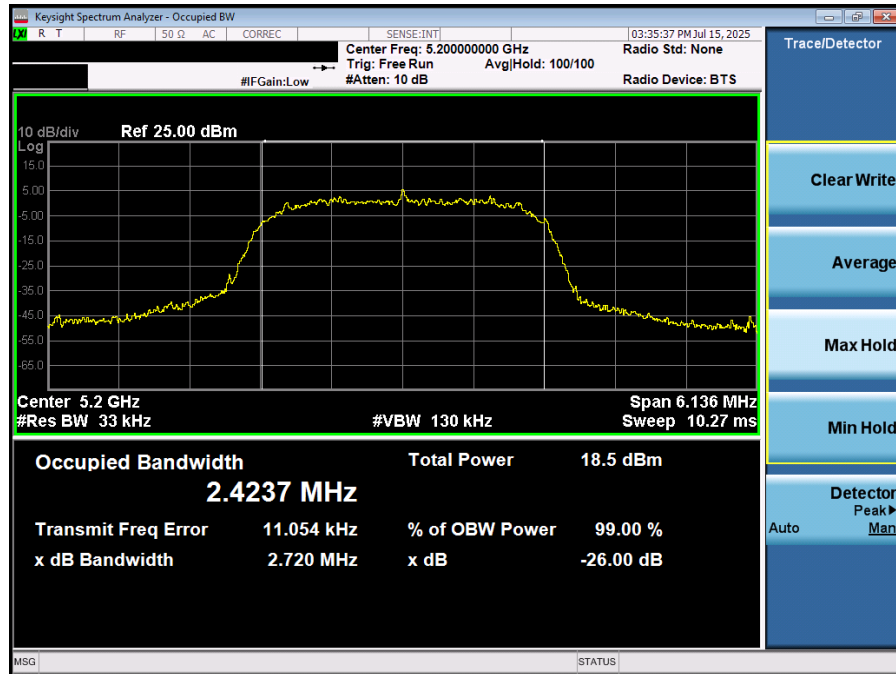
Plot 7-17. 26dB BW & 99% OBW (NB UNII HDRp4– 5200MHz)
