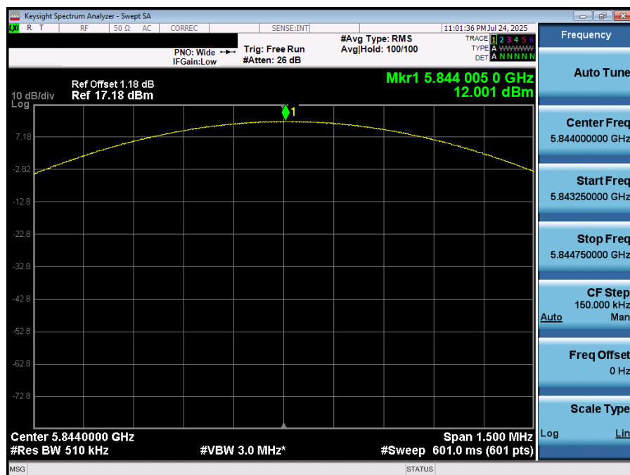
Plot 7-66. PSD (NB UNII BDR – 5844MHz)
