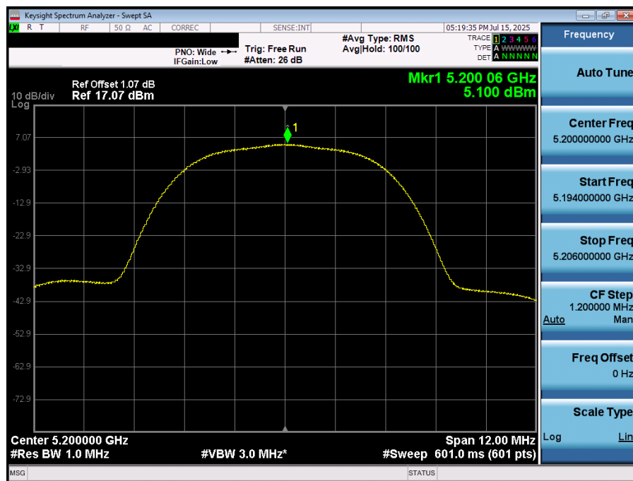
Plot 7-56. PSD (NB UNII HDR8 – 5200MHz)
