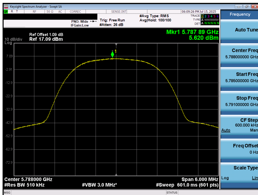
Plot 7-74. PSD (NB UNII HDR4 – 5788MHz)
