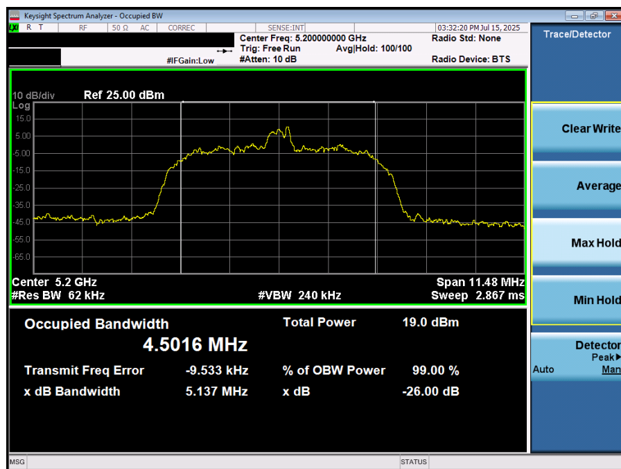
Plot 7-14. 26dB BW & 99% OBW (NB UNII HDR8- 5200MHz)
