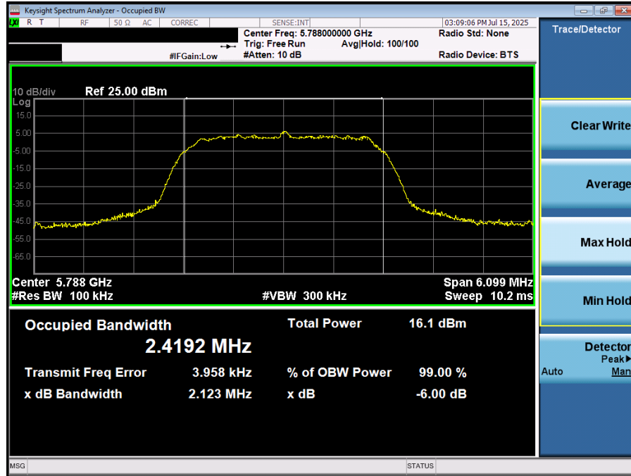
Plot 7-38. 6dB BW & 99% OBW (NB UNII HDRp4 – 5788MHz)
