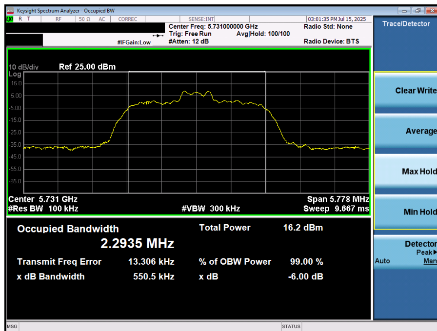
Plot 7-31. 6dB BW & 99% OBW (NB UNII HDR4 – 5731MHz)
