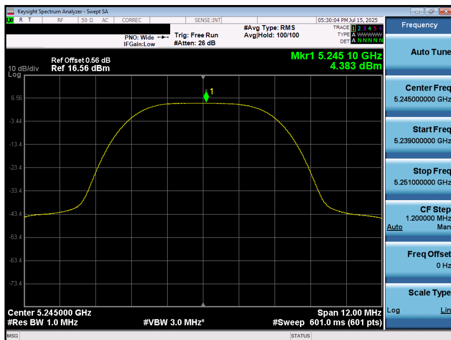
Plot 7-63. PSD (NB UNII HDRp8 – 5245MHz)
