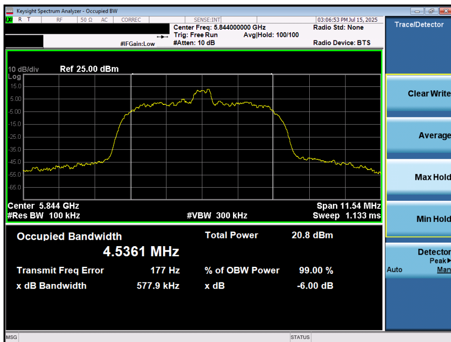
Plot 7-36. 6dB BW & 99% OBW (NB UNII HDR8 – 5844MHz)
