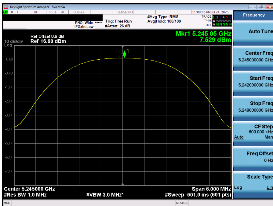
Plot 7-60. PSD (NB UNII HDRp4 – 5245MHz)
