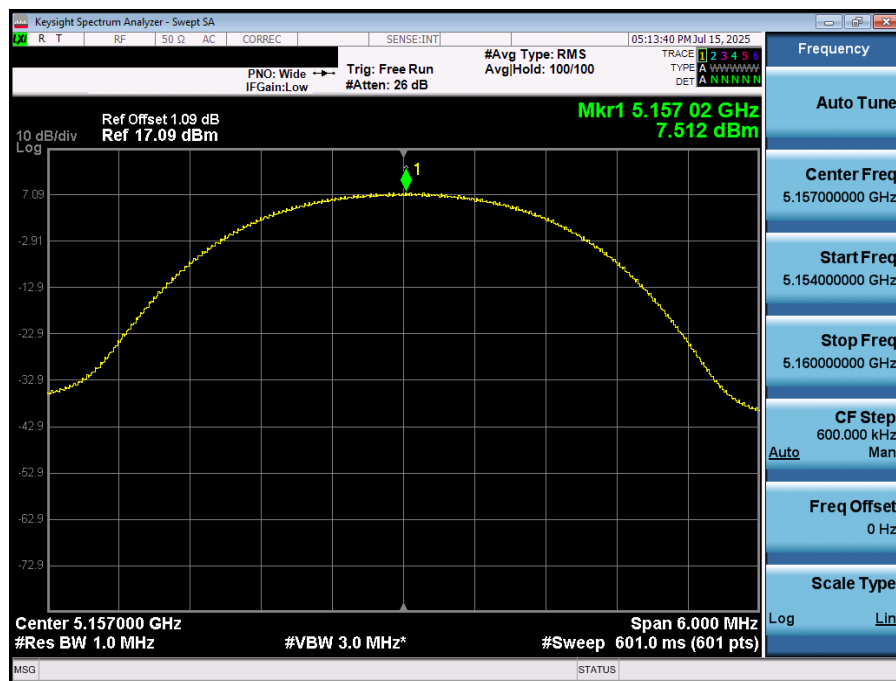
Plot 7-52. PSD (NB UNII HDR4 – 5157MHz)
