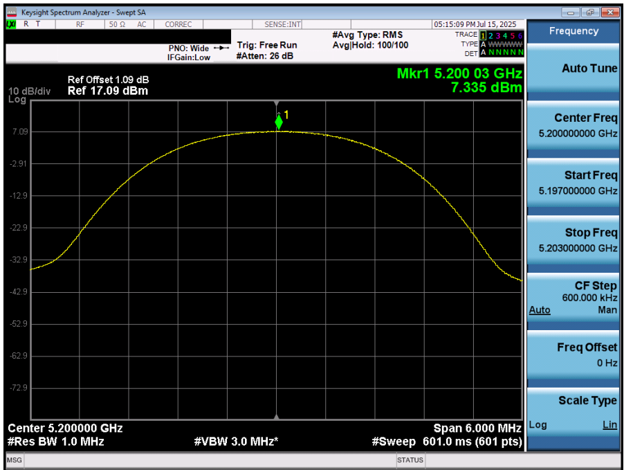
Plot 7-53. PSD (NB UNII HDR4 – 5200MHz)
