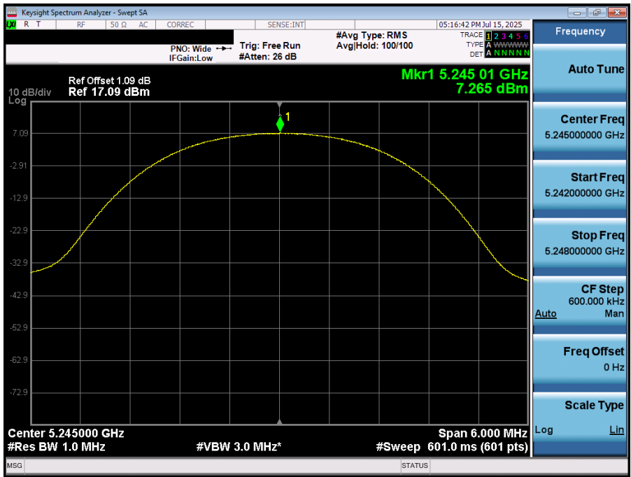
Plot 7-54. PSD (NB UNII HDR4 – 5245MHz)
