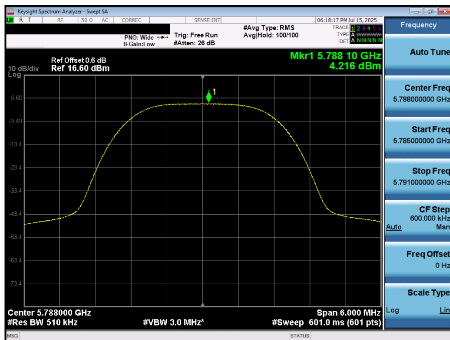
Plot 7-80. PSD (NB UNII HDRp4 – 5788MHz)
