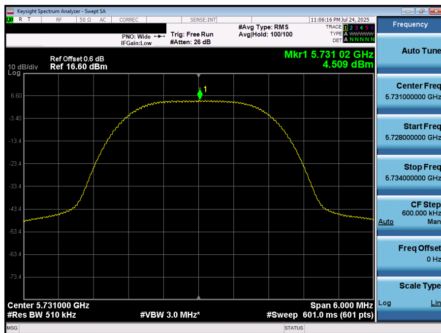
Plot 7-79. PSD (NB UNII HDRp4 – 5731MHz)
