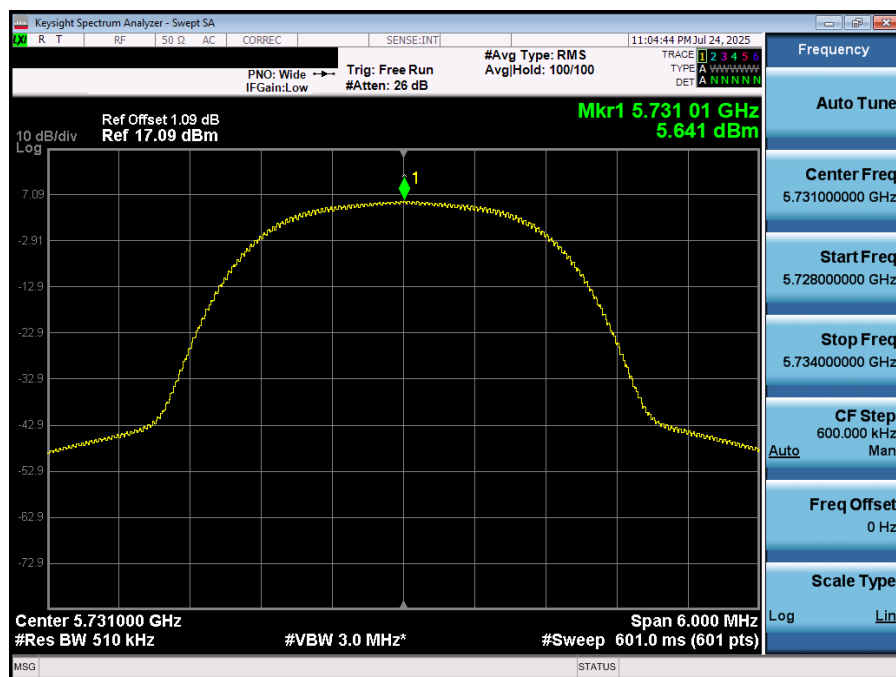
Plot 7-73. PSD (NB UNII HDR4 – 5731MHz)
