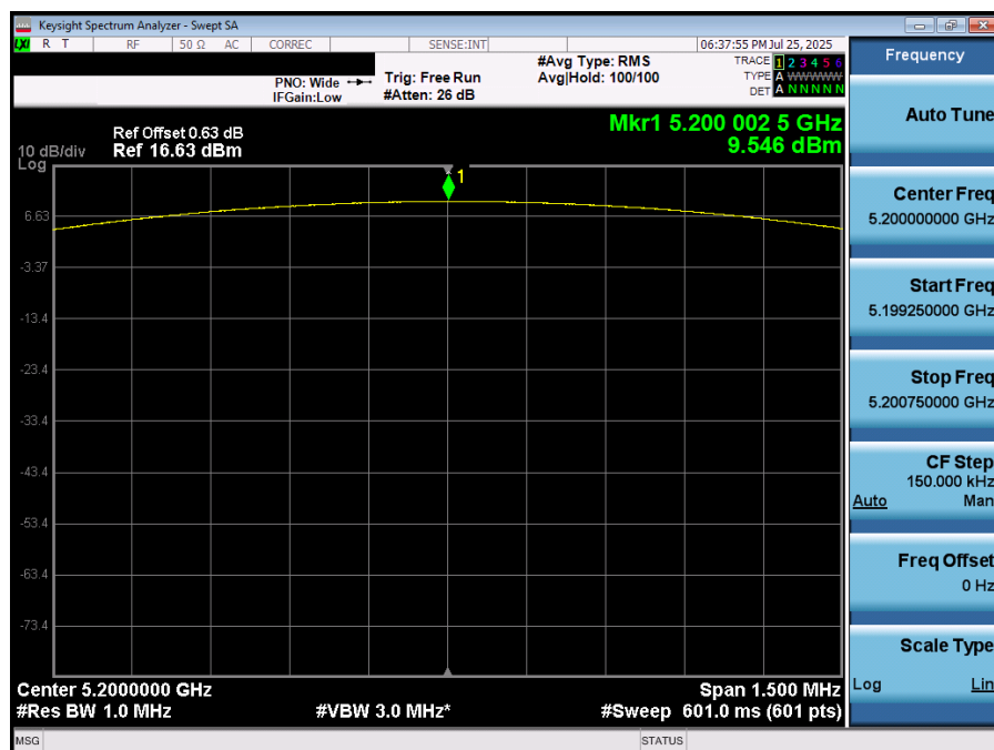
Plot 7-47. PSD (NB UNII LE1M – 5200MHz)
