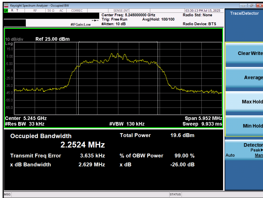
Plot 7-12. 26dB BW & 99% OBW (NB UNII HDR4– 5245MHz)
