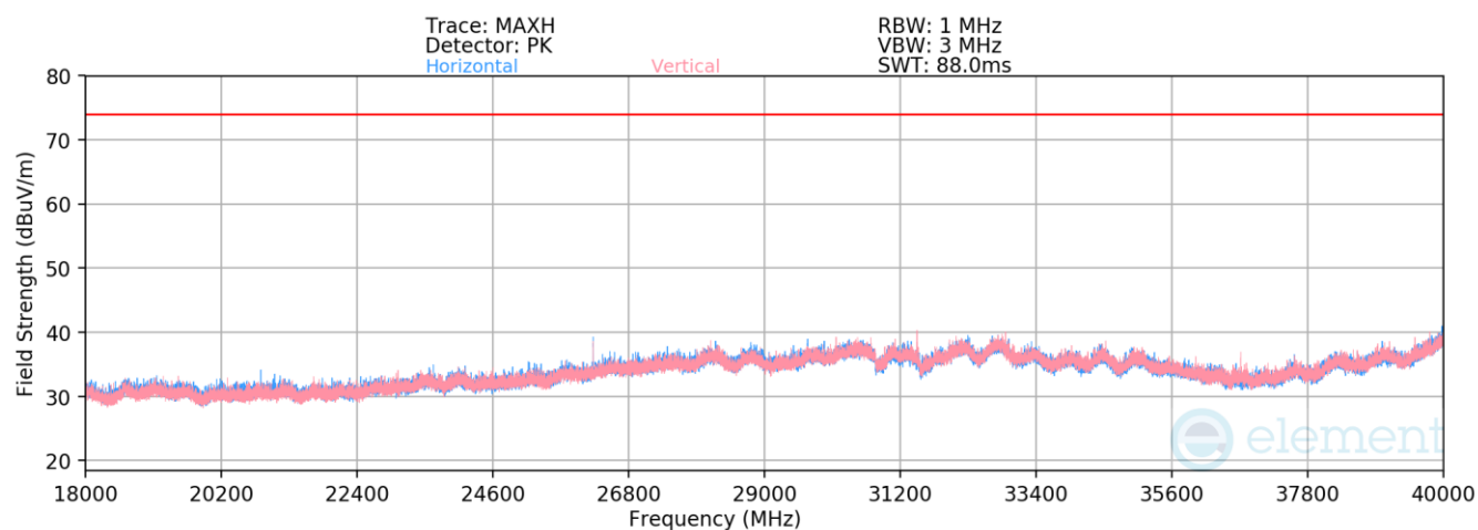
Plot 7-88. Radiated Spurious Emissions Above 18GHz (BDR GFSK – 5245MHz)
