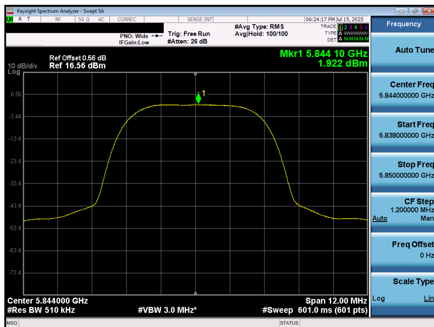
Plot 7-84. PSD (NB UNII HDRp8 – 5844MHz)
