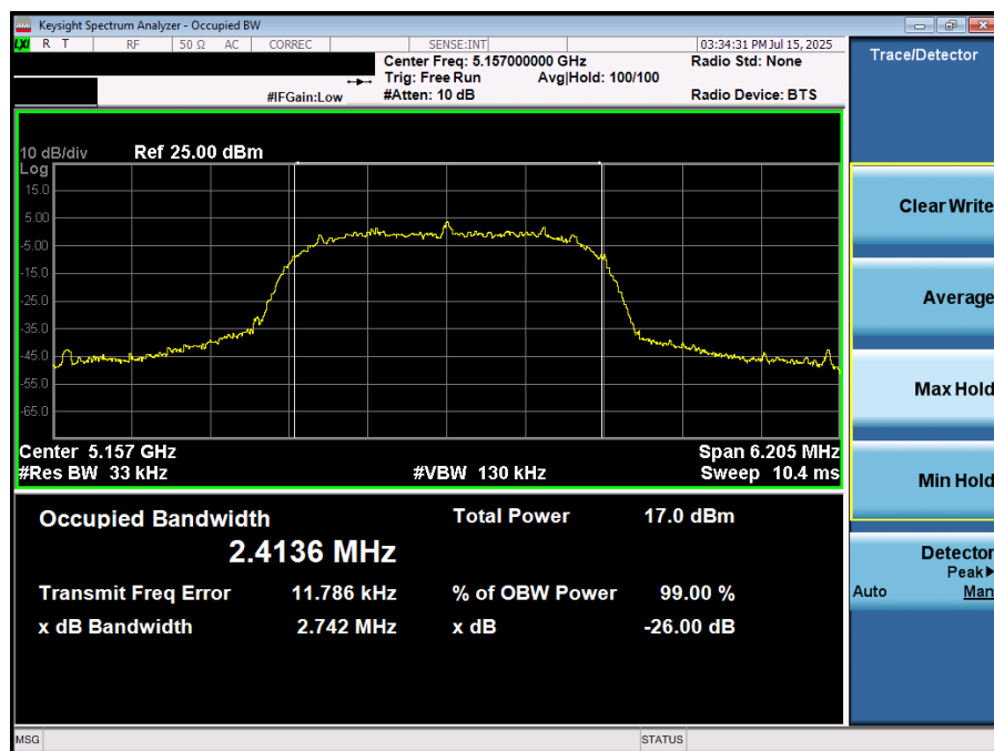
Plot 7-16. 26dB BW & 99% OBW (NB UNII HDRp4– 5157MHz)
