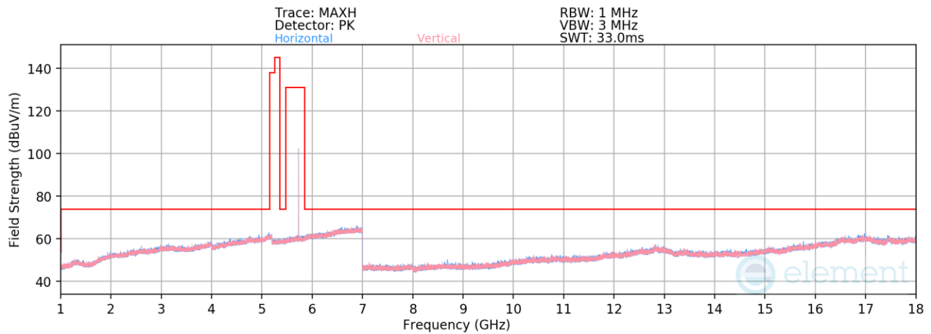
Plot 7-89. Radiated Spurious Emissions 1-18GHz (BDR GFSK – 5731MHz)
