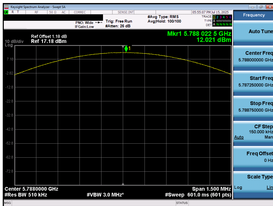
Plot 7-65. PSD (NB UNII BDR – 5788MHz)
