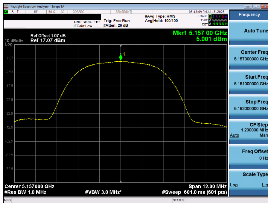
Plot 7-55. PSD (NB UNII HDR8 – 5157MHz)
