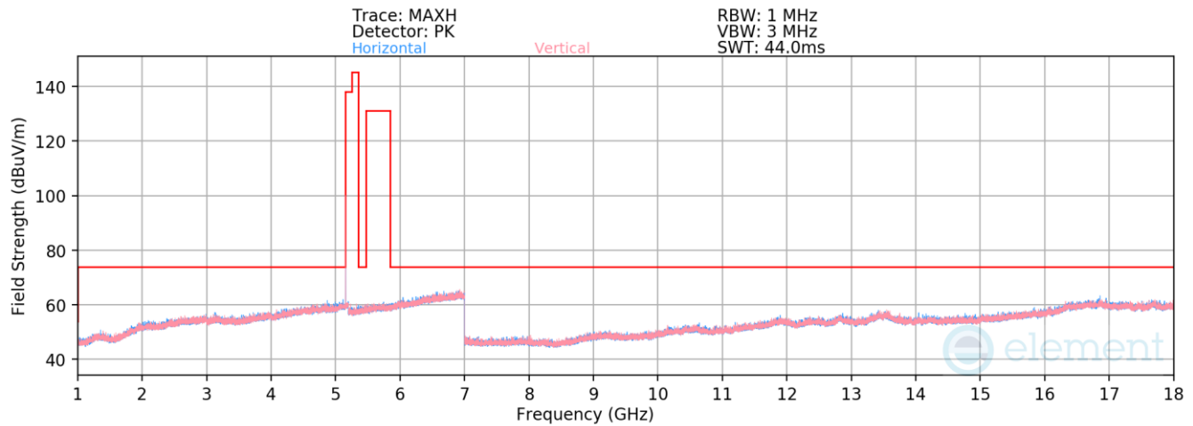
Plot 7-85. Radiated Spurious Emissions 1-18GHz (BDR GFSK – 5157MHz)
