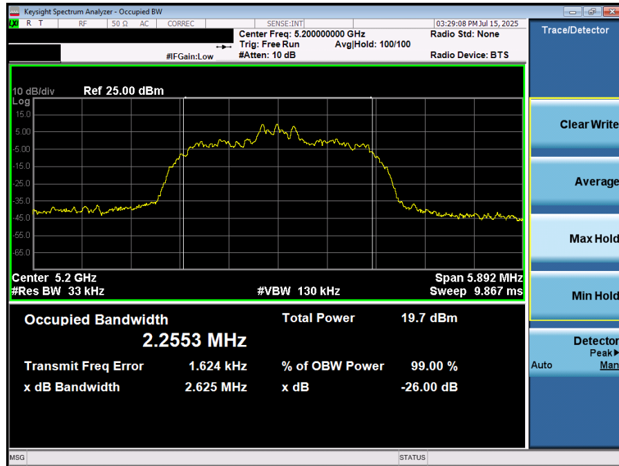
Plot 7-11. 26dB BW & 99% OBW (NB UNII HDR4– 5200MHz)
