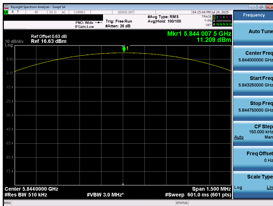
Plot 7-69. PSD (NB UNII LE1M – 5844MHz)
