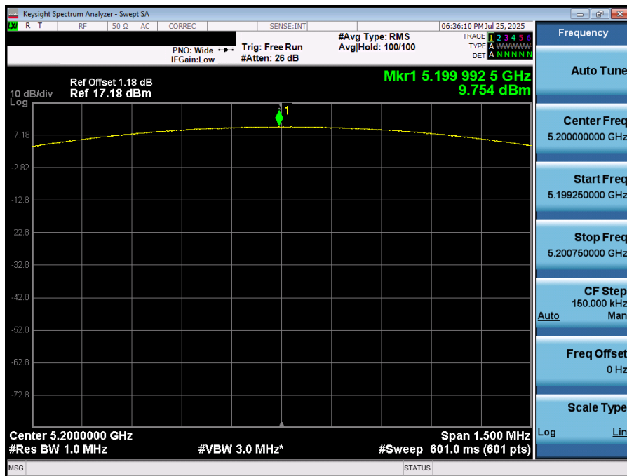
Plot 7-44. PSD (NB UNII BDR – 5200MHz)
