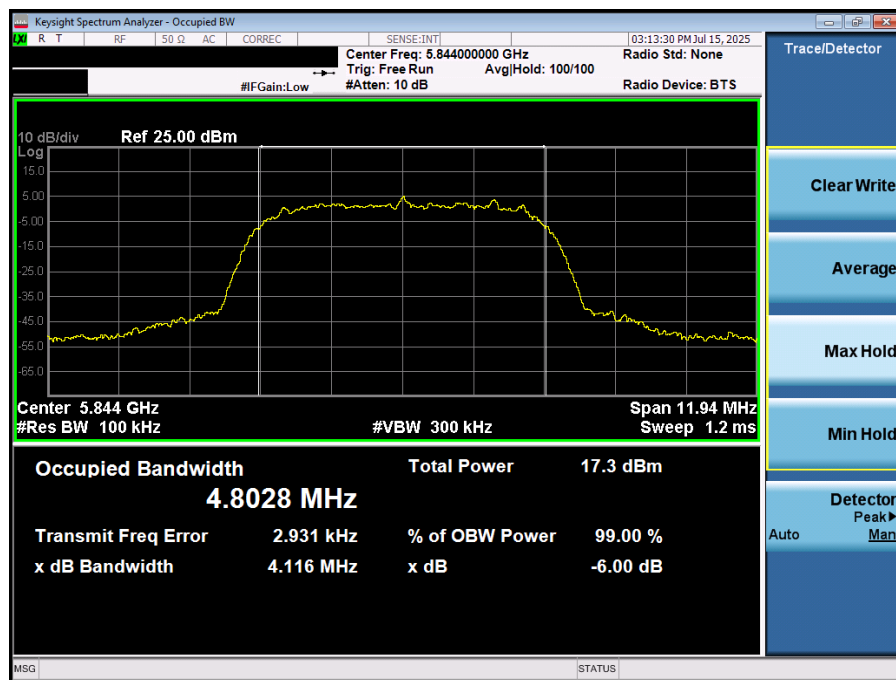
Plot 7-42. 6dB BW & 99% OBW (NB UNII HDRp8 – 5844MHz)
