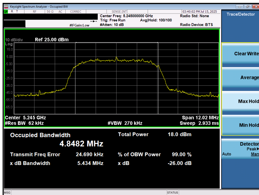
Plot 7-21. 26dB BW & 99% OBW (NB UNII HDRp8- 5245MHz)
