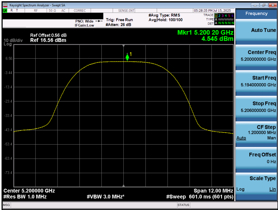
Plot 7-62. PSD (NB UNII HDRp8 – 5200MHz)
