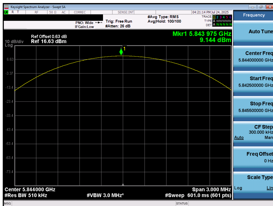
Plot 7-72. PSD (NB UNII LE2M – 5844MHz)
