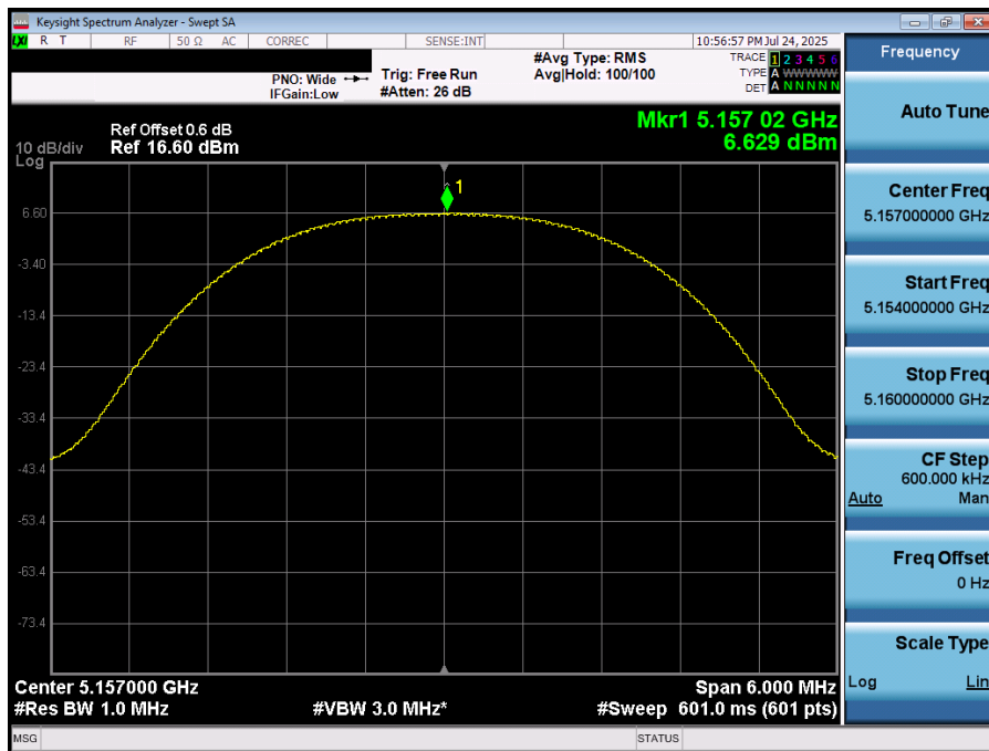
Plot 7-58. PSD (NB UNII HDRp4 – 5157MHz)
