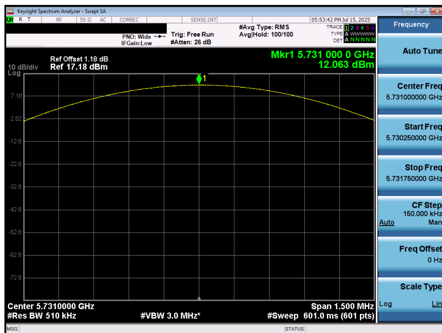
Plot 7-64. PSD (NB UNII BDR – 5731MHz)
