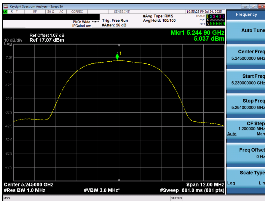
Plot 7-57. PSD (NB UNII HDR8 – 5245MHz)
