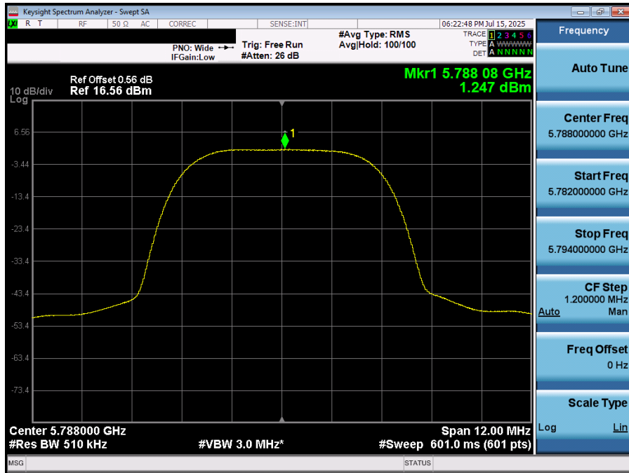
Plot 7-83. PSD (NB UNII HDRp8 – 5788MHz)
