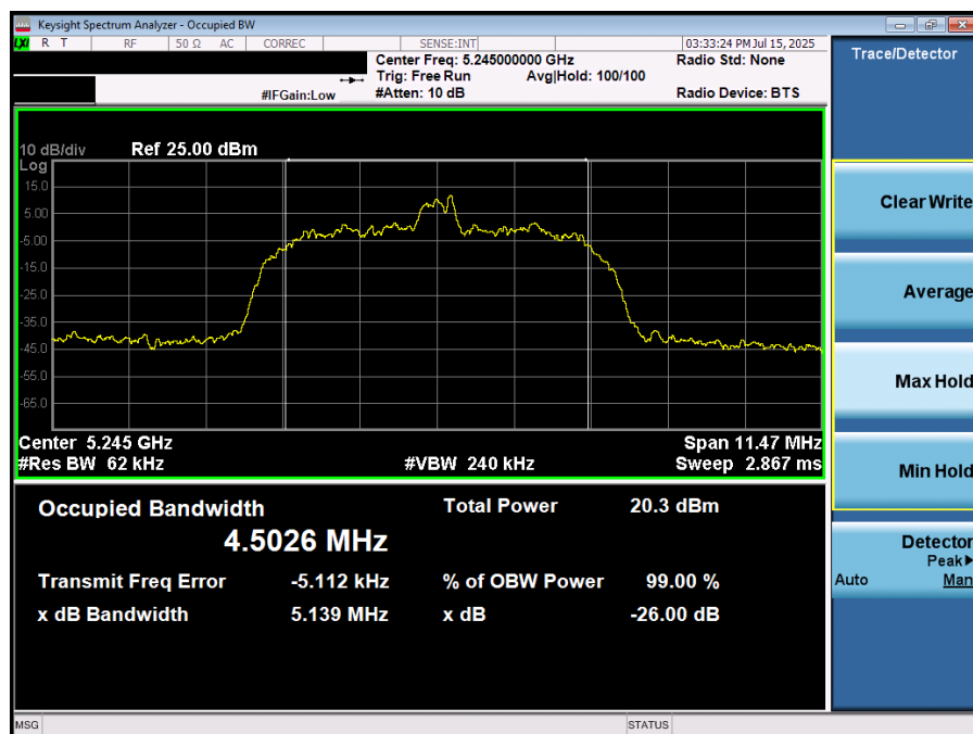
Plot 7-15. 26dB BW & 99% OBW (NB UNII HDR8– 5245MHz)
