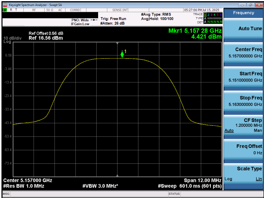
Plot 7-61. PSD (NB UNII HDRp8 – 5157MHz)
