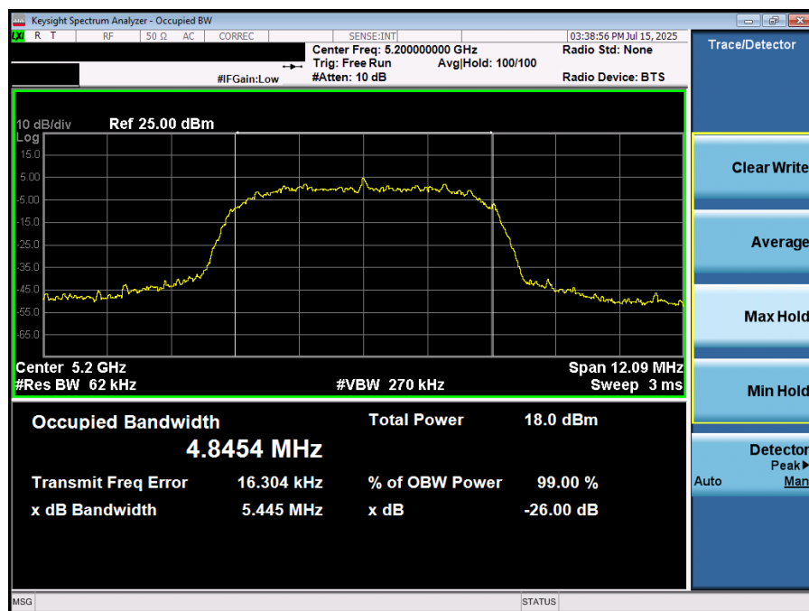
Plot 7-20. 26dB BW & 99% OBW (NB UNII HDRp8– 5200MHz)
