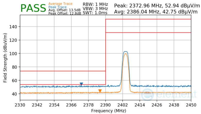
Plot 7-51. Radiated Restricted Lower Band Edge Measurement
