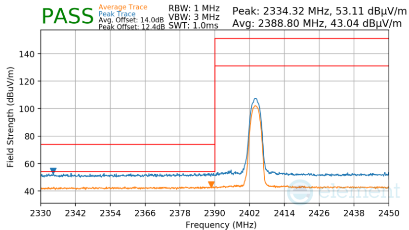
Plot 7-47. Radiated Restricted Lower Band Edge Measurement
