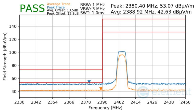
Plot 7-52. Radiated Restricted Lower Band Edge Measurement
