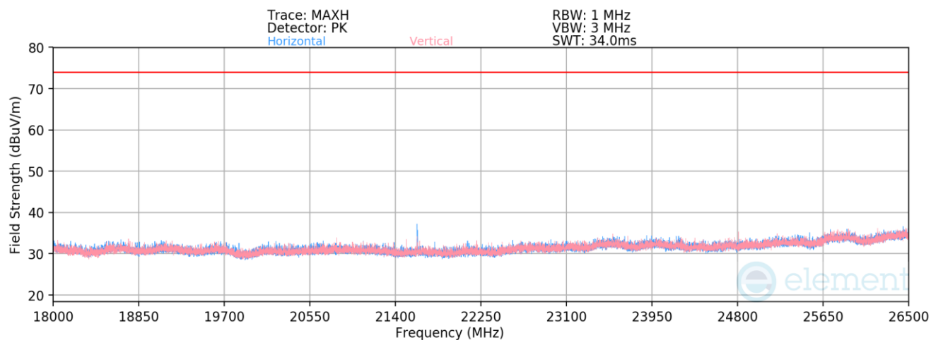
Plot 7-44. Radiated Spurious Emissions Above 18GHz (4Mbps, HDRp4 – Ch. 1)
