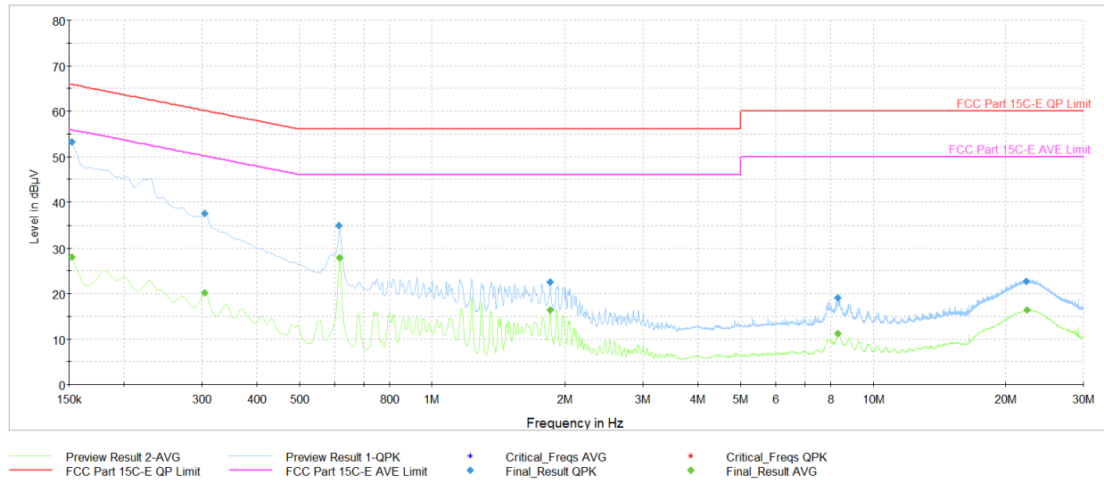
Plot 7-57. AC Line Conducted Plot with Bluetooth HDR (N, 4Mbps - Ch.38 with Laptop)
