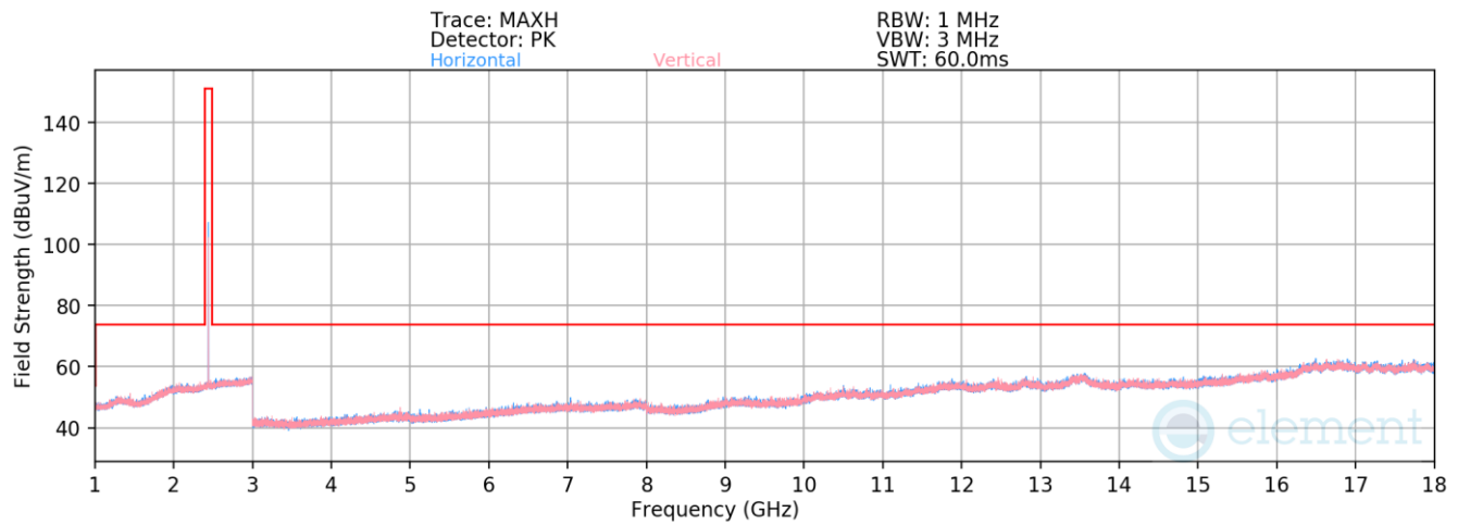
Plot 7-41. Radiated Spurious Emissions 1-18GHz (4Mbps, HDR4 – Ch. 38)
