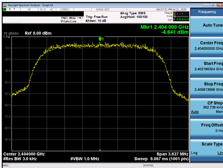
Plot 7-19. Power Spectral Density Plot (Bluetooth (HDP4), 4Mbps – Ch. 1)
