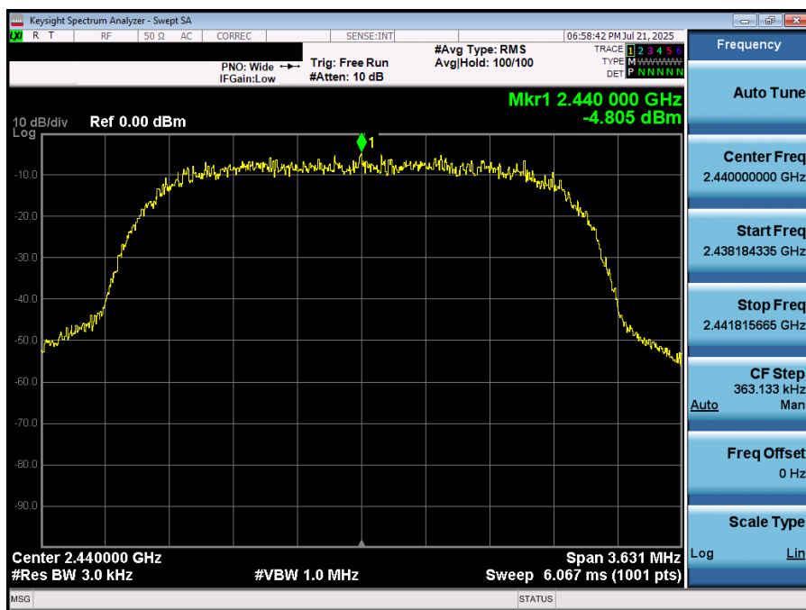
Plot 7-20. Power Spectral Density Plot (Bluetooth (HDP4), 4Mbps – Ch. 38)
