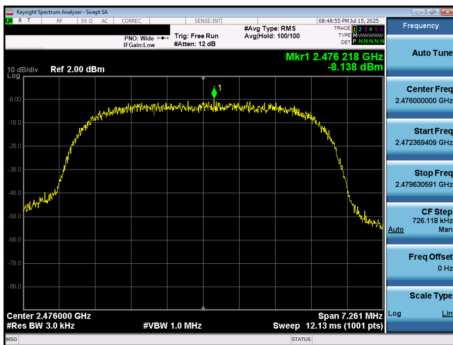
Plot 7-24. Power Spectral Density Plot (Bluetooth (HDRp8), 8Mbps – Ch. 73)
