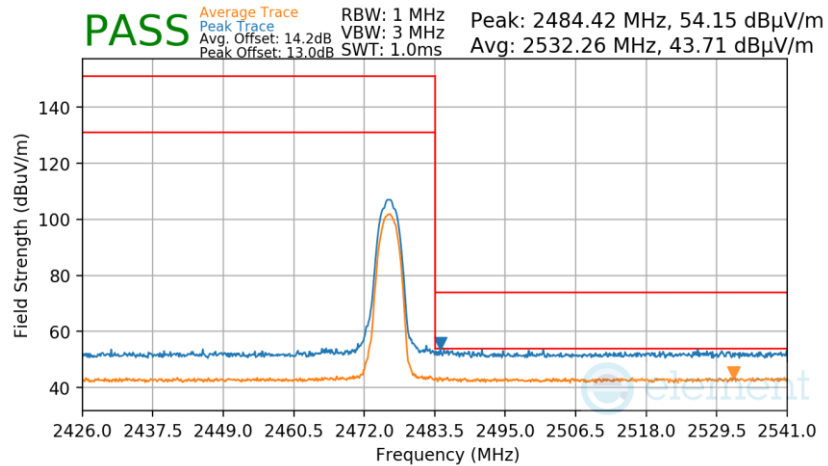
Plot 7-49. Radiated Restricted Upper Band Edge Measurement
