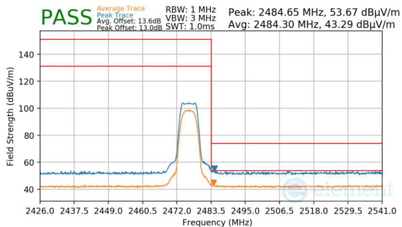
Plot 7-54. Radiated Restricted Upper Band Edge Measurement
