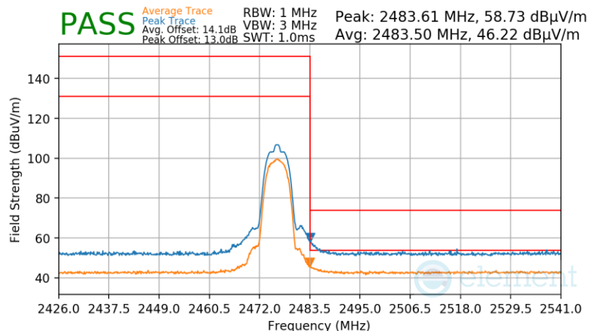
Plot 7-50. Radiated Restricted Upper Band Edge Measurement
