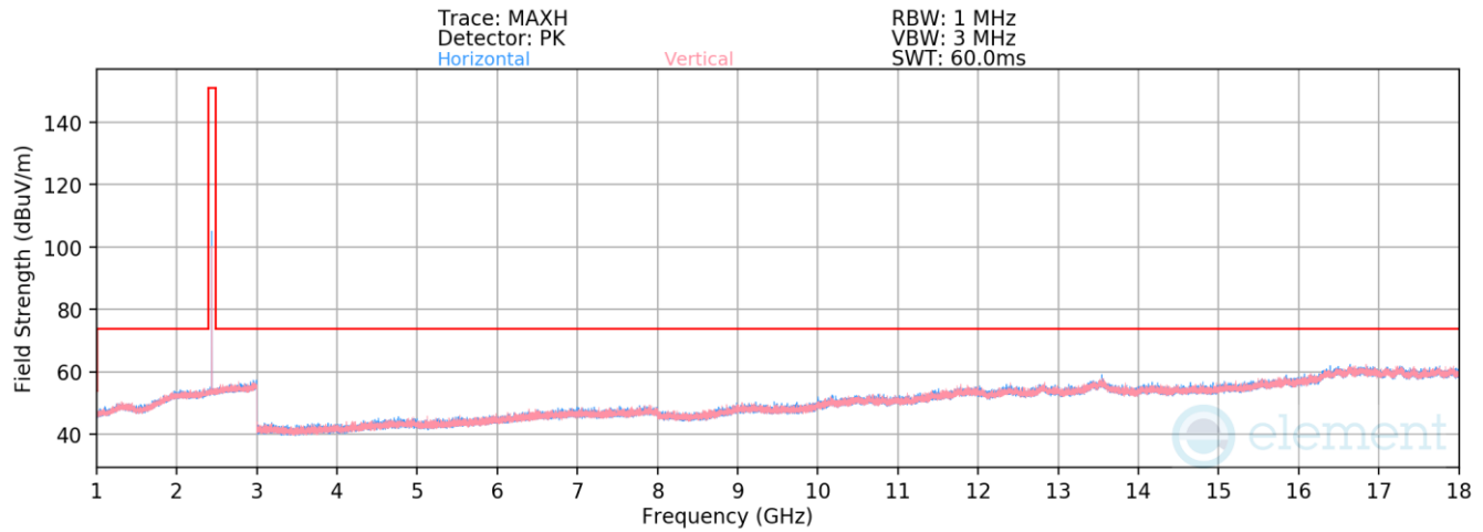
Plot 7-45. Radiated Spurious Emissions 1-18GHz (4Mbps, HDRp4 – Ch. 38)
