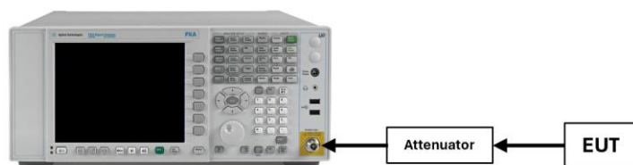
Figure 7-3. Test Instrument & Measurement Setup
