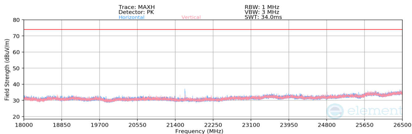
Plot 7-40. Radiated Spurious Emissions Above 18GHz (4Mbps, HDR4 – Ch. 1)
