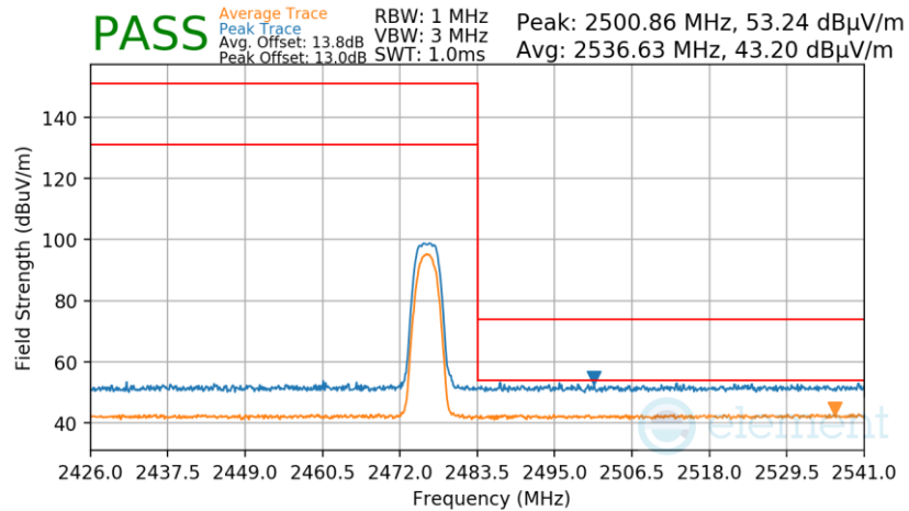
Plot 7-53. Radiated Restricted Upper Band Edge Measurement
