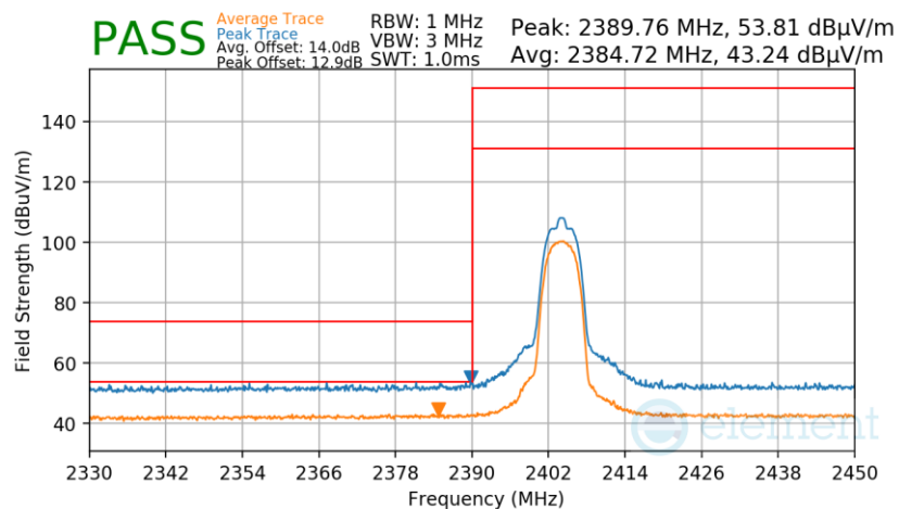
Plot 7-48. Radiated Restricted Lower Band Edge Measurement
