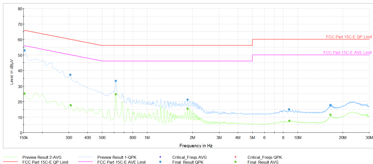
Plot 7-56. AC Line Conducted Plot with Bluetooth HDR (L1, 4Mbps - Ch.38 with Laptop)
