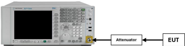
Figure 7-1. Test Instrument & Measurement Setup
