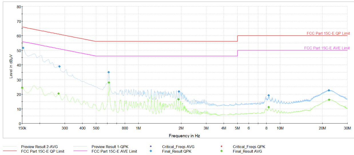
Plot 7-33. AC Line Conducted Plot with Bluetooth LE (N, 1Mbps – Ch.0, with Laptop)
