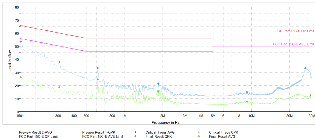
Plot 7-32. AC Line Conducted Plot with Bluetooth LE (L1, 1Mbps – Ch.0 with Laptop)
