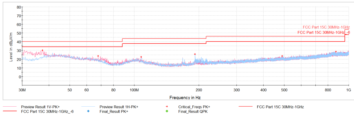
Plot 7-31. Radiated Spurious Emissions Below 1GHz (1Mbps – Ch.0, Pol. H & V, with AC/DC Adapter)
