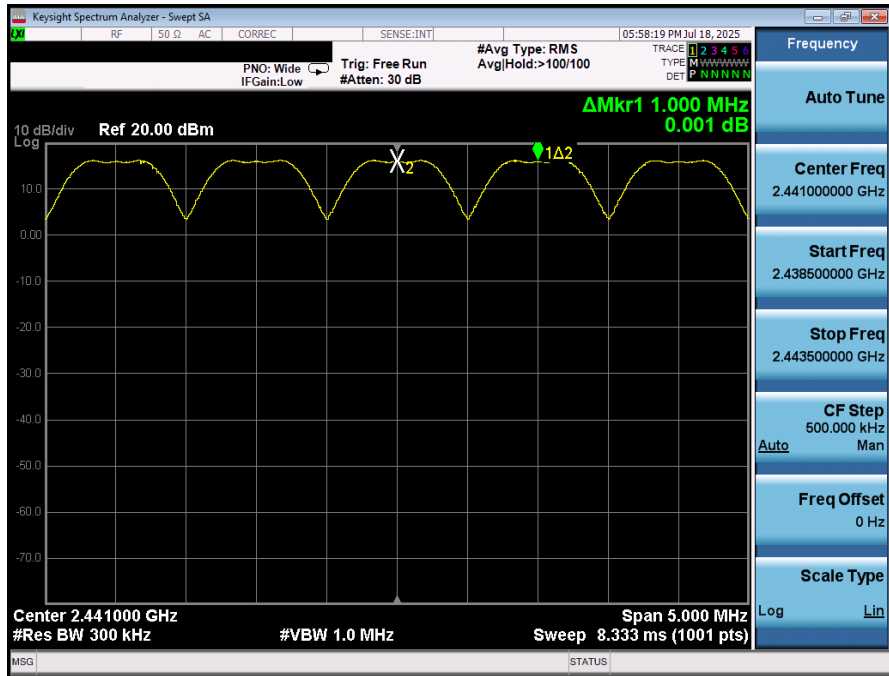
Plot 7-15. Channel Spacing Plot (Bluetooth, GFSK)
