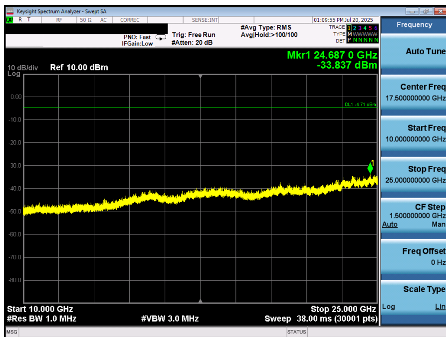
Plot 7-24. Conducted Spurious Plot (Bluetooth, GFSK – Ch. 0)
