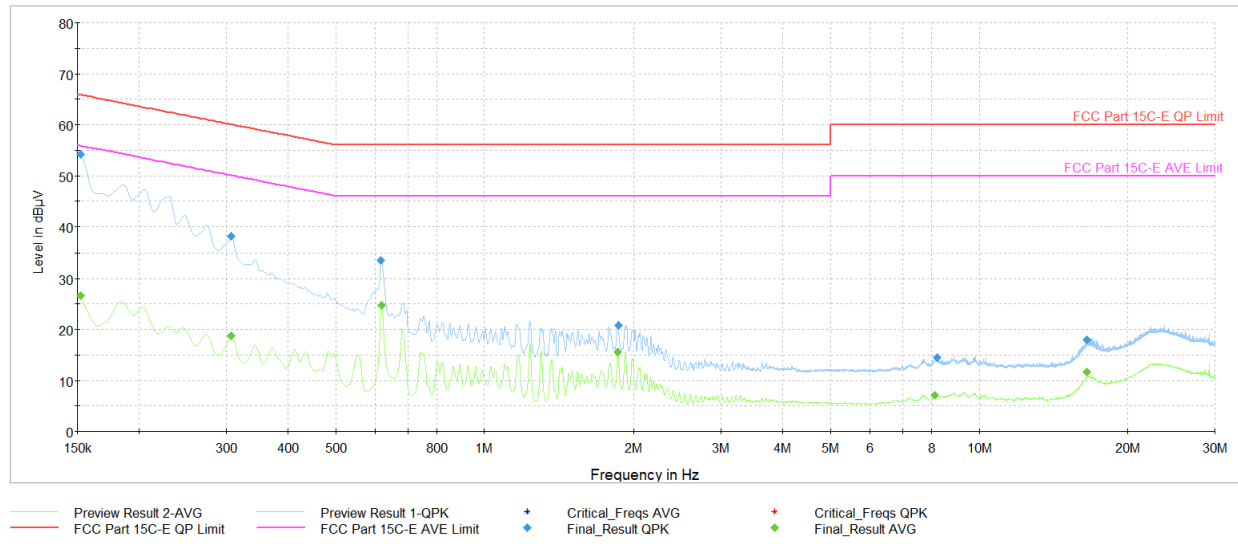
Plot 7-38. AC Line-Conducted Test Plot (L1, GFSK – Ch.78, with Laptop)
