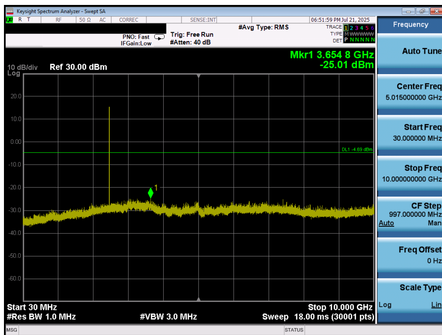
Plot 7-27. Conducted Spurious Plot (Bluetooth, GFSK – Ch. 78)
