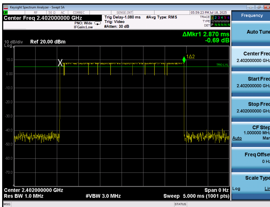
Plot 7-17. Time of Occupancy Plot (Bluetooth, GFSK)
