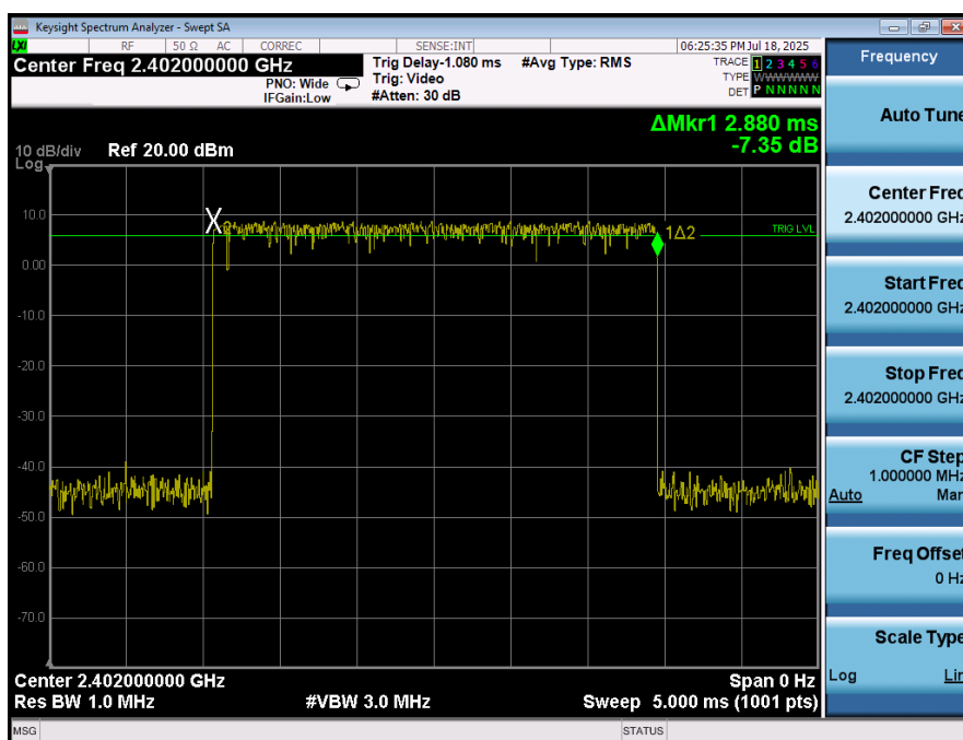
Plot 7-18. Time of Occupancy Plot (Bluetooth, 8DPSK)
