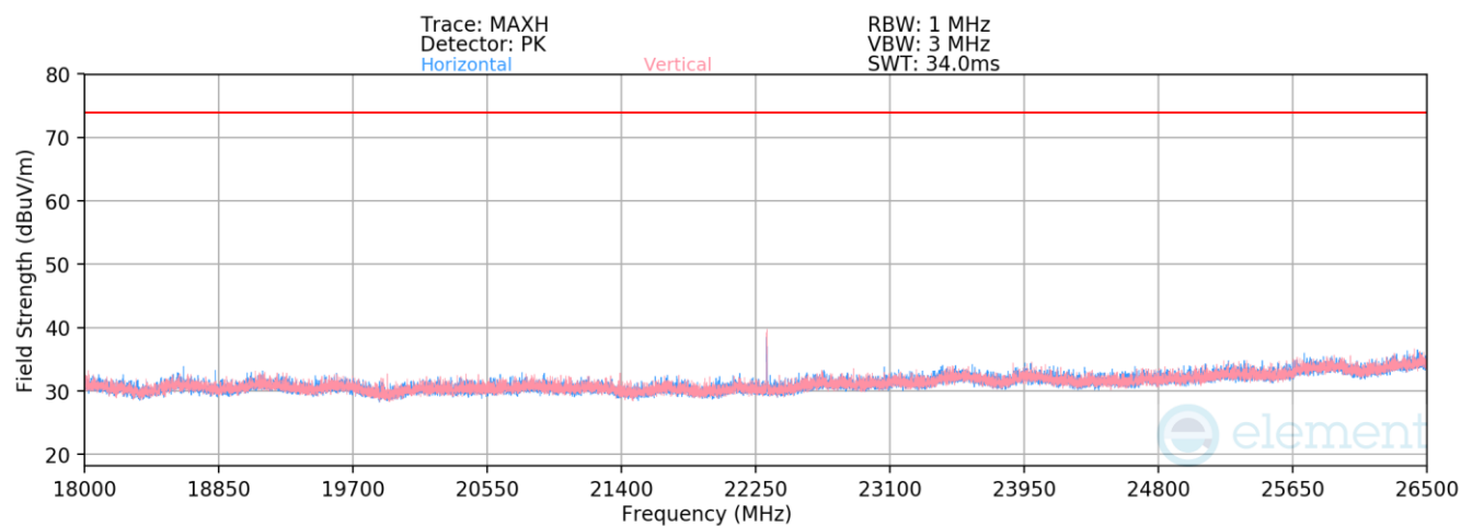
Plot 7-32. Radiated Spurious Emissions above 18GHz (BT GFSK – Ch. 78)
