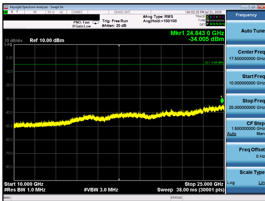
Plot 7-28. Conducted Spurious Plot (Bluetooth, GFSK – Ch. 78)
