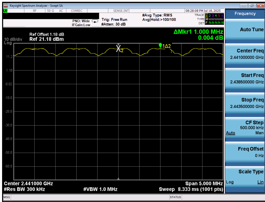
Plot 7-16. Channel Spacing Plot (Bluetooth, 8DPSK)
