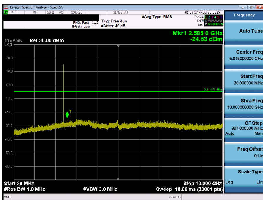
Plot 7-23. Conducted Spurious Plot (Bluetooth, GFSK – Ch. 0)
