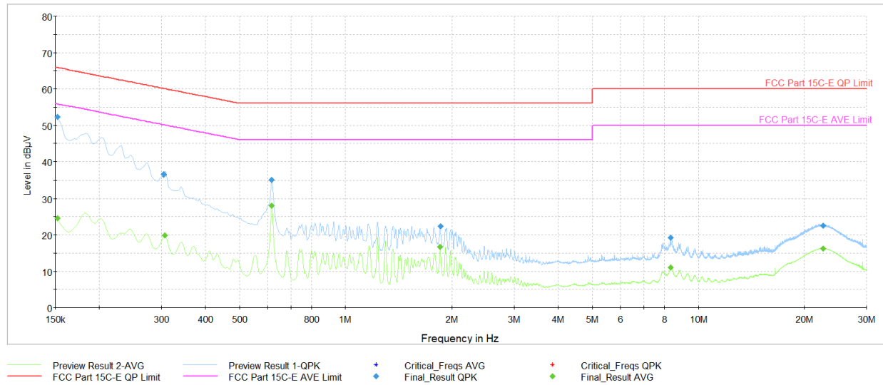
Plot 7-39. AC Line-Conducted Test Plot (N, GFSK – Ch.78, with Laptop)
