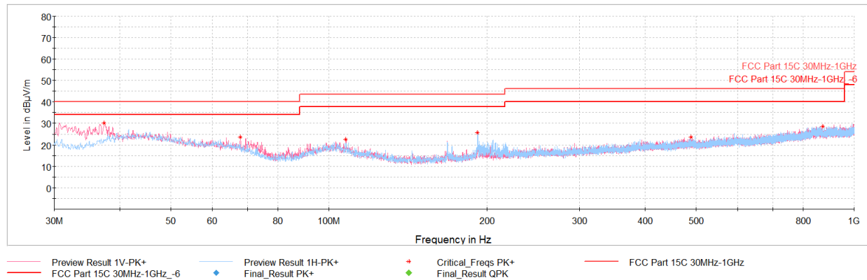
Plot 7-37. Radiated Spurious Emissions Below 1GHz (GFSK – Ch.78, with AC/DC Adapter)
