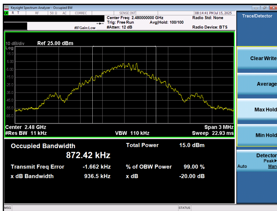
Plot 7-3. 20dB BW and 99% OBW Plot (Bluetooth, GFSK – Ch. 78)
