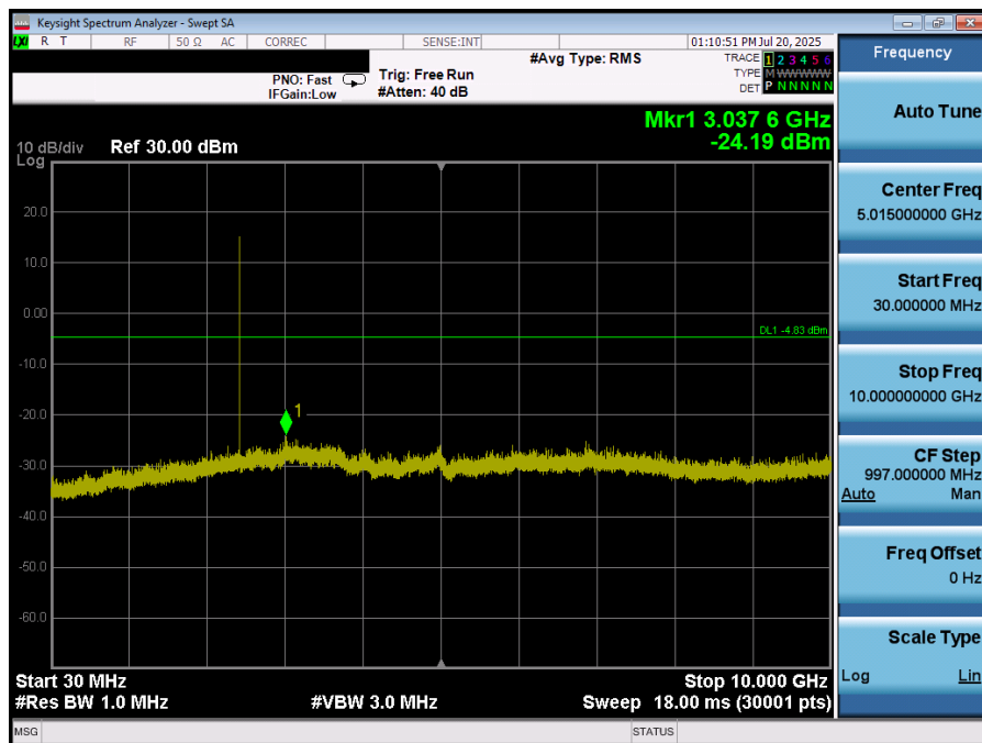
Plot 7-25. Conducted Spurious Plot (Bluetooth, GFSK – Ch. 39)
