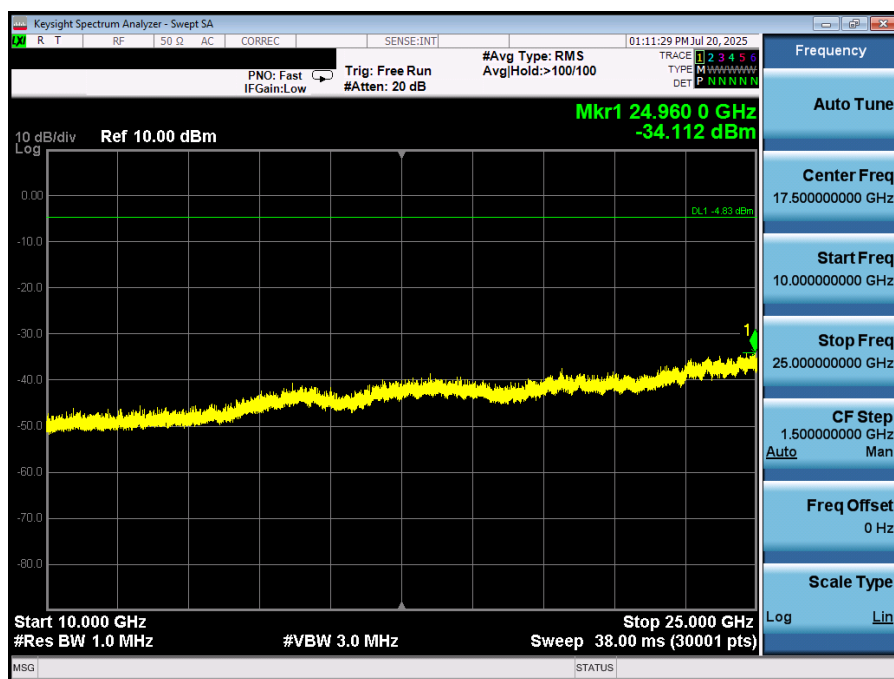
Plot 7-26. Conducted Spurious Plot (Bluetooth, GFSK Ch. 39)
