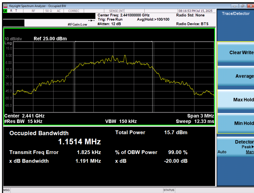
Plot 7-5. 20dB BW and 99% OBW Plot (Bluetooth, 8DPSK – Ch. 39)
