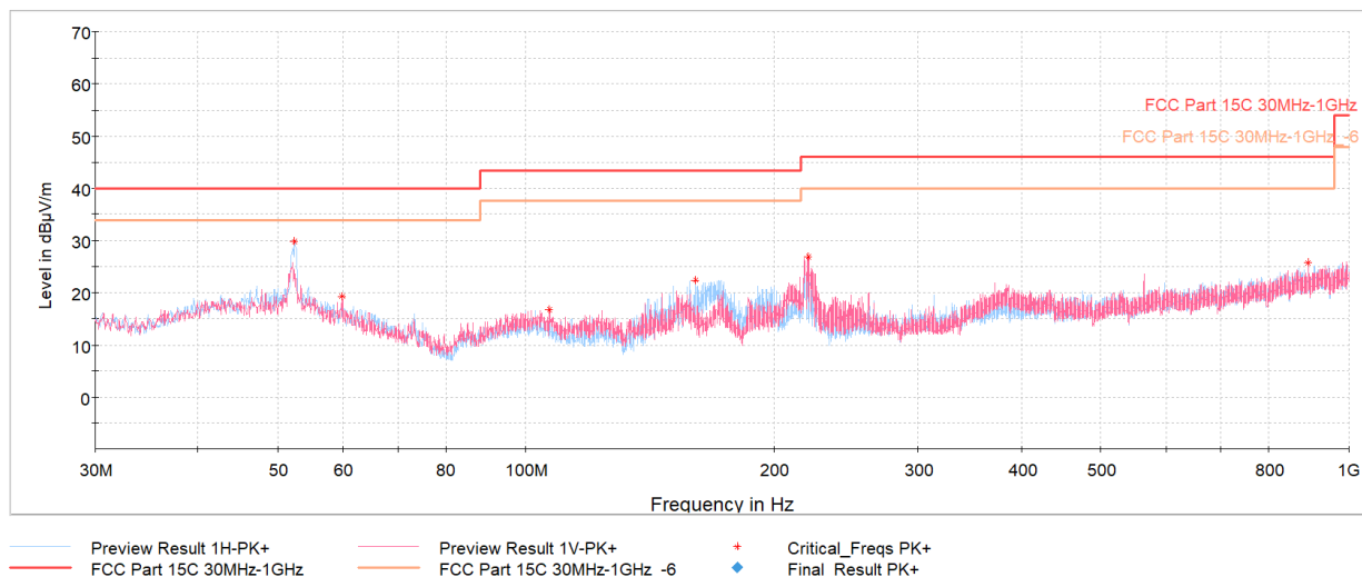
Plot 7-34. Co-Tx Radiated Spurious Emissions Below 1GHz with host PC via USB-C cable with wire charger
