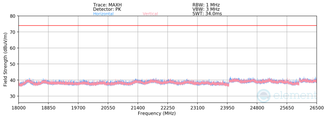
Plot 7-28. Radiated Spurious Emissions – Co-Tx Above 18GHz
