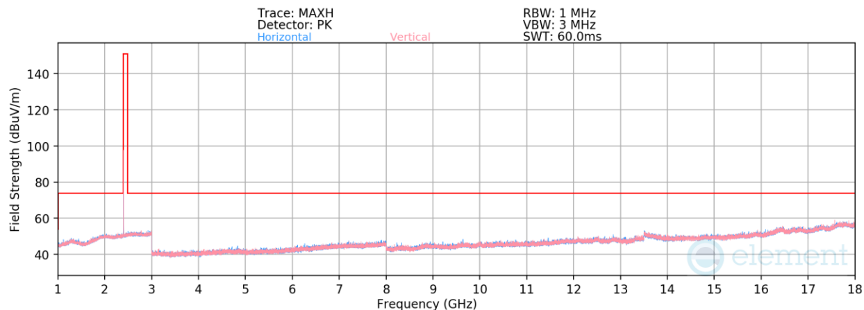
Plot 7-23. Radiated Spurious Emissions 1-18GHz (1Mbps – Ch. 0)
