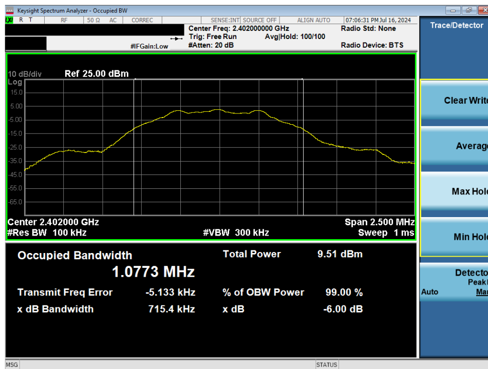
Plot 7-1. 6dB BW & 99% OBW Plot (Bluetooth (LE), 1Mbps – Ch. 0)
