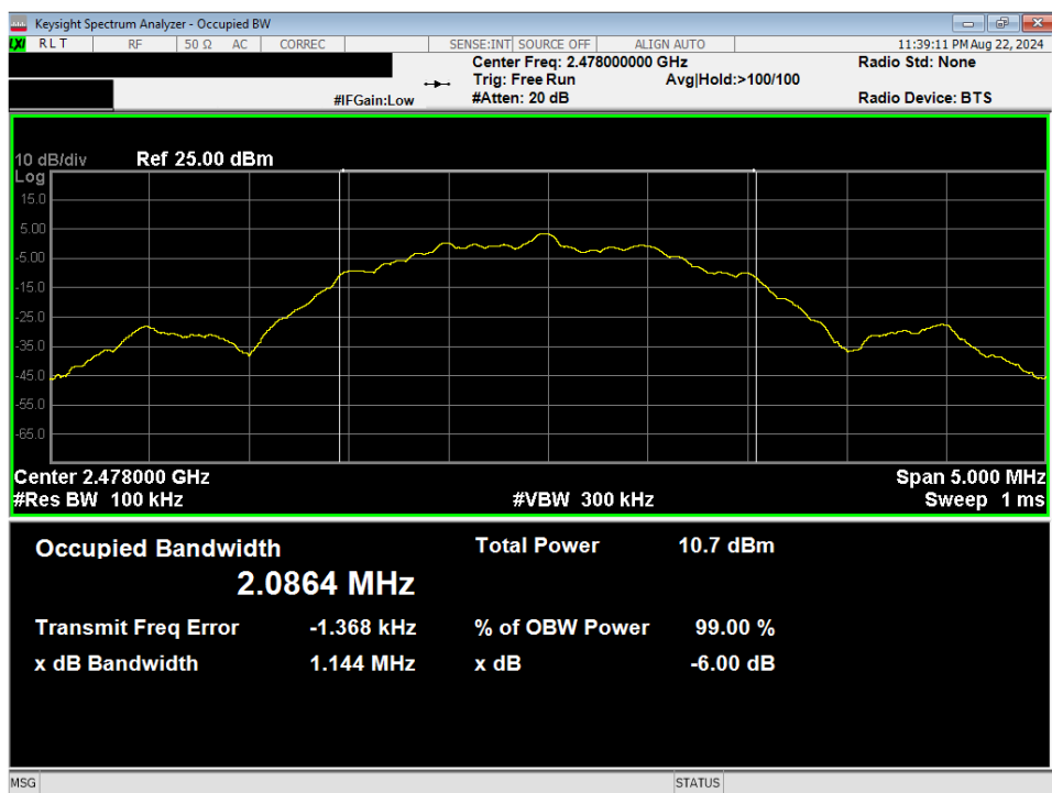
Plot 7-6. 6dB BW & 99% OBW Plot (Bluetooth (LE), 2Mbps – Ch. 38)
