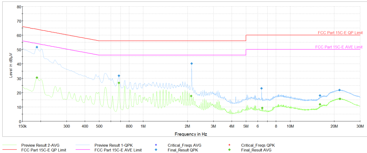
Plot 7-36. AC Line Conducted Plot with Bluetooth LE (N, 1Mbps, Ch.19, with host PC via USB-C cable with wire charger)
