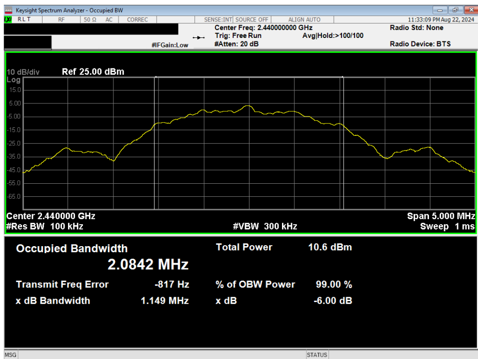
Plot 7-5. 6dB BW & 99% OBW Plot (Bluetooth (LE), 2Mbps – Ch. 19)
