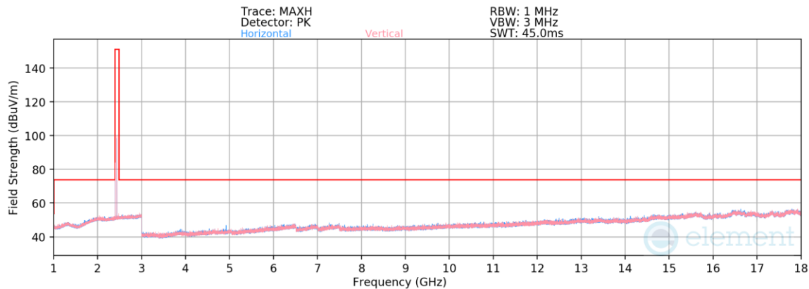
Plot 7-27. Radiated Spurious Emissions – Co-Tx 1-18GHz
