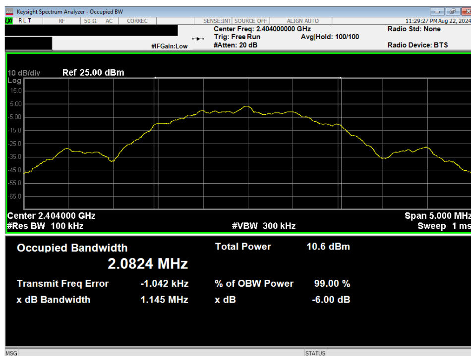
Plot 7-4. 6dB BW & 99% OBW Plot (Bluetooth (LE), 2Mbps – Ch. 1)
