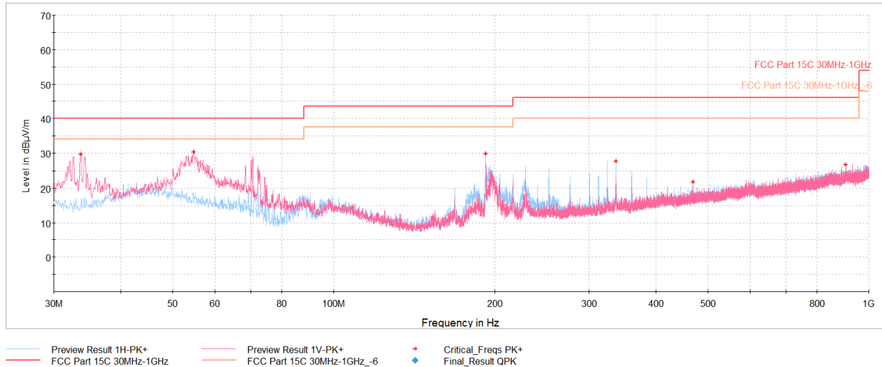
Plot 7-33. Radiated Spurious Emissions Below 1GHz (1Mbps – Ch.19, Pol. H & V, with AC/DC adaptor via USB-C cable with wire charger)
