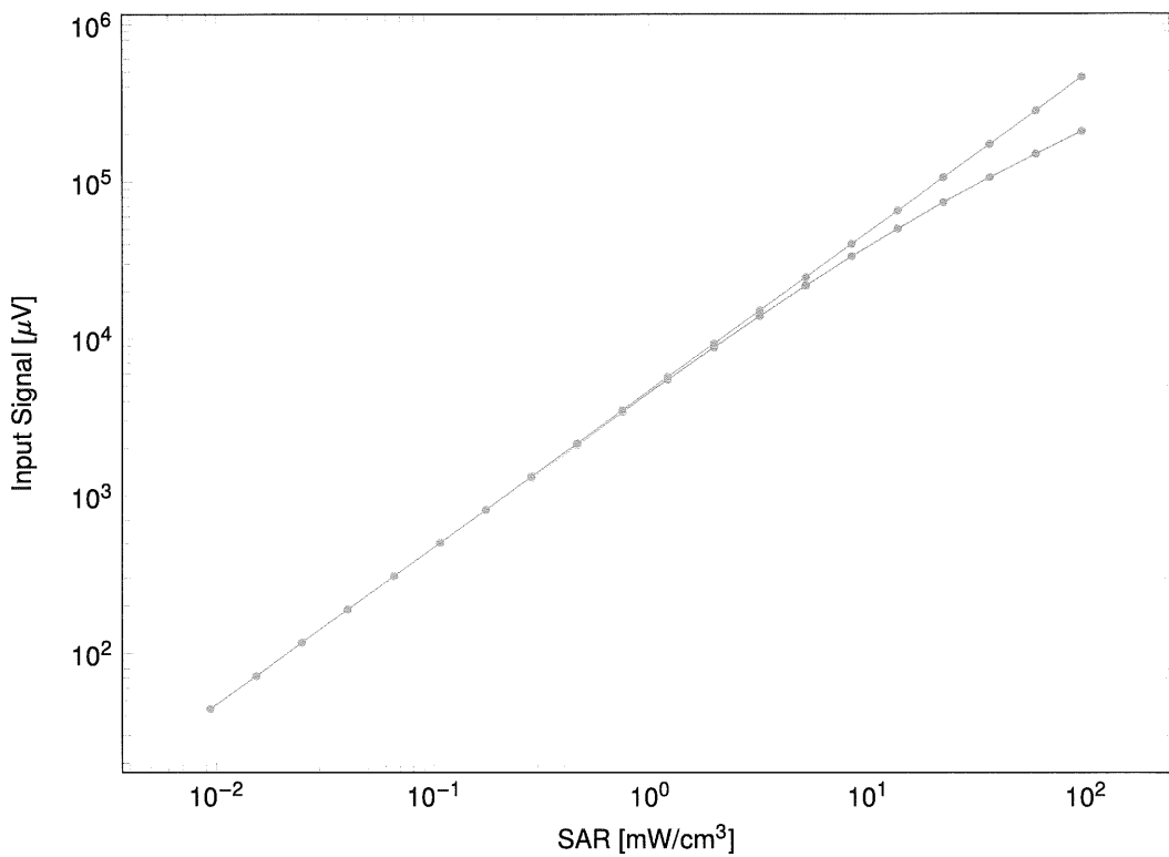
Dynamic Range f(SAR head ) (TEM cell, f eval = 1900MHz)
