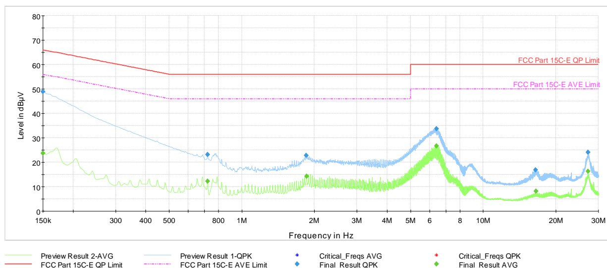
Plot 7-36. AC Line Conducted Plot with Bluetooth LE (N, 1Mbps – Ch.19 with host PC and USB-C cable)
