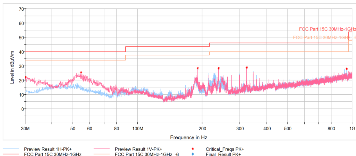
Plot 7-37. Radiated Spurious Emissions Below 1GHz (GFSK– Ch.78, with AC/DC Adapter & USB-C Cable)
