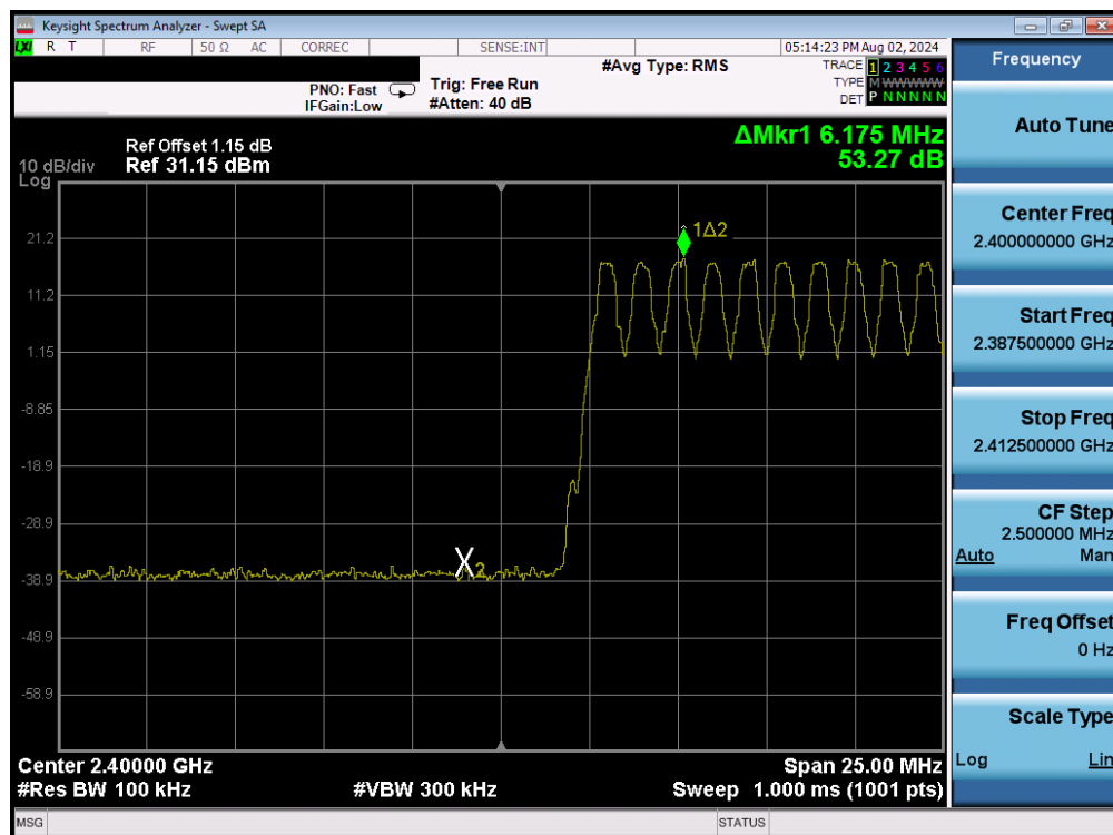
Plot 7-9. Band Edge Plot (Bluetooth with Hopping Enabled, GFSK – Ch. 0)
