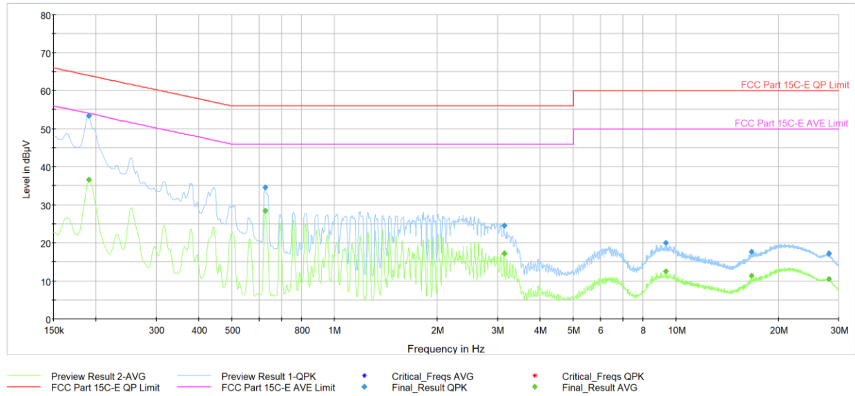
Plot 7-39. AC Line-Conducted Test Plot (N, GFSK – Ch.78, with host PC with USB-C cable)
