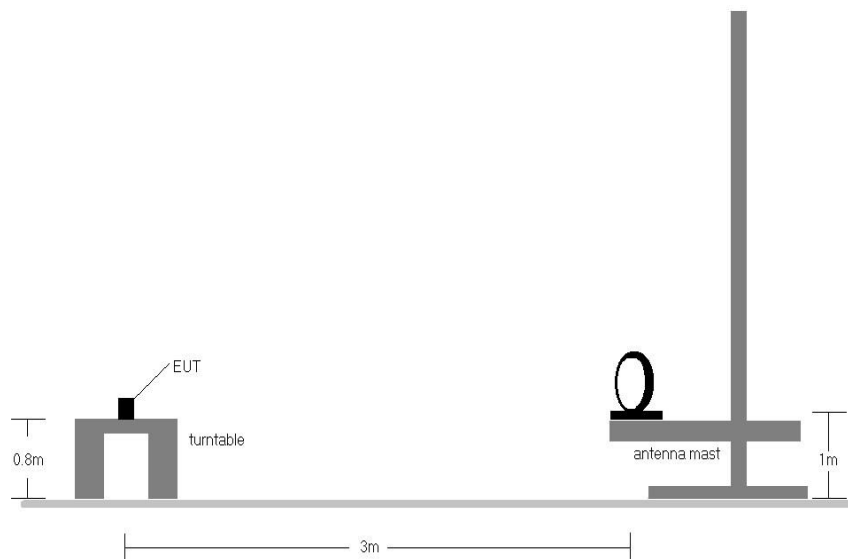
Figure 7-9. Radiated Test Setup < 30MHz
