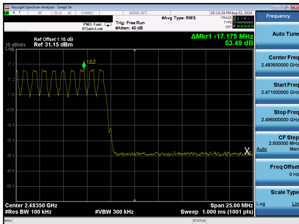
Plot 7-10. Band Edge Plot (Bluetooth with Hopping Enabled, GFSK – Ch. 78)
