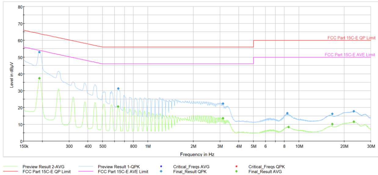
Plot 7-38. AC Line-Conducted Test Plot (L1, GFSK – Ch.78, with host PC with USB-C cable)
