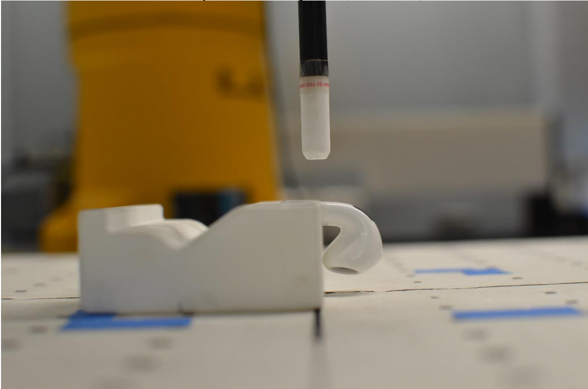
SAR Test Setup Photo 9: Body-Worn, Back Side, 9.69 mm
