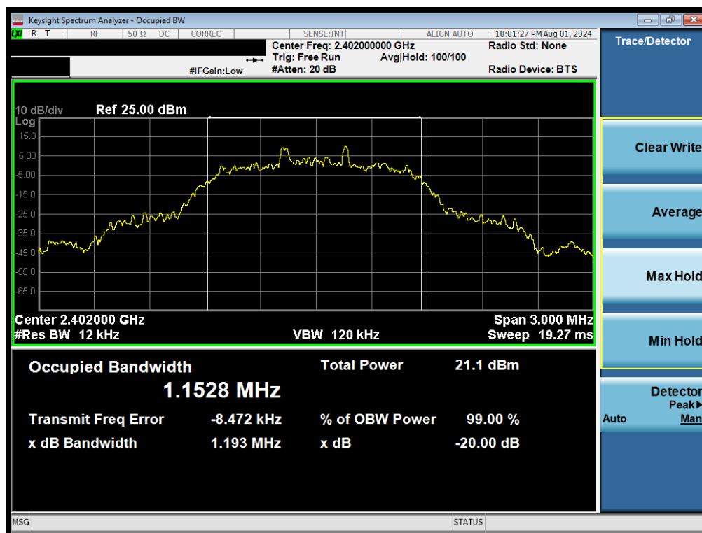
Plot 7-4. 20dB BW and 99% OBW Plot (Bluetooth, 8DPSK – Ch. 0)
