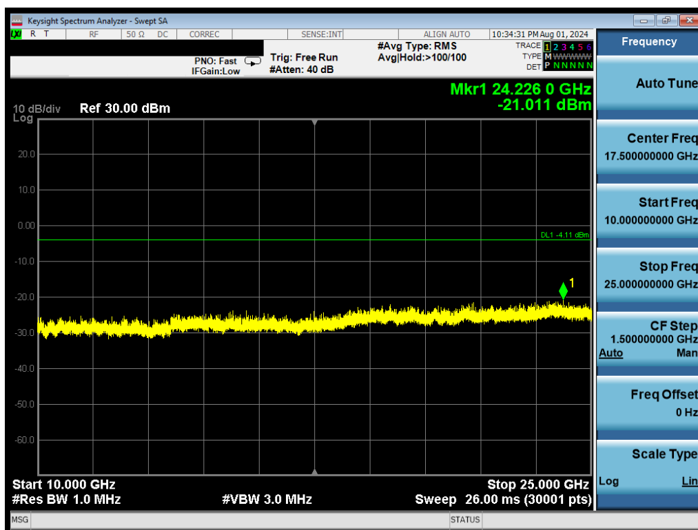
Plot 7-36. Conducted Spurious Plot (Bluetooth (HDR4), 4 Mbps, - Ch. 38)
