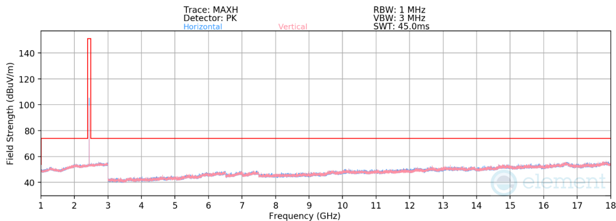
Plot 7-40. Radiated Spurious Emissions 1-18GHz (4Mbps, HDR4, - Ch. 38)
