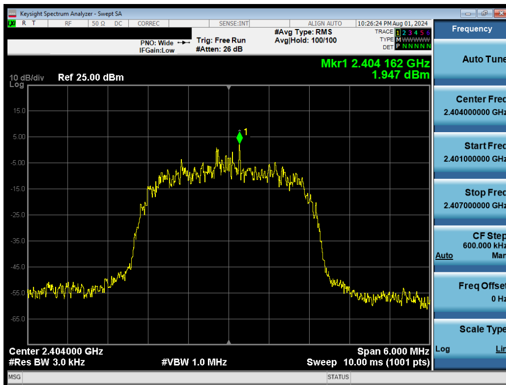
Plot 7-13. Power Spectral Density Plot (Bluetooth (HDR4), 4Mbps, – Ch. 1)
