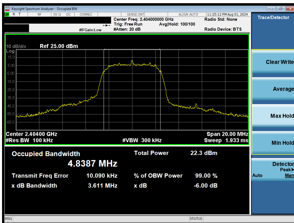
Plot 7-10. 6dB BW & 99% OBW Plot (Bluetooth (HDRp8), 8Mbps, – Ch. 1)
