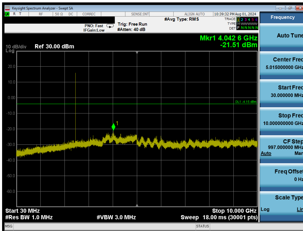
Plot 7-37. Conducted Spurious Plot (Bluetooth (HDR4), 4 Mbps, – Ch. 73)
