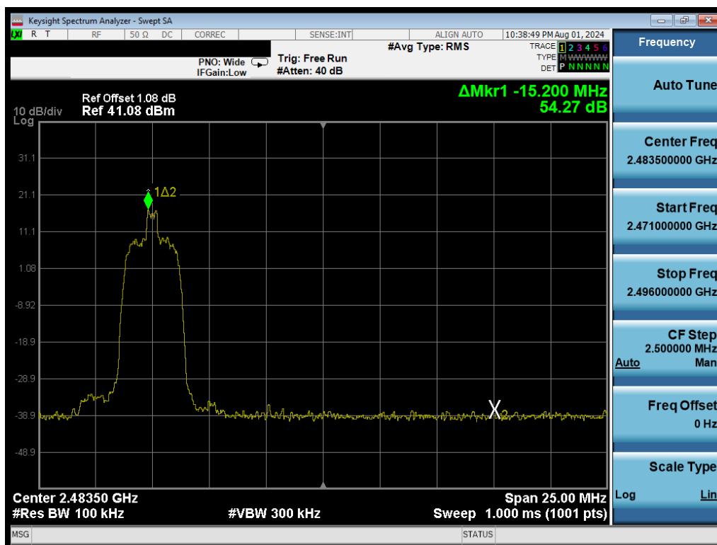
Plot 7-26. Band Edge Plot (Bluetooth (HDR4), – Ch. 73)
