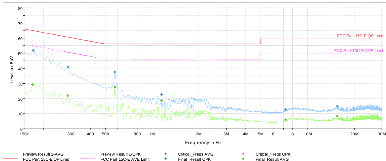
Plot 7-52. AC Line Conducted Plot with Bluetooth HDR (L1, 4Mbps - Ch.38 with host PC and USB-C cable)
