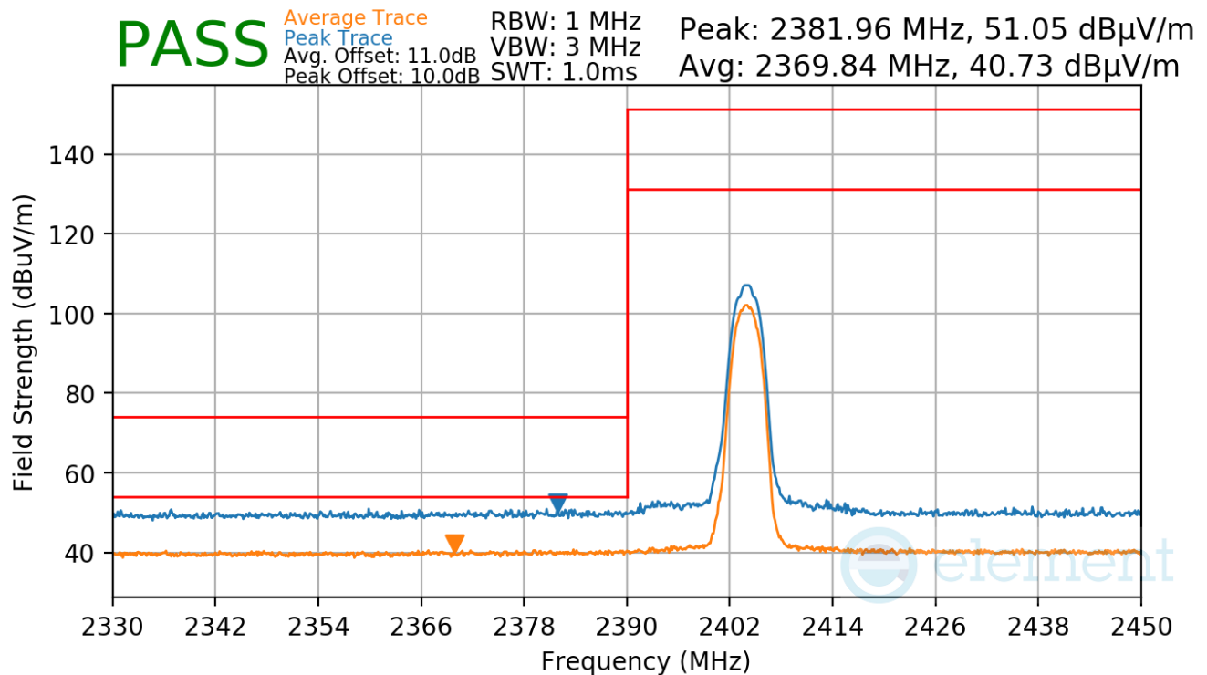
Plot 7-43. Radiated Restricted Lower Band Edge Measurement
