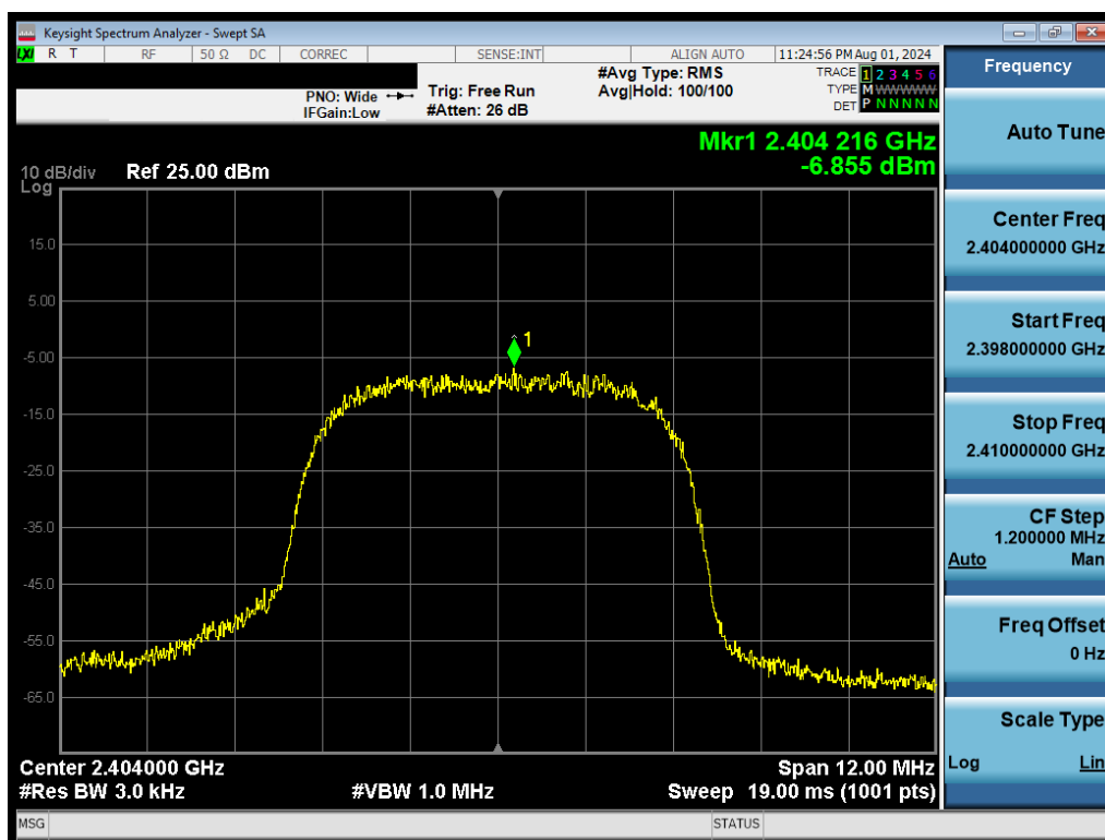
Plot 7-22. Power Spectral Density Plot (Bluetooth (HDRp8), 8Mbps, – Ch. 1)
