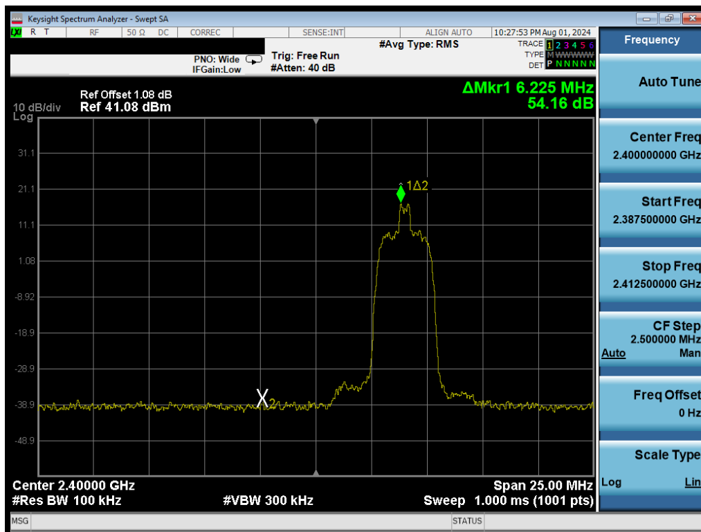
Plot 7-25. Band Edge Plot (Bluetooth (HDR4), – Ch. 1)
