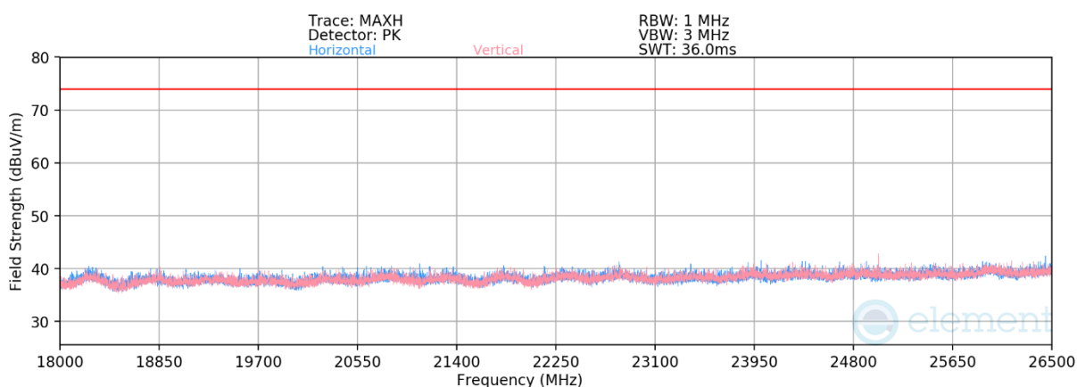
Plot 7-41. Radiated Spurious Emissions Above 18GHz (4Mbps, HDR4, - Ch. 38)
