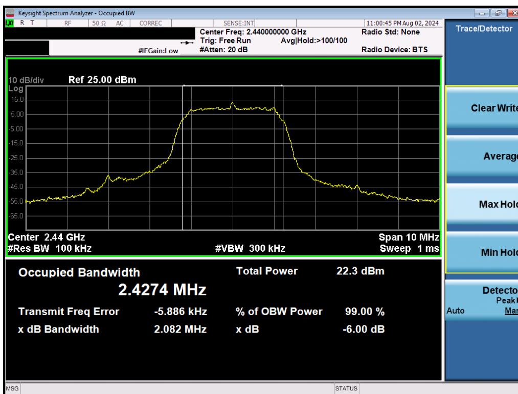
Plot 7-8. 6dB BW & 99% OBW Plot Bluetooth (HDRp4), 4Mbps, – Ch. 37)
