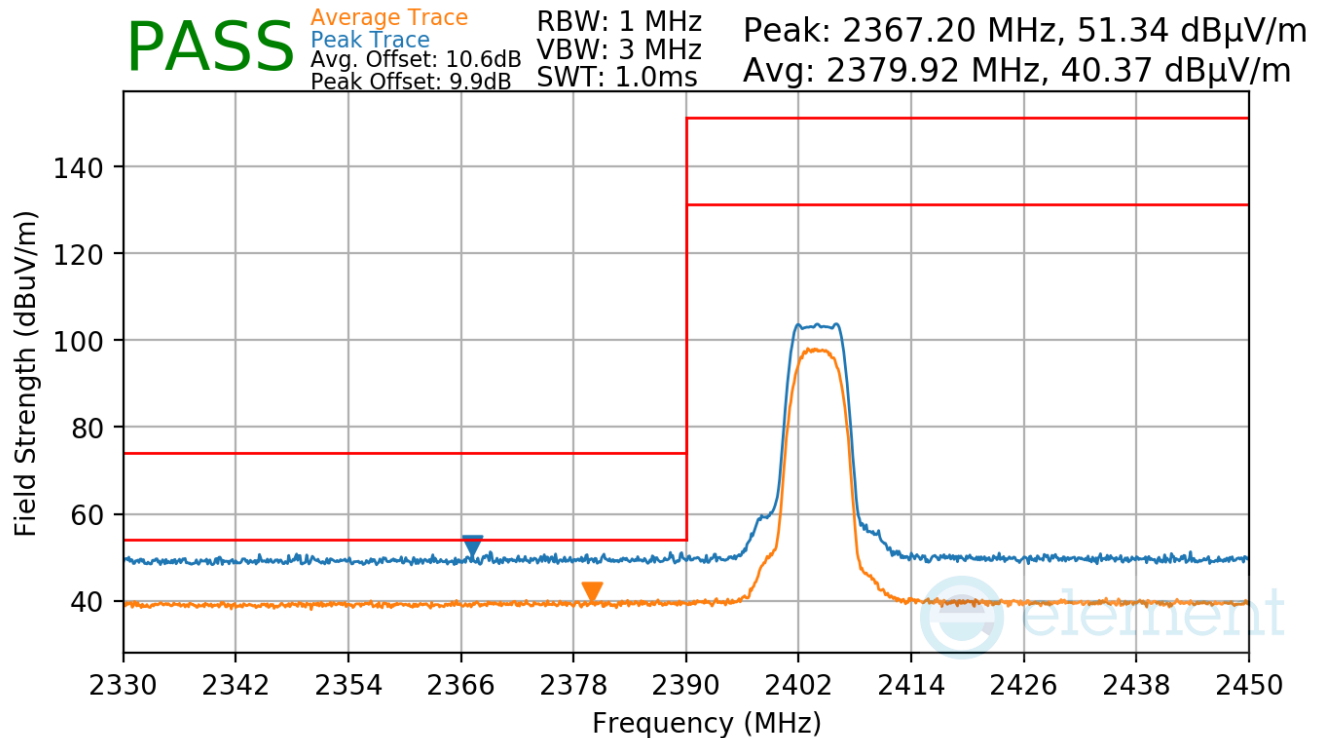
Plot 7-46. Radiated Restricted Lower Band Edge Measurement
