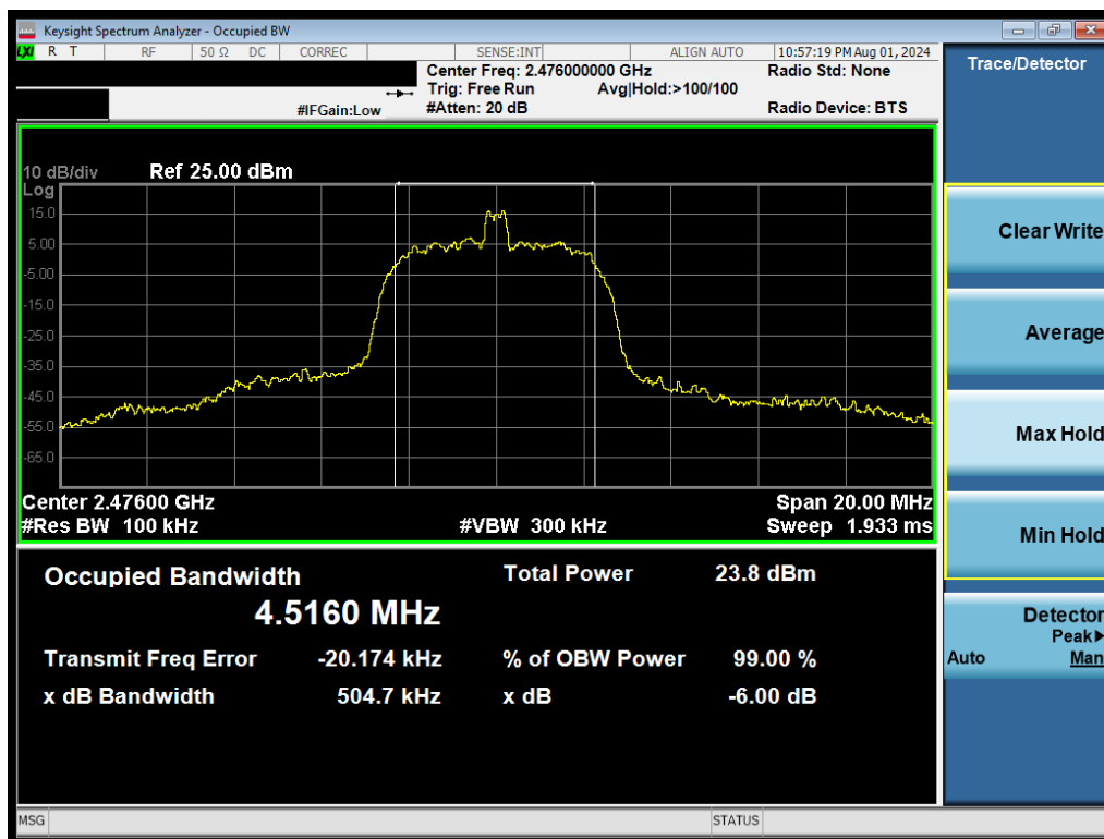
Plot 7-6. 6dB BW & 99% OBW Plot (Bluetooth (HDR8), 8Mbps, – Ch. 73)
