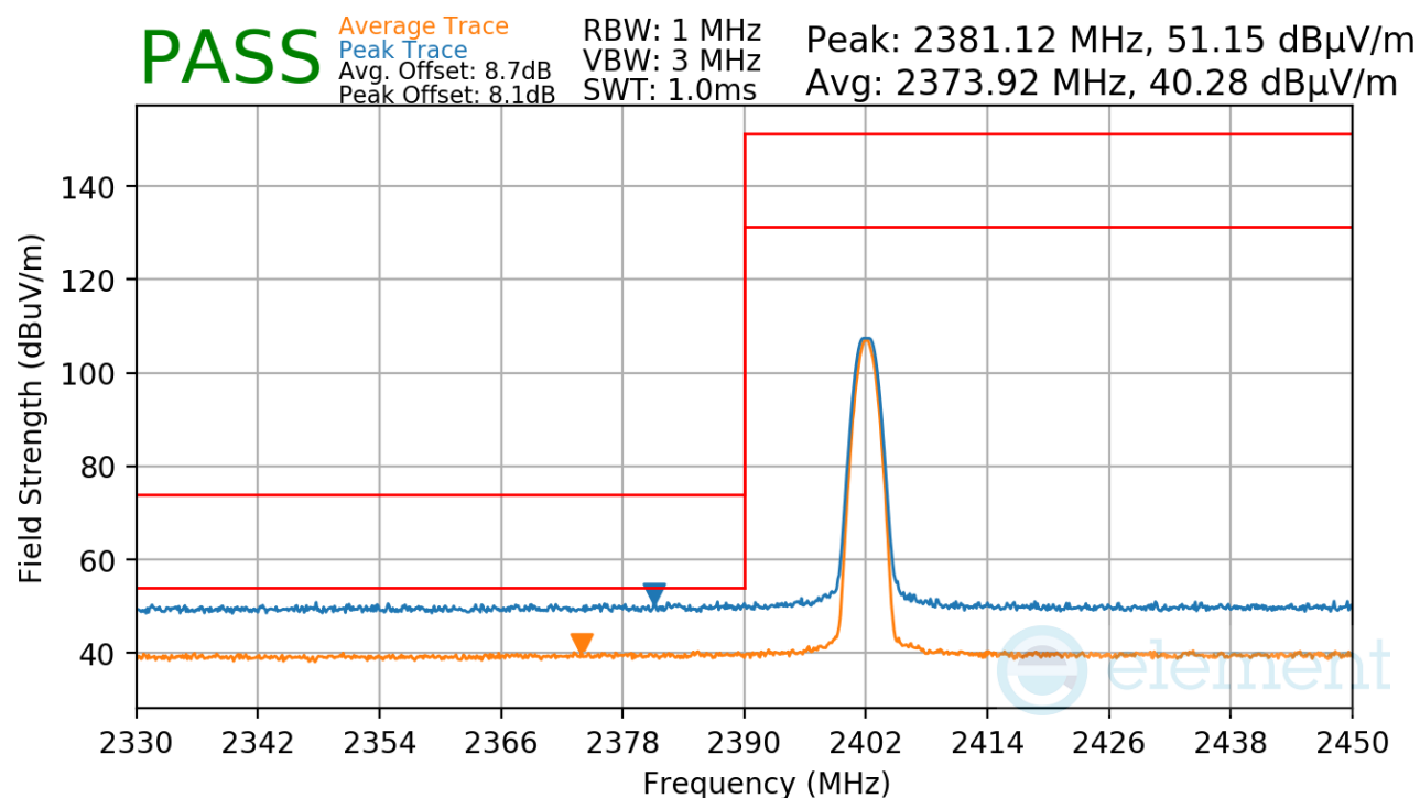
Plot 7-29. Radiated Restricted Lower Band Edge Measurement (Average & Peak)
