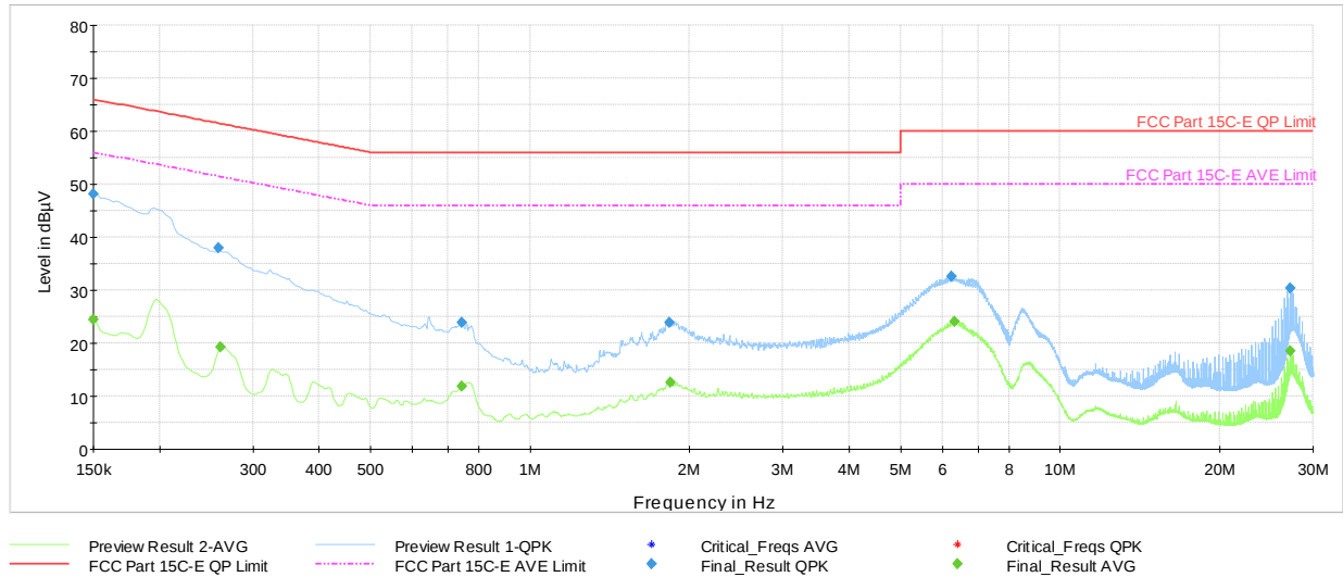
Plot 7-36. AC Line Conducted Plot with Bluetooth LE (N, 1Mbps – Ch.39 with host PC and USB-C Cable)
