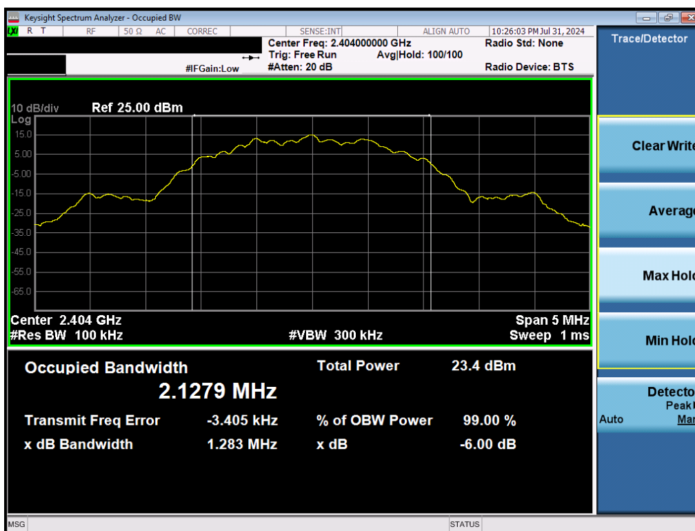
Plot 7-4. 6dB BW & 99% OBW Plot (Bluetooth (LE), 2Mbps – Ch. 1)
