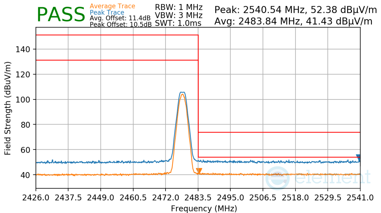
Plot 7-32. Radiated Restricted Upper Band Edge Measurement (Average & Peak)
