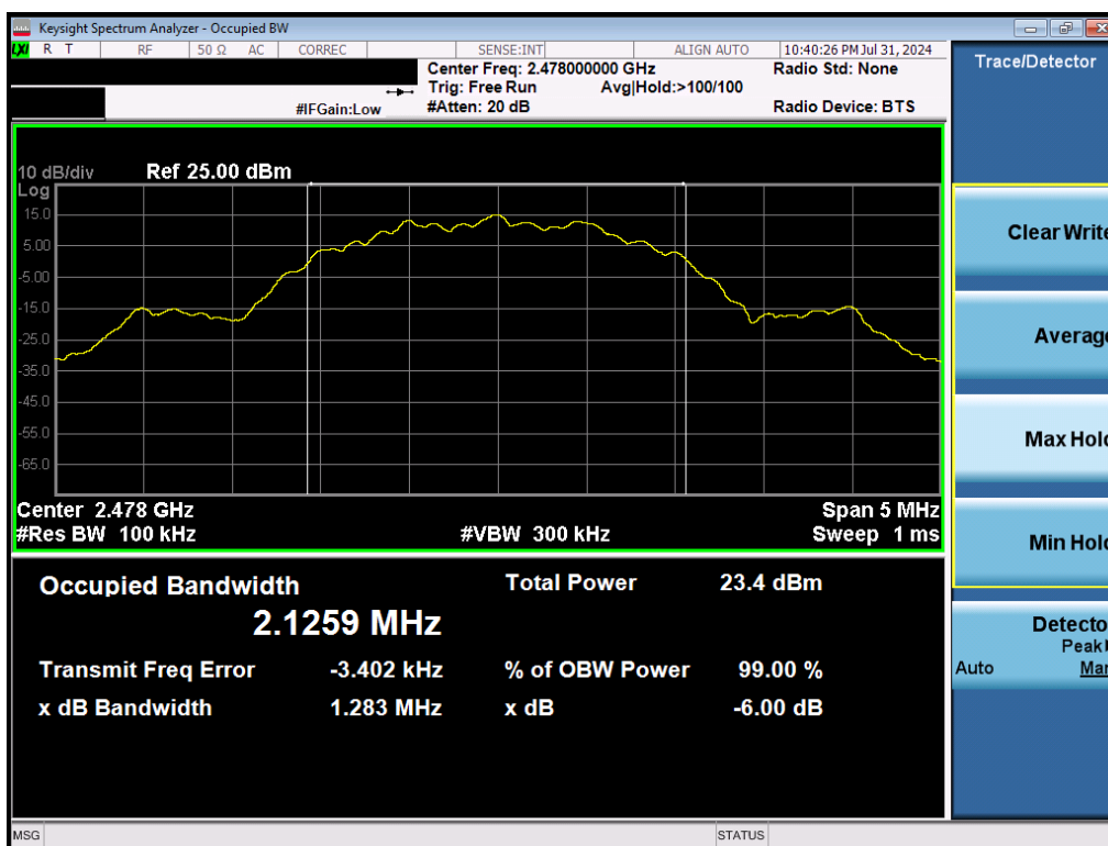
Plot 7-6. 6dB BW & 99% OBW Plot (Bluetooth (LE), 2Mbps – Ch. 38)
