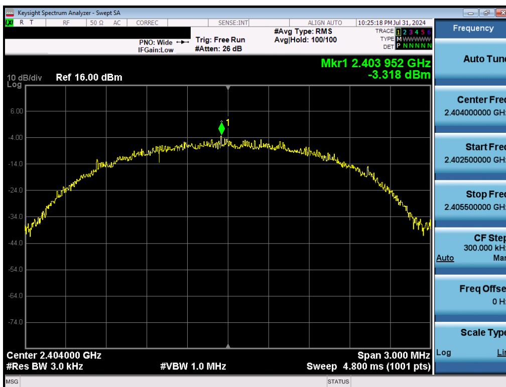
Plot 7-10. Power Spectral Density Plot (Bluetooth (LE), 2Mbps – Ch. 1)
