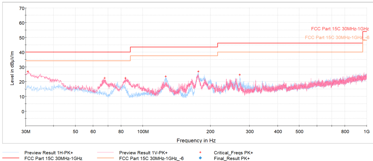
Plot 7-33. Radiated Spurious Emissions Below 1GHz (1Mbps – Ch.39, Pol. H & V, with host PC and USB-C Cable)
