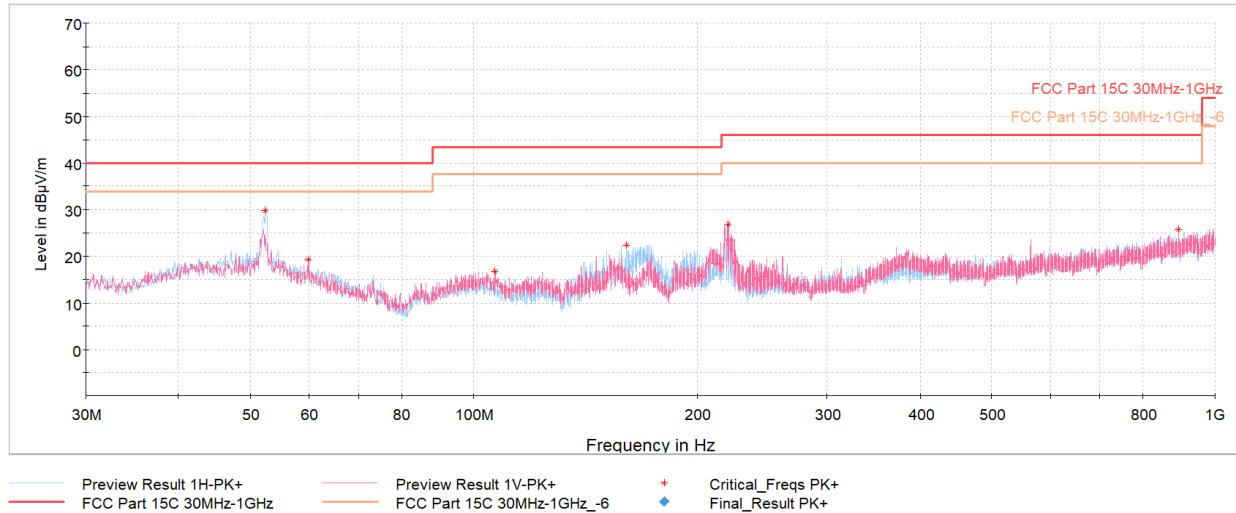
Plot 7-34. Co-Tx Radiated Spurious Emissions Below 1GHz with host PC and USB-C Cable
