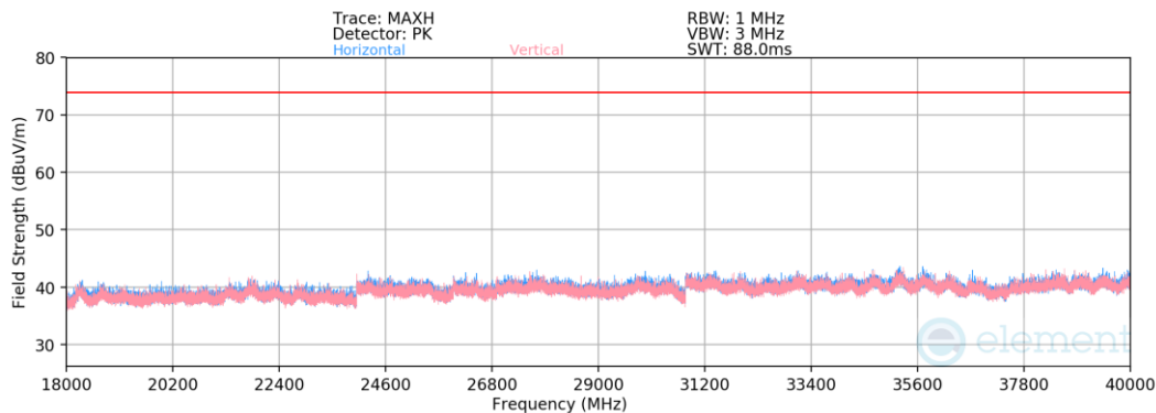
Plot 7-28. Radiated Spurious Emissions – Co-Tx Above 18GHz
