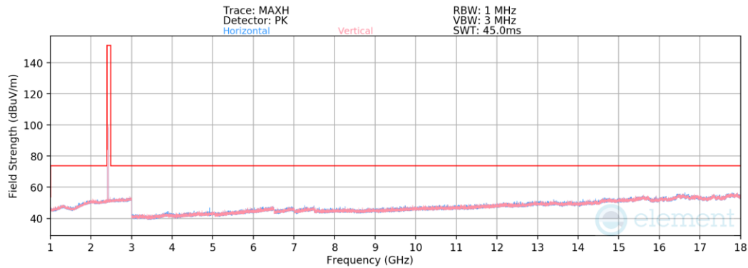
Plot 7-27. Radiated Spurious Emissions – Co-Tx 1-18GHz
