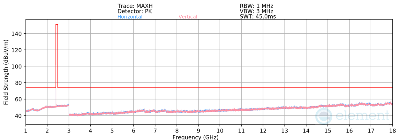
Plot 7-23. Radiated Spurious Emissions 1-18GHz (1Mbps – Ch. 0)
