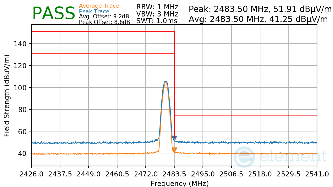
Plot 7-30. Radiated Restricted Upper Band Edge Measurement (Average & Peak)
