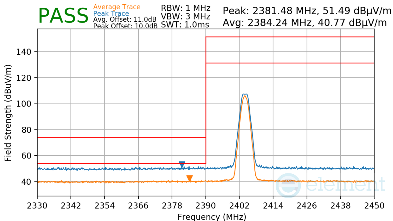
Plot 7-31. Radiated Restricted Lower Band Edge Measurement (Average & Peak)
