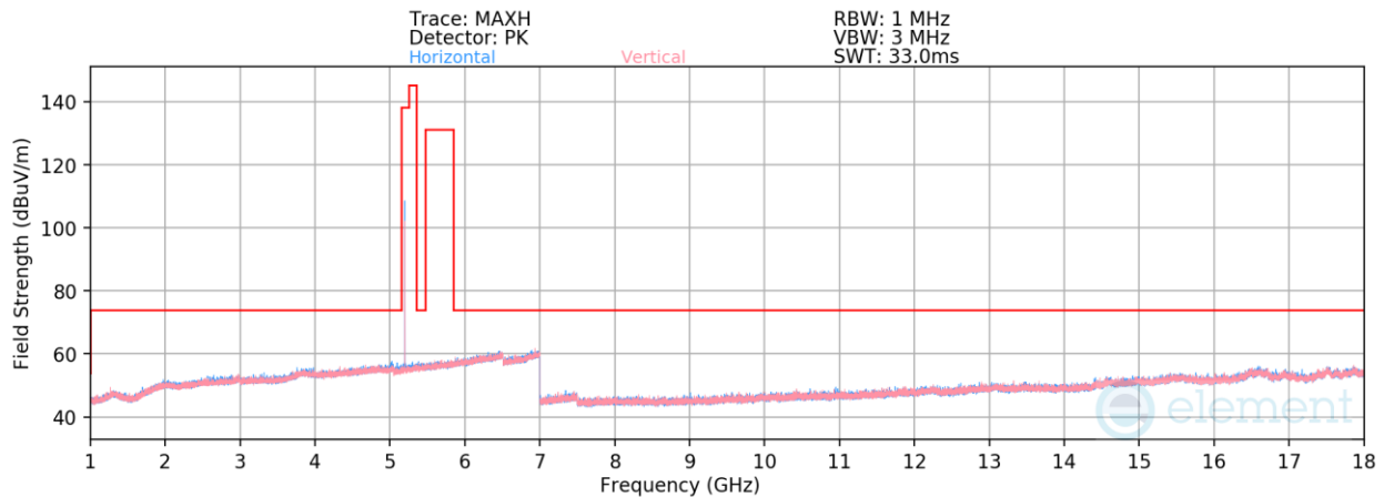
Plot 7-74. Radiated Spurious Emissions 1-18GHz (NB UNII BDR – 5201MHz)
