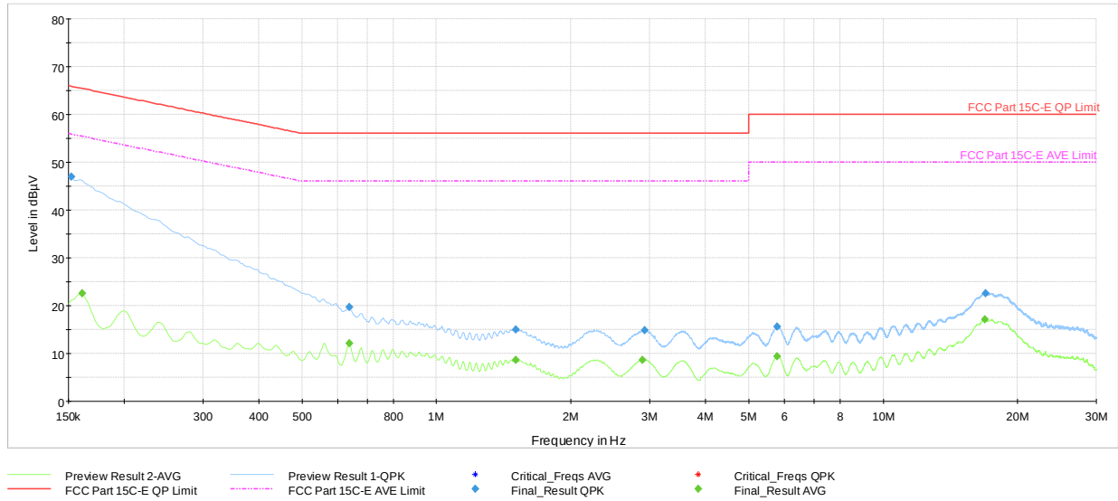
Plot 7-39. AC Line-Conducted Test Plot (N, GFSK – Ch.78, with Laptop + USB-C Cable)
