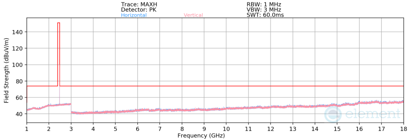
Plot 7-31. Radiated Spurious Emissions above 1GHz (BT GFSK – Ch. 78)
