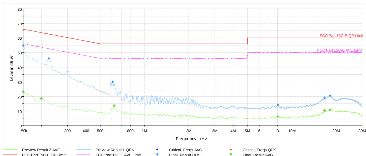
Plot 7-38. AC Line-Conducted Test Plot (L1, GFSK – Ch.78, with Laptop + USB-C Cable)
