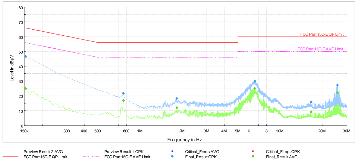
Plot 7-33. AC Line Conducted Plot with Bluetooth LE (N, 1Mbps – Ch.19, with host PC and USB-C Cable)
