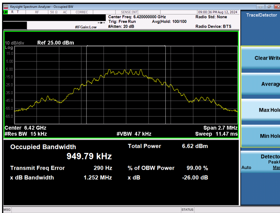
Plot 7-3. 26dB BW & 99% OBW (NB UNII BDR – 6420MHz)
