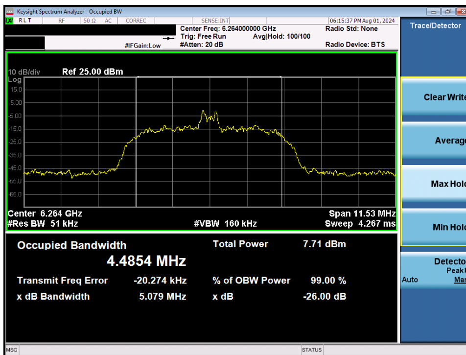
Plot 7-11. 26dB BW & 99% OBW (NB UNII HDR8 – 6264MHz)
