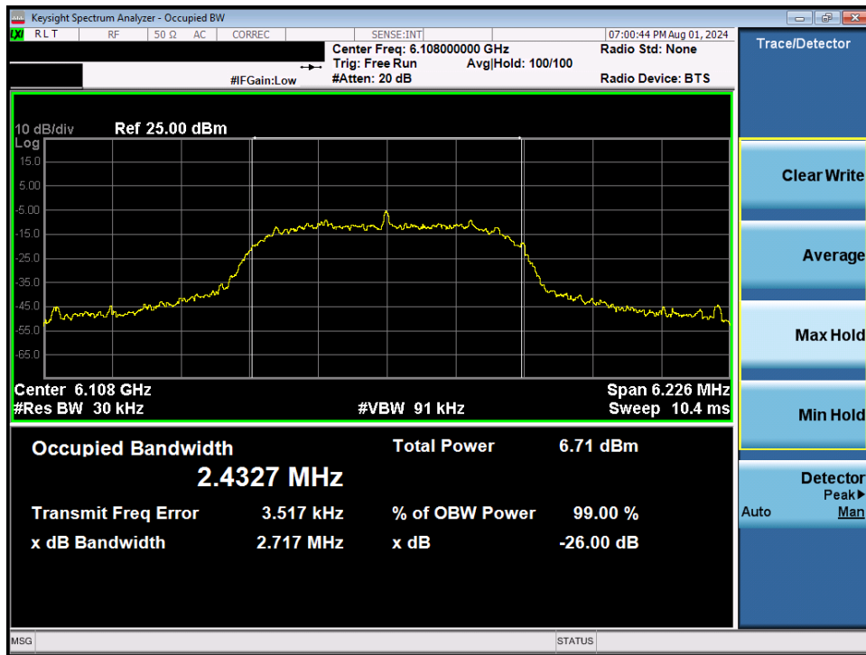
Plot 7-13. 26dB BW & 99% OBW (NB UNII HDRp4 – 6108MHz)
