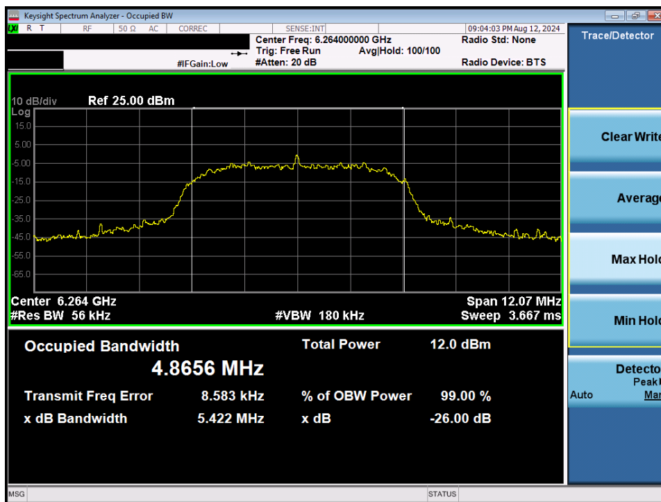
Plot 7-17. 26dB BW & 99% OBW (NB UNII HDRp8 – 6264MHz)
