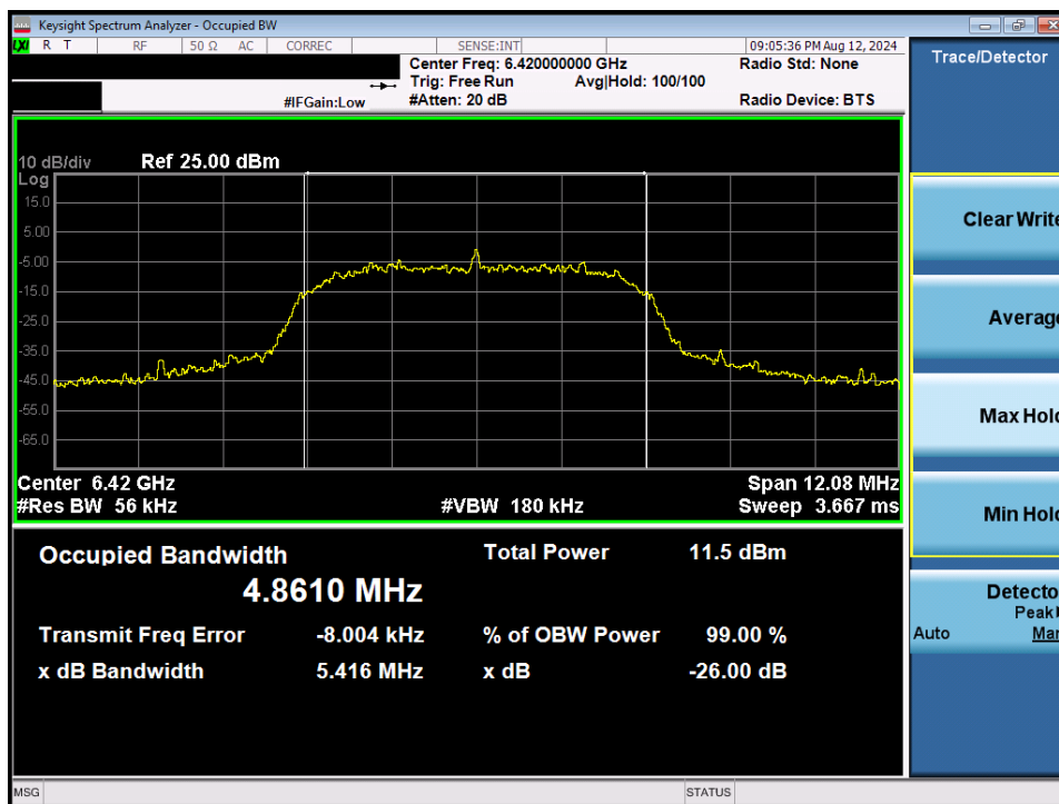
Plot 7-18. 26dB BW & 99% OBW (NB UNII HDRp8 – 6420MHz)
