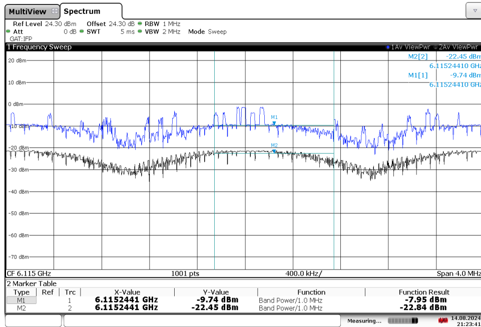
Plot 7-59. Power Spectral Density Plot (NB UNII, 6115MHz)
