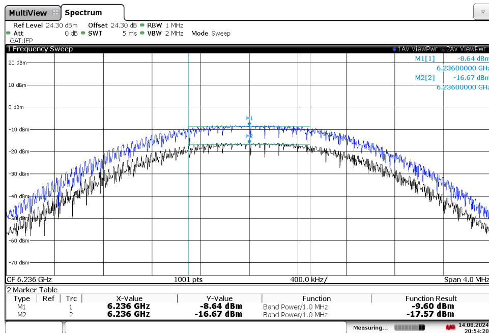
Plot 7-60. Power Spectral Density Plot (NB UNII, 6236MHz)
