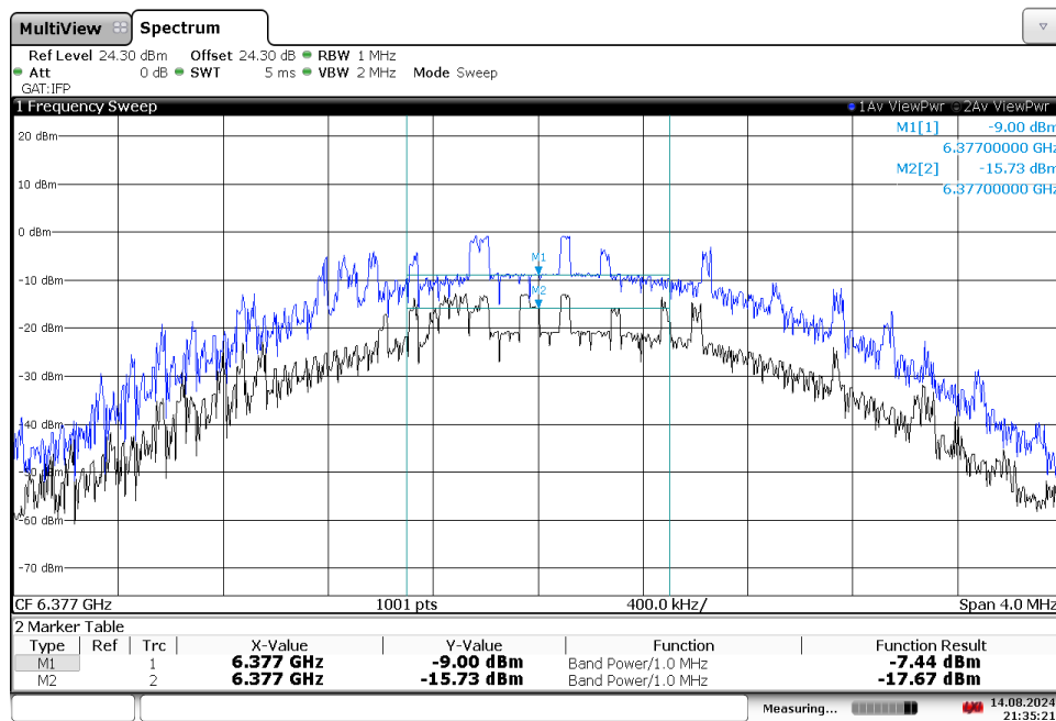
Plot 7-61. Power Spectral Density Plot (NB UNII, 6377MHz)
