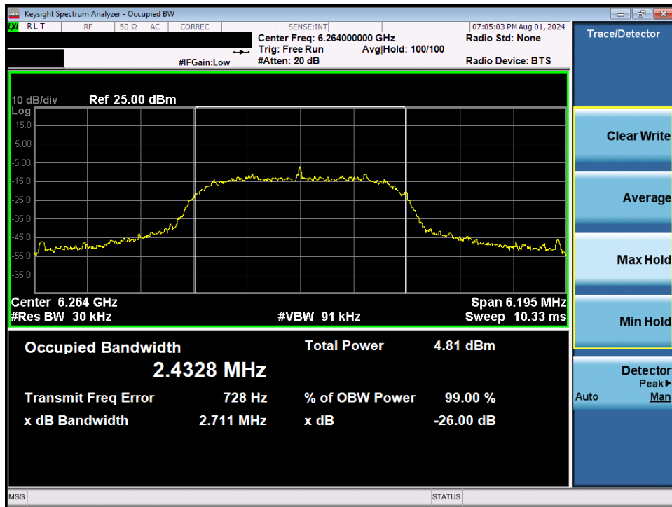
Plot 7-14. 26dB BW & 99% OBW (NB UNII HDRp4 – 6264MHz)
