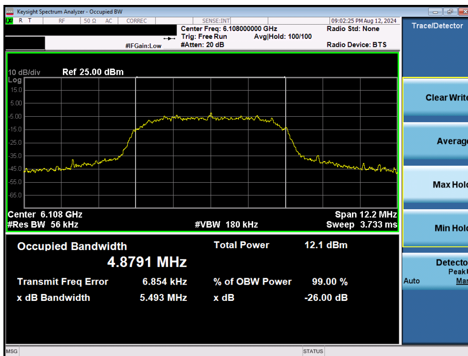
Plot 7-16. 26dB BW & 99% OBW (NB UNII HDRp8 – 6108MHz)
