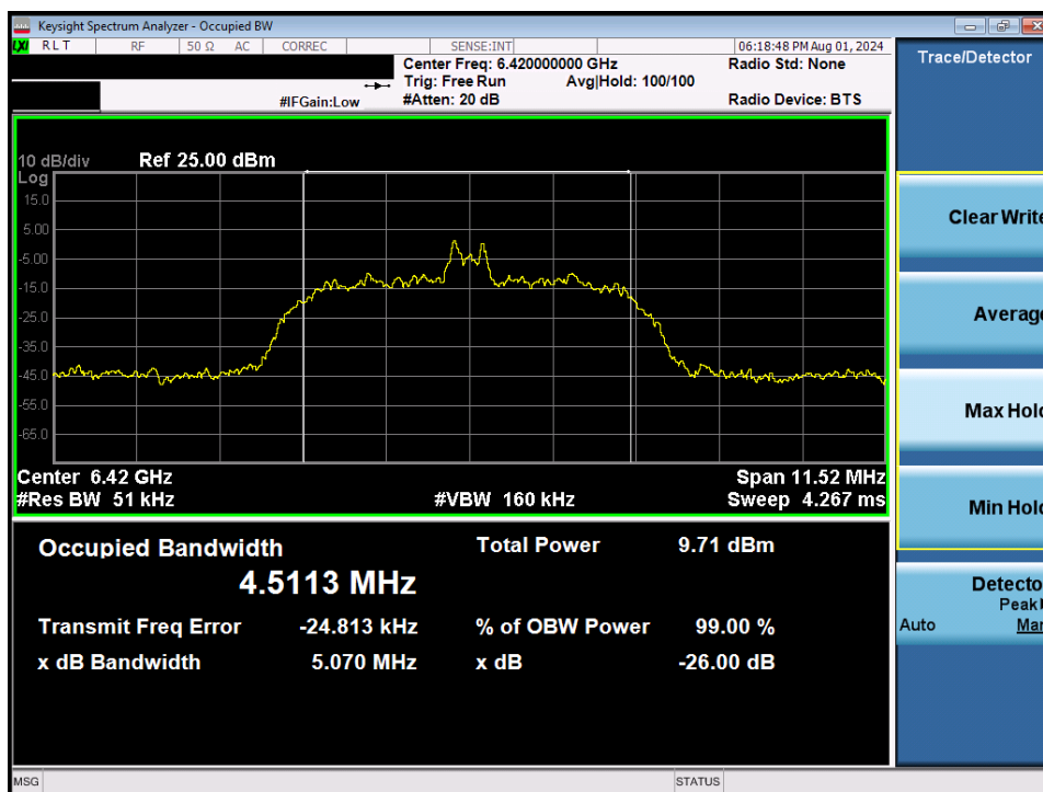
Plot 7-12. 26dB BW & 99% OBW (NB UNII HDR8 – 6420MHz)
