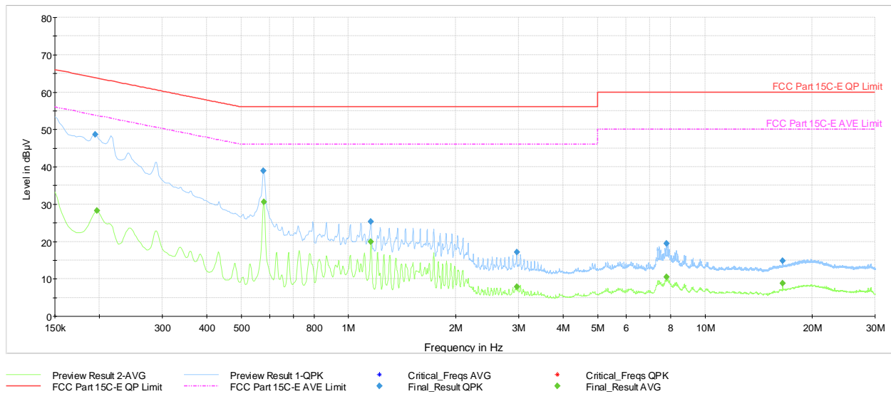
Plot 7-52. AC Line Conducted Plot with Bluetooth HDR (L1, 4Mbps - Ch.38 with host PC and USB-C cable)
