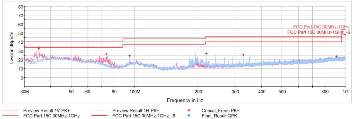
Plot 7-24. RSE 30MHz - 1GHz (LE2M - 5844MHz), with AC/DC Adapter and USB-C cable
