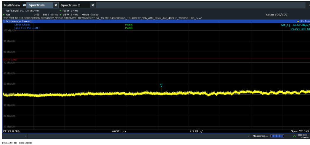
Plot 7-19. Radiated Spurious Emissions Above 18GHz (LE2M – 5844MHz Pol. H)
