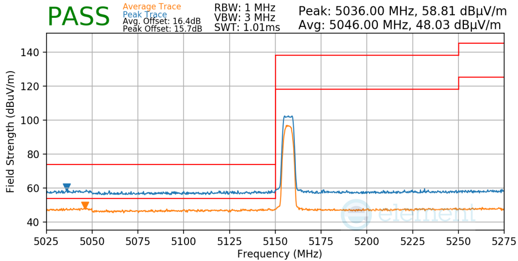
Plot 7-60. Radiated Lower Band Edge Measurement
