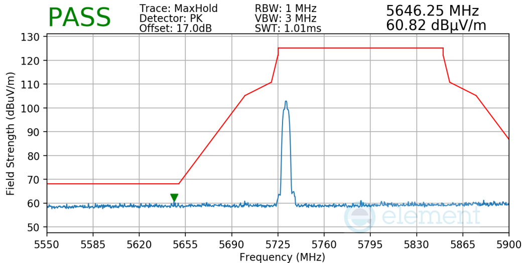
Plot 7-62. Radiated Lower Band Edge Measurement
