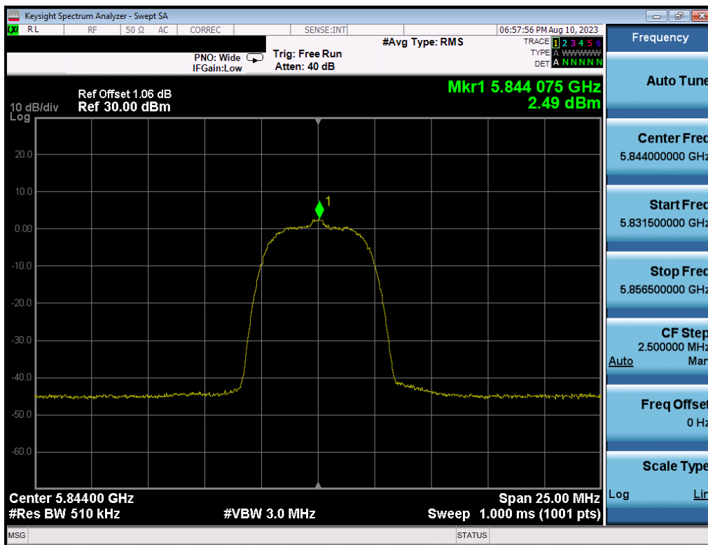
Plot 7-42. PSD (HDR8, 5844MHz)
