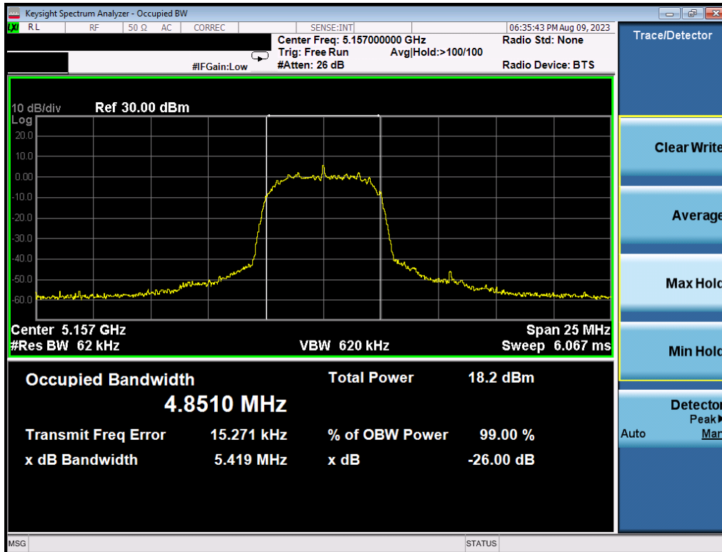
Plot 7-10. 26dB BW & 99% OBW (HDRp8, 5157MHz)
