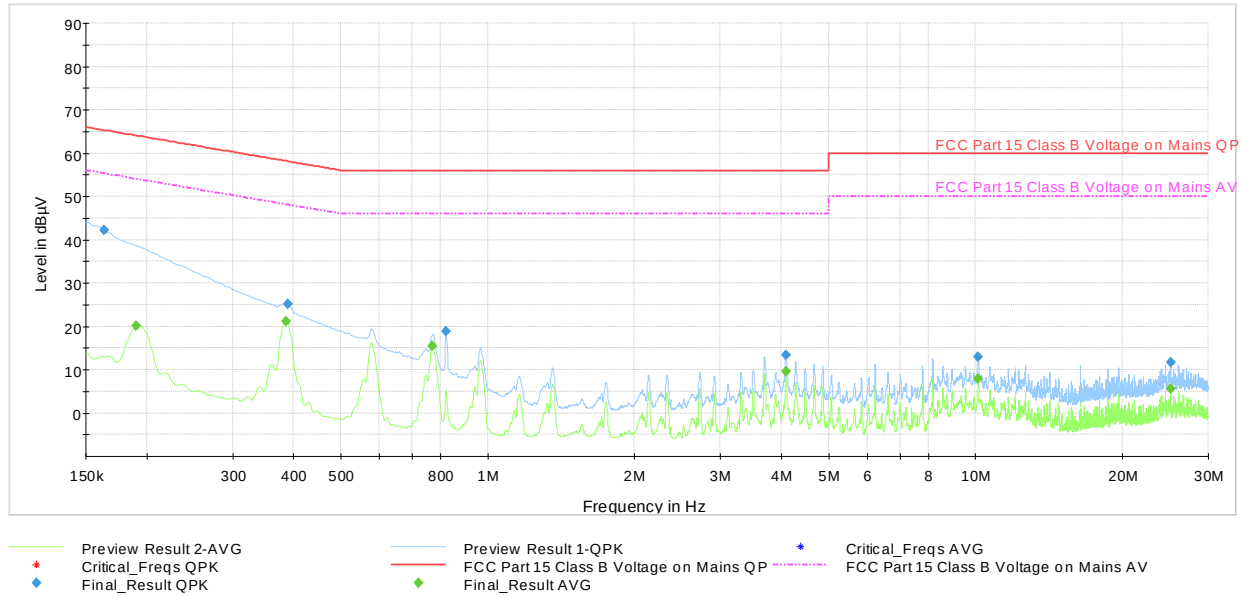
Plot 7-71. AC Line Conducted Plot (HDR4 – 5788MHz) (N) with host PC and USB-C cable
