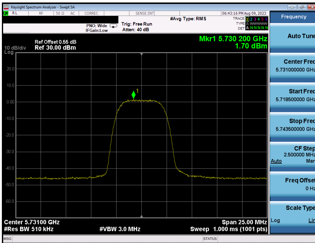
Plot 7-46. PSD (HDRp8, 5731MHz)
