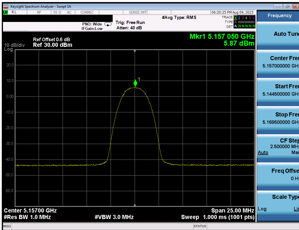
Plot 7-31. PSD (HDRp4, 5157MHz)
