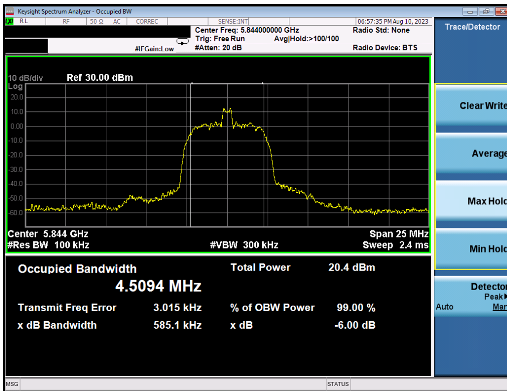
Plot 7-18. 6dB BW & 99% OBW (HDR8, 5844MHz)
