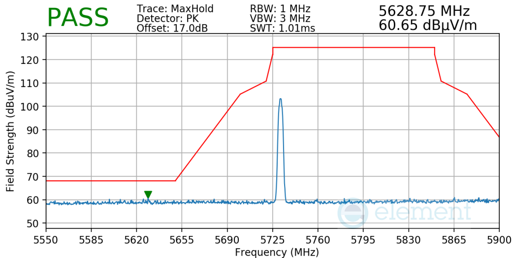
Plot 7-61. Radiated Lower Band Edge Measurement
