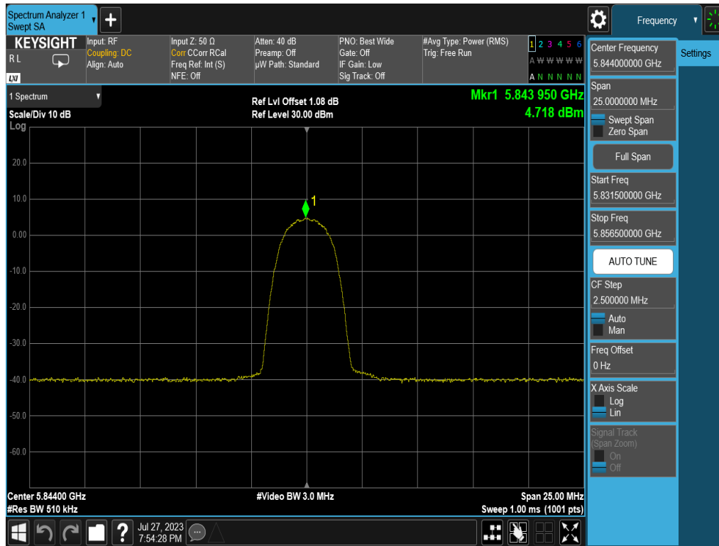
Plot 7-39. PSD (HDR4, 5844MHz)
