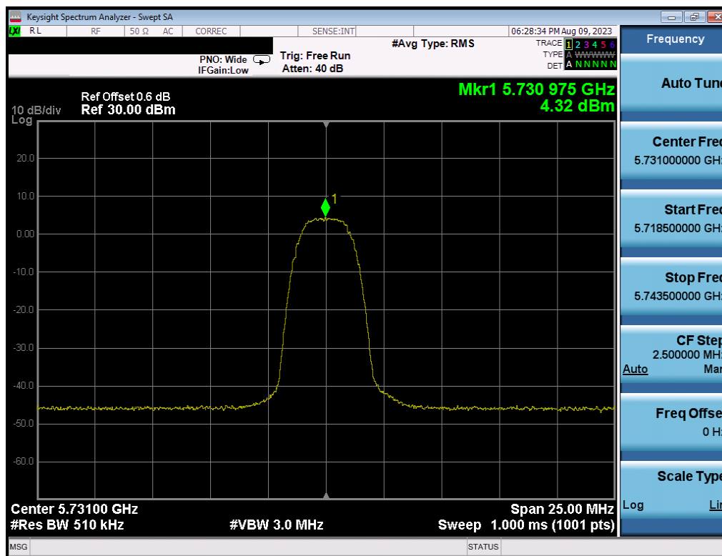
Plot 7-43. PSD (HDRp4, 5731MHz)
