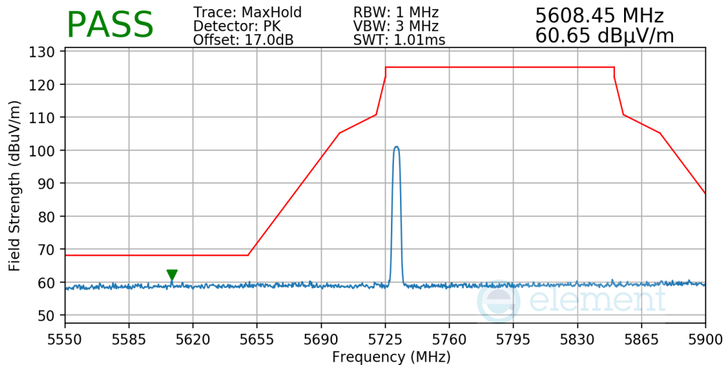
Plot 7-63. Radiated Lower Band Edge Measurement
