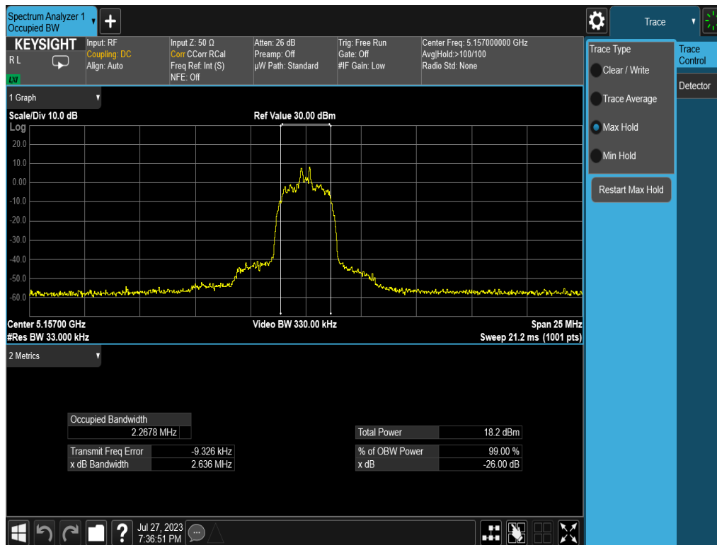
Plot 7-1. 26dB BW & 99% OBW (HDR4, 5157MHz)
