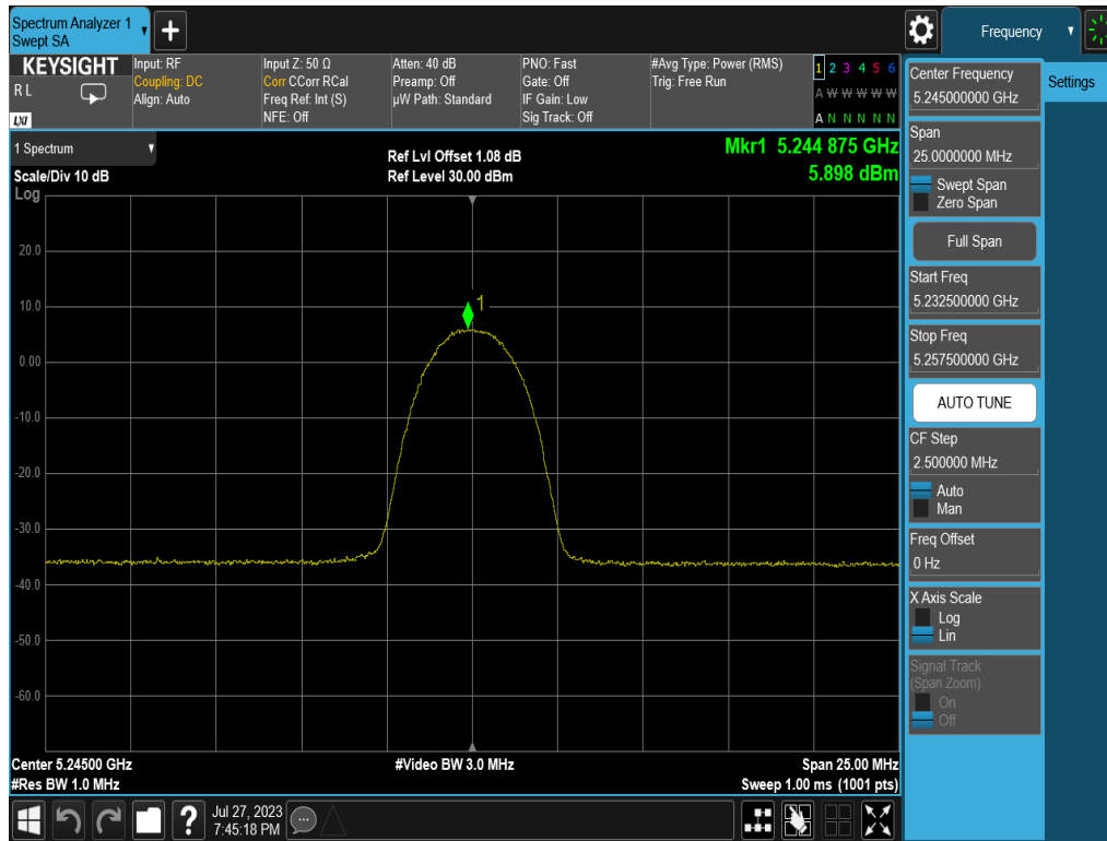
Plot 7-27. PSD (HDR4, 5245MHz)
