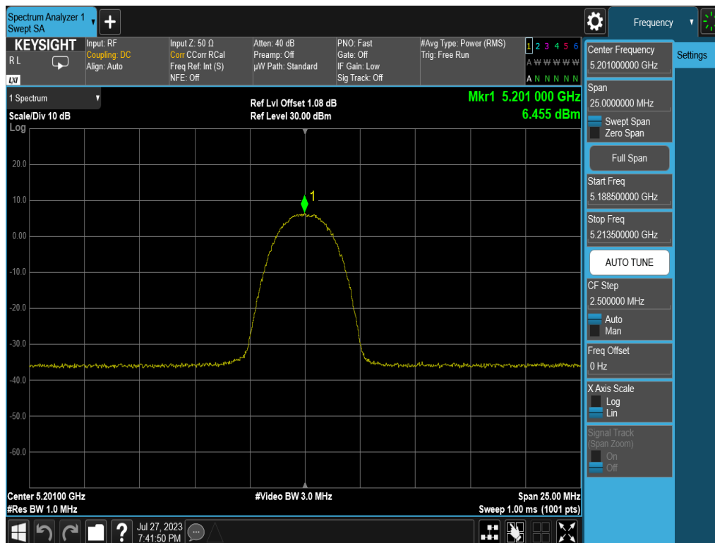
Plot 7-26. PSD (HDR4, 5201MHz)
