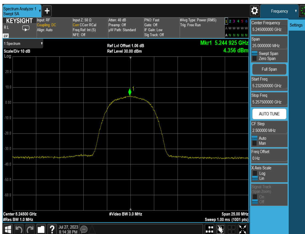
Plot 7-30. PSD (HDR8, 5245MHz)
