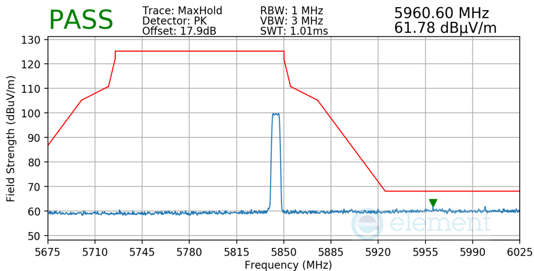
Plot 7-68. Radiated Upper Band Edge Measurement
