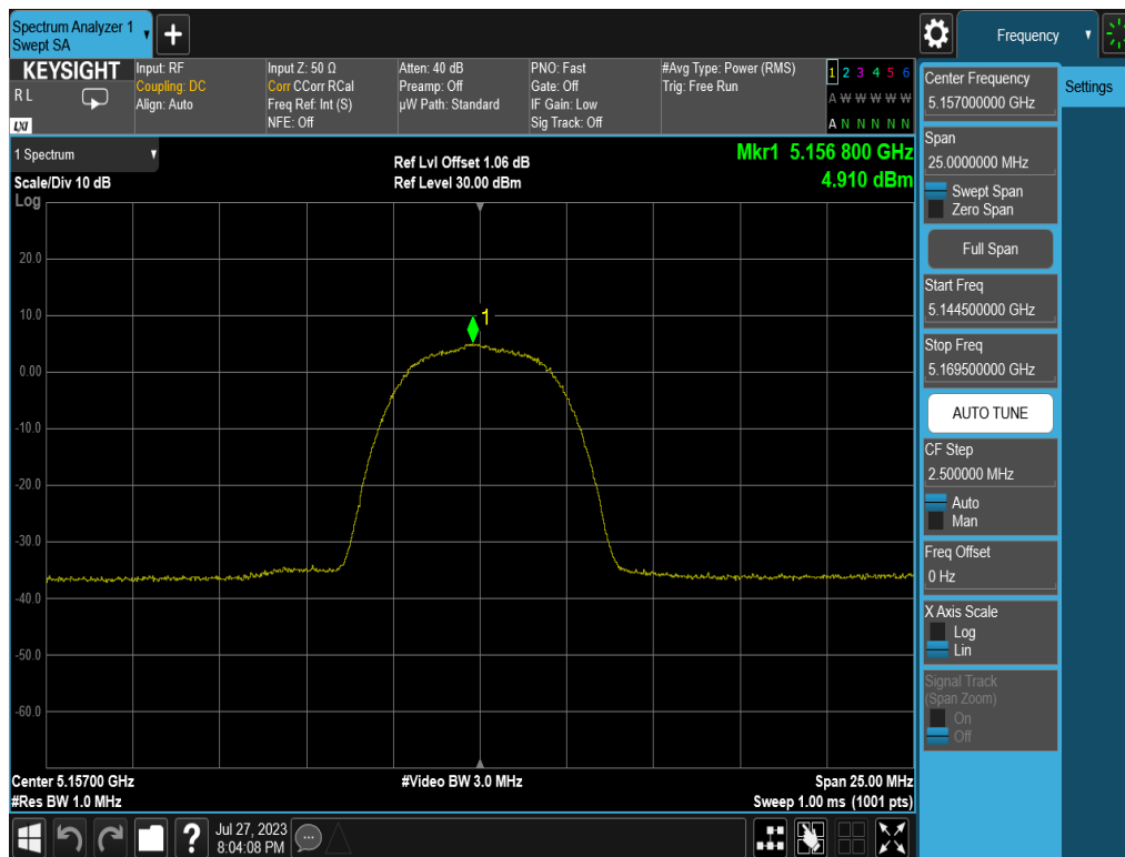
Plot 7-28. PSD (HDR8, 5157MHz)
