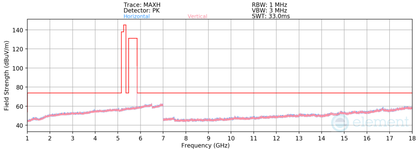
Plot 7-54. Radiated Spurious Emissions 1-18GHz (HDR4 – 5844MHz)
