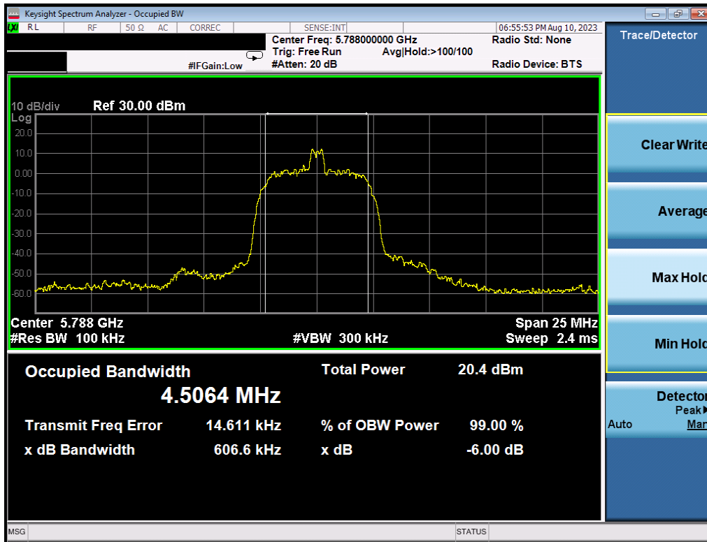
Plot 7-17. 6dB BW & 99% OBW (HDR8, 5788MHz)
