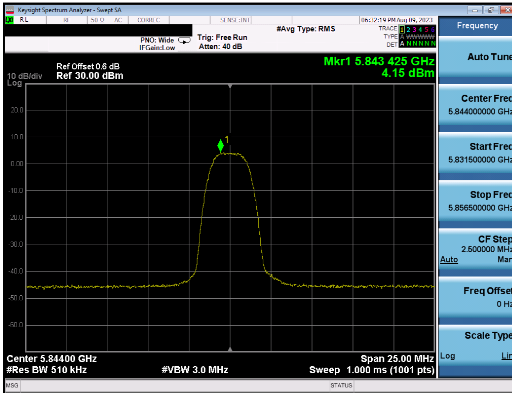
Plot 7-45. PSD (HDRp4, 5844MHz)
