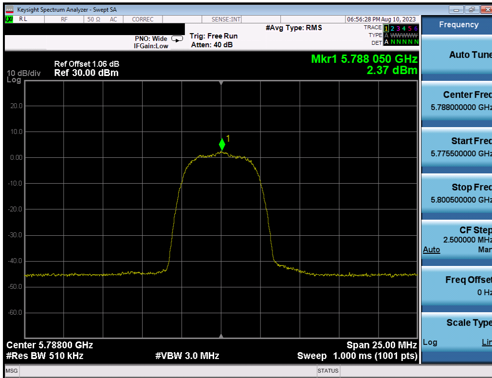
Plot 7-41. PSD (HDR8, 5788MHz)
