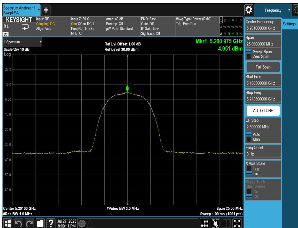
Plot 7-29. PSD (HDR8, 5201MHz)
