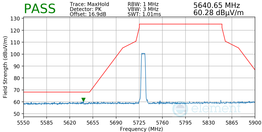
Plot 7-64. Radiated Lower Band Edge Measurement
