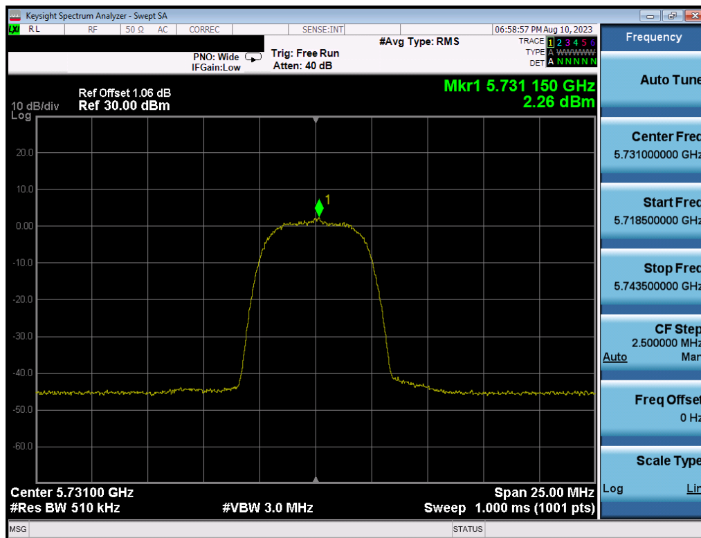
Plot 7-40. PSD (HDR8, 5731MHz)
