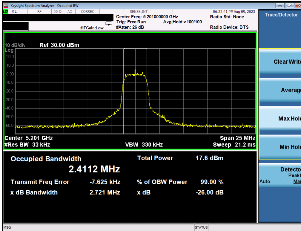
Plot 7-8. 26dB BW & 99% OBW (HDRp4, 5201MHz)
