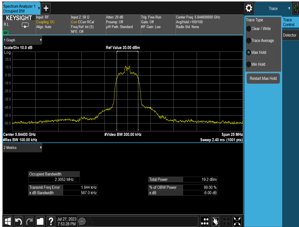
Plot 7-15. 6dB BW & 99% OBW (HDR4, 5844MHz)
