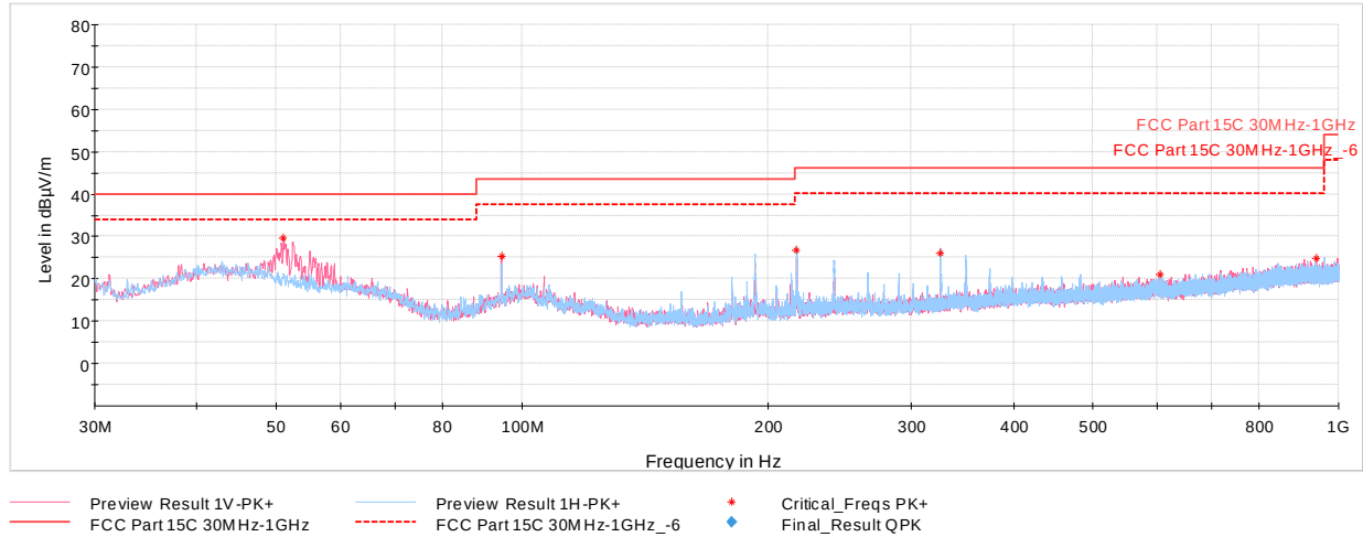
Plot 7-69. Radiated Spurious Emissions 30MHz - 1GHz (HDR4 – 5788MHz), with AC/DC Adapter and USB-C cable
