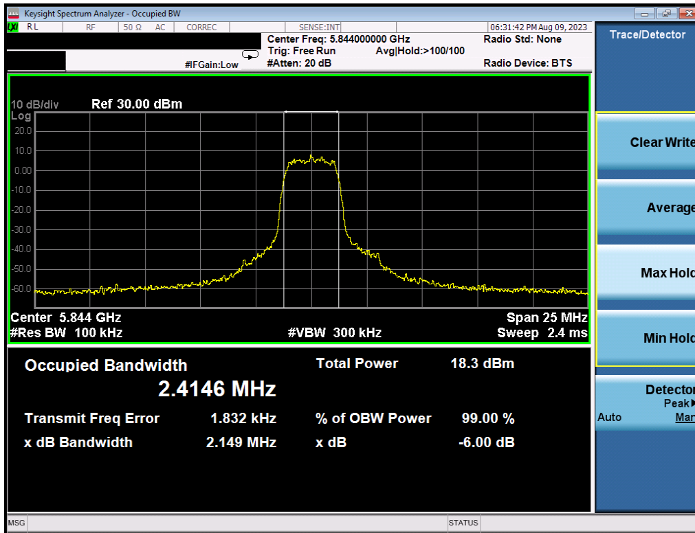
Plot 7-21. 6dB BW & 99% OBW (HDRp4, 5844MHz)
