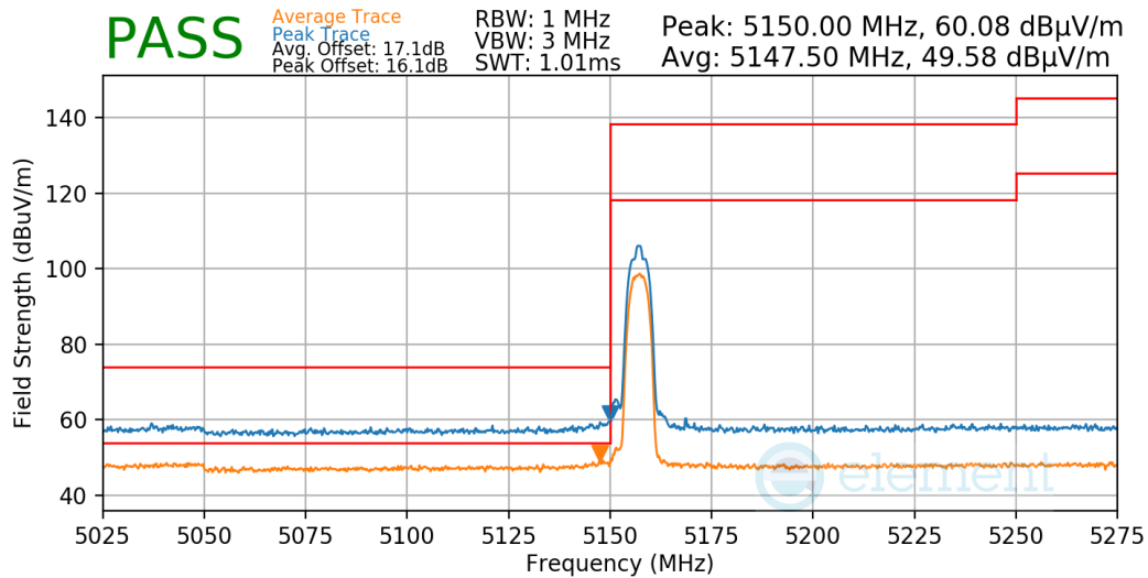
Plot 7-58. Radiated Lower Band Edge Measurement
