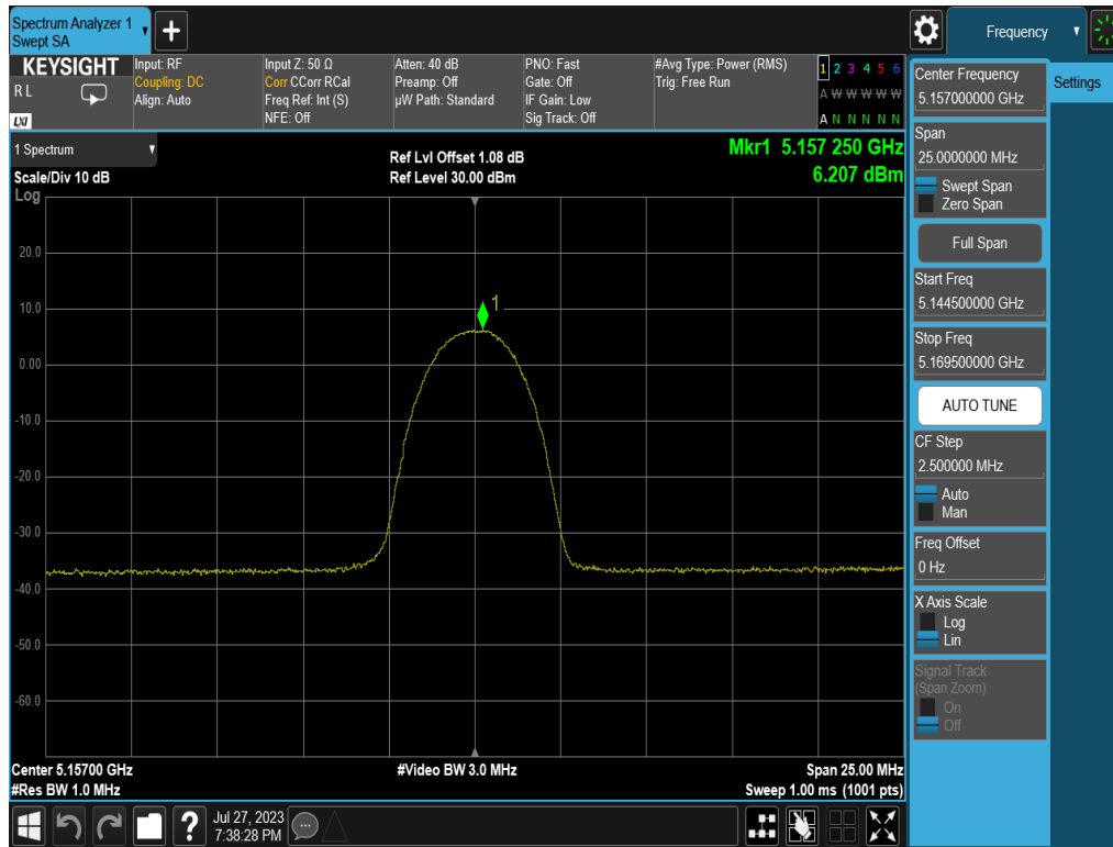
Plot 7-25. PSD (HDR4, 5157MHz)
