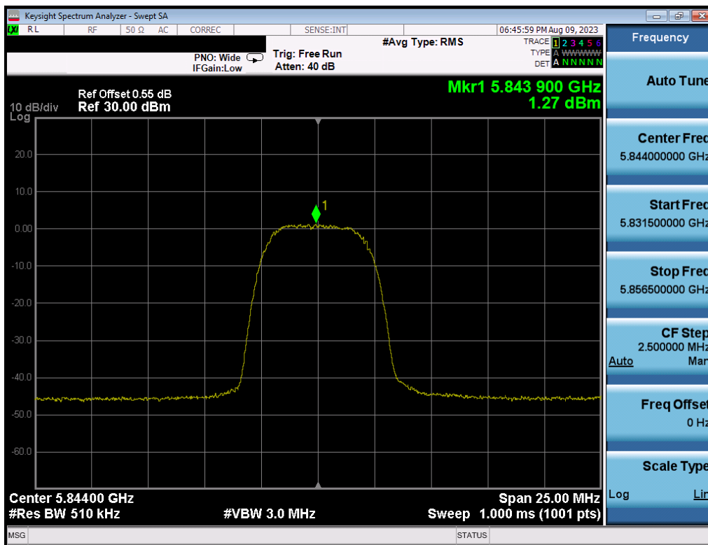
Plot 7-48. PSD (HDRp8, 5844MHz)
