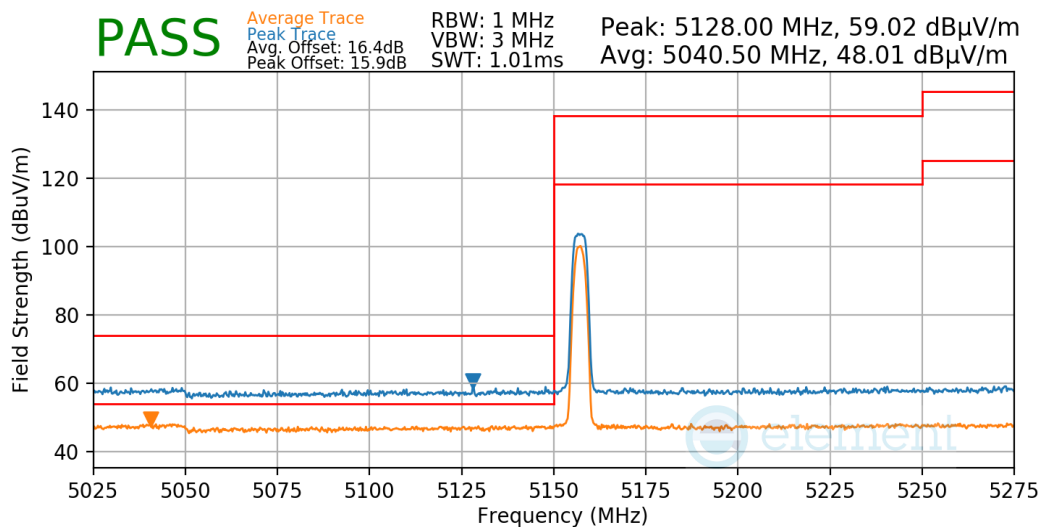
Plot 7-59. Radiated Lower Band Edge Measurement
