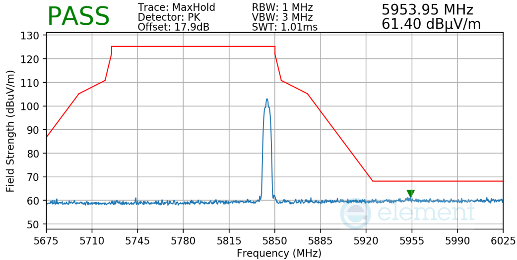
Plot 7-66. Radiated Upper Band Edge Measurement
