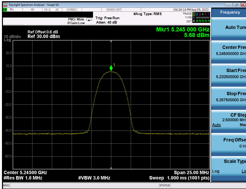
Plot 7-33. PSD (HDRp4, 5245MHz)
