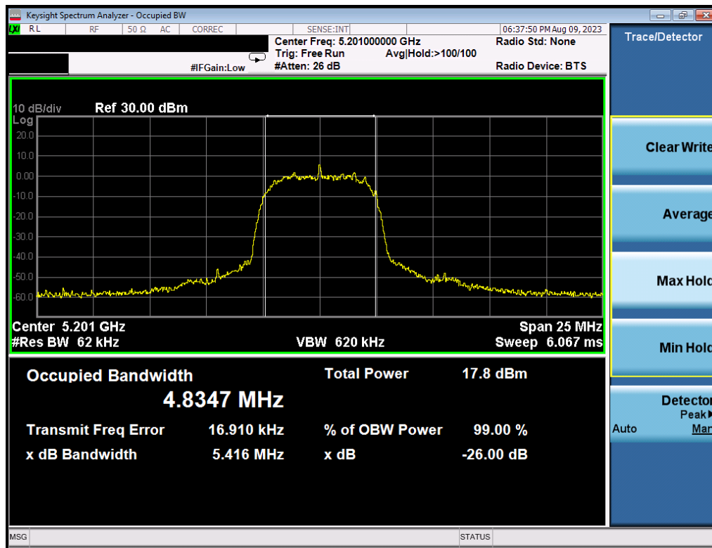
Plot 7-11. 26dB BW & 99% OBW (HDRp8, 5201MHz)
