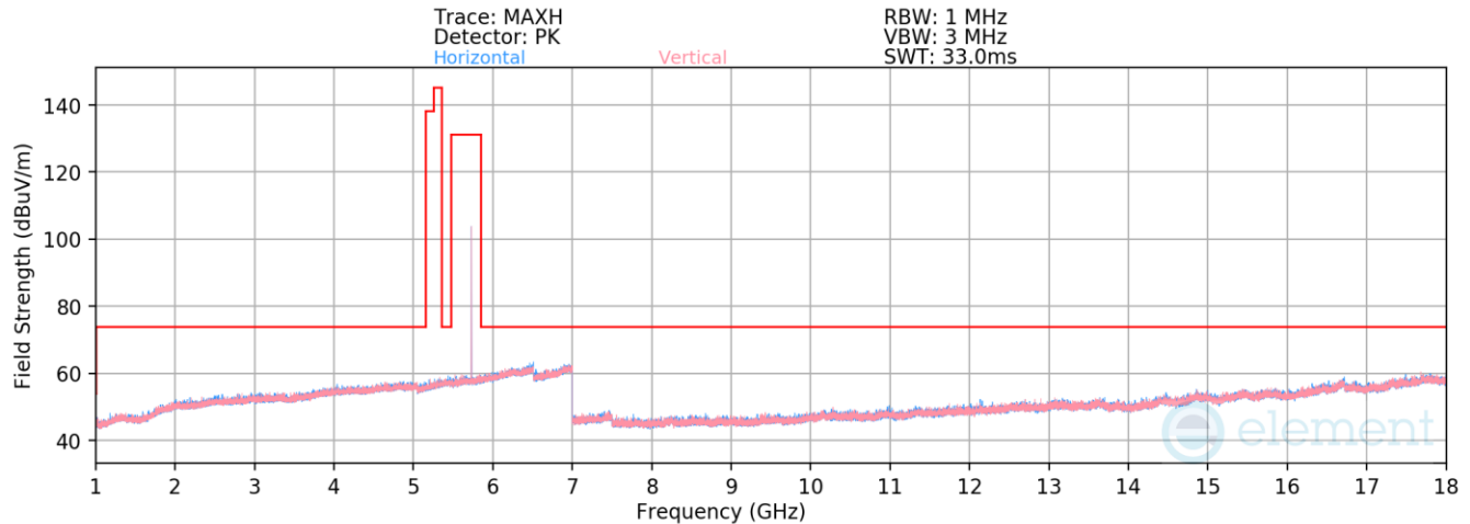
Plot 7-52. Radiated Spurious Emissions 1-18GHz (HDR4 – 5731MHz)
