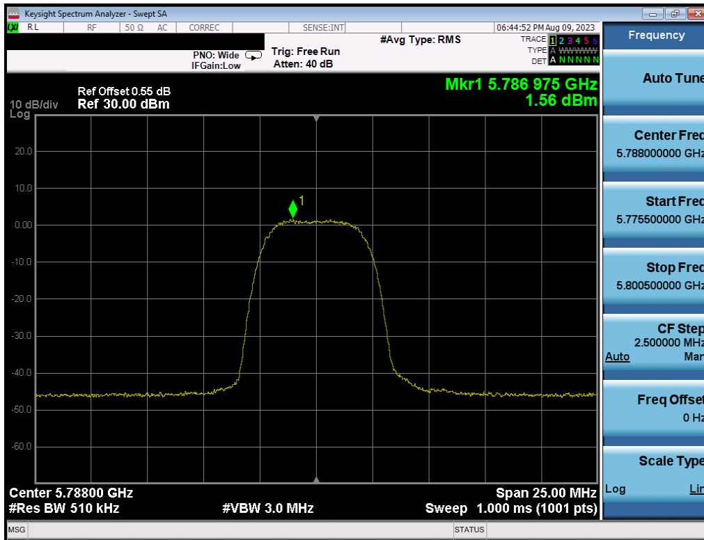
Plot 7-47. PSD (HDRp8, 5788MHz)
