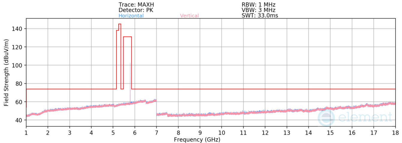
Plot 7-53. Radiated Spurious Emissions 1-18GHz (HDR4 – 5788MHz)
