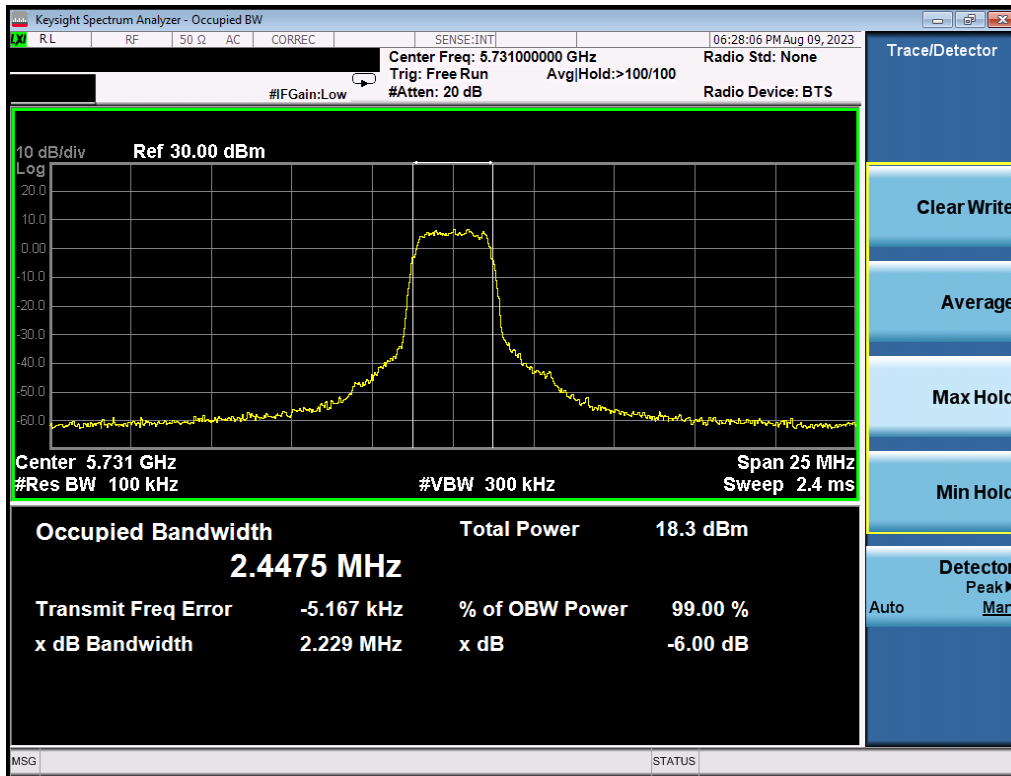
Plot 7-19. 6dB BW & 99% OBW (HDRp4, 5731MHz)
