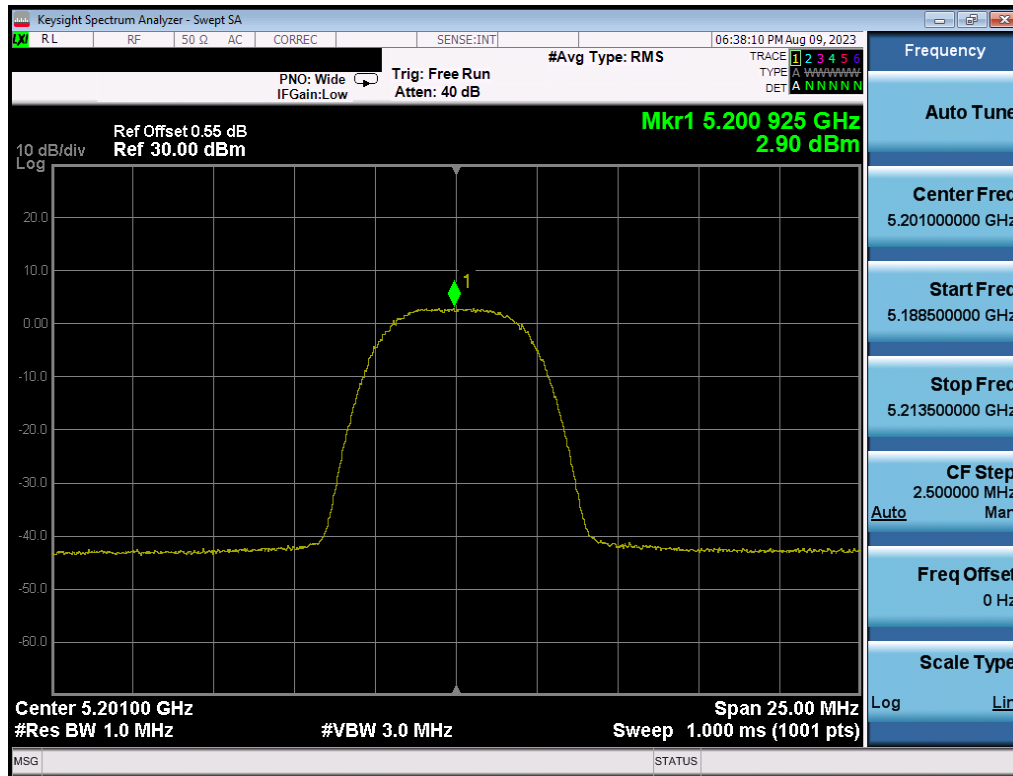
Plot 7-35. PSD (HDRp8, 5201MHz)
