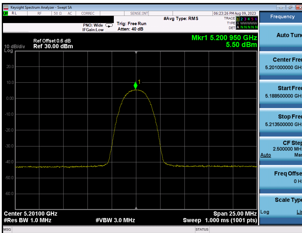
Plot 7-32. PSD (HDRp4, 5201MHz)
