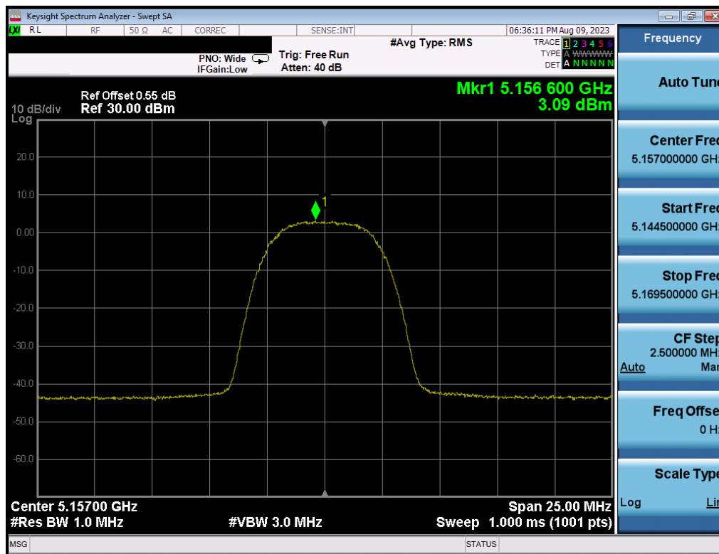
Plot 7-34. PSD (HDRp8, 5157MHz)
