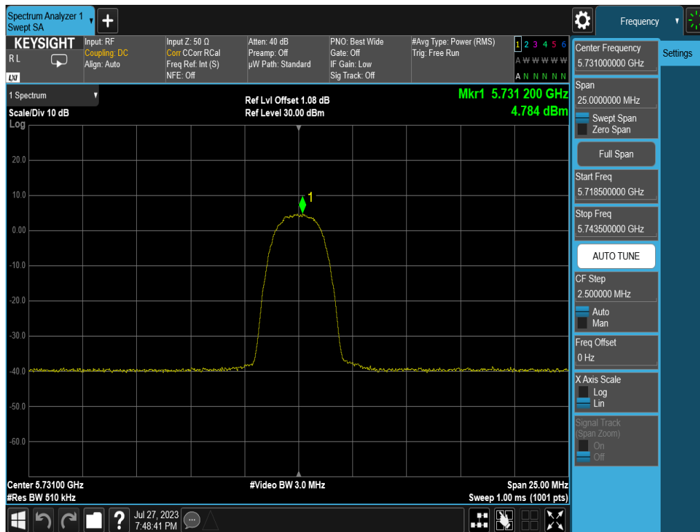
Plot 7-37. PSD (HDR4, 5731MHz)
