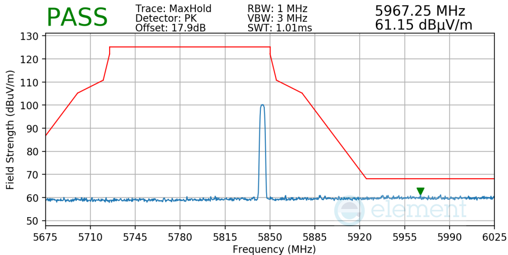
Plot 7-67. Radiated Upper Band Edge Measurement
