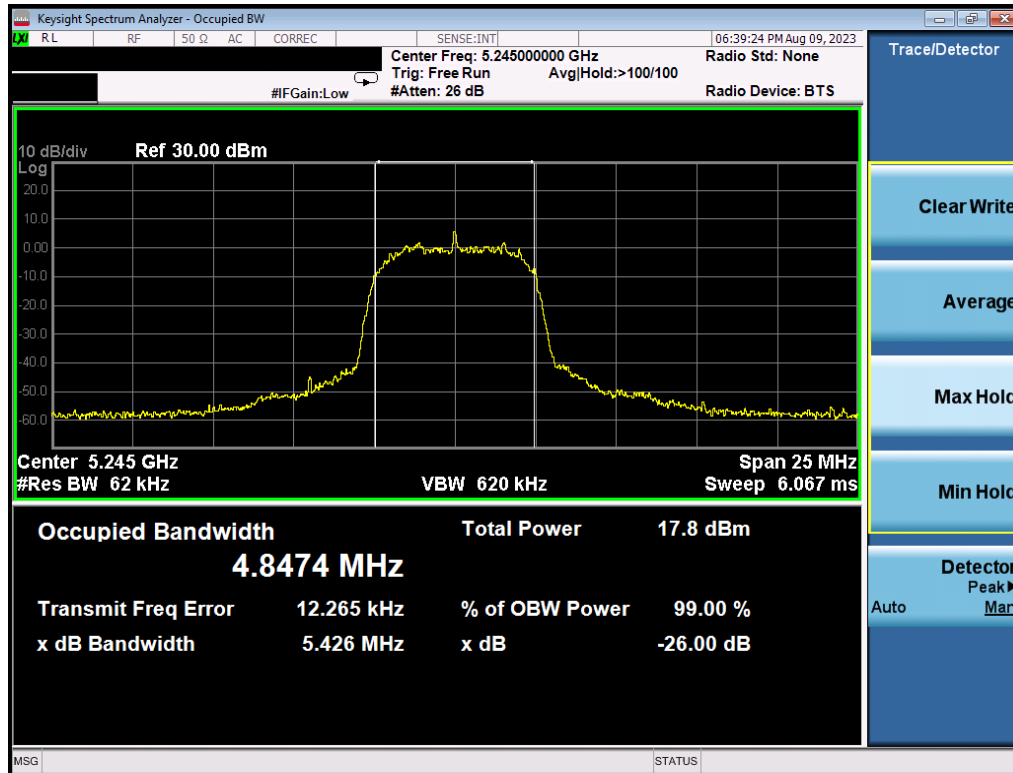
Plot 7-12. 26dB BW & 99% OBW (HDRp8, 5245MHz)
