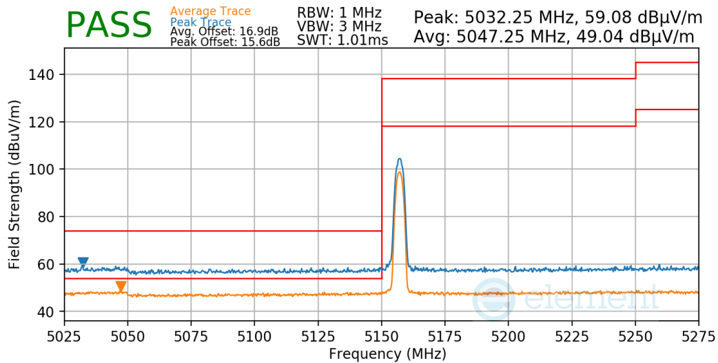
Plot 7-57. Radiated Lower Band Edge Measurement
