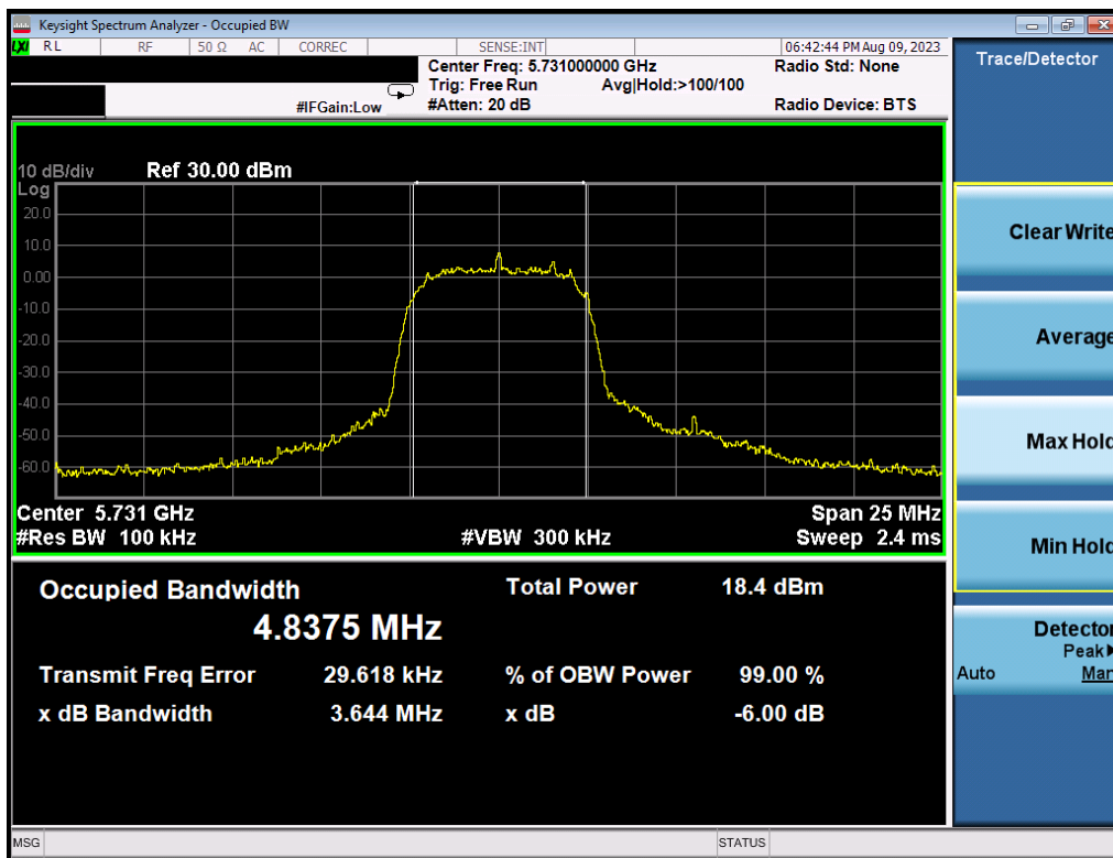
Plot 7-22. 6dB BW & 99% OBW (HDRp8, 5731MHz)
