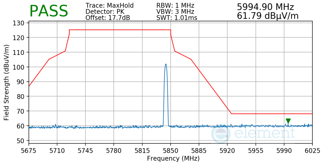
Plot 7-65. Radiated Upper Band Edge Measurement
