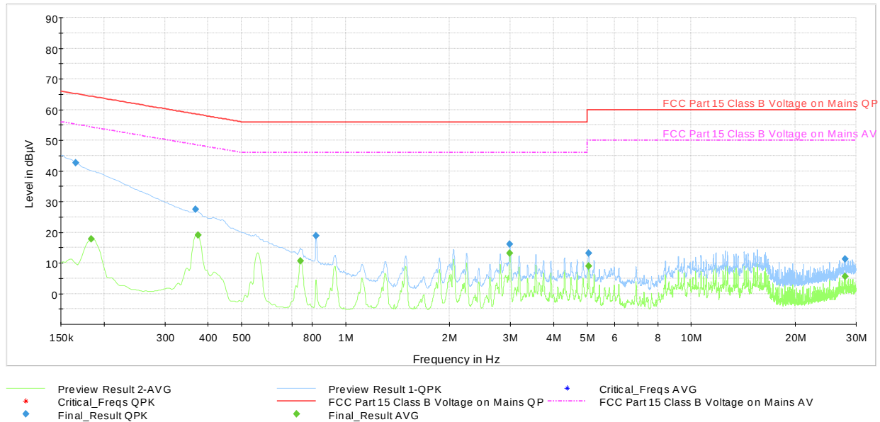
Plot 7-70. AC Line Conducted Plot (HDR4 – 5788MHz) (L1) with host PC and USB-C cable
