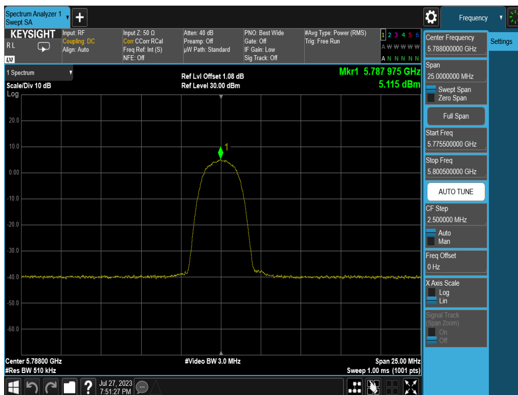
Plot 7-38. PSD (HDR4, 5788MHz)
