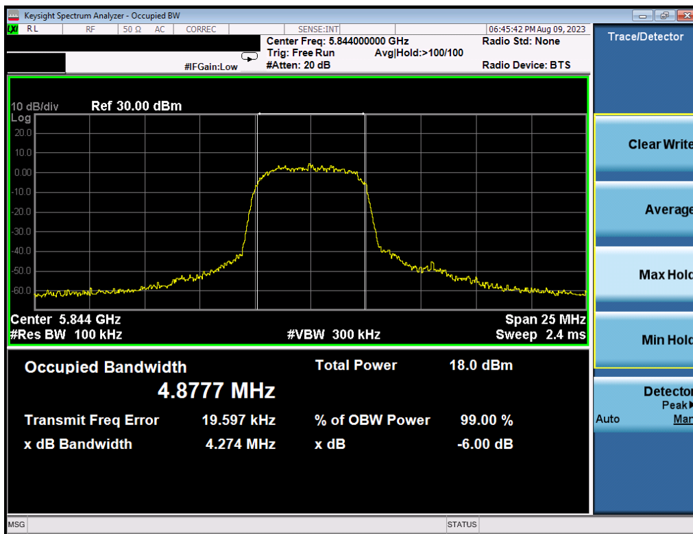
Plot 7-24. 6dB BW & 99% OBW (HDRp8, 5844MHz)
