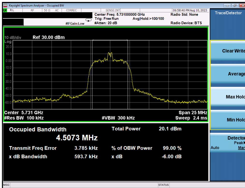
Plot 7-16. 6dB BW & 99% OBW (HDR8, 5731MHz)
