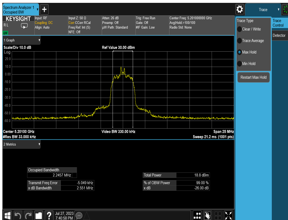
Plot 7-2. 26dB BW & 99% OBW (HDR4, 5201MHz)
