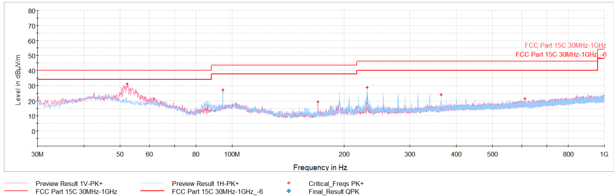
Plot 7-24. RSE 30MHz - 1GHz (BDR - 5844MHz), with AC/DC Adapter and USB-C Cable
