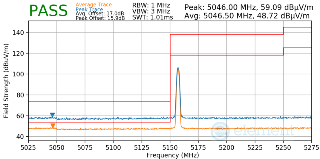
Plot 7-21. Radiated Lower Band Edge Measurement
