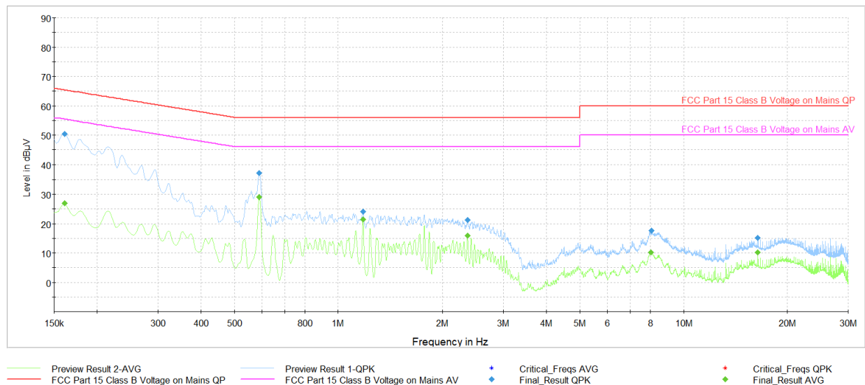
Plot 7-26. AC Line Conducted Plot (BDR – 5844MHz) (N) with host PC and USB-C Cable
