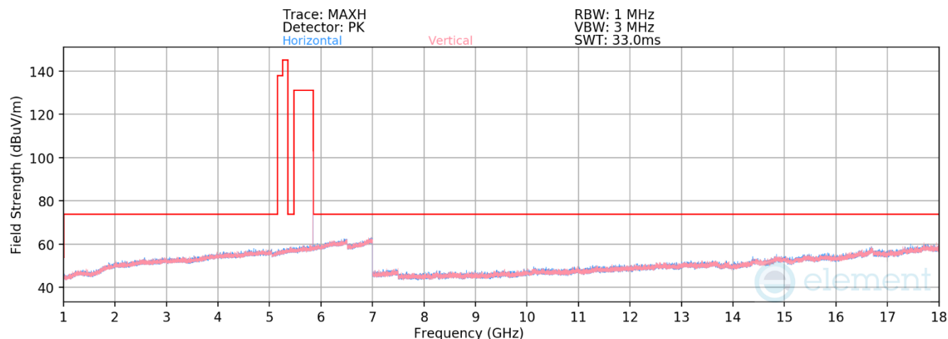
Plot 7-18. Radiated Spurious Emissions 1-18GHz (BDR – 5844MHz)
