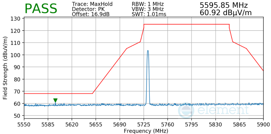
Plot 7-22. Radiated Lower Band Edge Measurement
