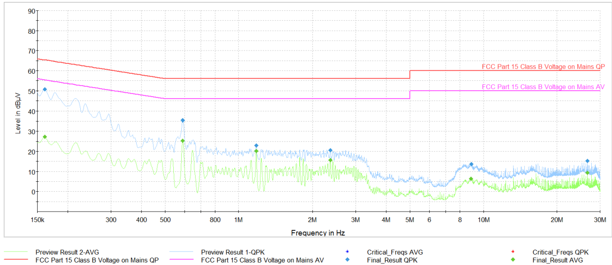
Plot 7-25. AC Line Conducted Plot (BDR – 5844MHz) (L1) with host PC and USB-C Cable
