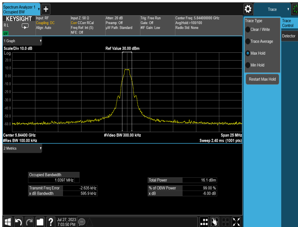
Plot 7-6. 6dB BW & 99% OBW (BDR, 5844MHz)
