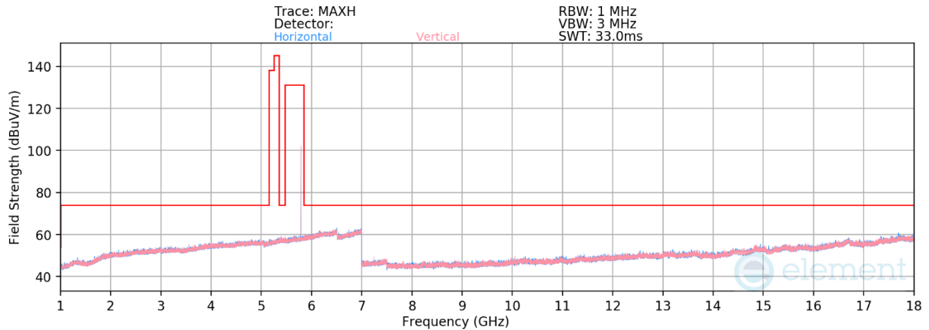
Plot 7-17. Radiated Spurious Emissions 1-18GHz (BDR – 5788MHz)
