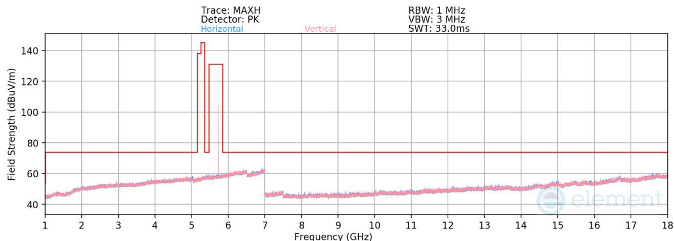
Plot 7-16. Radiated Spurious Emissions 1-18GHz (BDR – 5731MHz)
