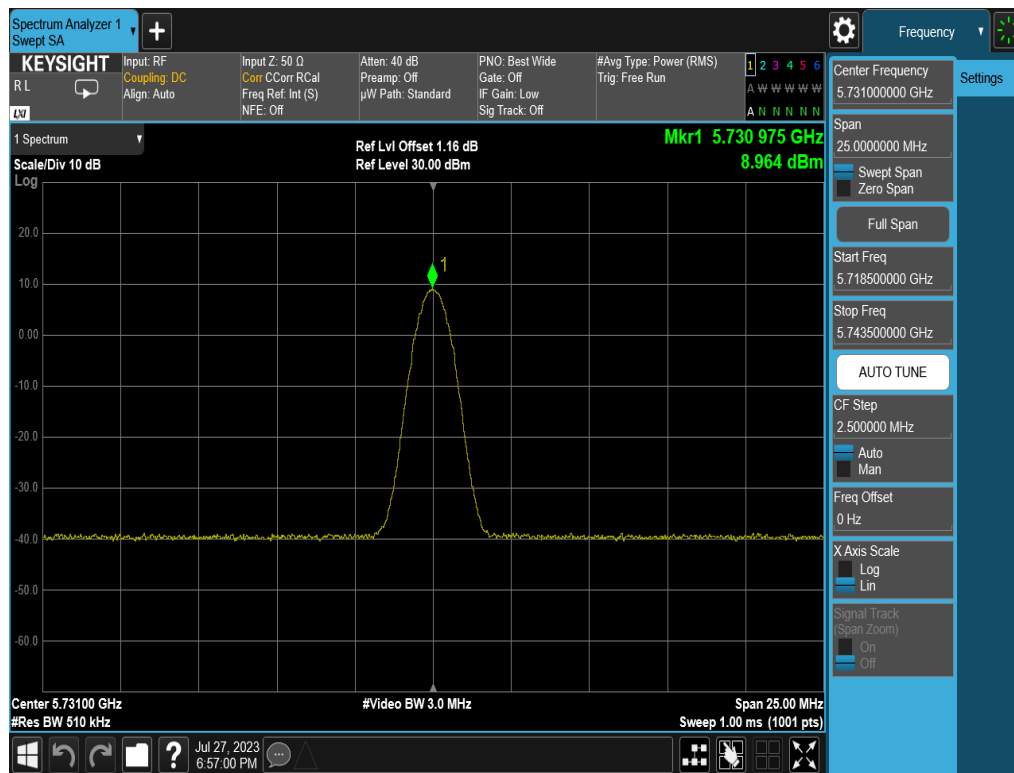
Plot 7-10. PSD (BDR, 5731MHz)
