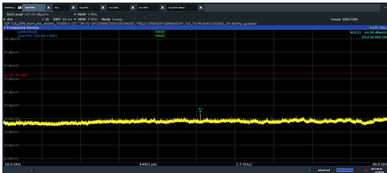
Plot 7-19. Radiated Spurious Emissions Above 18GHz (BDR – 5844MHz Pol. H)
