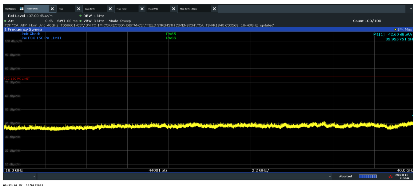
Plot 7-26. Radiated Spurious Emissions Above 18GHz H Polarity (1Mbps – Ch. 39)
