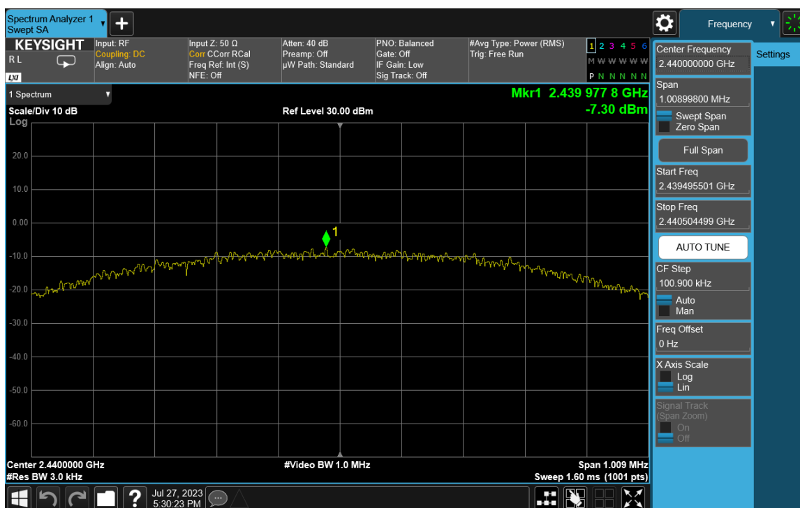
Plot 7-8. Power Spectral Density Plot (Bluetooth (LE), 1Mbps – Ch. 19)
