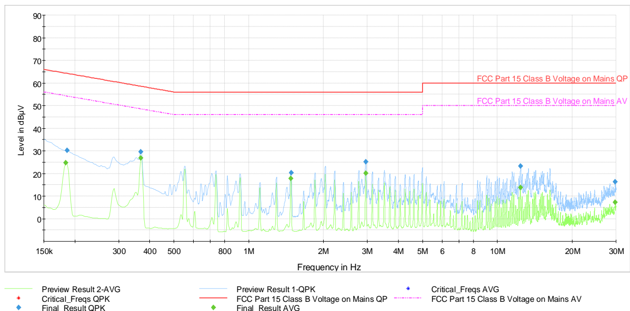
Plot 7-37. AC Line Conducted Plot with Bluetooth LE (L1, 1Mbps – Ch.39 with Laptop)
