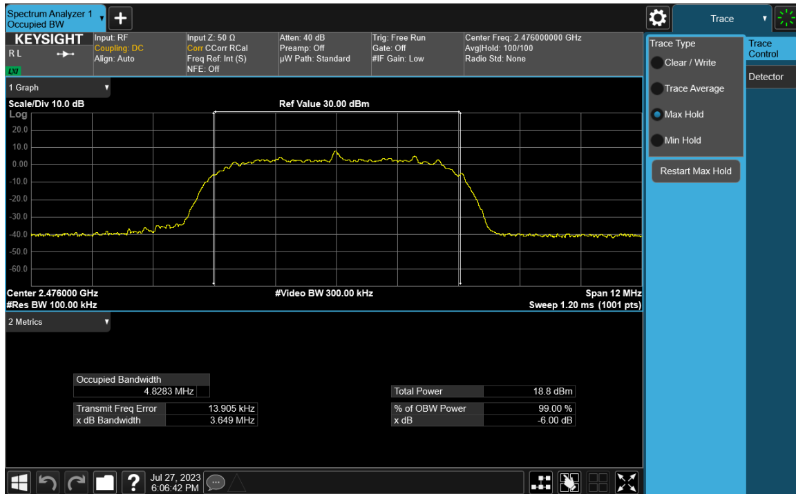
Plot 7-12. 6dB BW & 99% OBW Plot (Bluetooth (HDRp8), 8Mbps – Ch. 73)
