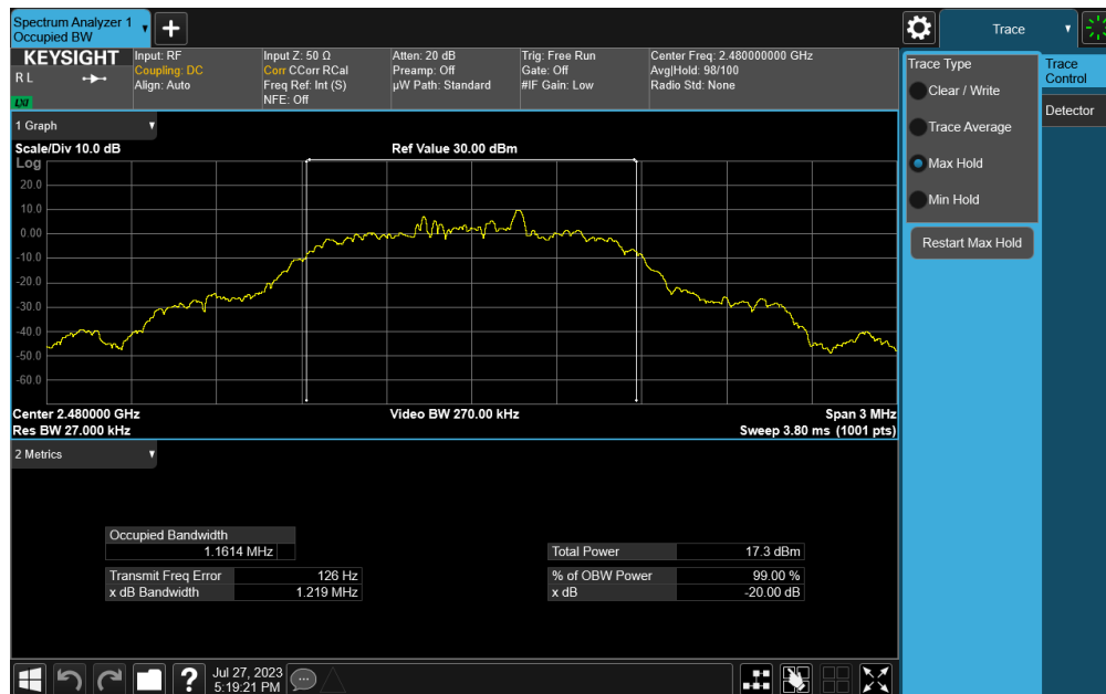
Plot 7-6. 20dB BW and 99% OBW Plot (Bluetooth, 8DPSK – Ch. 78)
