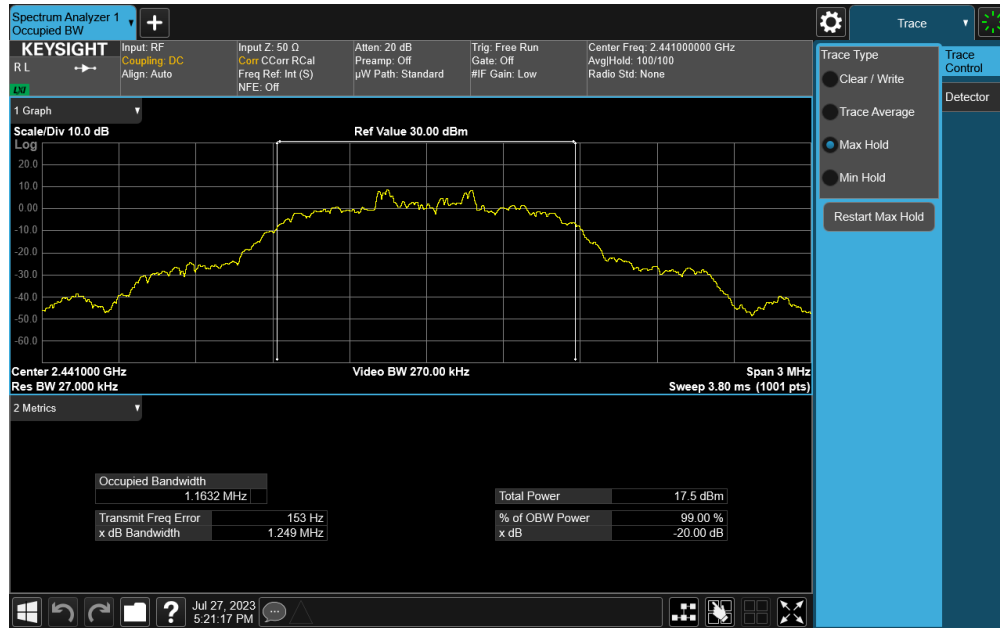
Plot 7-5. 20dB BW and 99% OBW Plot (Bluetooth, 8DPSK – Ch. 39)
