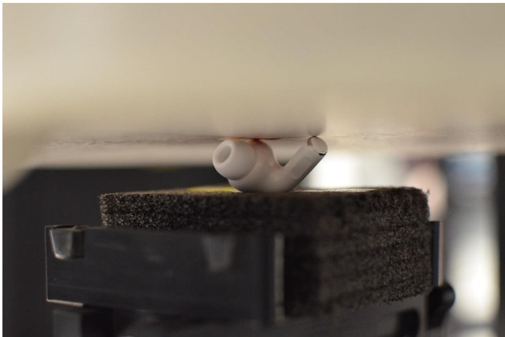
SAR Test Setup Photo 1: Head, Right Earbud, 0 mm
