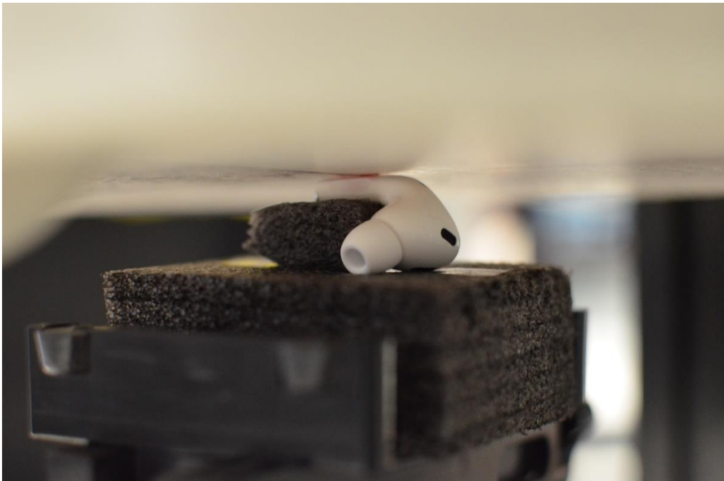
SAR Test Setup Photo 3: Body-Worn, Back Side, 0 mm
