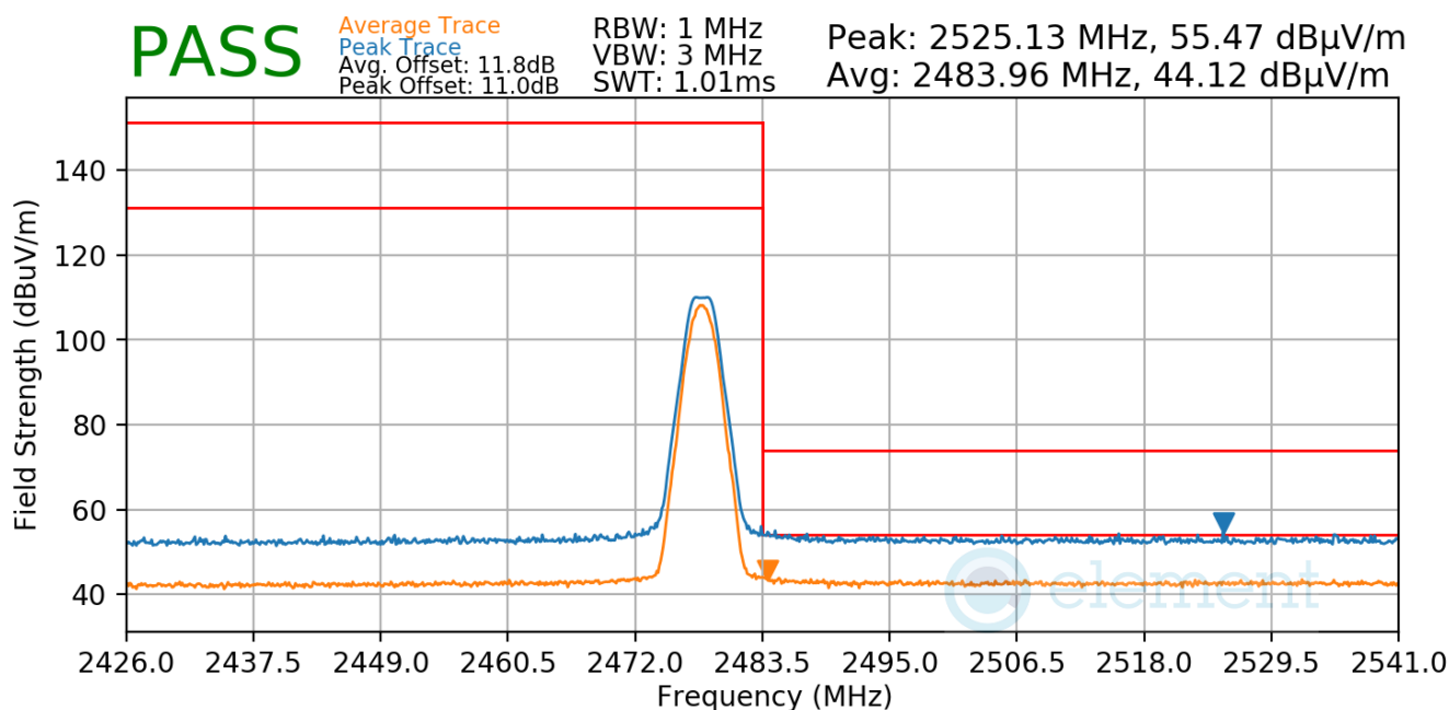
Plot 7-34. Radiated Restricted Upper Band Edge Measurement (Average & Peak)
