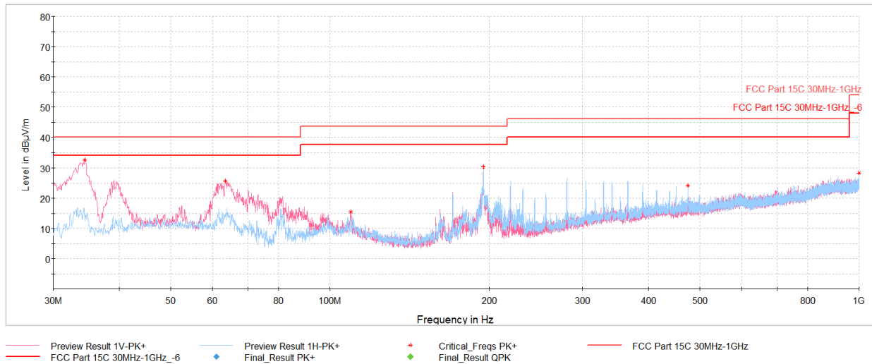
Plot 7-36. Co-Tx Radiated Spurious Emissions Below 1GHz with AC/DC Adapter and USB-C cable
