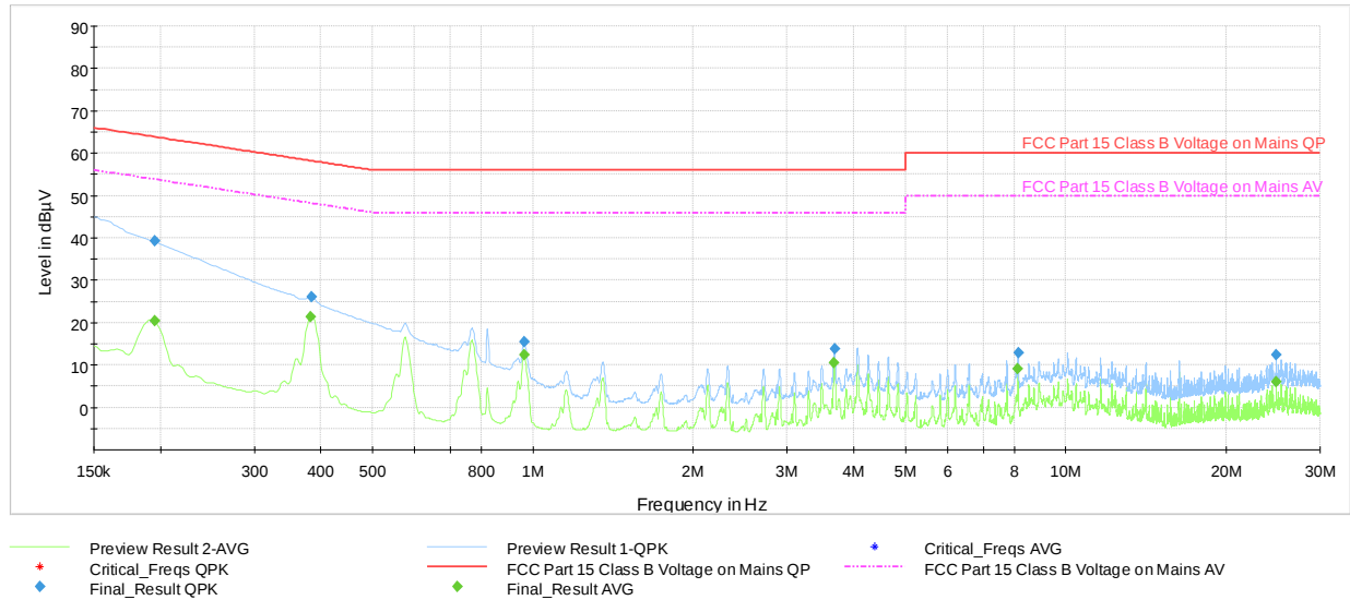
Plot 7-38. AC Line Conducted Plot with Bluetooth LE (N, 1Mbps – Ch.19, with host PC and USB-C cable)
