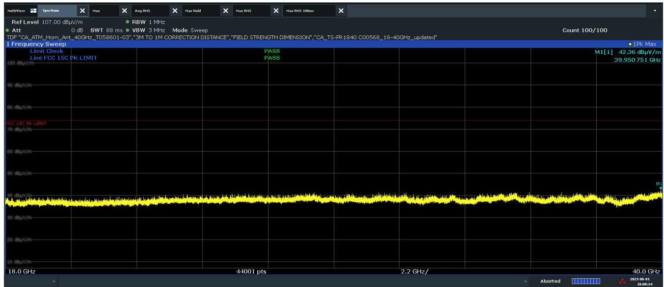
Plot 7-26. Radiated Spurious Emissions Above 18GHz H Polarity (1Mbps – Ch. 19)
