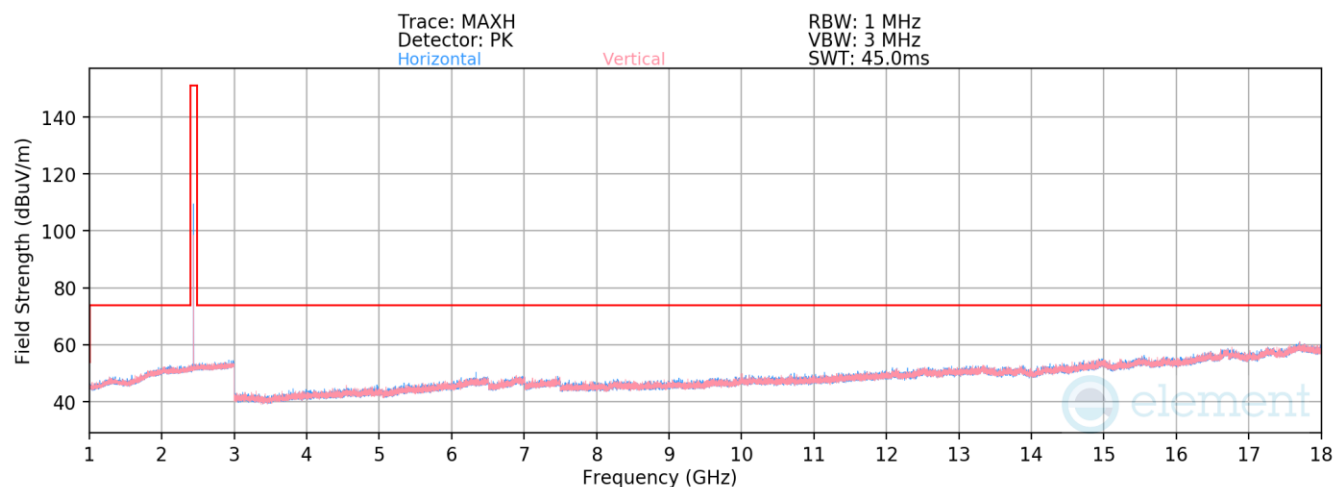
Plot 7-24. Radiated Spurious Emissions 1-18GHz (1Mbps – Ch. 19)
