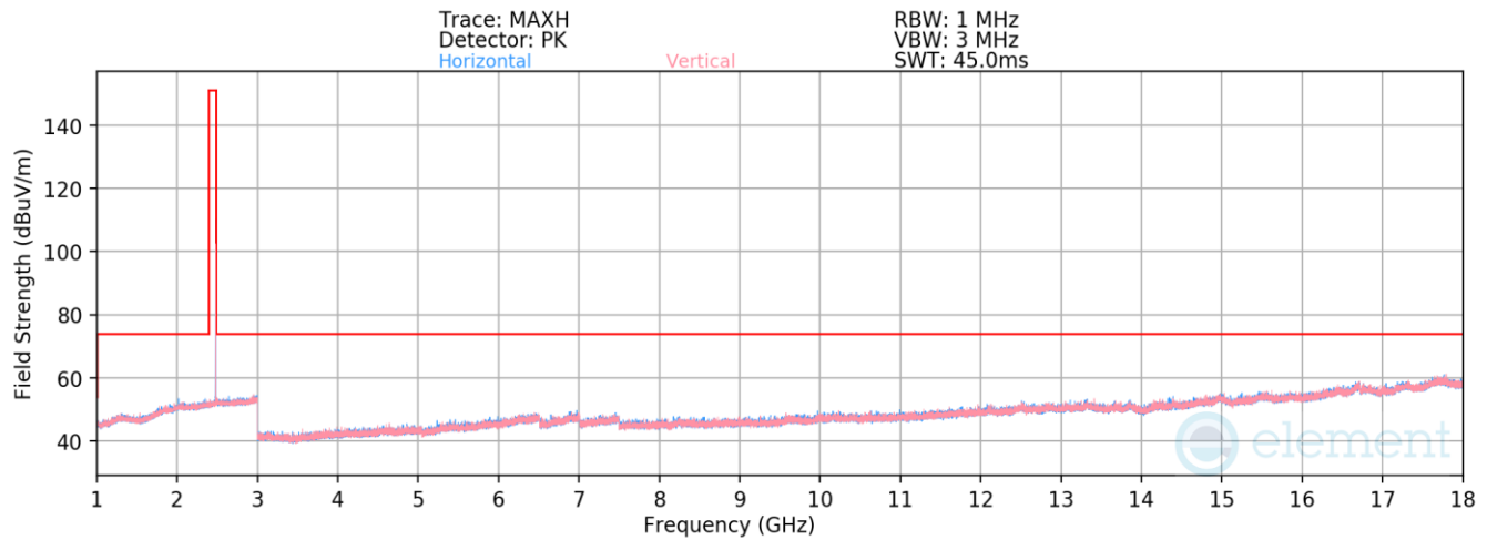
Plot 7-25. Radiated Spurious Emissions 1-18GHz (1Mbps – Ch. 39)
