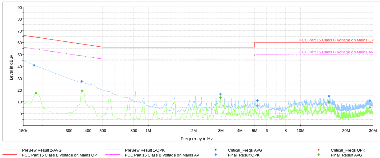
Plot 7-37. AC Line Conducted Plot with Bluetooth LE (L1, 1Mbps – Ch.19 with host PC and USB-C cable)
