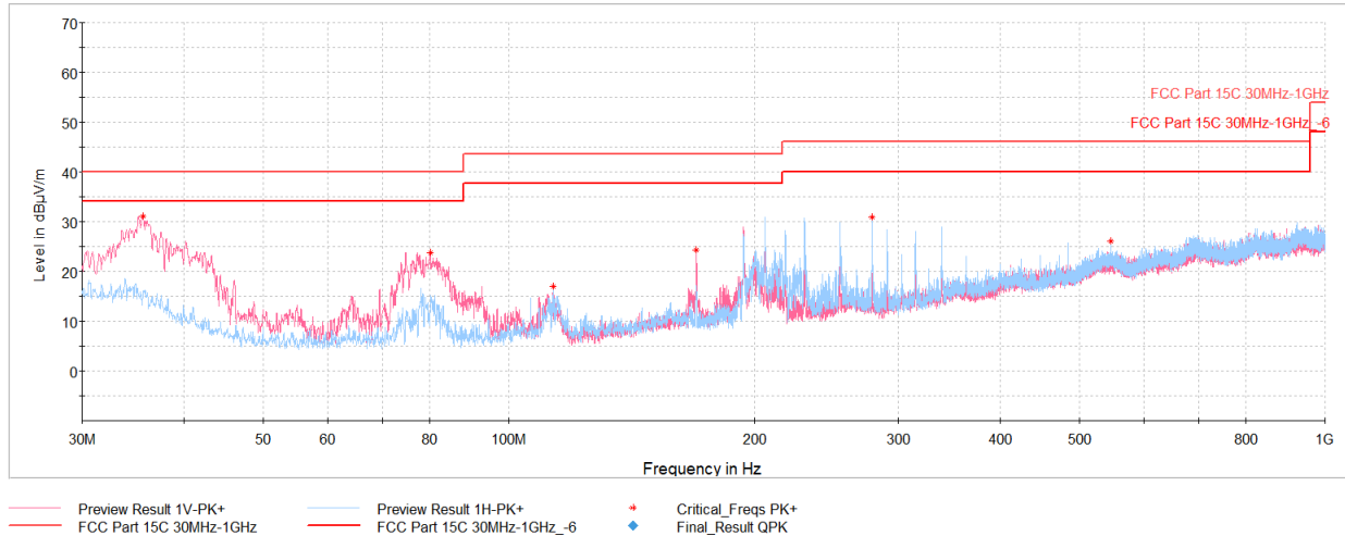
Plot 7-35. Radiated Spurious Emissions Below 1GHz (1Mbps – Ch.19, Pol. H & V, with AC/DC Adapter and USB-C cable)
