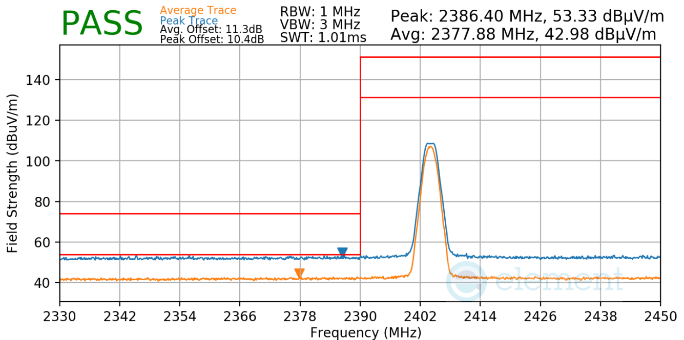
Plot 7-33. Radiated Restricted Lower Band Edge Measurement (Average & Peak)
