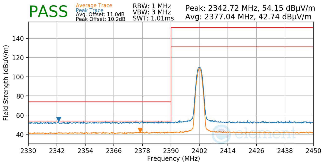
Plot 7-31. Radiated Restricted Lower Band Edge Measurement (Average & Peak)
