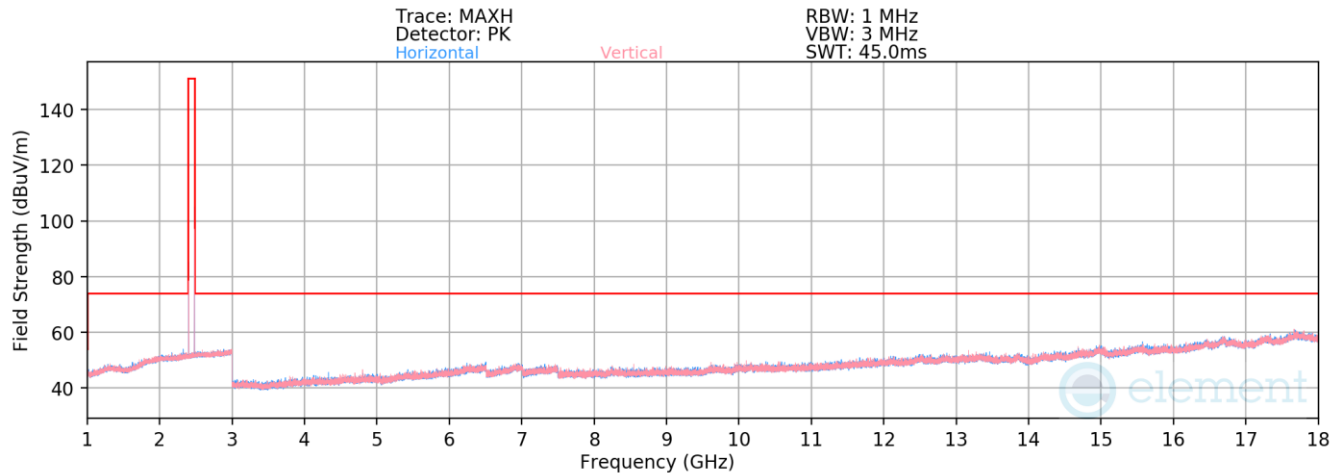
Plot 7-28. Radiated Spurious Emissions – Cot-Tx 1-18GHz
