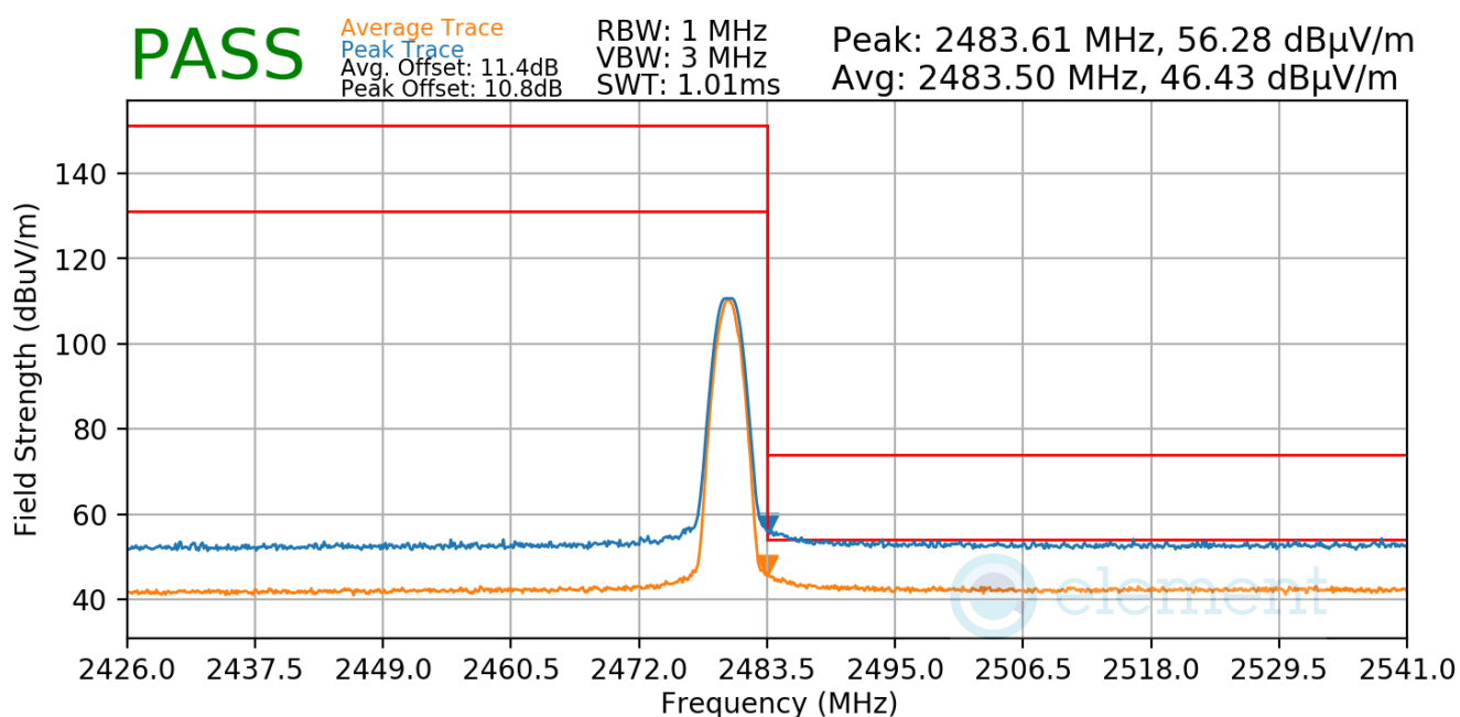
Plot 7-32. Radiated Restricted Upper Band Edge Measurement (Average & Peak)
