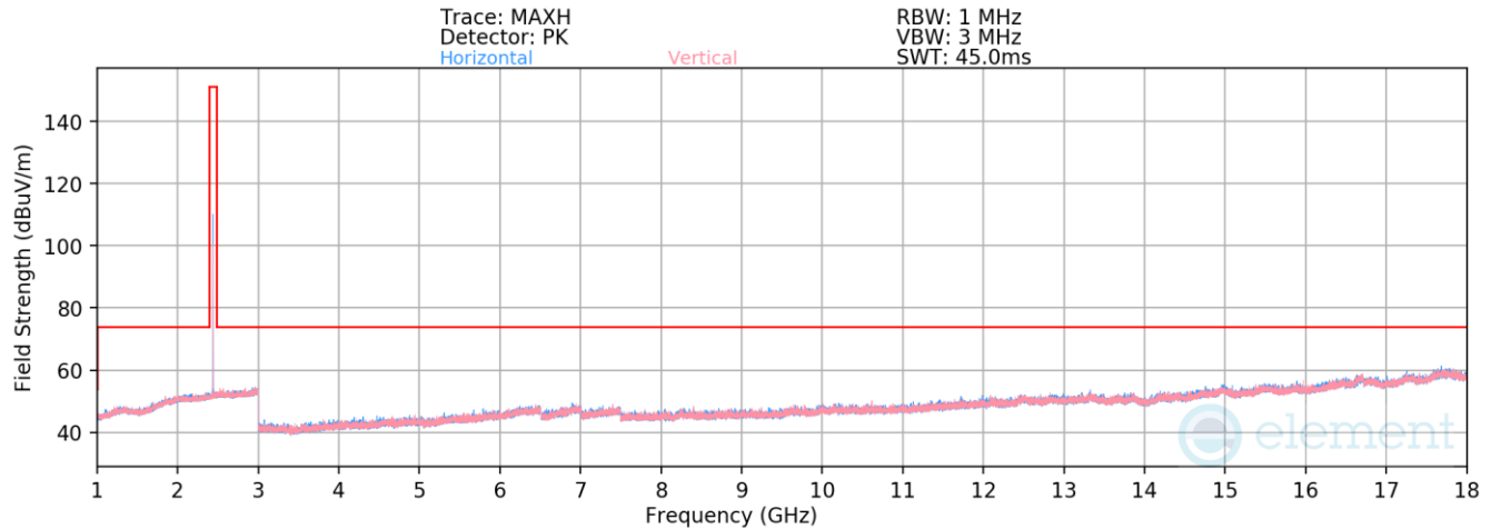
Plot 7-30. Radiated Spurious Emissions above 1GHz (BT GFSK – Ch. 39)
