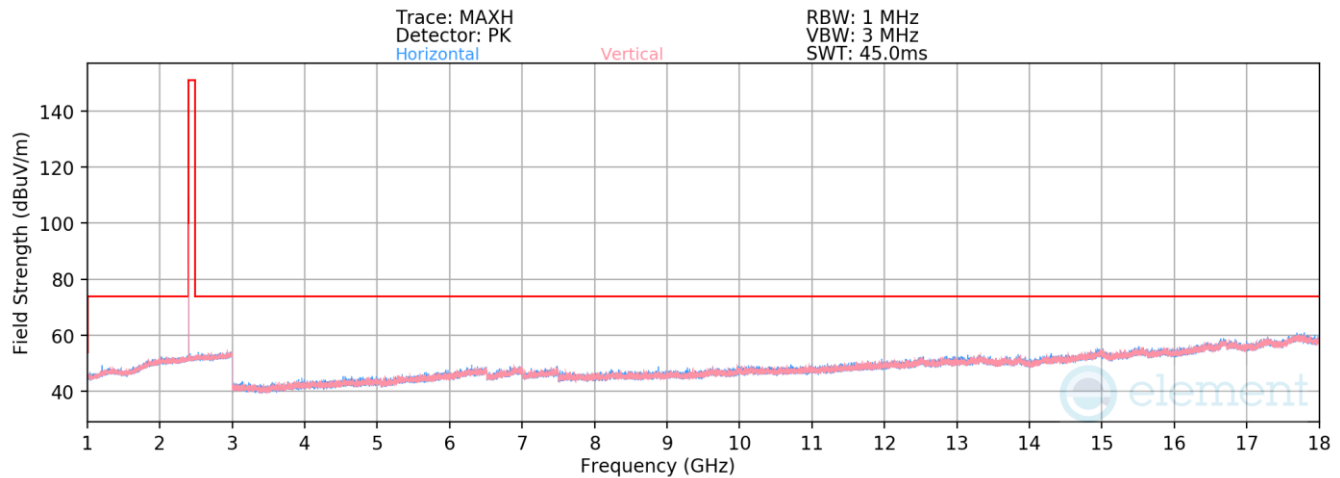
Plot 7-29. Radiated Spurious Emissions above 1GHz (BT GFSK – Ch. 0)
