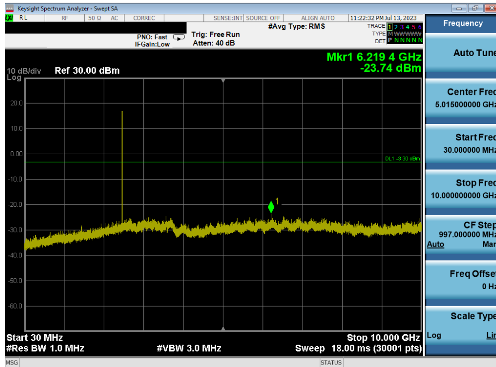
Plot 7-27. Conducted Spurious Plot (Bluetooth, GFSK – Ch. 78)
