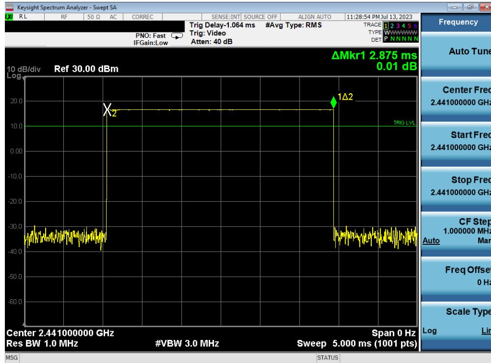
Plot 7-17. Time of Occupancy Plot (Bluetooth, GFSK)
