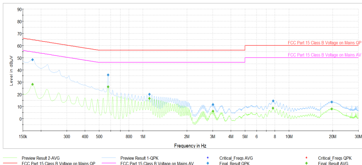
Plot 7-40. AC Line-Conducted Test Plot (N, GFSK – Ch.0, with host PC and USB-C cable)
