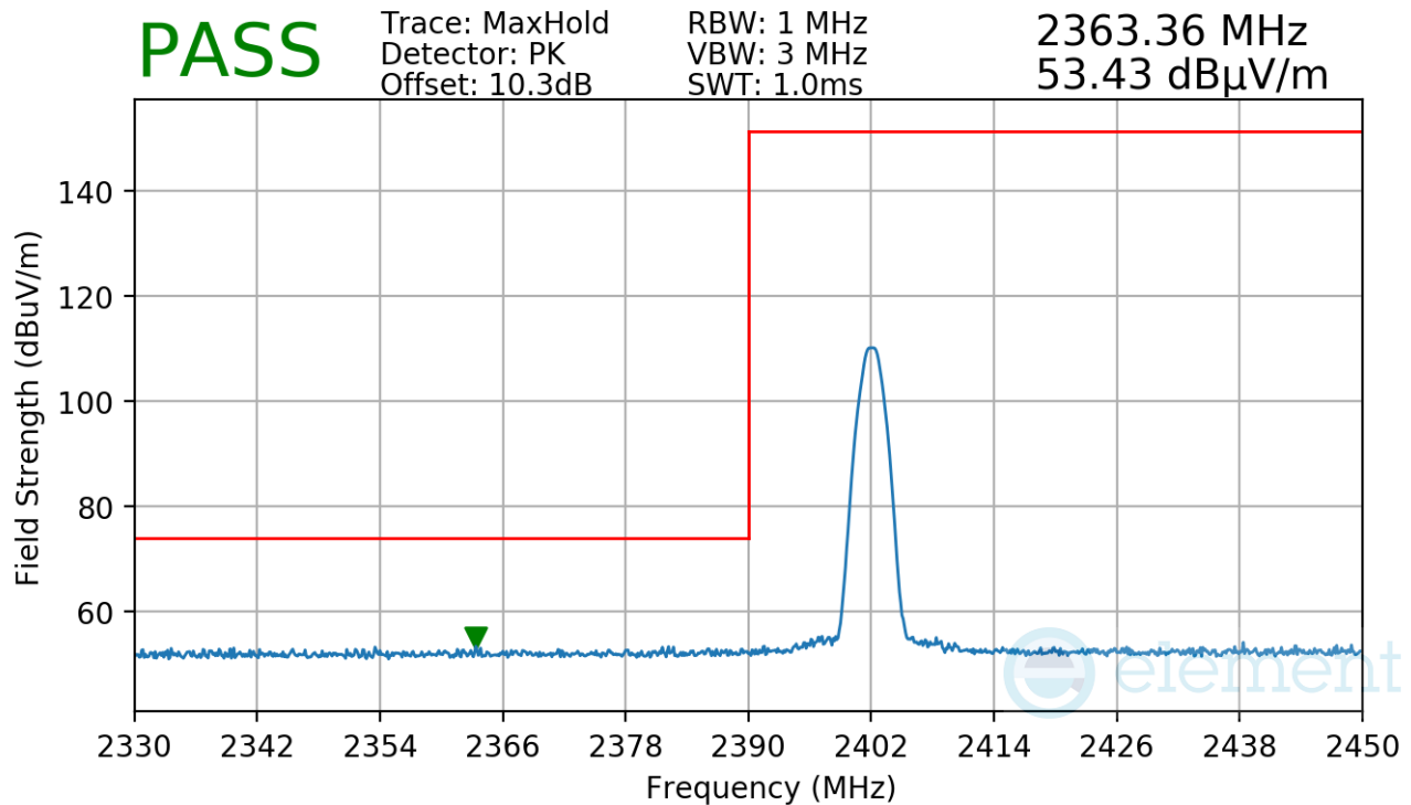
Plot 7-35. Radiated Restricted Lower Band Edge Measurement
