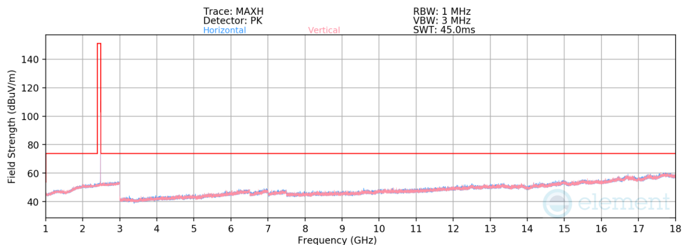
Plot 7-31. Radiated Spurious Emissions above 1GHz (BT GFSK – Ch. 78)
