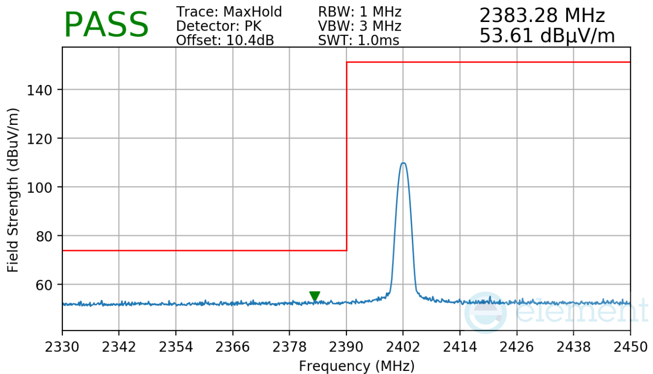
Plot 7-34. Radiated Restricted Lower Band Edge Measurement
