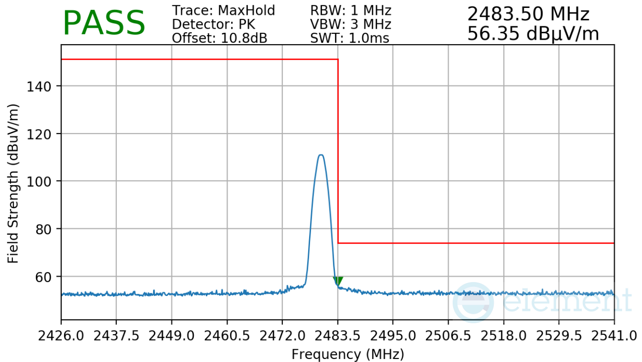
Plot 7-37. Radiated Restricted Upper Band Edge Measurement
