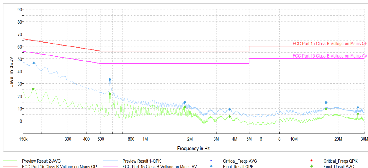
Plot 7-39. AC Line-Conducted Test Plot (L1, GFSK – Ch.0, with host PC and USB-C cable)
