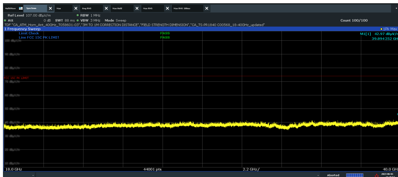
Plot 7-33. Radiated Spurious Emissions above 18GHz (BT GFSK – Ch. 0, Pol V)
