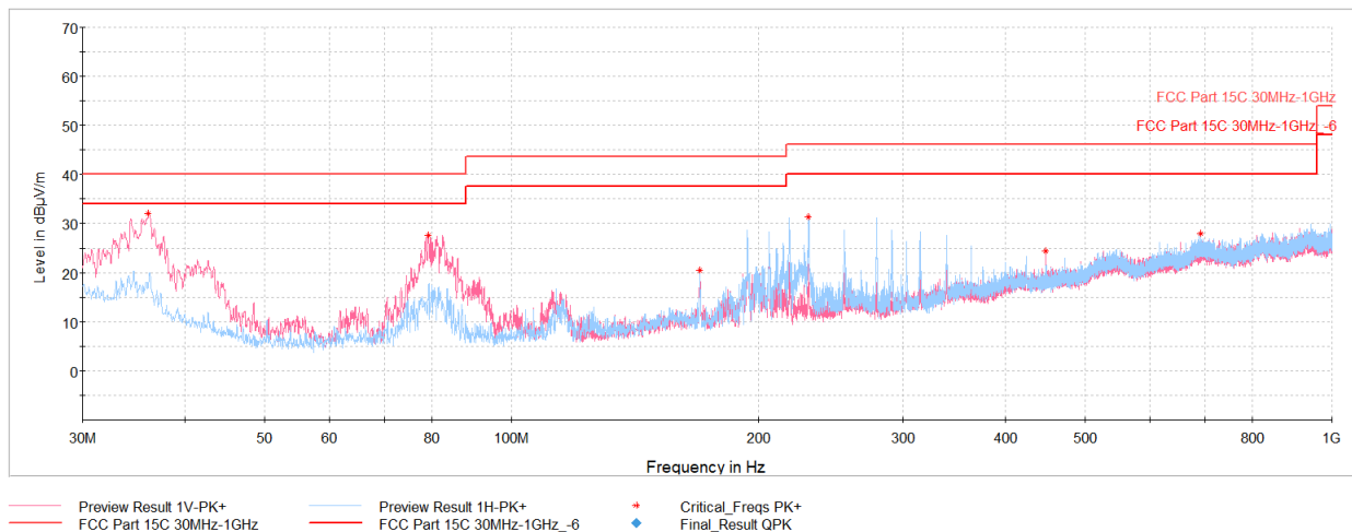
Plot 7-38. Radiated Spurious Emissions Below 1GHz (GFSK – Ch.0, with AC/DC Adapter and USB-C cable)
