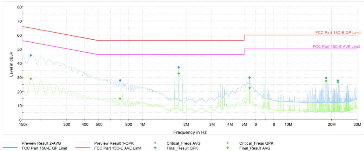
Plot 6-13. AC Line Conducted Plot (L1 - Mode 2, with Magnetic Charger & Laptop)
