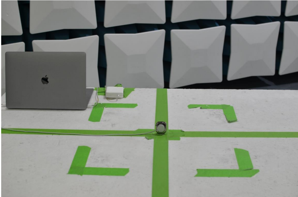
Figure 21: 30MHz-1GHz Test Setup (Front View)
