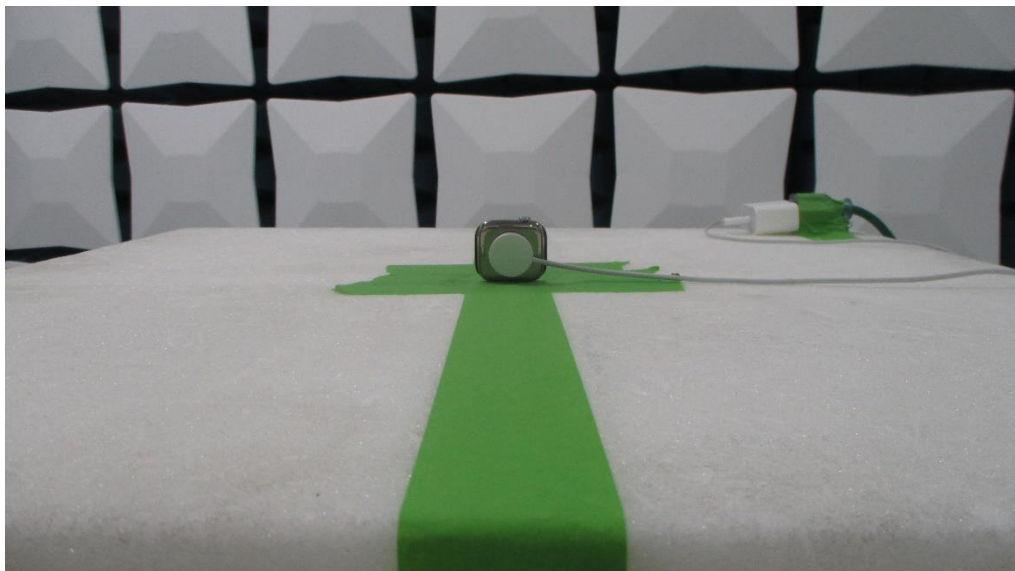
Figure 7: 1-18GHz Test Setup (Front View)
