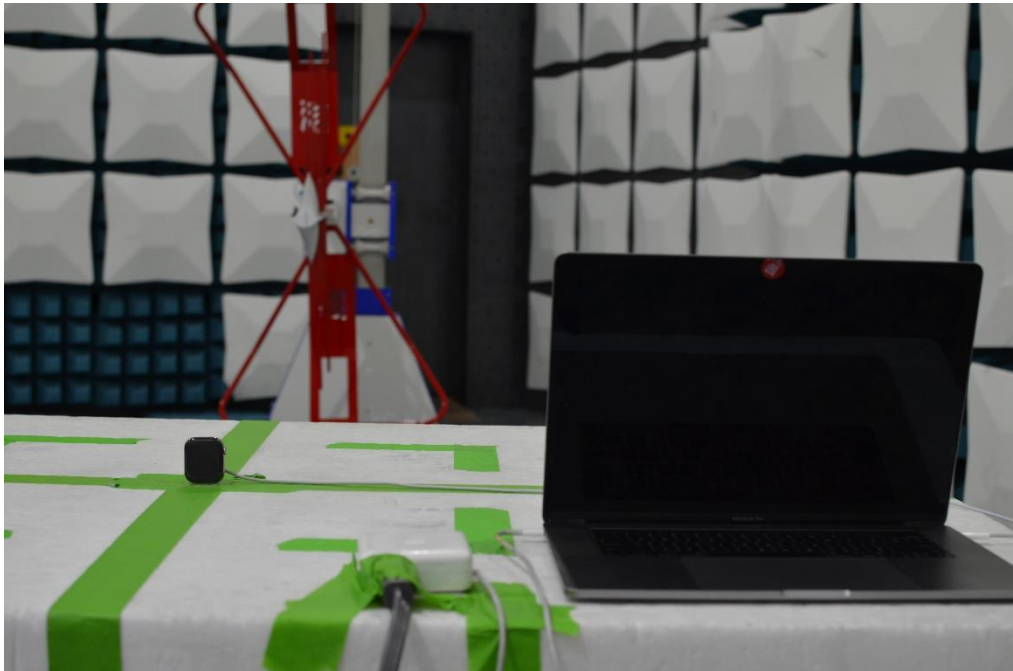
Figure 22: 30MHz-1GHz Test Setup (Rear View)
