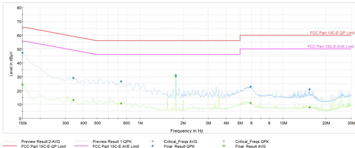
Plot 7-78. AC Line Conducted Plot 802.11b - Ch.6 (L1, with Laptop + Magnetic charger)
