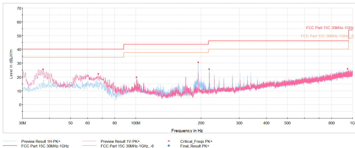
Plot 7-37. Radiated Spurious Emissions Below 1GHz (1Mbps, ePA – Ch.19, Pol. H & V, with AC/DC Adapter + Magnetic Charger)
