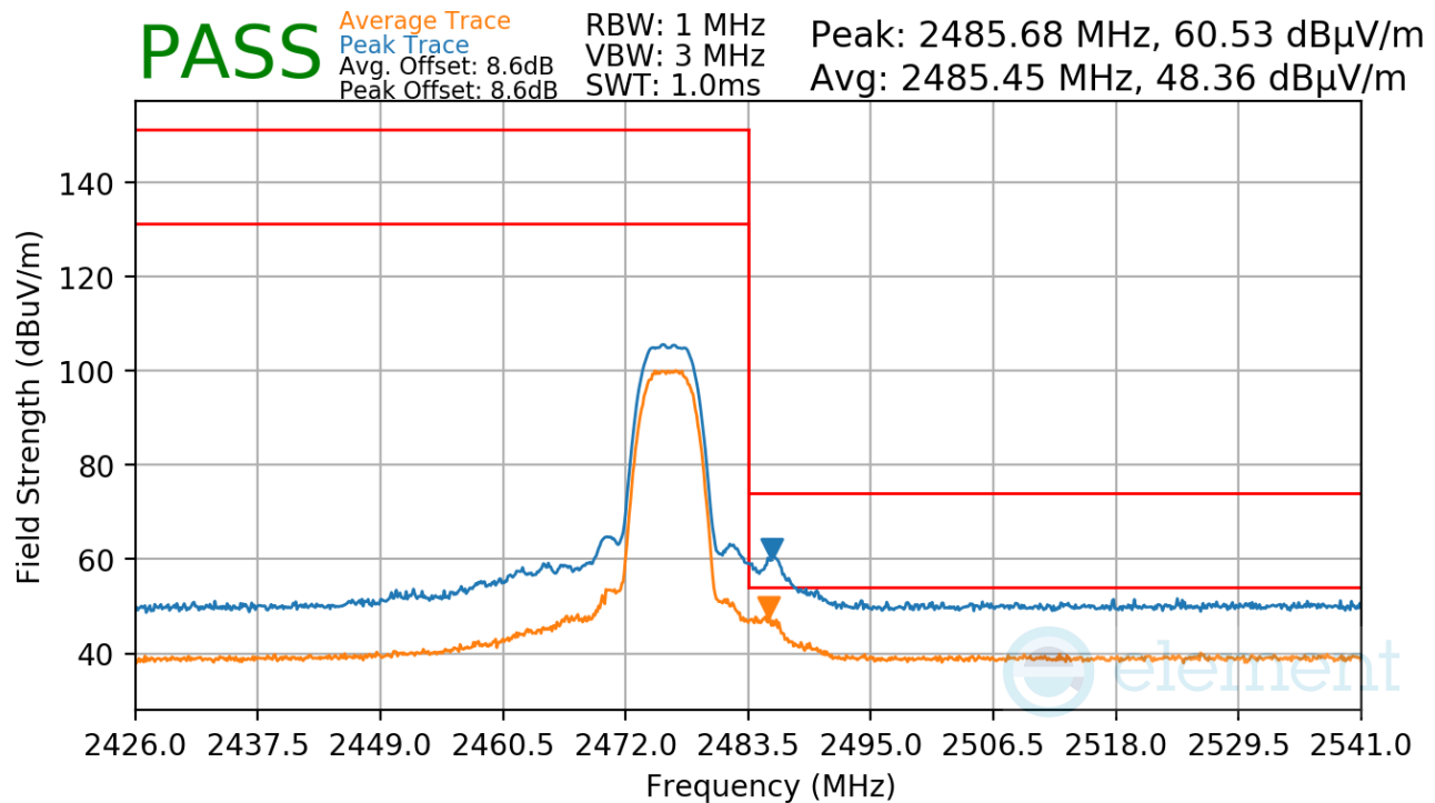
Plot 7-36. Radiated Restricted Upper Band Edge Measurement
