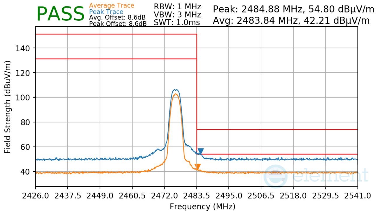
Plot 7-35. Radiated Restricted Upper Band Edge Measurement
