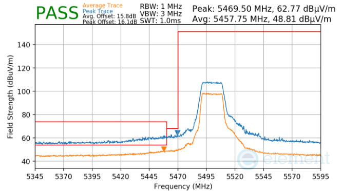
Plot 7-48. (Pk & Avg, Ch.100, 802.11n, MCS0)
