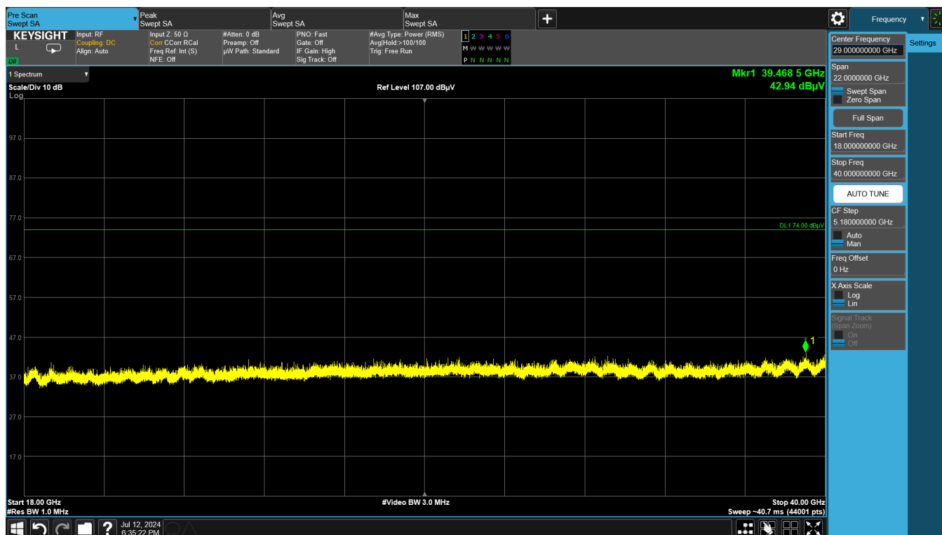
Plot 7-43. Radiated Spurious Emissions Simultaneous Transmission 18GHz – 40GHz Pol V
