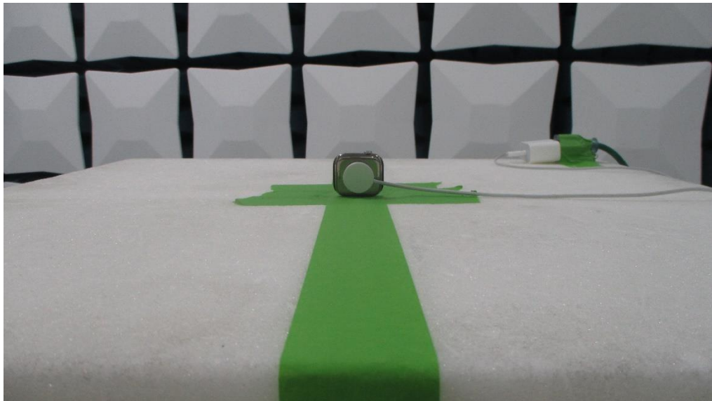
Figure 3: 1-18GHz Test Setup (Front View)
