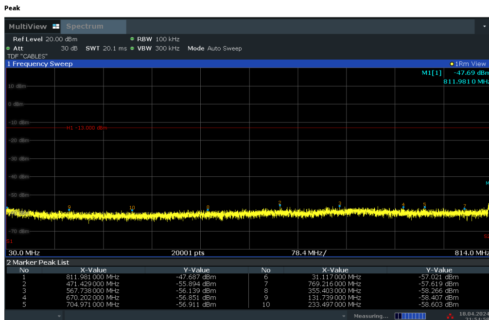
Plot 7-19. Conducted Spurious Plot (LTE Band 26 - 5MHz QPSK - RB Size 1, RB Offset 0 - High Channel)
