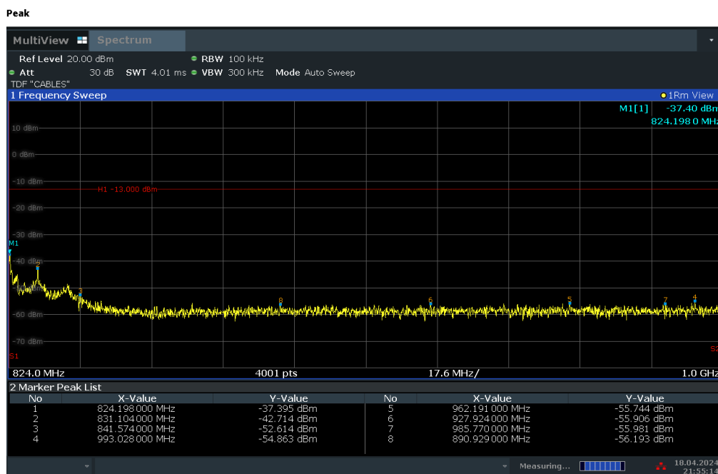
Plot 7-20. Conducted Spurious Plot (LTE Band 26 - 5MHz QPSK - RB Size 1, RB Offset 0 - High Channel)
