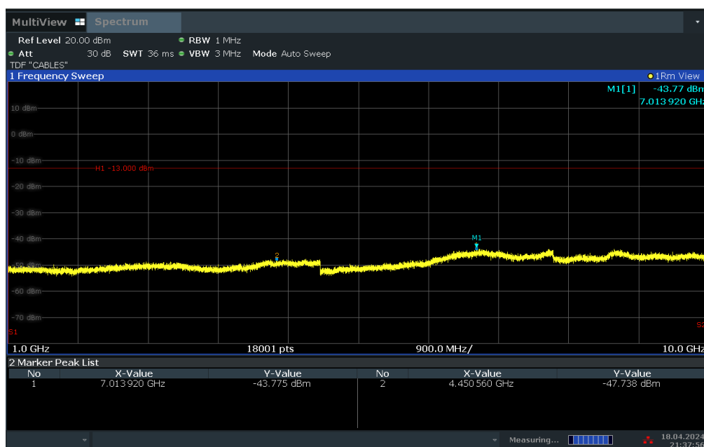
Plot 7-27. Conducted Spurious Plot (LTE Band 14 - 10MHz QPSK - RB Size 1, RB Offset 0 - Mid Channel)
