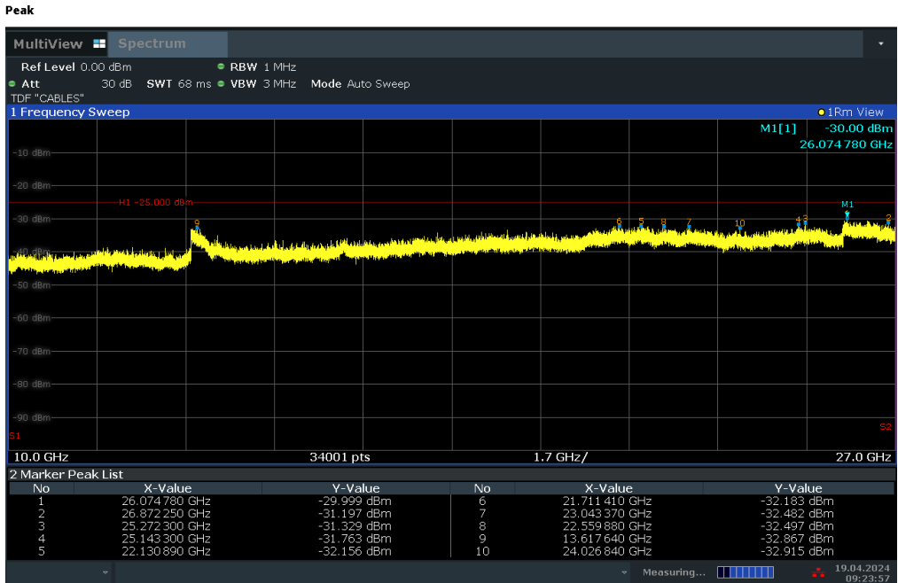
Plot 7-32. Conducted Spurious Plot (LTE Band 41 - 20MHz QPSK – RB Size 1, RB Offset 0 – Low Channel)
