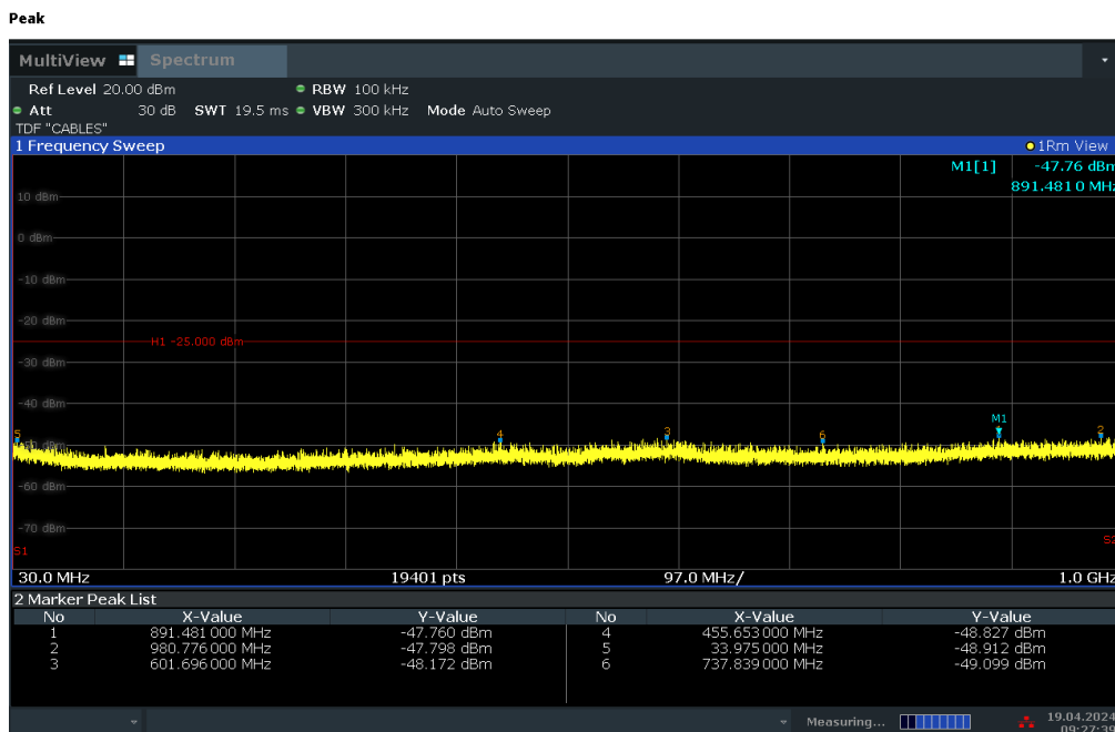
Plot 7-37. Conducted Spurious Plot (LTE Band 41 - 20MHz QPSK – RB Size 1, RB Offset 0 – High Channel)
