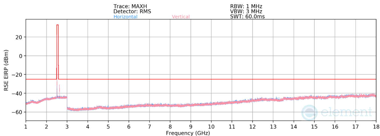
Plot 7-68. Antenna FCM Radiated Spurious Plot 1GHz – 18GHz (LTE Band 7)
