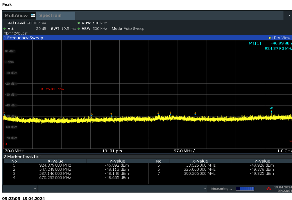
Plot 7-29. Conducted Spurious Plot (LTE Band 41 - 20MHz QPSK – RB Size 1, RB Offset 0 – Low Channel)
