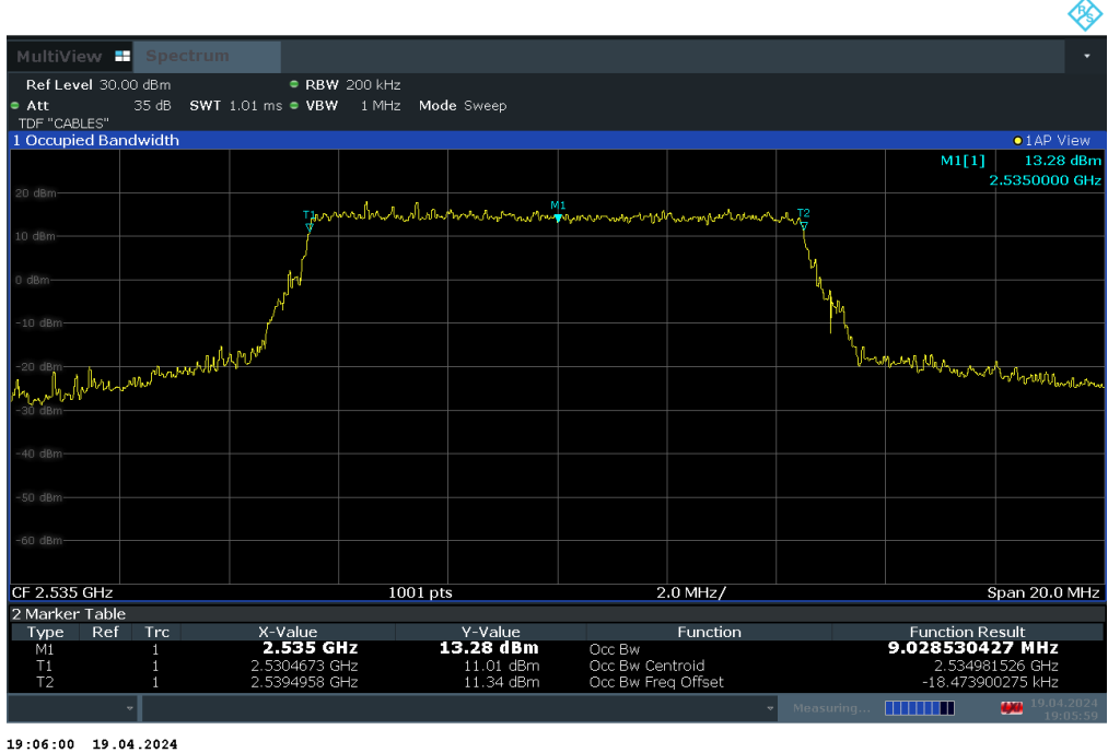
Plot 7-3. Occupied Bandwidth Plot (LTE Band 7 - 10MHz QPSK - Full RB)
