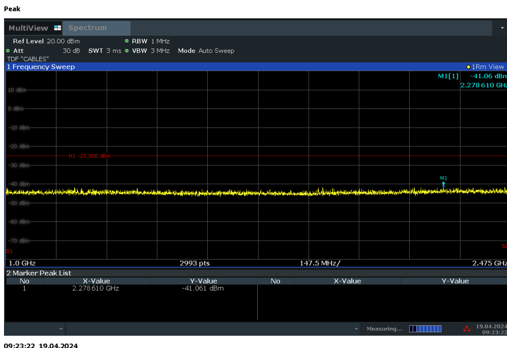
Plot 7-30. Conducted Spurious Plot (LTE Band 41 - 20MHz QPSK – RB Size 1, RB Offset 0 – Low Channel)
