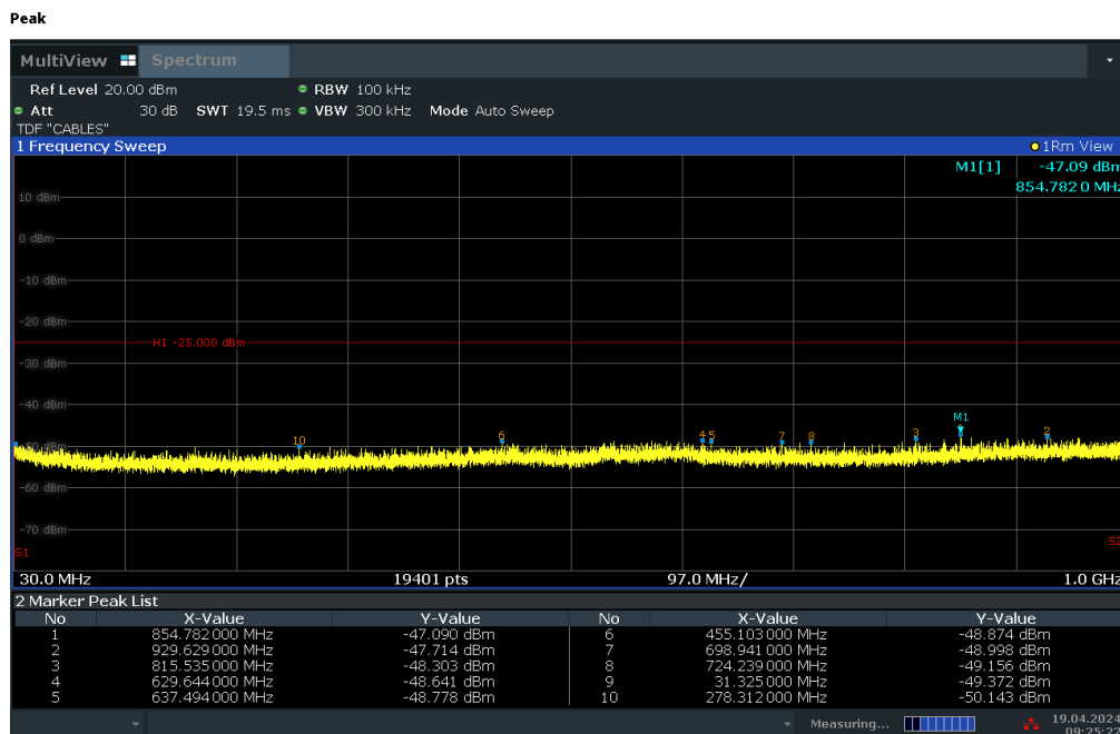
Plot 7-33. Conducted Spurious Plot (LTE Band 41 - 20MHz QPSK – RB Size 1, RB Offset 0 – Mid Channel)
