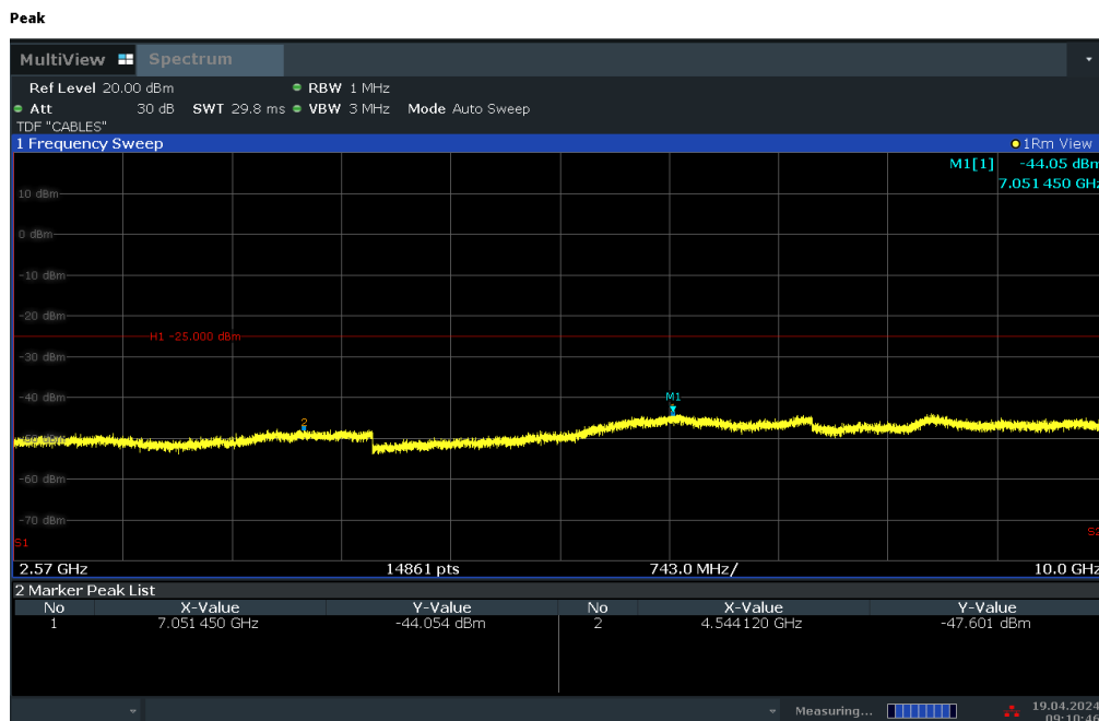
Plot 7-19. Conducted Spurious Plot (LTE Band 7 - 20MHz QPSK – RB Size 1, RB Offset 0 – Low Channel)
