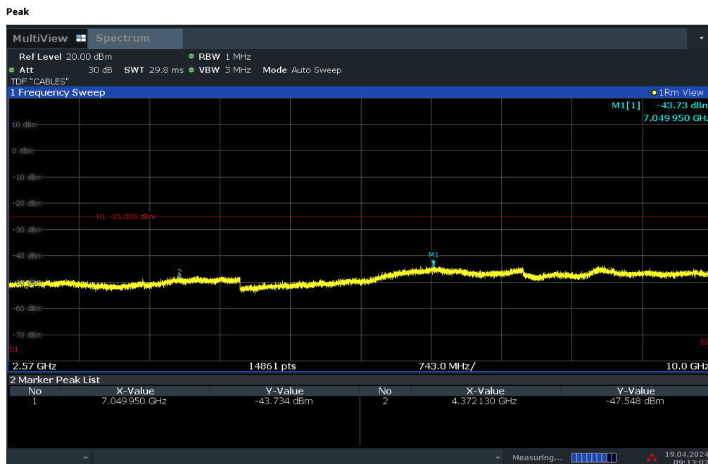
Plot 7-23. Conducted Spurious Plot (LTE Band 7 - 20MHz QPSK – RB Size 1, RB Offset 0 – Mid Channel)
