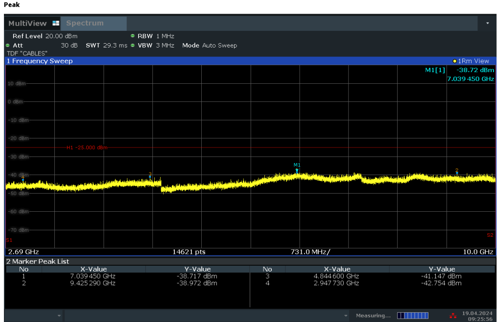
Plot 7-35. Conducted Spurious Plot (LTE Band 41 - 20MHz QPSK – RB Size 1, RB Offset 0 – Mid Channel)
