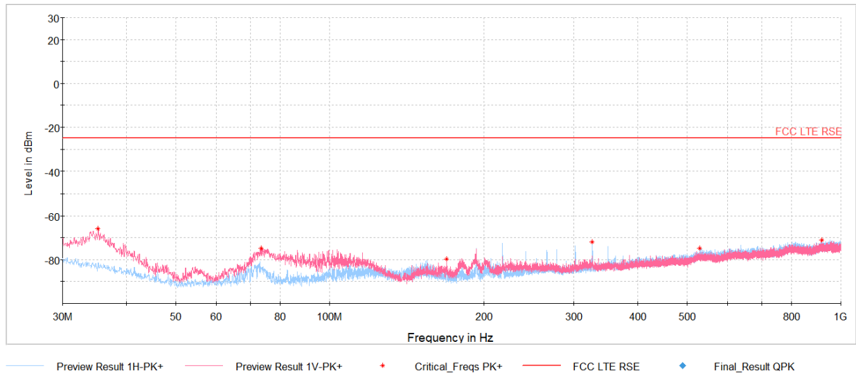
Plot 7-72. Antenna FCM Radiated Spurious Emissions -Simultaneous Transmission 30MHz – 1GHz
