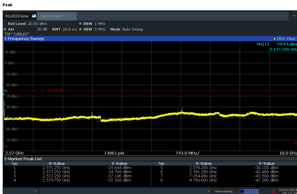
Plot 7-27. Conducted Spurious Plot (LTE Band 7 - 20MHz QPSK – RB Size 1, RB Offset 0 – High Channel)
