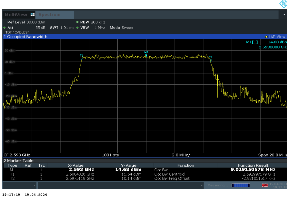
Plot 7-11. Occupied Bandwidth Plot (LTE Band 41 - 10MHz QPSK - Full RB)
