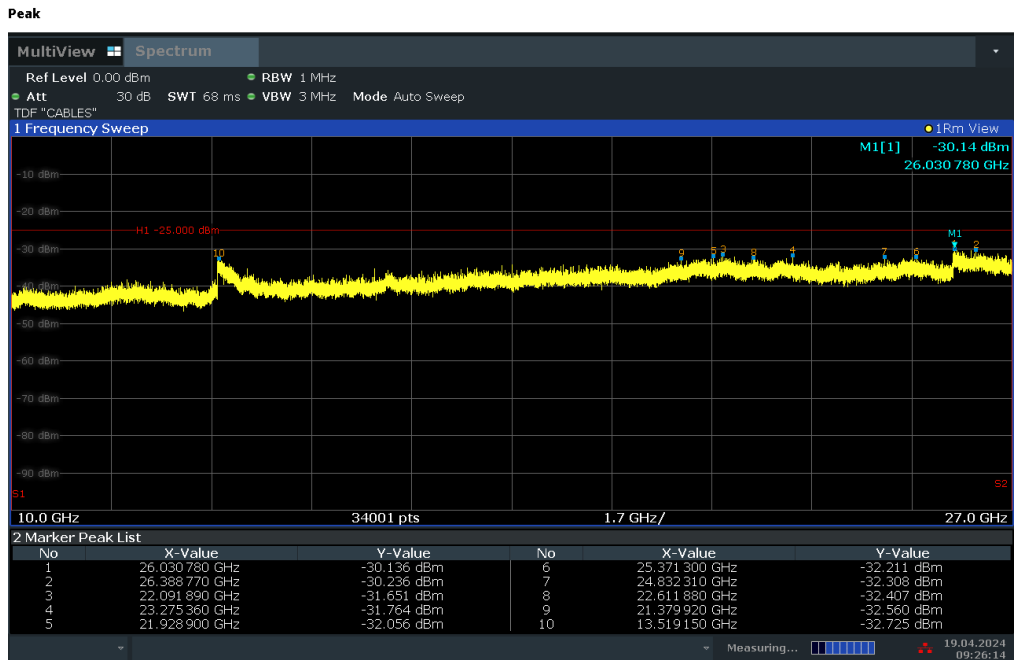
Plot 7-36. Conducted Spurious Plot (LTE Band 41 - 20MHz QPSK – RB Size 1, RB Offset 0 – Mid Channel)
