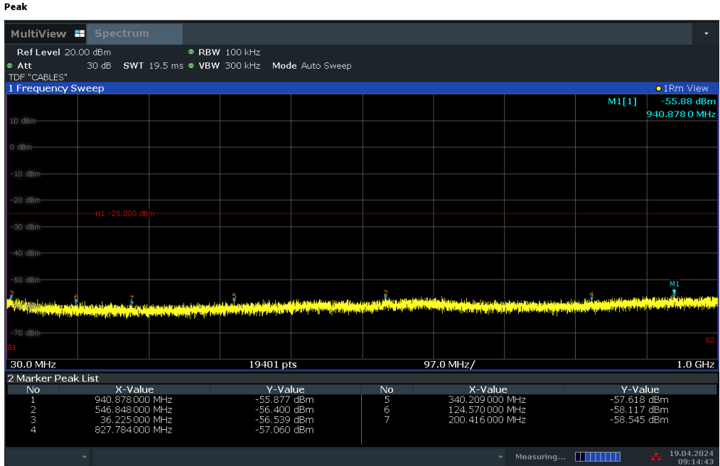
Plot 7-25. Conducted Spurious Plot (LTE Band 7 - 20MHz QPSK – RB Size 1, RB Offset 0 – High Channel)
