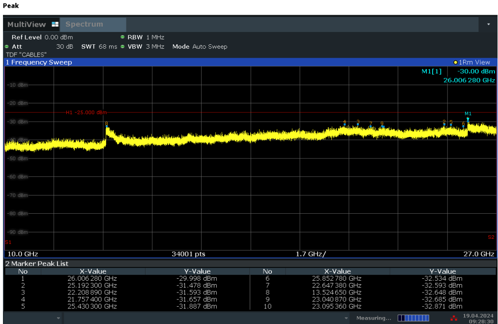
Plot 7-40. Conducted Spurious Plot (LTE Band 41 - 20MHz QPSK – RB Size 1, RB Offset 0 – High Channel)
