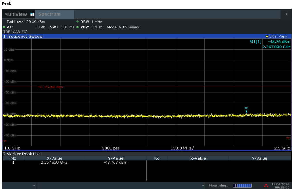
Plot 7-26. Conducted Spurious Plot (LTE Band 7 - 20MHz QPSK – RB Size 1, RB Offset 0 – High Channel)
