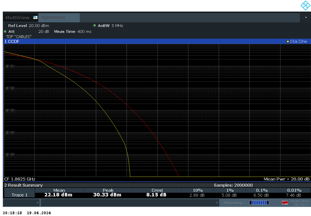
Plot 7-95. PAR Plot (LTE Band 25 - 5MHz 16-QAM - Full RB Configuration)
