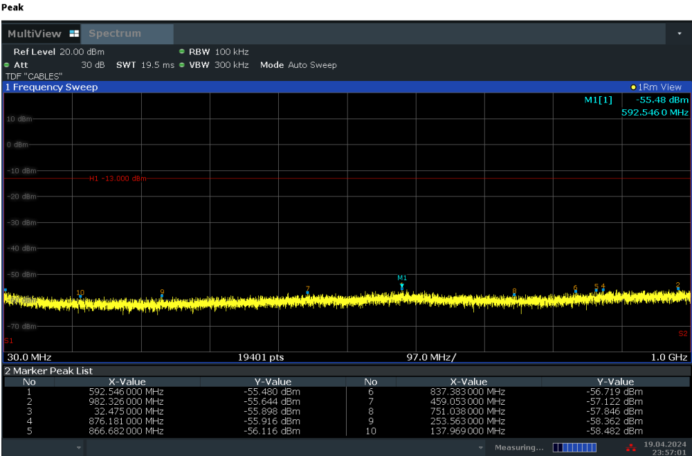
Plot 7-34. Conducted Spurious Plot (WCDMA Ch. 9538)
