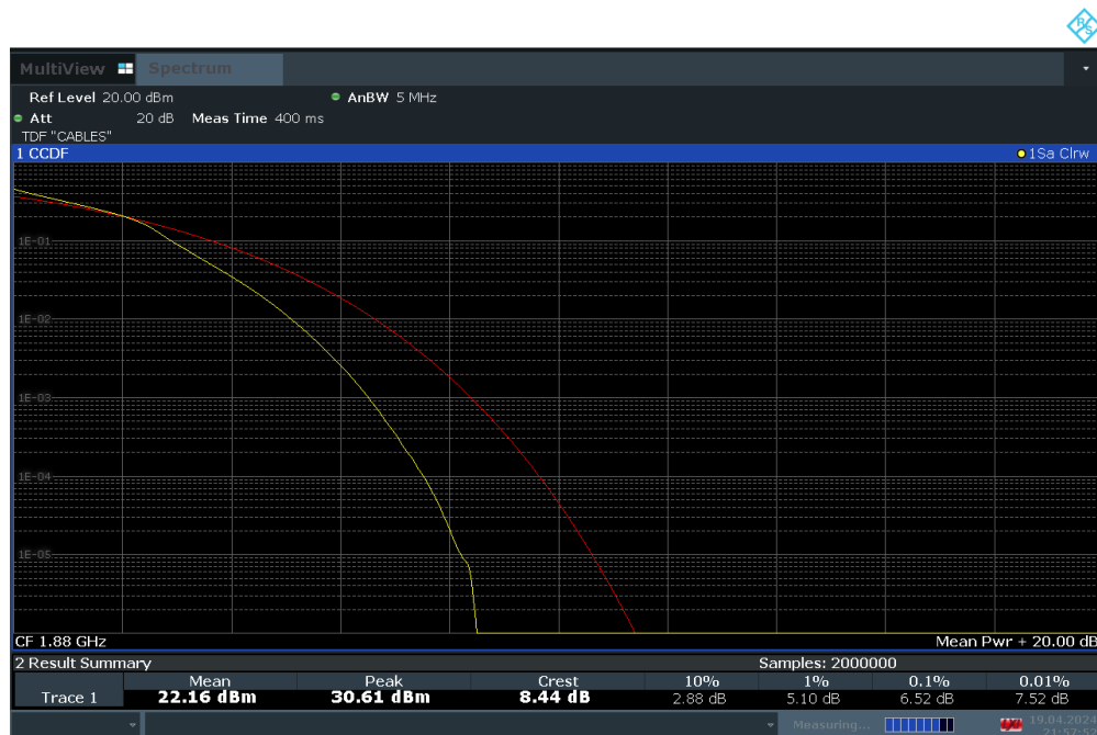
Plot 7-107. PAR Plot (LTE Band 2 - 5MHz 16-QAM - Full RB Configuration)
