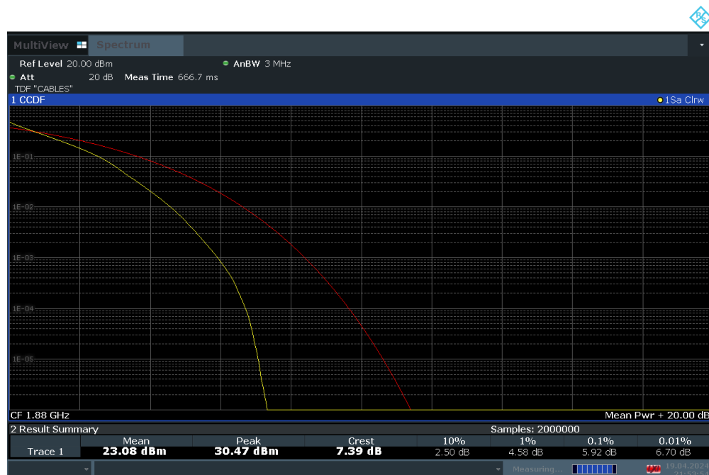
Plot 7-104. PAR Plot (LTE Band 2 - 3MHz QPSK - Full RB Configuration)
