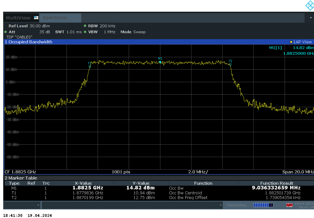
Plot 7-7. Occupied Bandwidth Plot (LTE Band 25/2 - 10MHz QPSK - Full RB Configuration)
