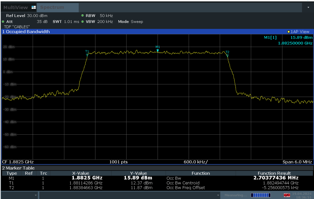
Plot 7-3. Occupied Bandwidth Plot (LTE Band 25/2 - 3MHz QPSK - Full RB Configuration)
