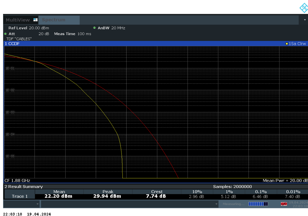
Plot 7-111. PAR Plot (LTE Band 2 - 15MHz 16-QAM - Full RB Configuration)
