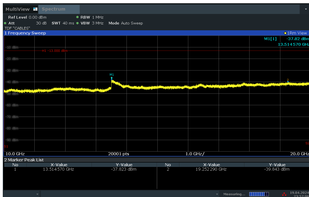
Plot 7-29. Conducted Spurious Plot (WCDMA Ch. 9262)
