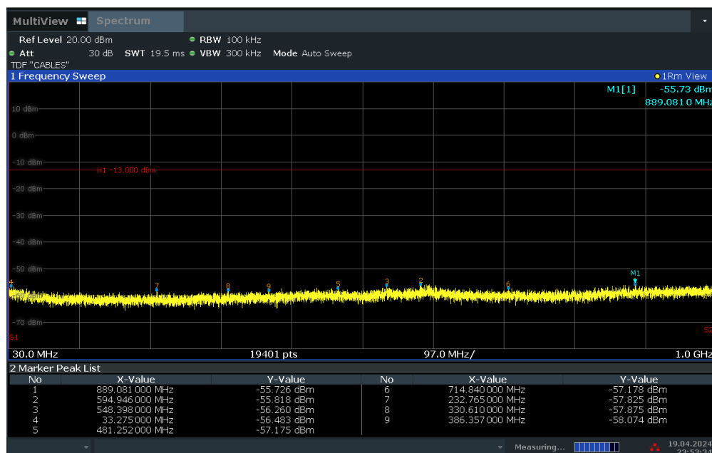
Plot 7-30. Conducted Spurious Plot (WCDMA Ch. 9400)
