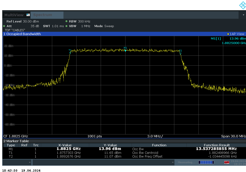
Plot 7-9. Occupied Bandwidth Plot (LTE Band 25/2 - 15MHz QPSK - Full RB Configuration)
