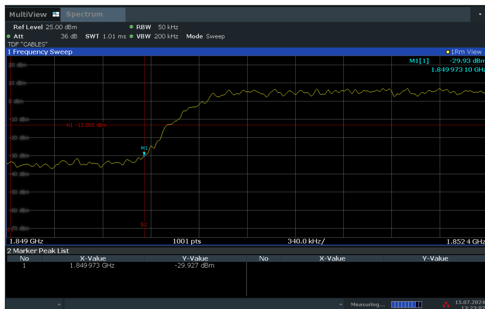
Plot 7-86. Lower Band Edge Plot (WCDMA PCS – Ch. 9262)
