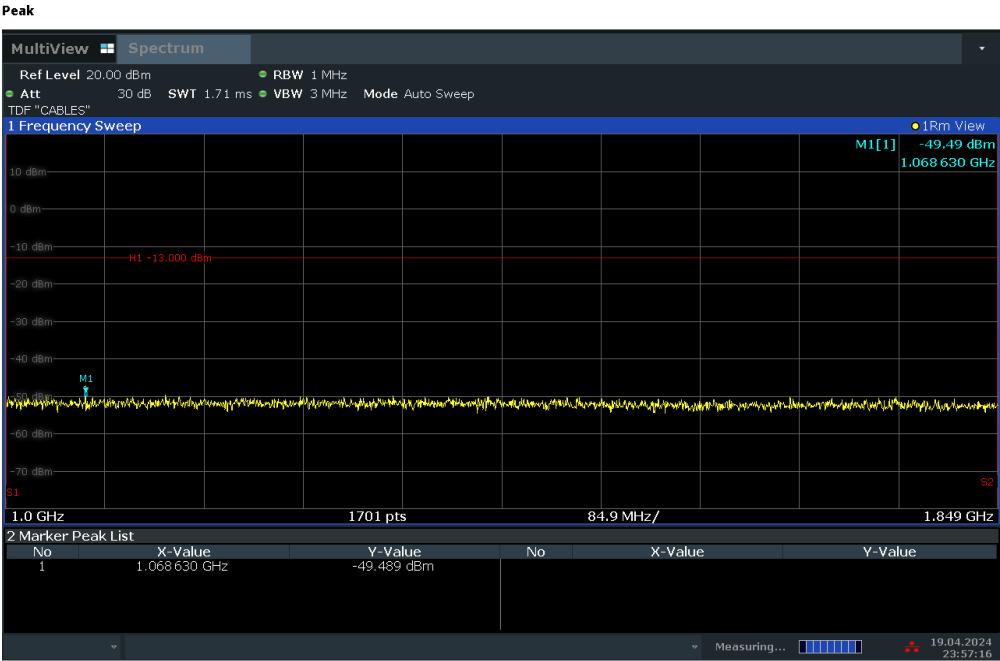
Plot 7-35. Conducted Spurious Plot (WCDMA Ch. 9538)
