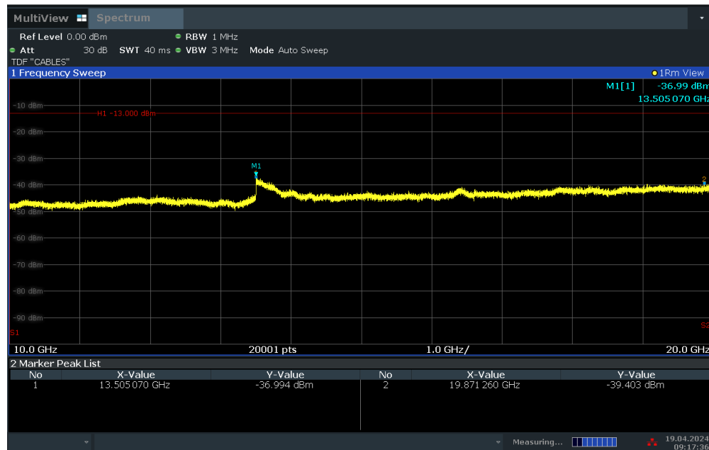
Plot 7-17. Conducted Spurious Plot (LTE Band 25/2 - 20MHz QPSK - RB Size 1, RB Offset 0 - Low Channel)
