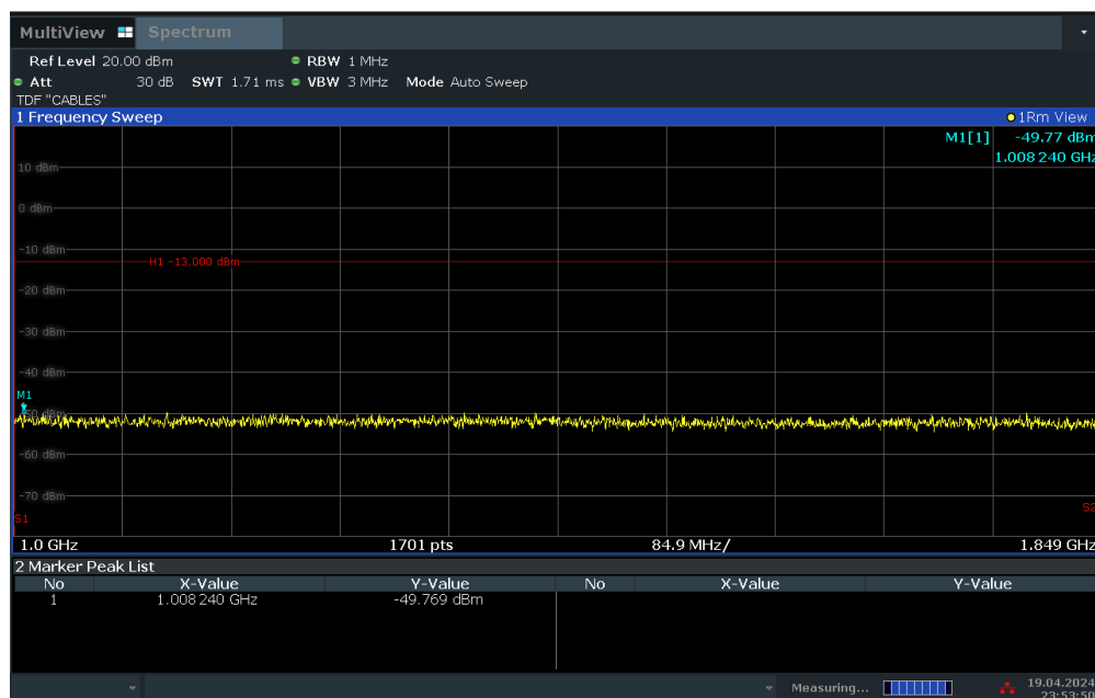
Plot 7-31. Conducted Spurious Plot (WCDMA Ch. 9400)
