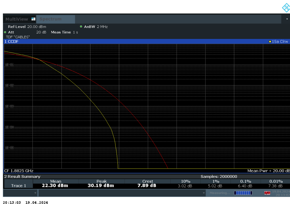
Plot 7-91. PAR Plot (LTE Band 25 - 1.4MHz 16-QAM - Full RB Configuration)
