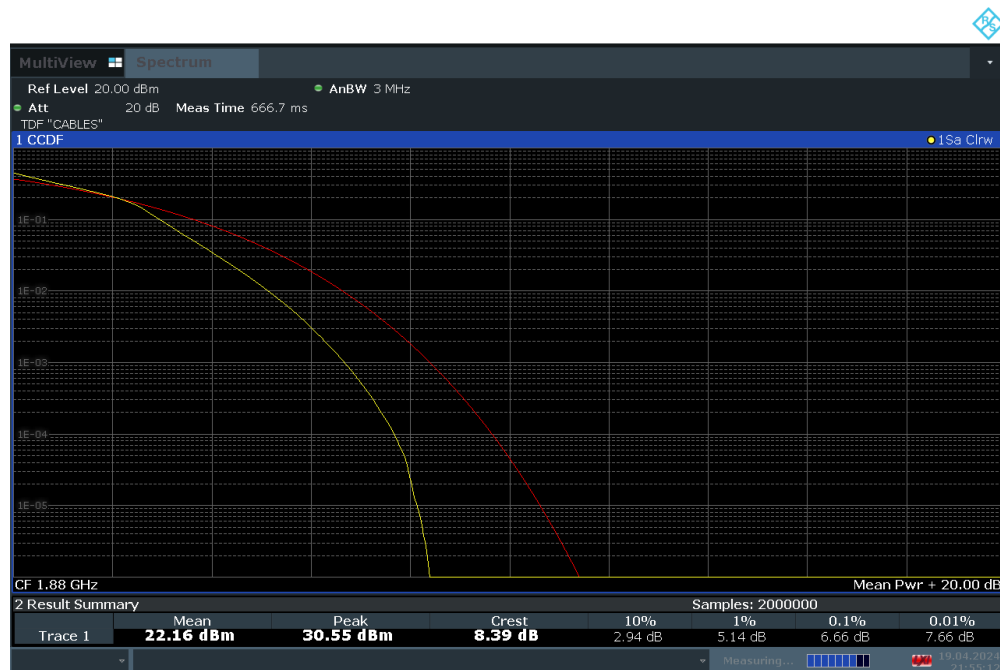
Plot 7-105. PAR Plot (LTE Band 2 - 3MHz 16-QAM - Full RB Configuration)
