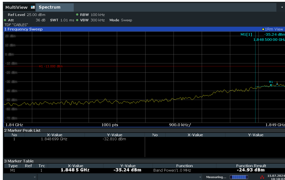
Plot 7-87. Extended Lower Band Edge Plot (WCDMA PCS – Ch. 9262)
