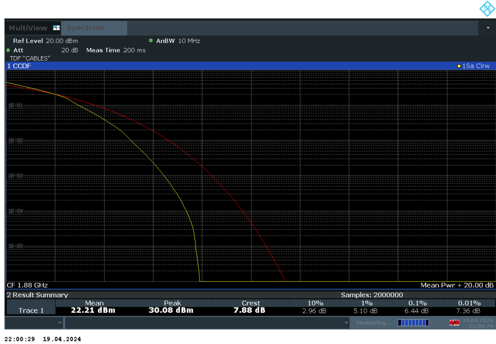
Plot 7-109. PAR Plot (LTE Band 2 - 10MHz 16-QAM - Full RB Configuration)
