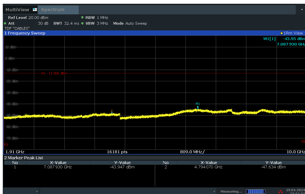
Plot 7-28. Conducted Spurious Plot (WCDMA Ch. 9262)
