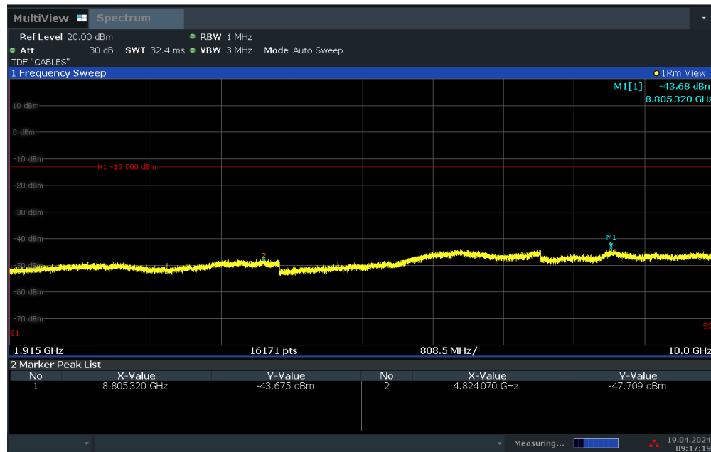
Plot 7-16. Conducted Spurious Plot (LTE Band 25/2 - 20MHz QPSK - RB Size 1, RB Offset 0 - Low Channel)
