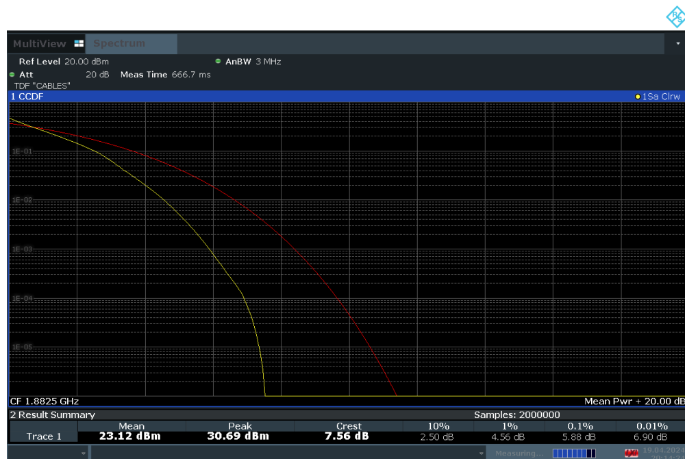
Plot 7-92. PAR Plot (LTE Band 25 - 3MHz QPSK - Full RB Configuration)
