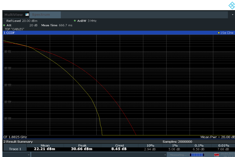
Plot 7-93. PAR Plot (LTE Band 25 - 3MHz 16-QAM - Full RB Configuration)
